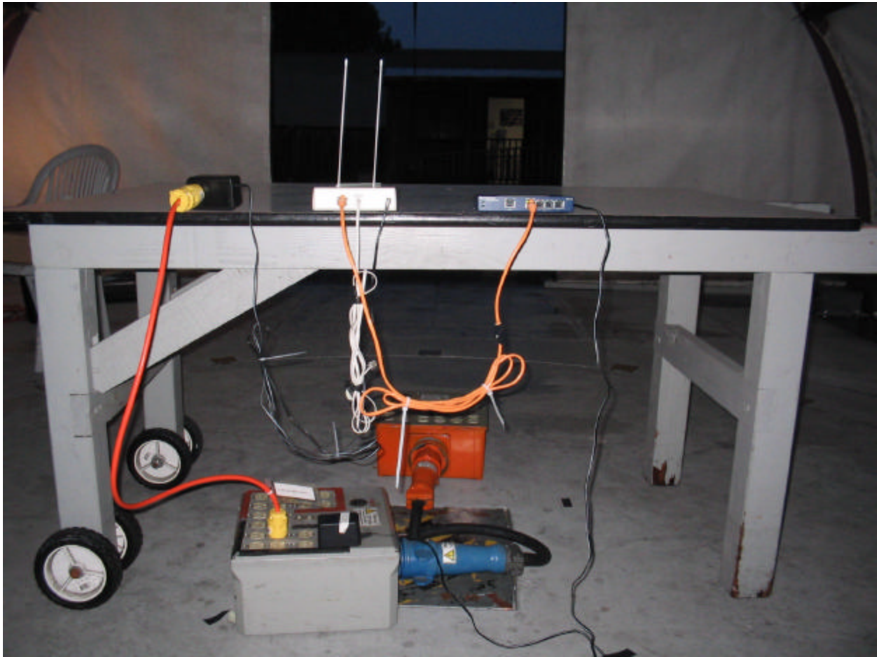
Figure 3: Radiated Emissions - Rear View
