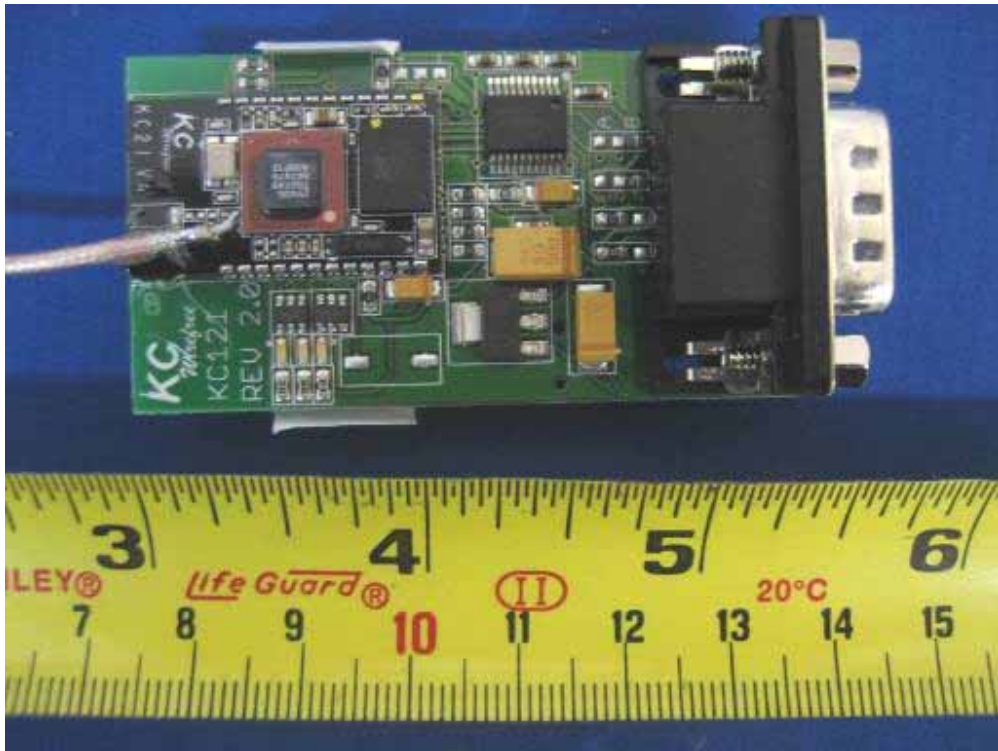
Bluetooth Radio Module- Top View
