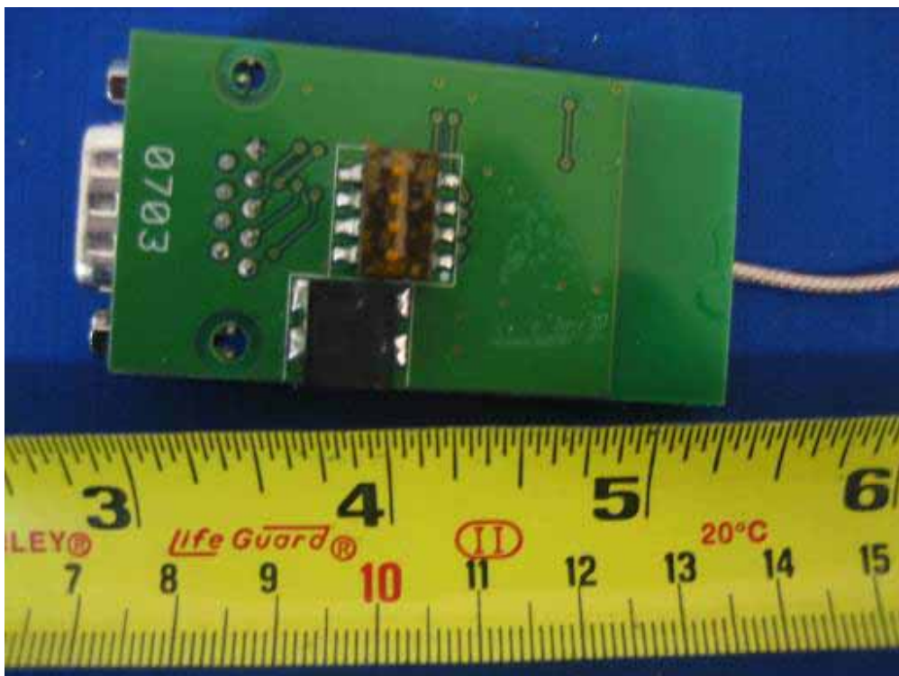
Bluetooth Radio Module- Bottom View
