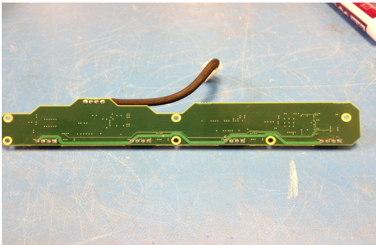
Legacy receiver Interconnect Board Bottom
