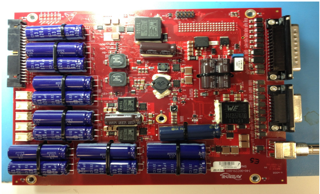
Power Supply Board Top
