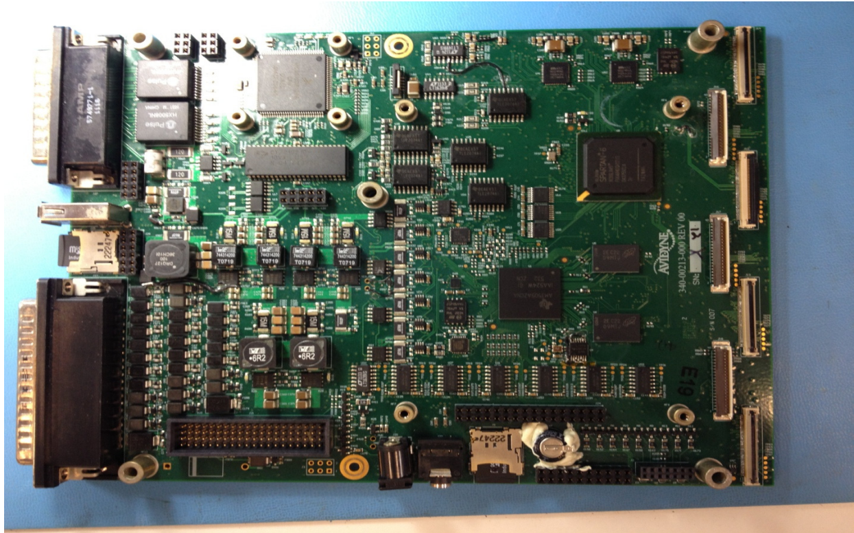
Processor Board Top
