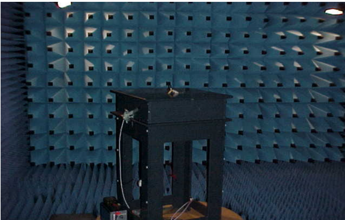
Radiated spurious emission 1-26 GHz
