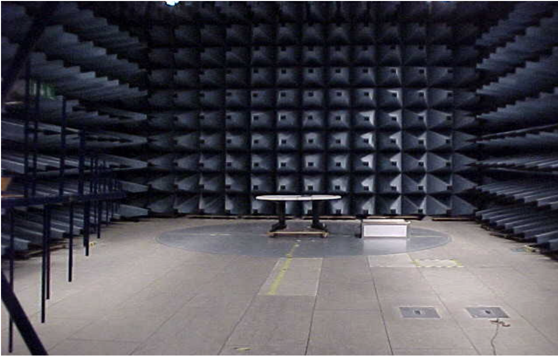
Radiated spurious emission 30-1000 MHz
