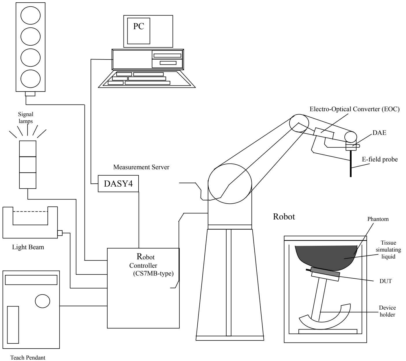
Fig. 5.1 DASY4 system
