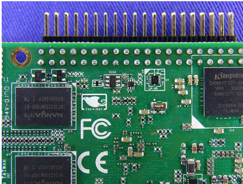
(26) EUT Photo
