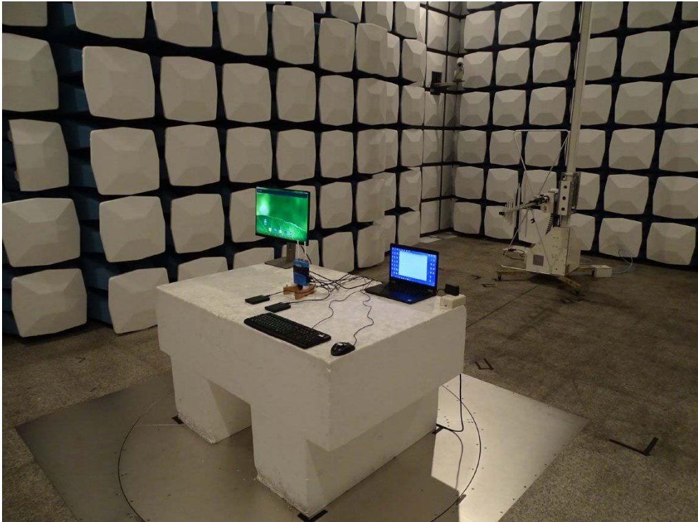
Back View of Radiated Test_ATM020-W050U
