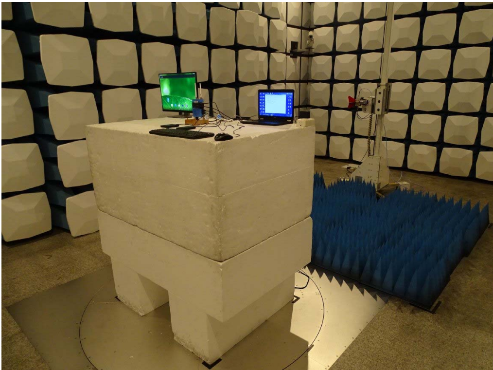
Front View of Radiated Test (Horn)_ATM020-W050U
