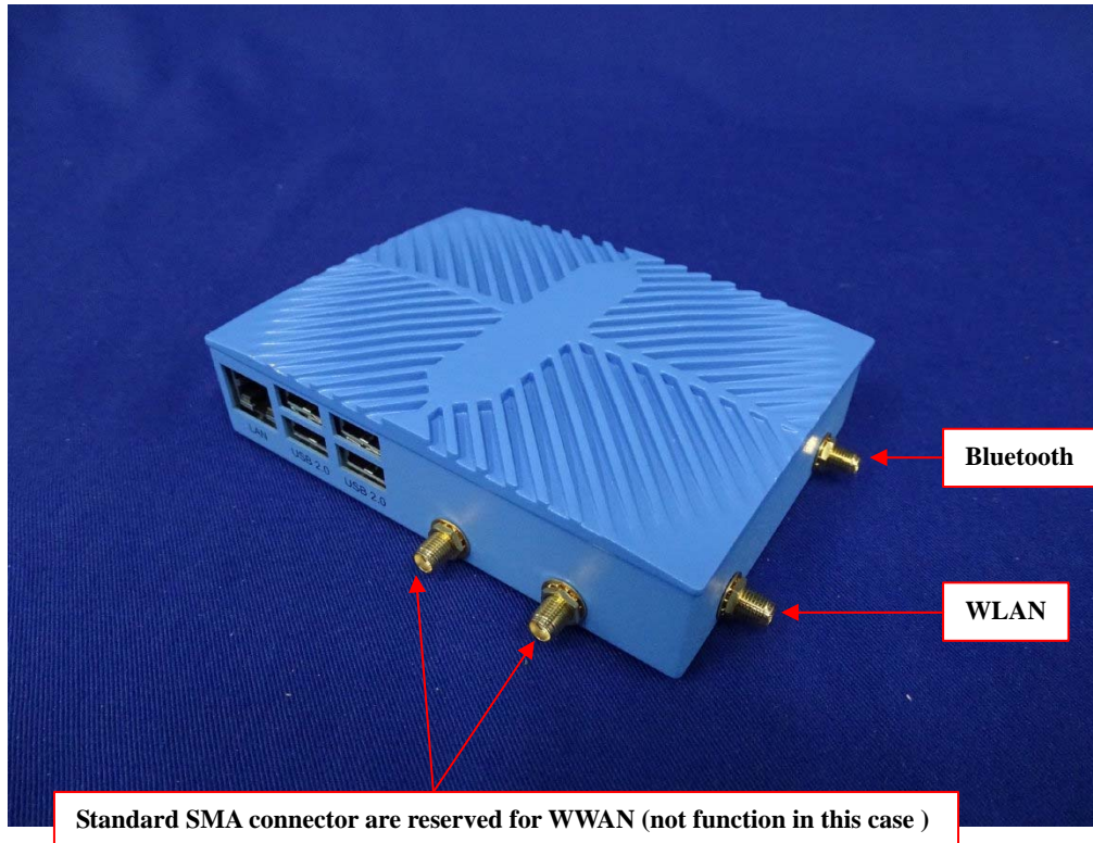
(1) EUT Photo
