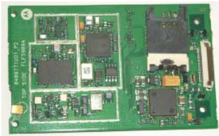
Photograph 9-2: Front side of module main board with shields removed.
