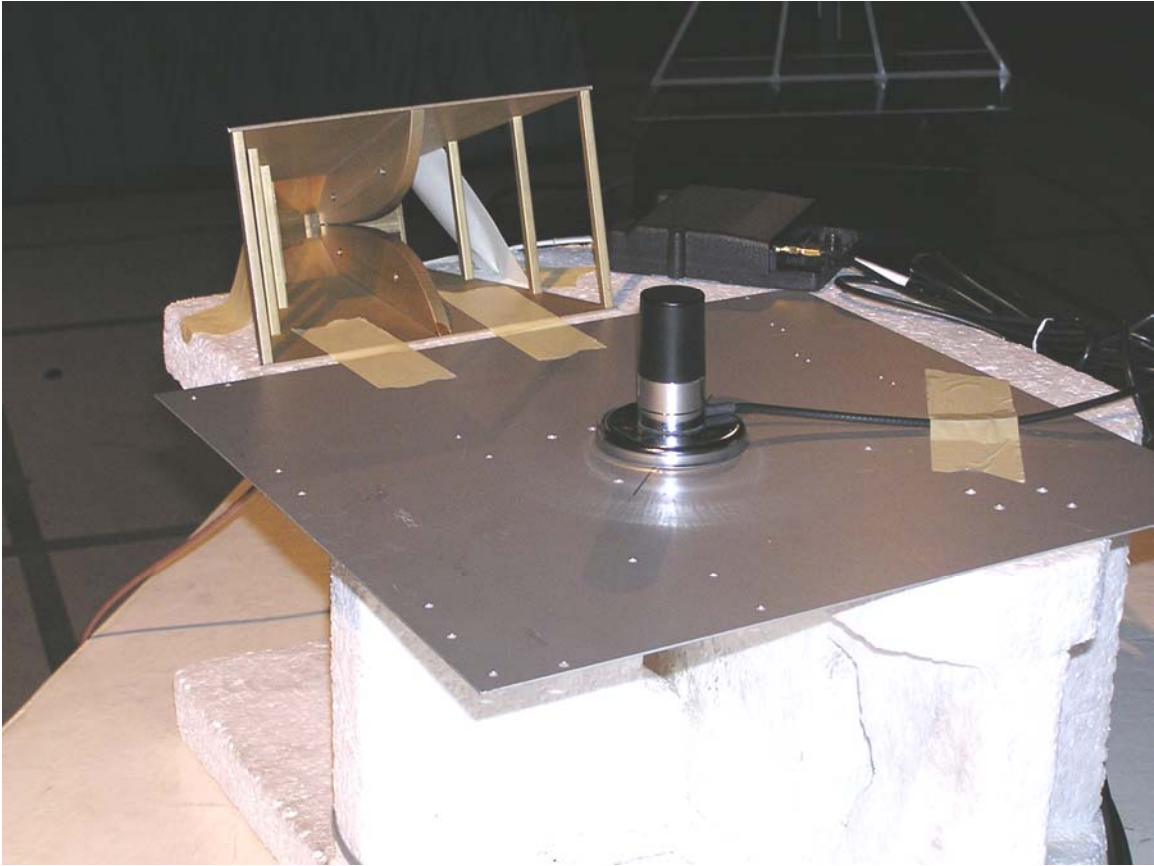
Test setup – Radiated Emissions (Horn antenna was used for signaling purpose only)
