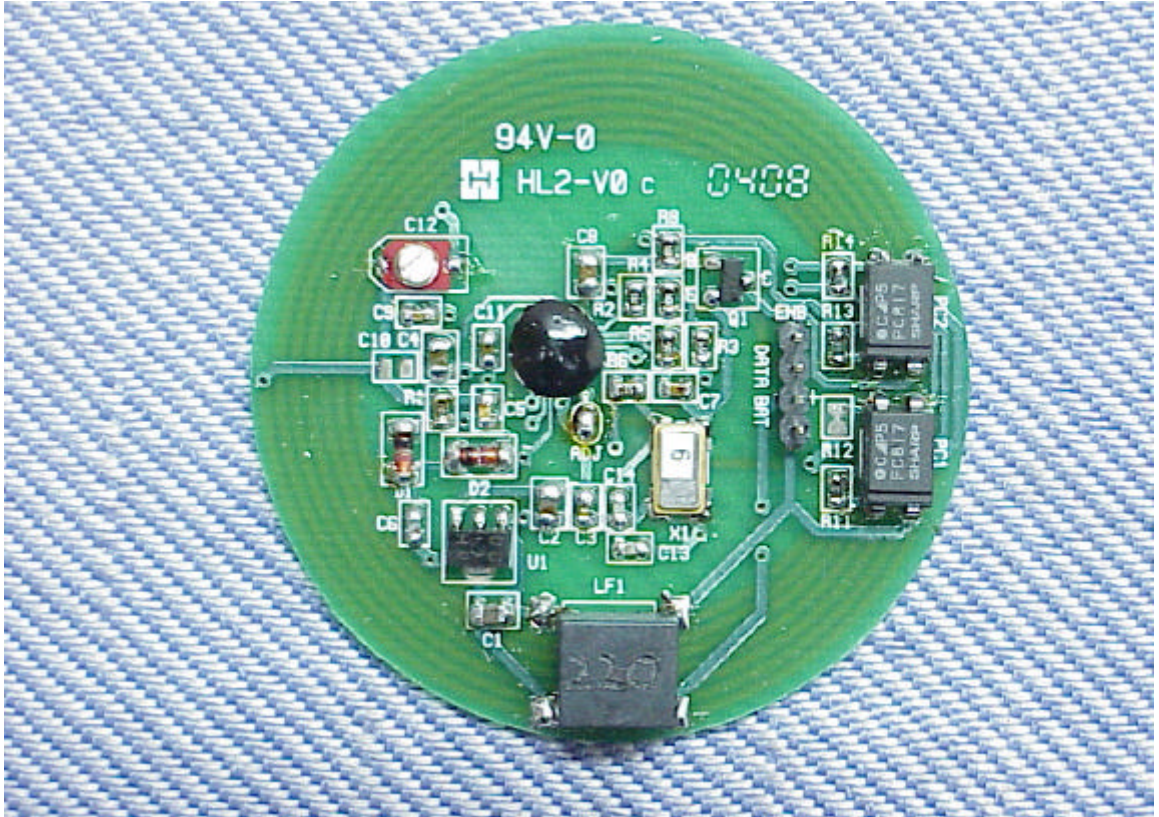
Primary PCB (Component Side)
