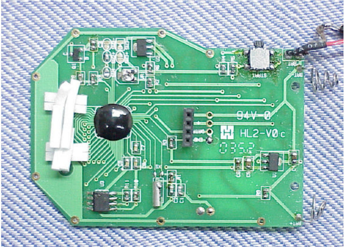
Sub PCB (Component Side)
