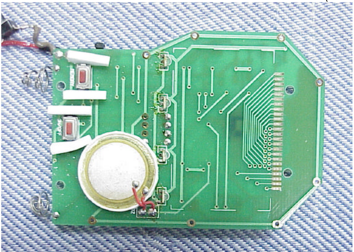
Sub PCB (Foil Side)
