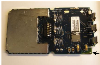
S4 Internal PCB Bottom Side
