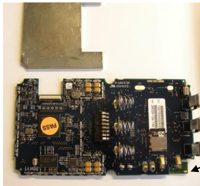
S4 Internal PCB Bottom Side shield removed
