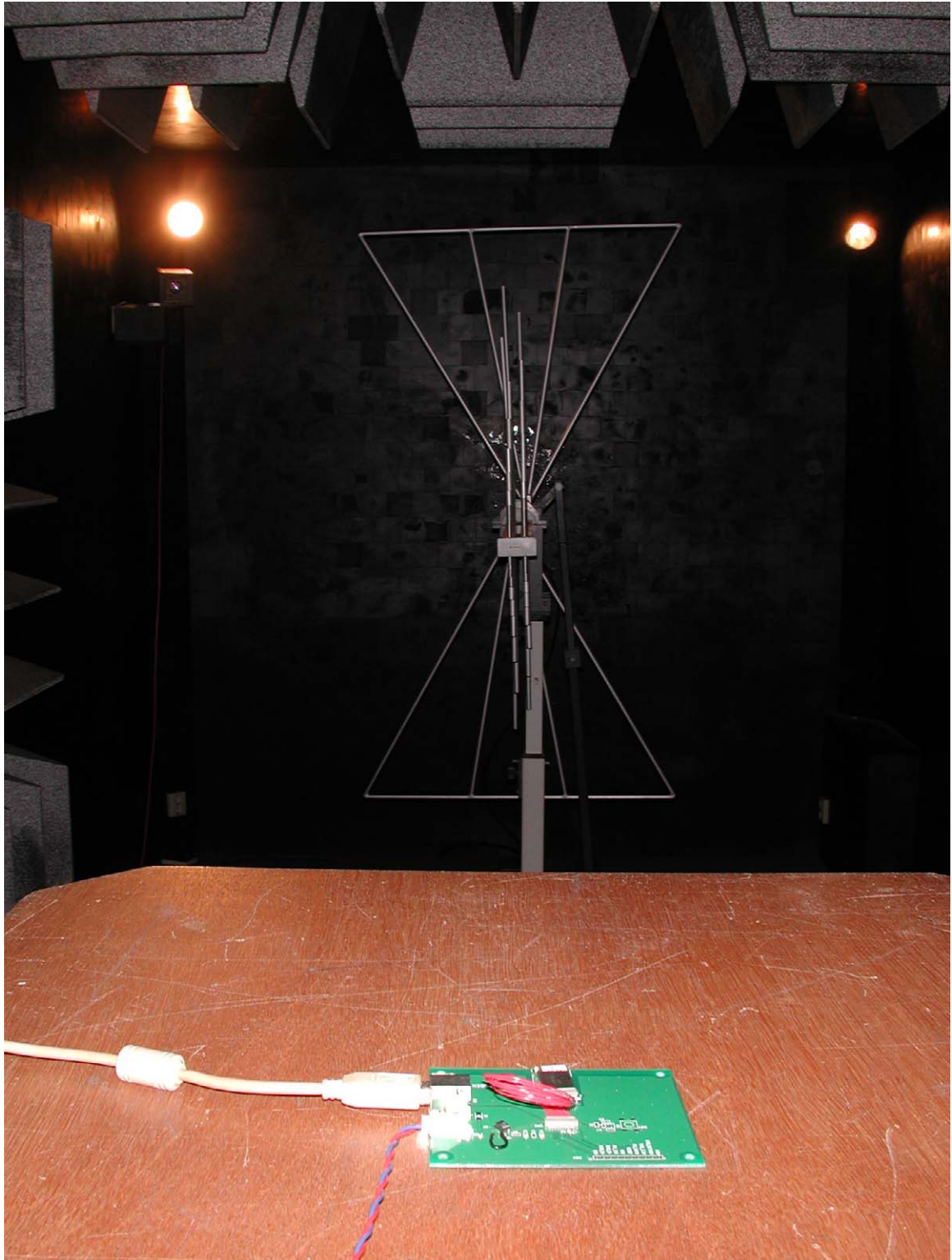
Photograph 1: Radiated measurements test setup < 1000 MHz
