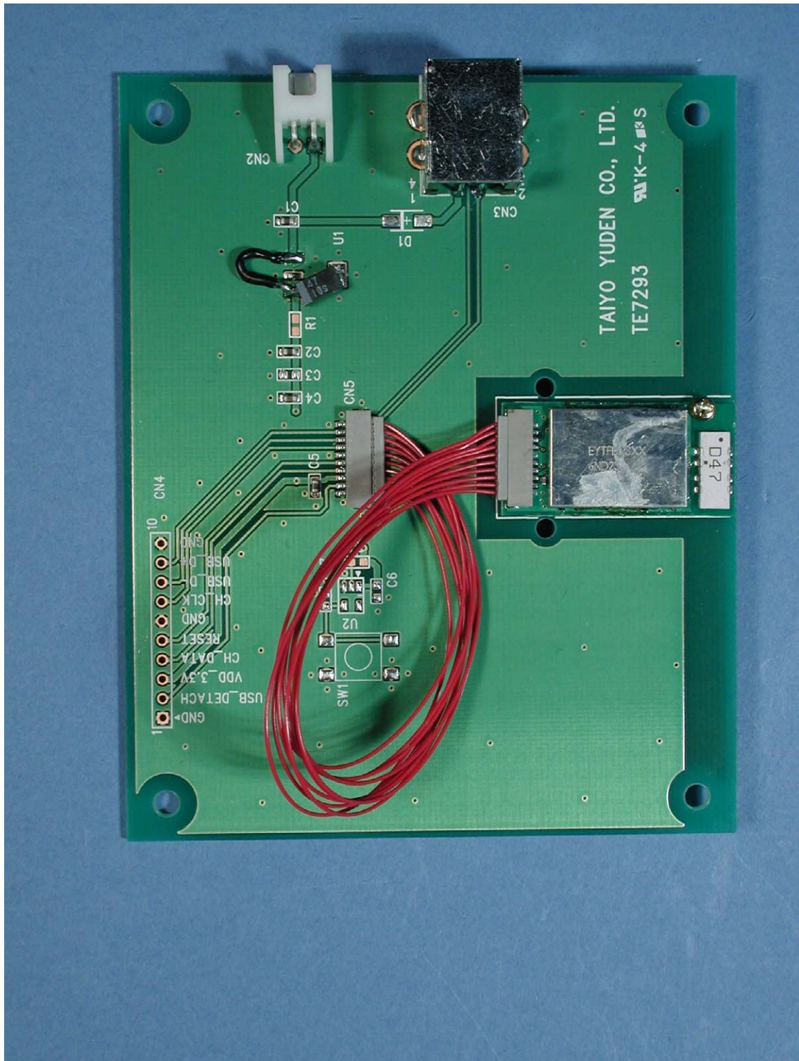
Photograph 1: EYTFECSXX with integrated antenna on evaluation board
