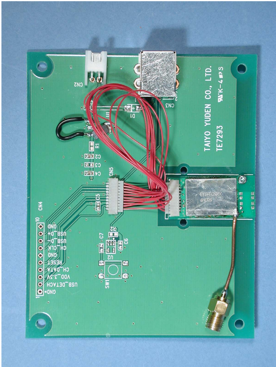
Photograph 2: EYTFECSXX with temporary SMA connector on evaluation board
