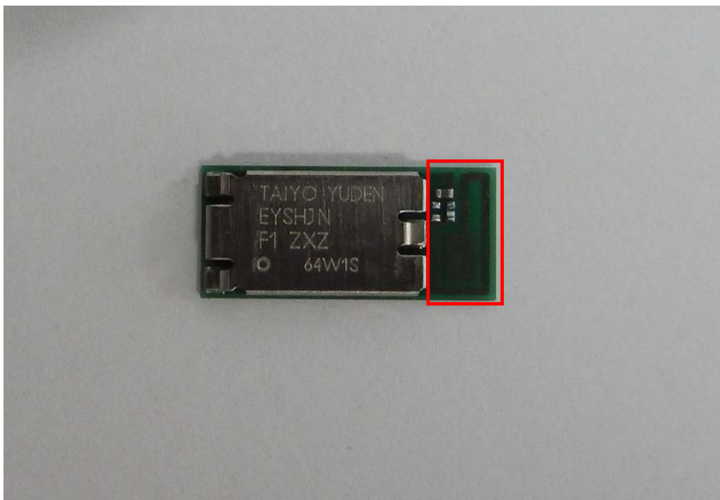
Antenna Location
