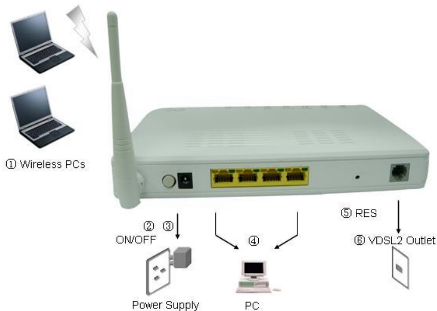
Figure 4: Overview of Hardware Connections for X5671
