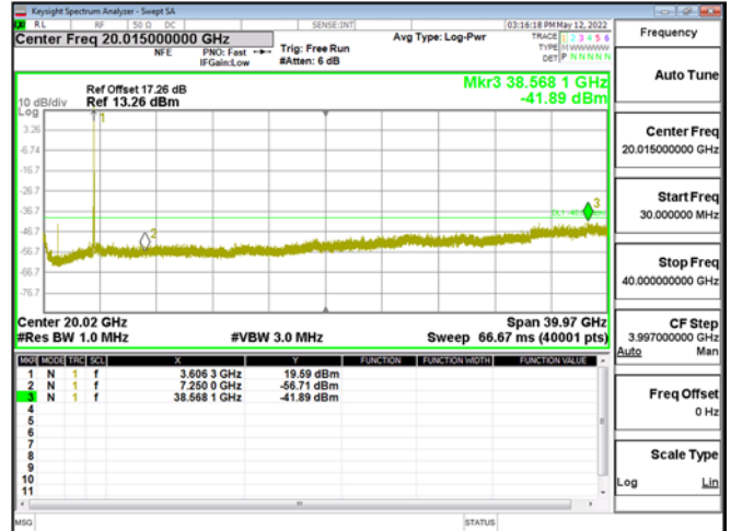
Band48-Part96_40MHz_CP_OFDM_SCS30kHz_OPSK_RB1_1_CH645332
