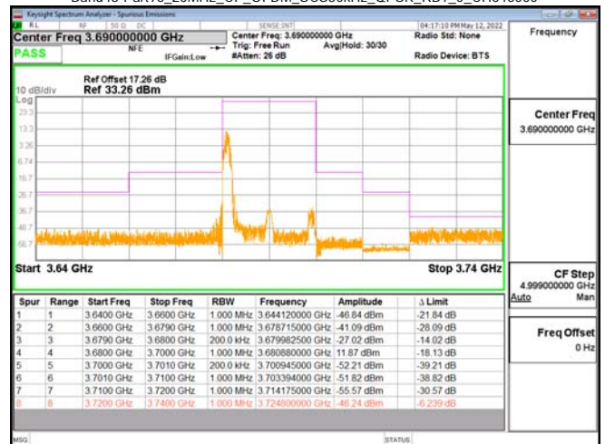
Band48-Part96_20MHz_CP_OFDM_SCS30kHz_QPSK_RB1_0_CH646000
