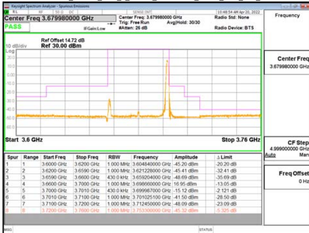
Band48-Part96_40MHz_DFT_s_OFDM_SCS30kHz_BPSK_RB1_105_CH645332
