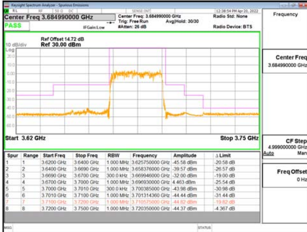
Band48-Part96_30MHz_DFT_s_OFDM_SCS30kHz_BPSK_RB75_0_CH645666
