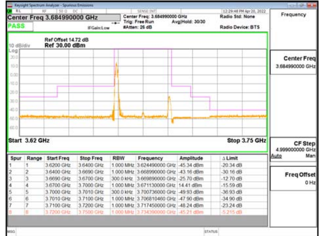
Band48-Part96_30MHz_CP_OFDM_SCS30kHz_QPSK_RB1_0_CH645666
