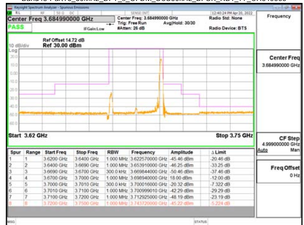
Band48-Part96_30MHz_DFT_s_OFDM_SCS30kHz_BPSK_RB1_77_CH645666
