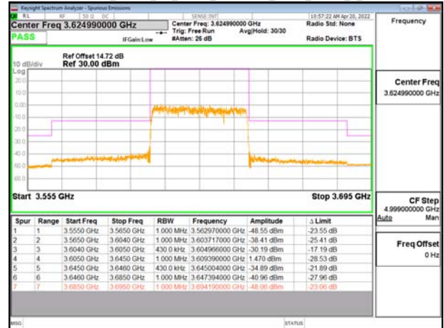
Band48-Part96_40MHz_CP_OFDM_SCS30kHz_QPSK_RB106_0_CH645332
