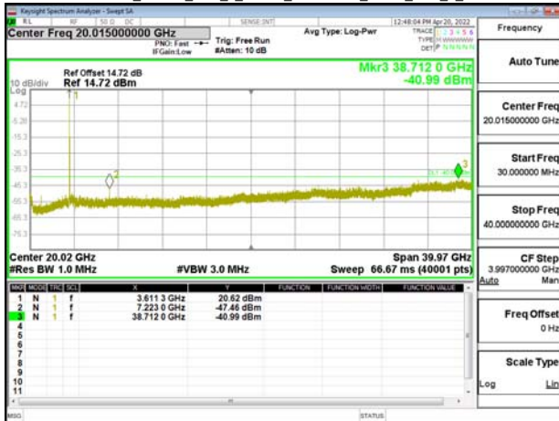
Band48-Part96_30MHz_DFT_s_OFDM_SCS30kHz_BPSK_RB1_1_CH645666
