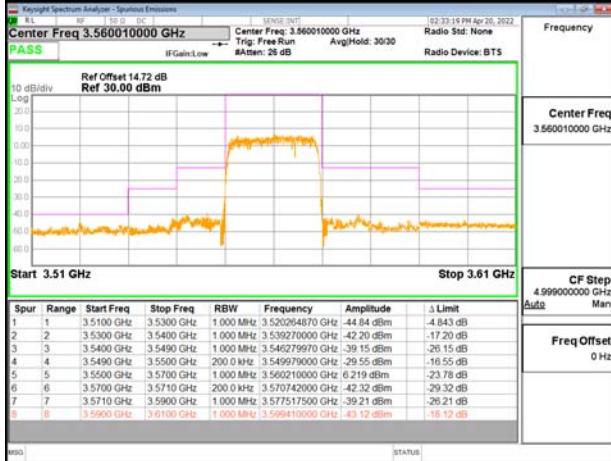
Band48-Part96_20MHz_DFT_s_OFDM_SCS30kHz_BPSK_RB50_0_CH641666
