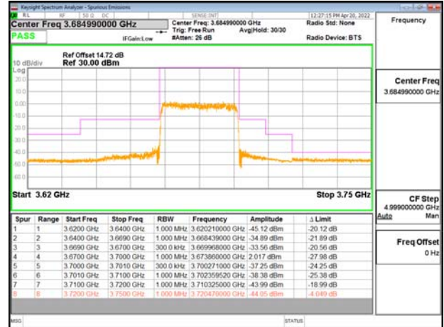
Band48-Part96_30MHz_CP_OFDM_SCS30kHz_QPSK_RB78_0_CH645666
