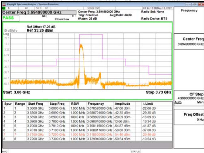
Band48-Part96_10MHz_CP_OFDM_SCS30kHz_QPSK_RB1_0_CH646332
