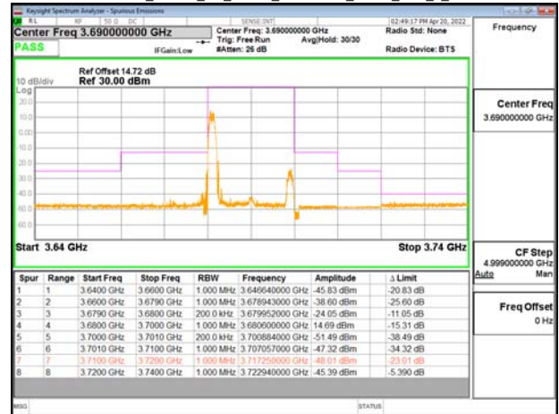
Band48-Part96_20MHz_CP_OFDM_SCS30kHz_QPSK_RB1_0_CH646000
