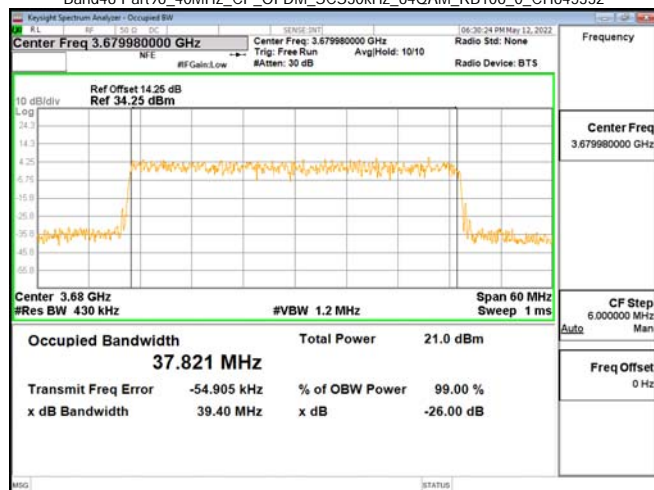
Band48-Part96_40MHz_CP_OFDM_SCS30kHz_64QAM_RB106_0_CH645332
