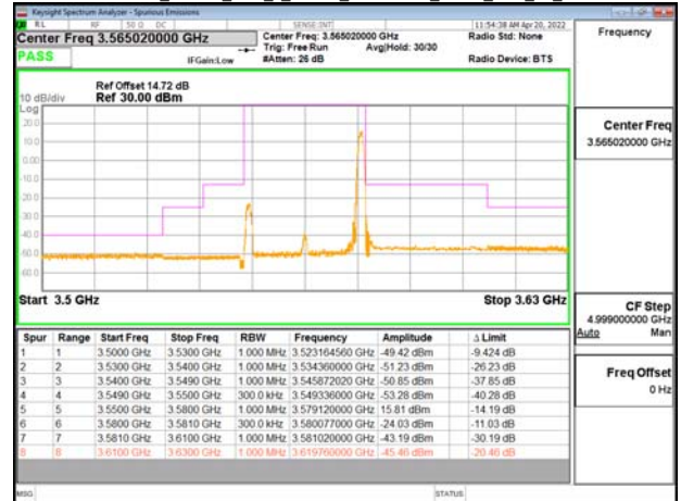
Band48-Part96_30MHz_DFT_s_OFDM_SCS30kHz_BPSK_RB1_77_CH641666
