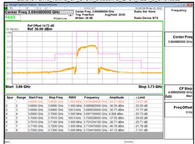
Band48-Part96_10MHz_CP_OFDM_SCS30kHz_QPSK_RB24_0_CH646332
