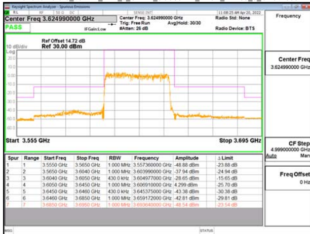
Band48-Part96_40MHz_DFT_s_OFDM_SCS30kHz_BPSK_RB100_0_CH645332
