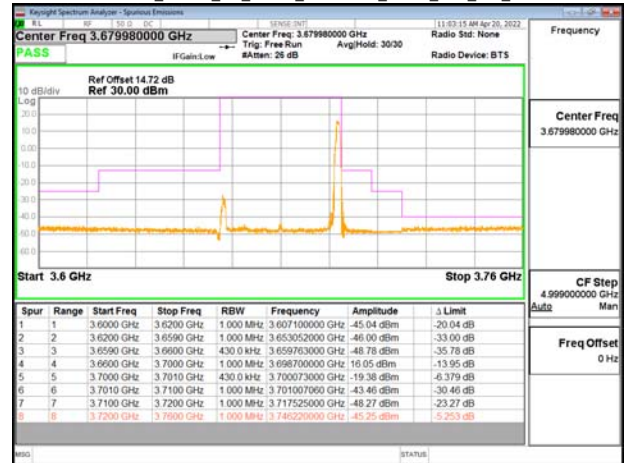
Band48-Part96_40MHz_CP_OFDM_SCS30kHz_OPSK_RB1_105_CH645332
