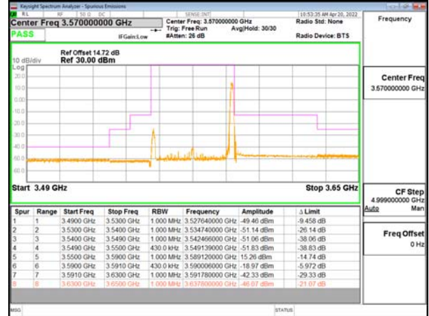
Band48-Part96_40MHz_CP_OFDM_SCS30kHz_OPSK_RB1_105_CH641666
