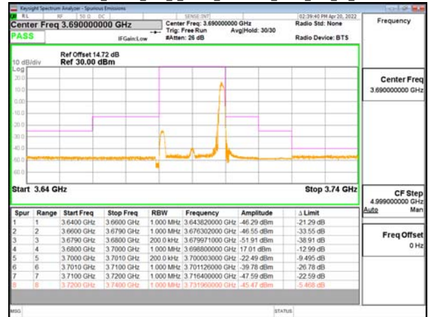
Band48-Part96_20MHz_DFT_s_OFDM_SCS30kHz_BPSK_RB1_50_CH646000
