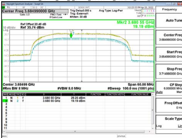
Band48-Part96_30MHz_DFT_s_OFDM_SCS30kHz_256QAM_RB75_0_CH645666
