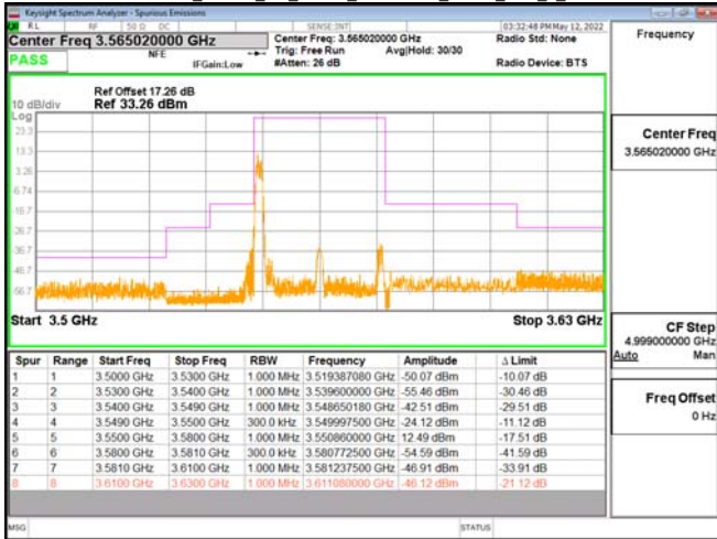
Band48-Part96_30MHz_CP_OFDM_SCS30kHz_QPSK_RB1_0_CH641666
