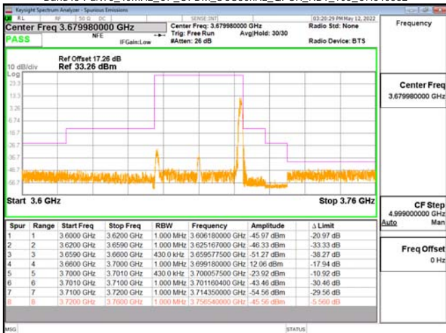
Band48-Part96_40MHz_CP_OFDM_SCS30kHz_QPSK_RB1_105_CH645332
