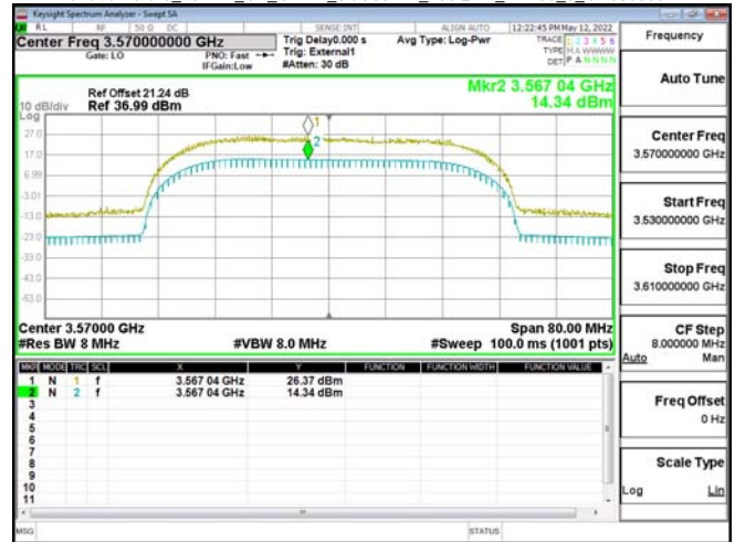
Band48-Part96_40MHz_CP_OFDM_SCS30kHz_256QAM_RB106_0_CH641666
