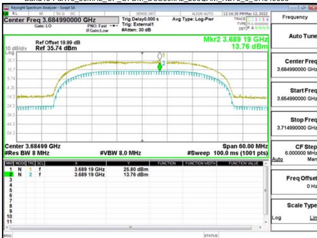
Band48-Part96_30MHz_CP_OFDM_SCS30kHz_256QAM_RB78_0_CH645666
