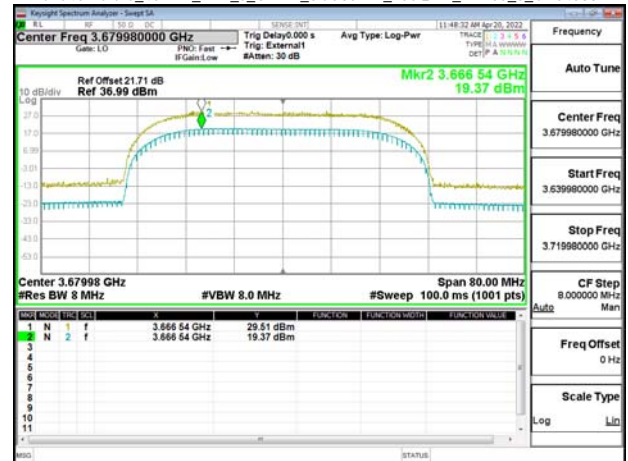
Band48-Part96_40MHz_DFT_s_OFDM_SCS30kHz_256QAM_RB100_0_CH645332
