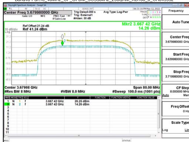
Band48-Part96_40MHz_CP_OFDM_SCS30kHz_256QAM_RB106_0_CH645332
