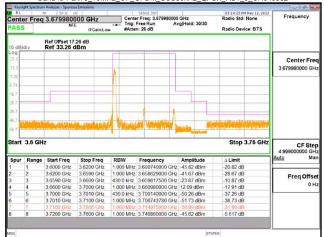
Band48-Part96_40MHz_CP_OFDM_SCS30kHz_QPSK_RB1_0_CH645332
