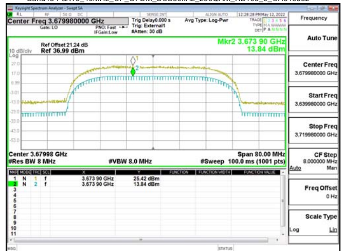
Band48-Part96_40MHz_CP_OFDM_SCS30kHz_256QAM_RB106_0_CH645332
