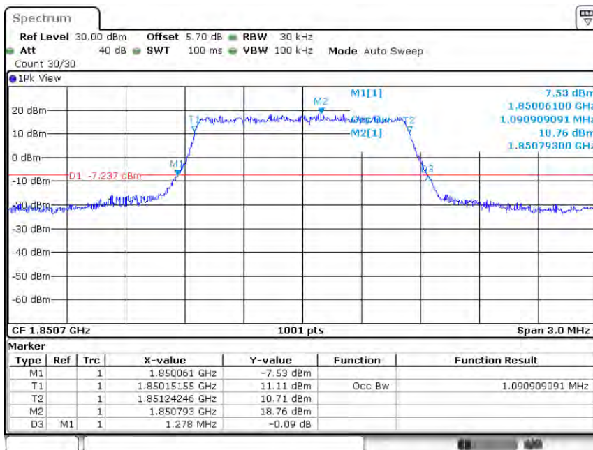
Band2-1.4MHz-QPSK-18607-6RB#0-1.091
