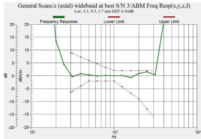
Figure C.4 Frequency Response of WCDMA1900 - OTT VoIP
