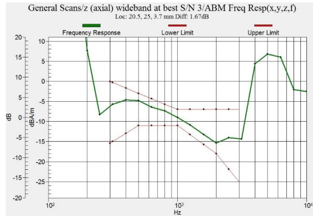
Figure C.1 Frequency Response of WCDMA 1900
