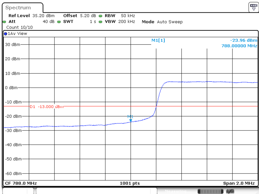
Band14-5MHz-QPSK-23305-25RB#0
