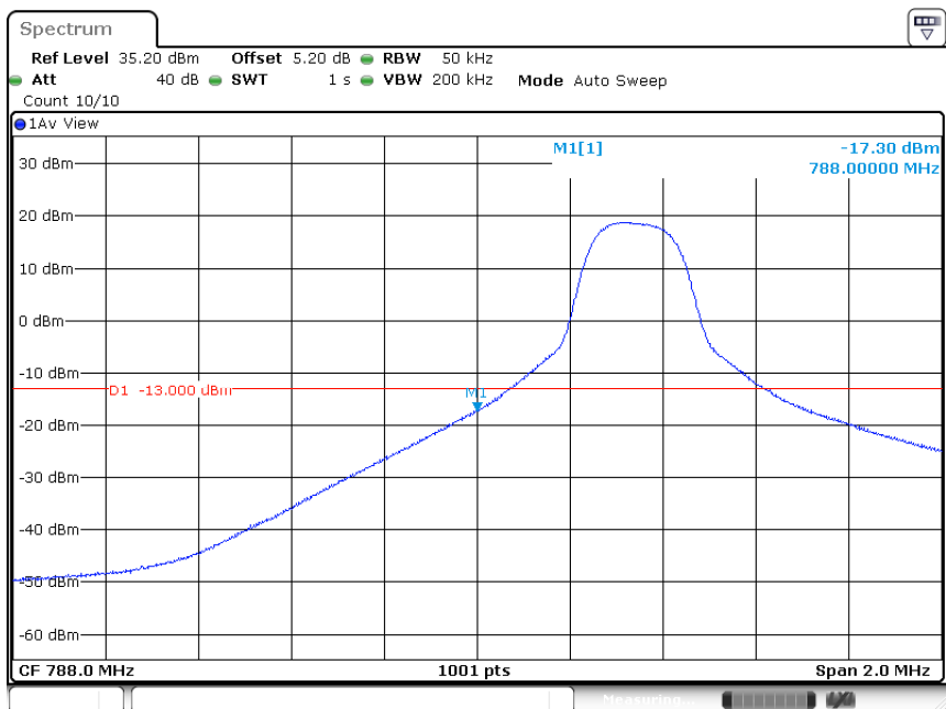
Band14-5MHz-QPSK-23305-1RB#0
