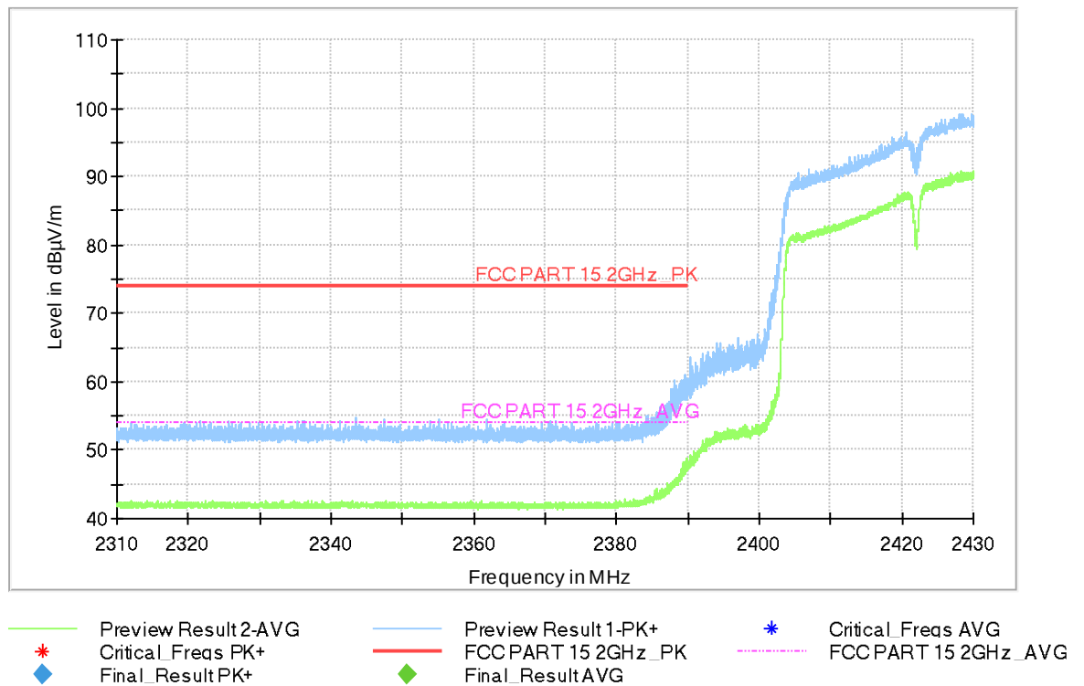
Fig.A.5.2.7 Radiated band Edges (802.11n-HT40, Ch 3)
