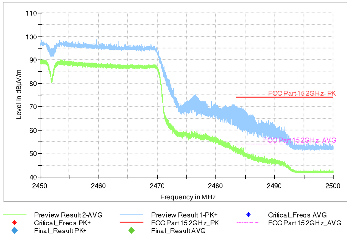
Fig.A.5.2.8 Radiated band Edges (802.11n-HT40, Ch 9)
