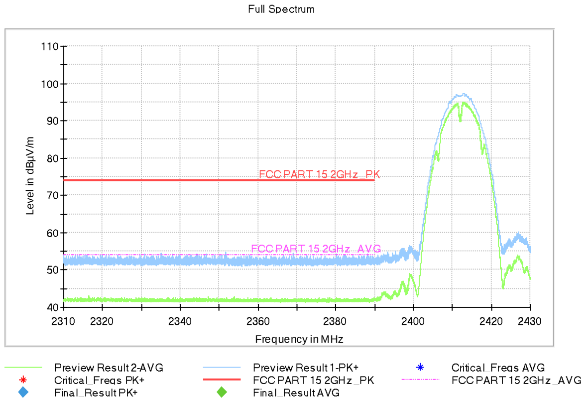
Fig.A.5.2.1 Radiated band Edges (802.11b, Ch 1)
