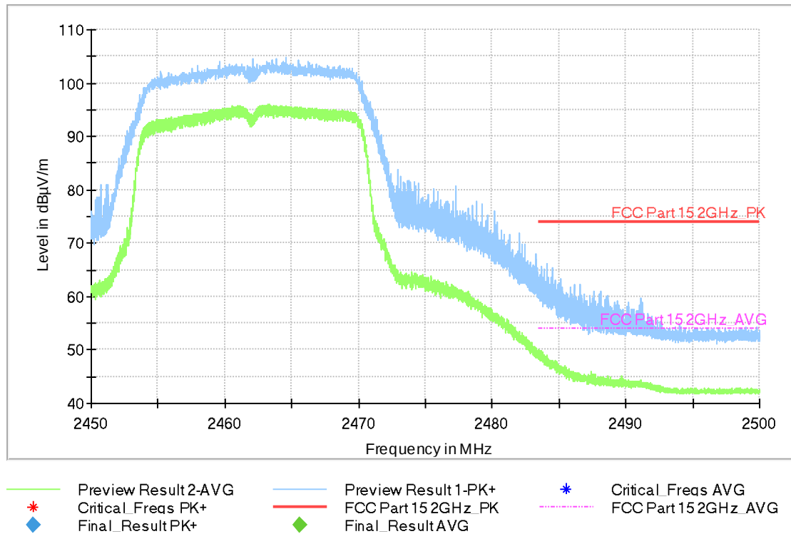
Fig.A.5.2.4 Radiated band Edges (802.11g, Ch 11)
