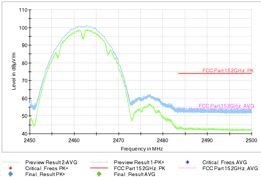
Fig.A.5.2.2 Radiated band Edges (802.11b, Ch 11)
