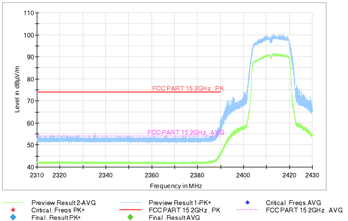
Fig.A.5.2.3 Radiated band Edges (802.11g, Ch 1)
