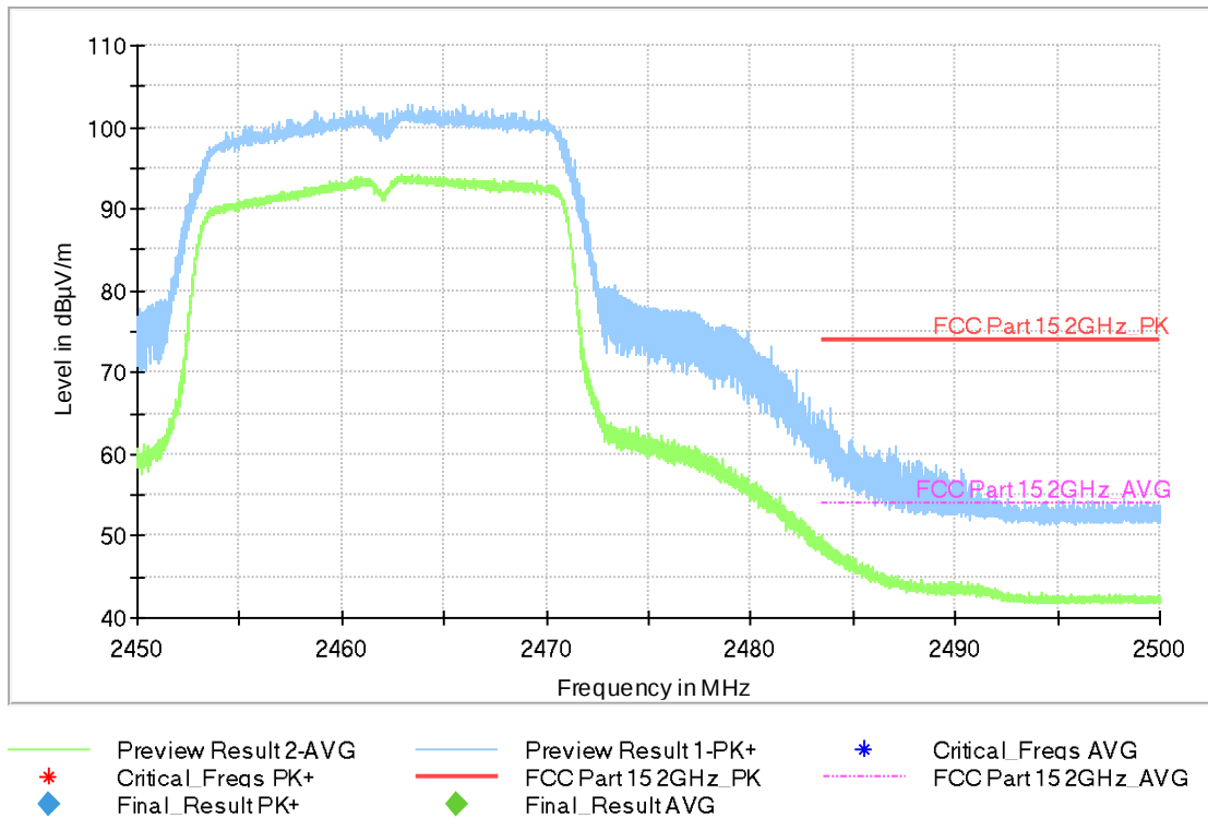
Fig.A.5.2.6 Radiated band Edges (802.11n-HT20, Ch 11)
