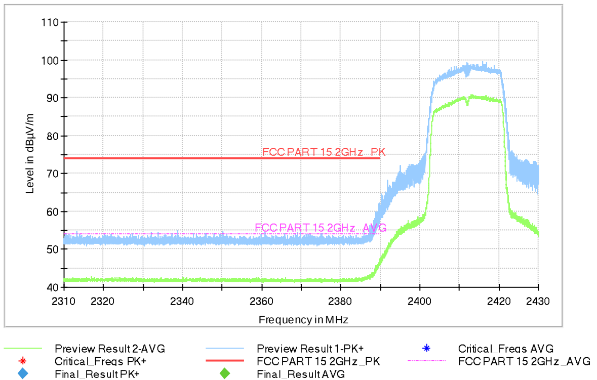
Fig.A.5.2.5 Radiated band Edges (802.11n-HT20, Ch 1)
