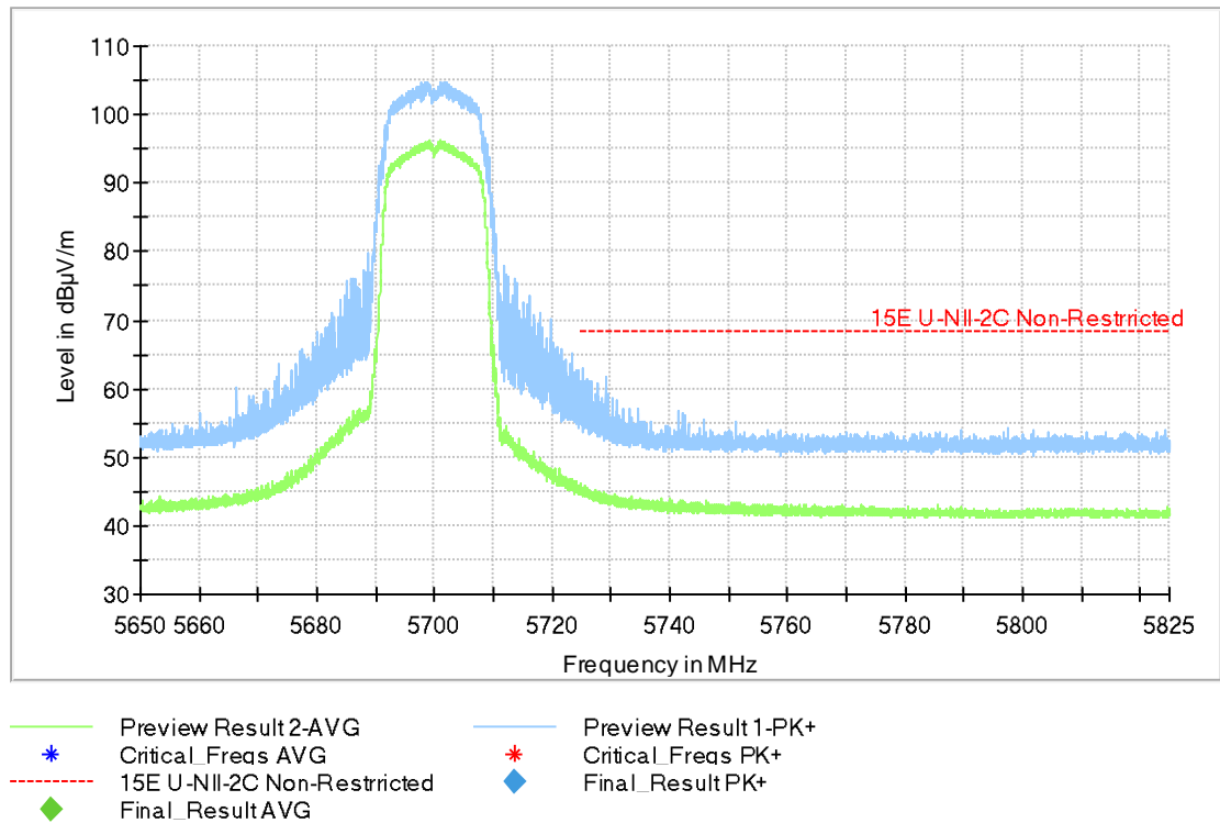
Fig.37 Band Edges (802.11a, 5700MHz)
