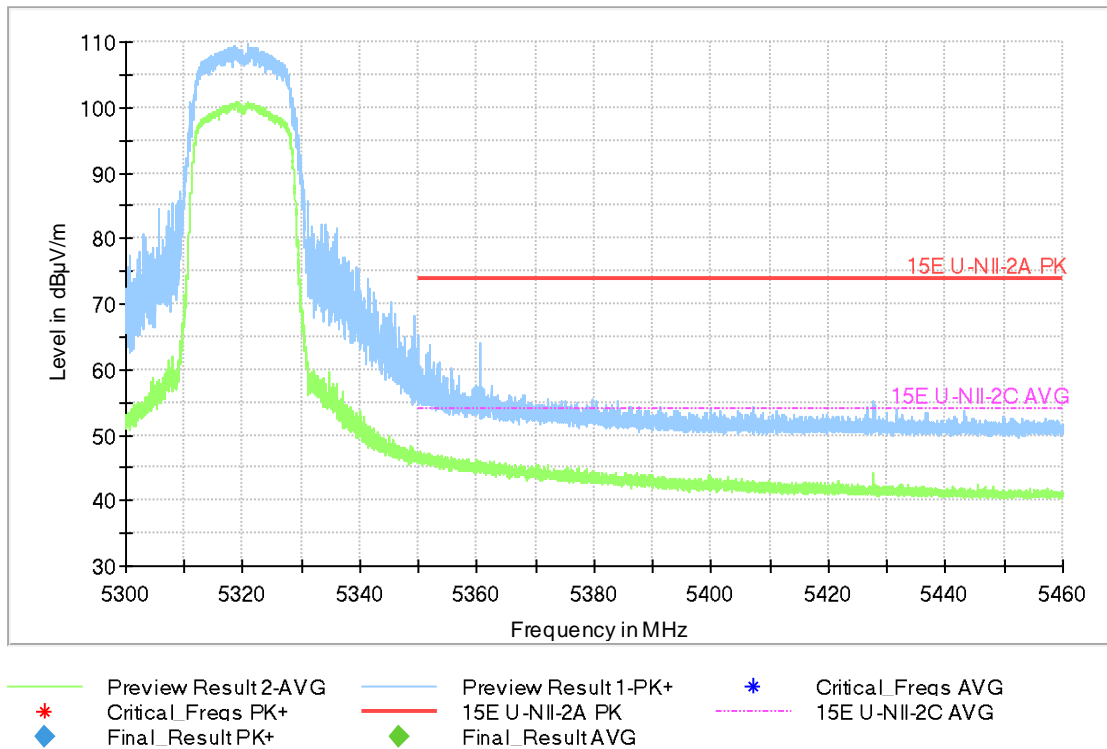
Fig.35 Band Edges (802.11a, 5320MHz)
