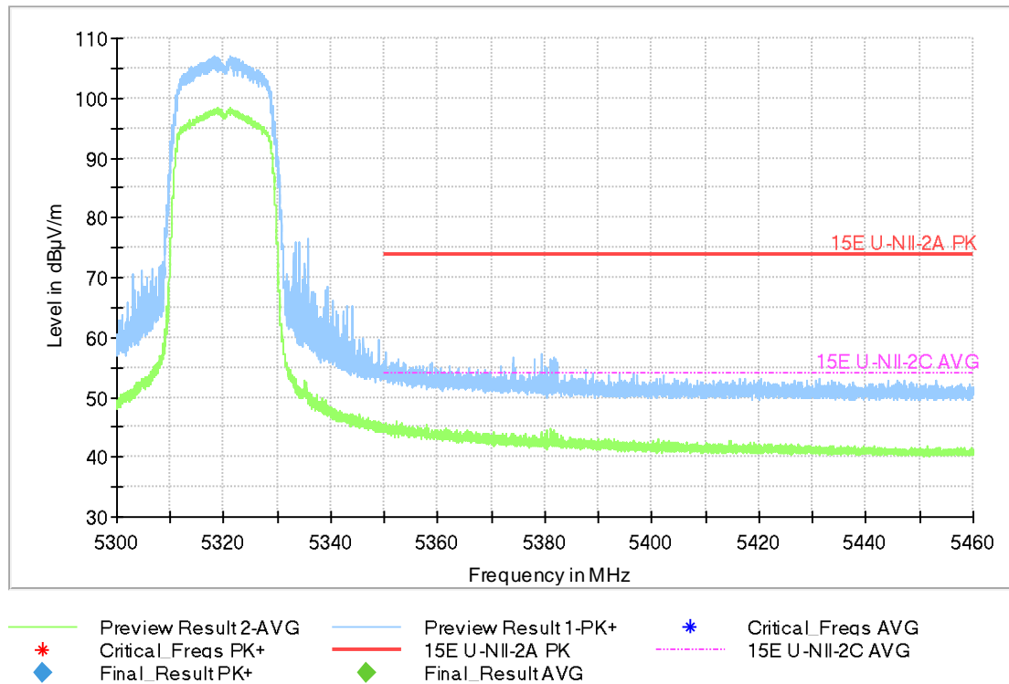
Fig.43 Band Edges (802.11ac-HT20, 5320MHz)
