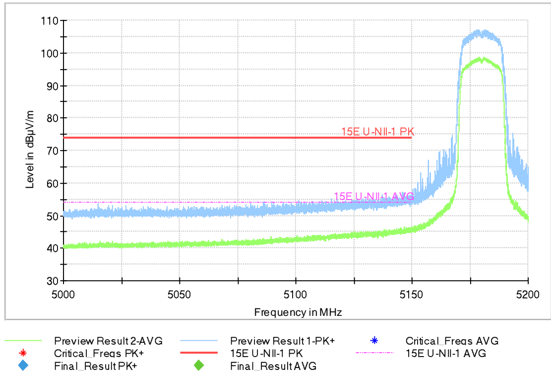
Fig.42 Band Edges (802.11ac-HT20, 5180MHz)
