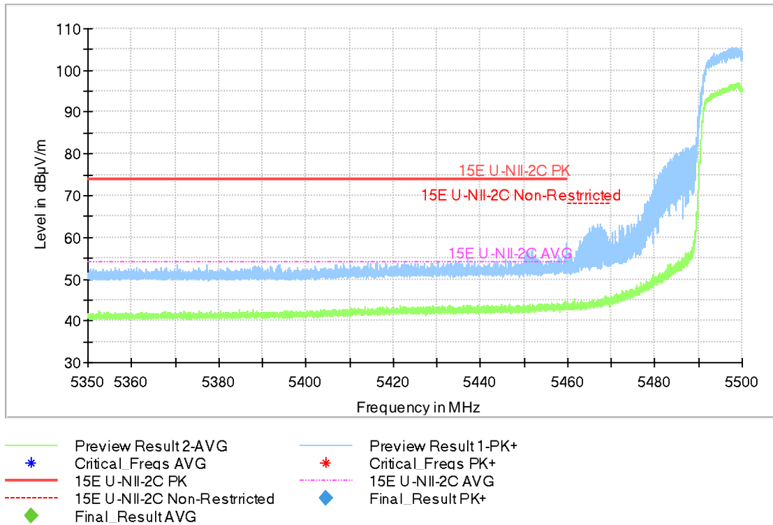
Fig.40 Band Edges (802.11n-HT20, 5500MHz)
