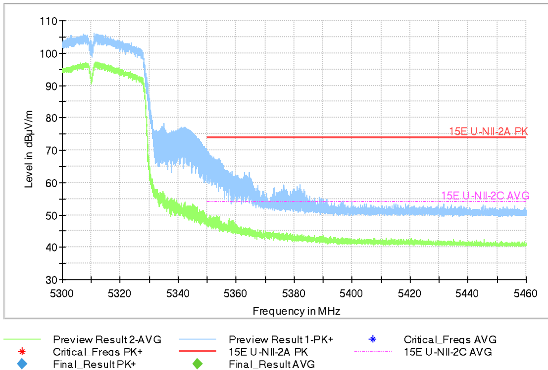
Fig.47 Band Edges (802.11n-HT40, 5310MHz)
