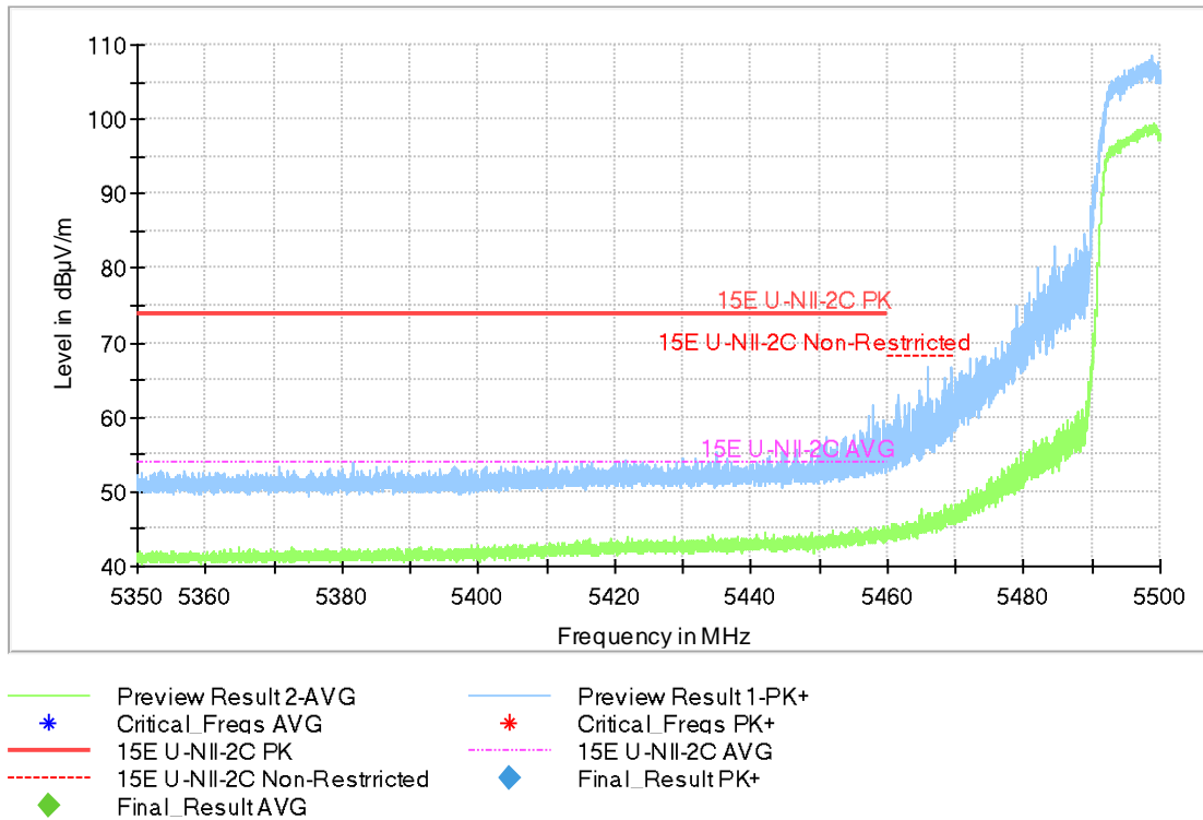
Fig.36 Band Edges (802.11a, 5500MHz)
