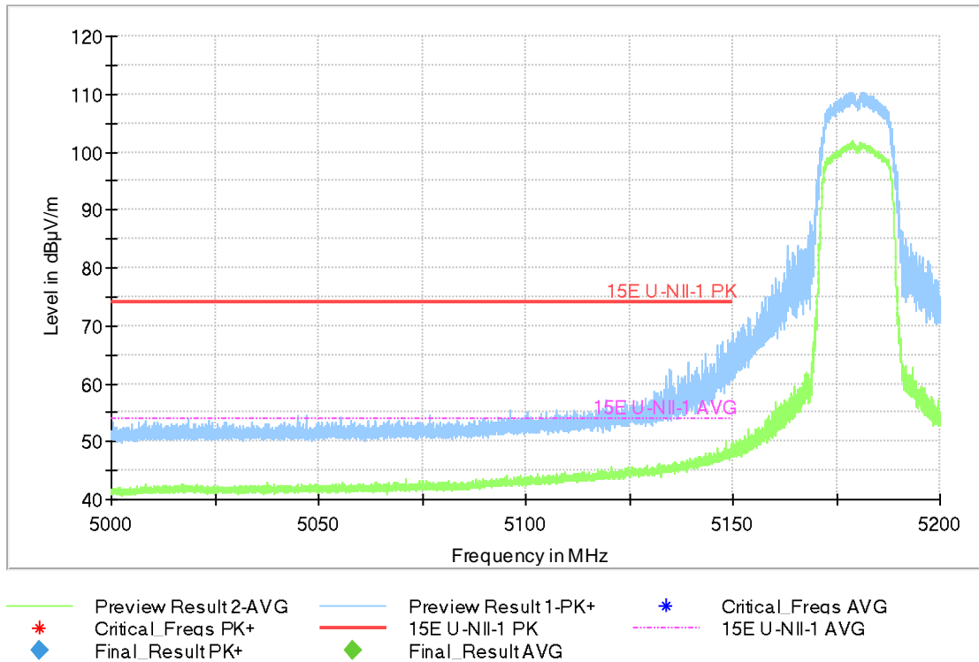
Fig.34 Band Edges (802.11a, 5180MHz)
