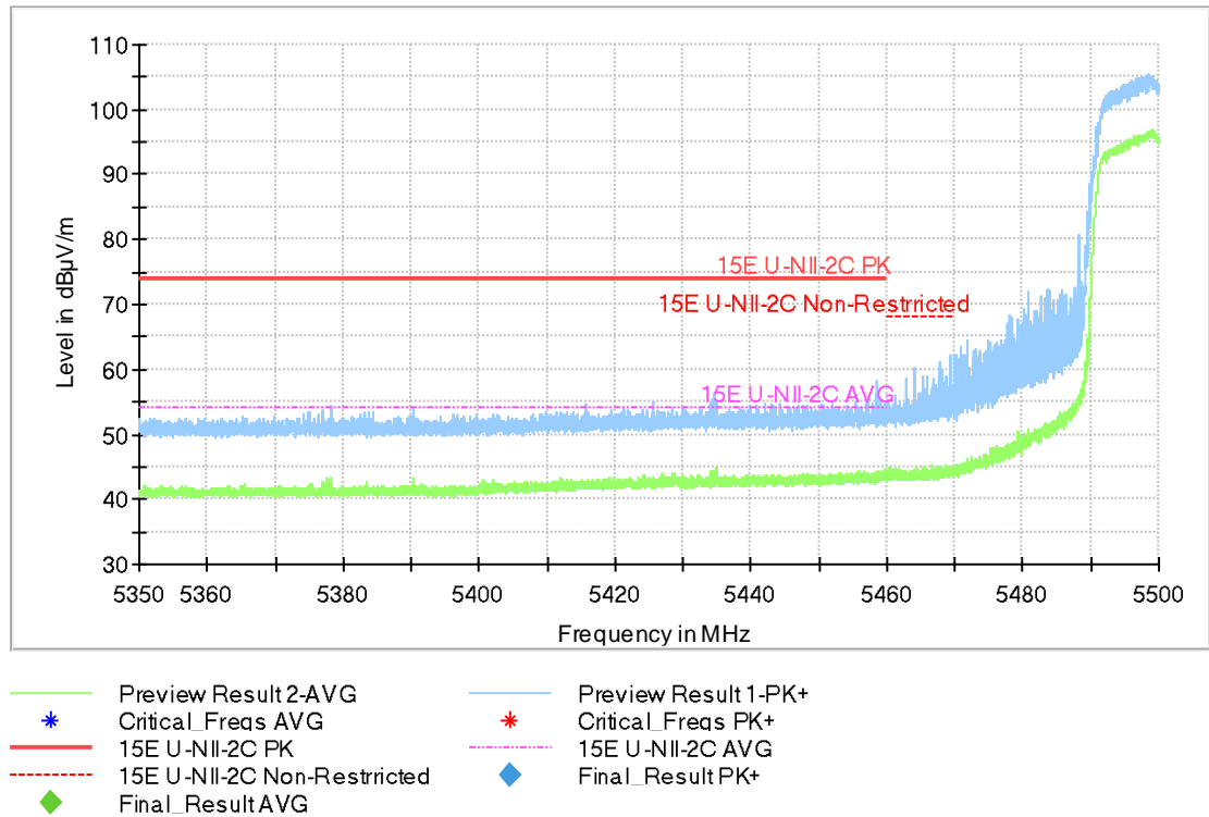
Fig.44 Band Edges (802.11ac-HT20, 5500MHz)
