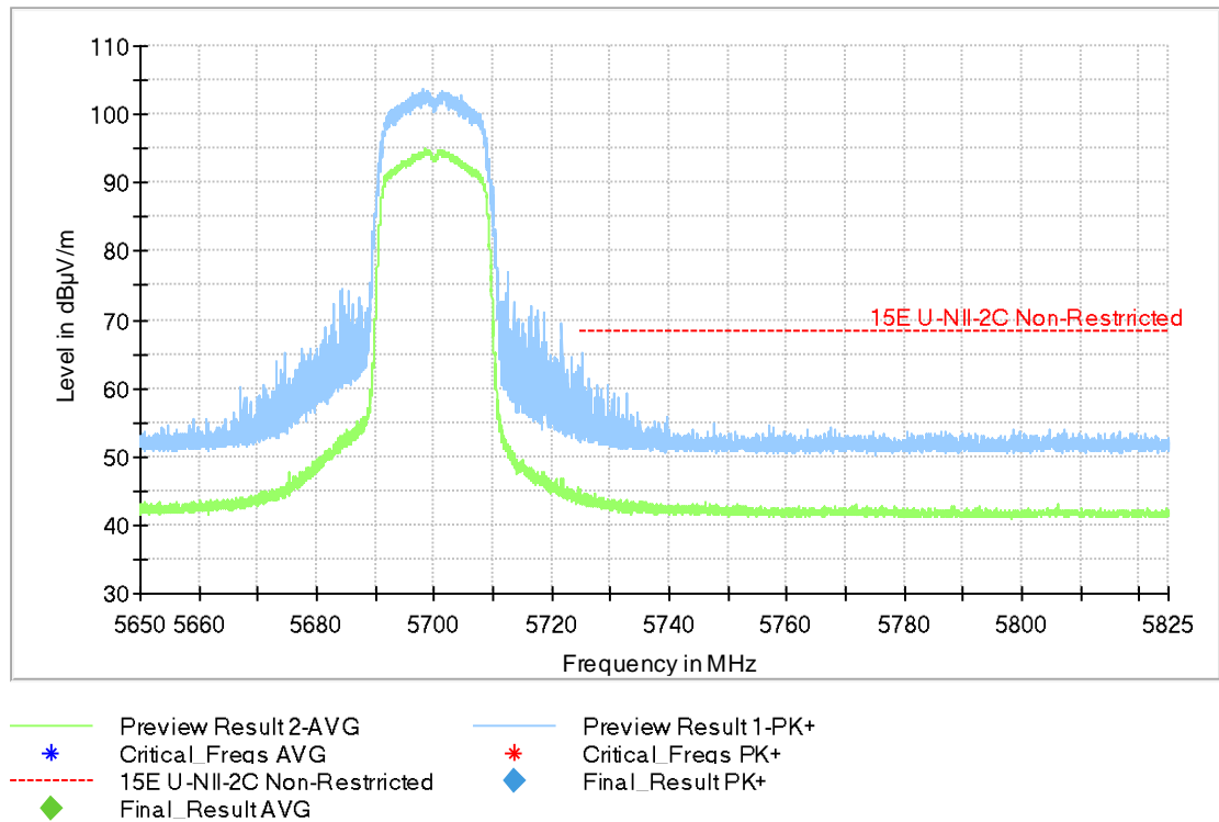
Fig.45 Band Edges (802.11ac-HT20, 5700MHz)
