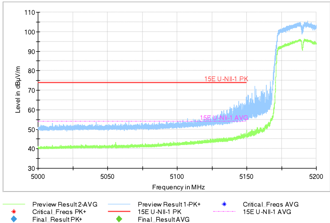
Fig.50 Band Edges (802.11ac-HT40, 5190MHz)
