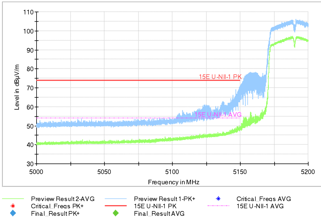
Fig.46 Band Edges (802.11n-HT40, 5190MHz)
