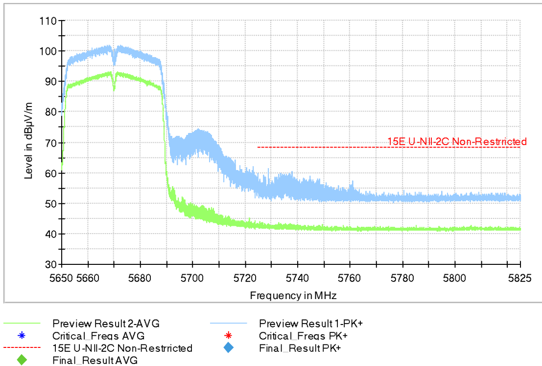
Fig.49 Band Edges (802.11n-HT40, 5670MHz)
