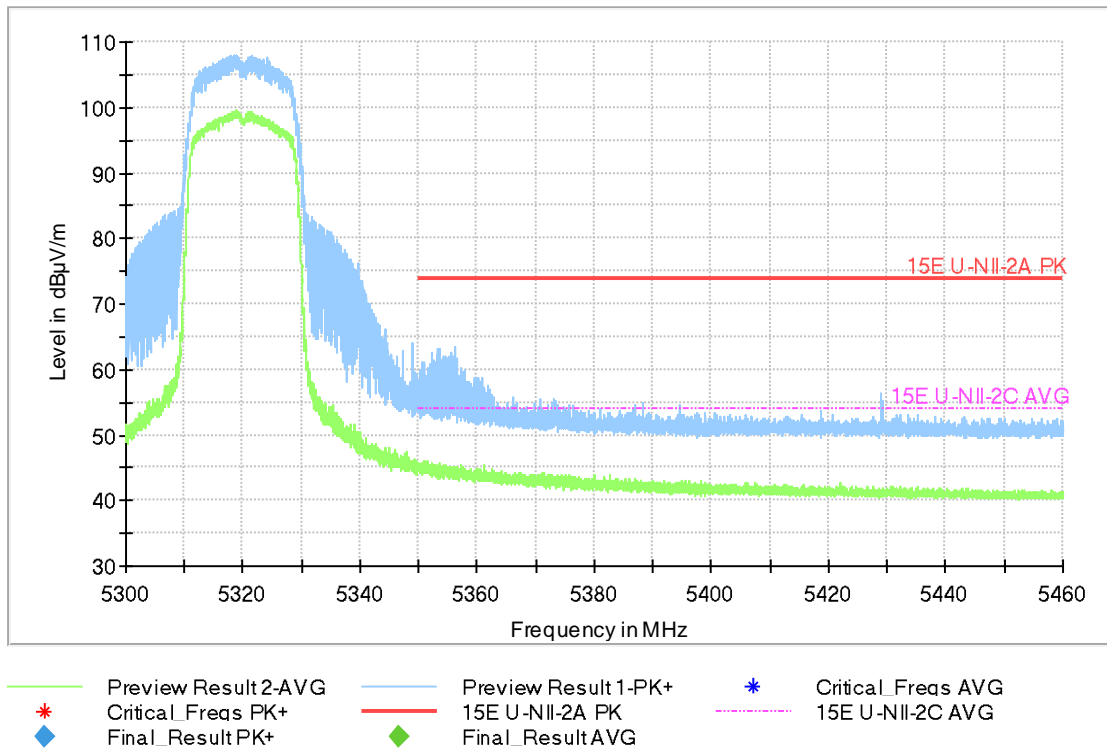
Fig.39 Band Edges (802.11n-HT20, 5320MHz)
