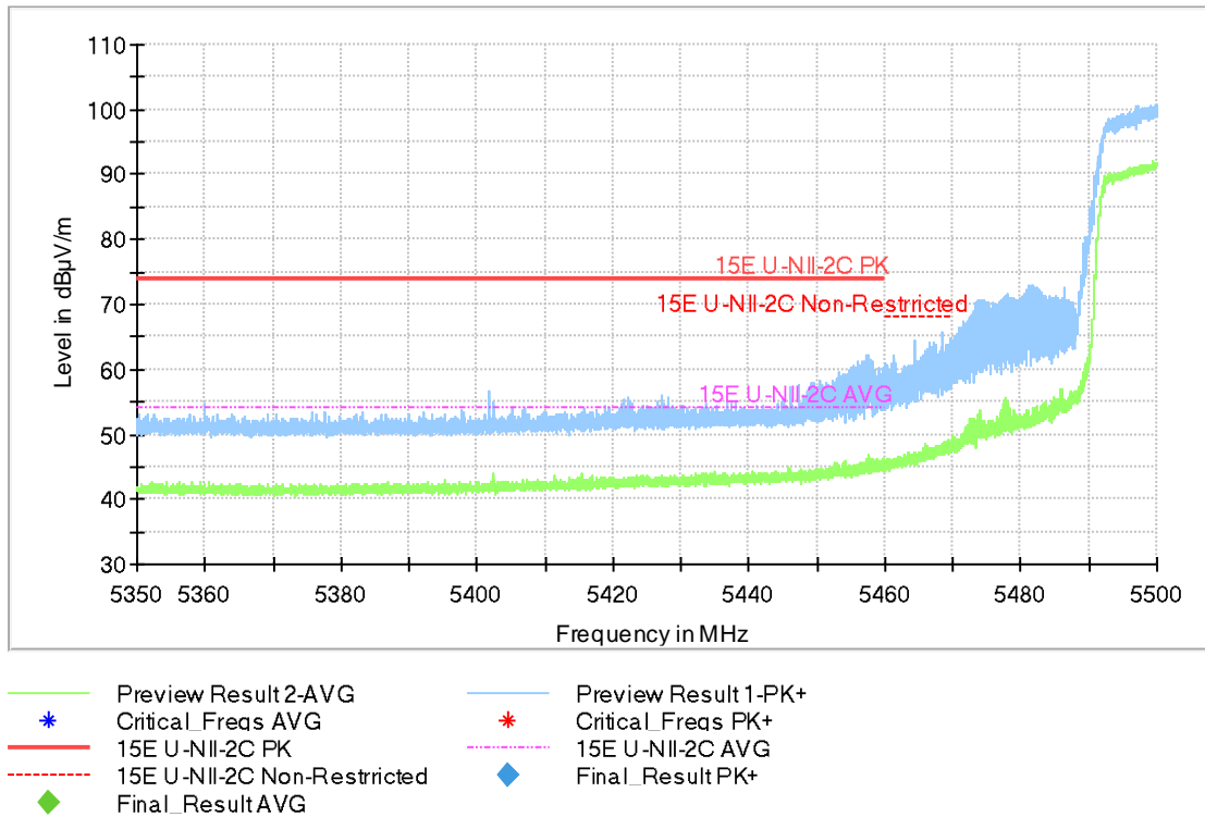
Fig.48 Band Edges (802.11n-HT40, 5510MHz)
