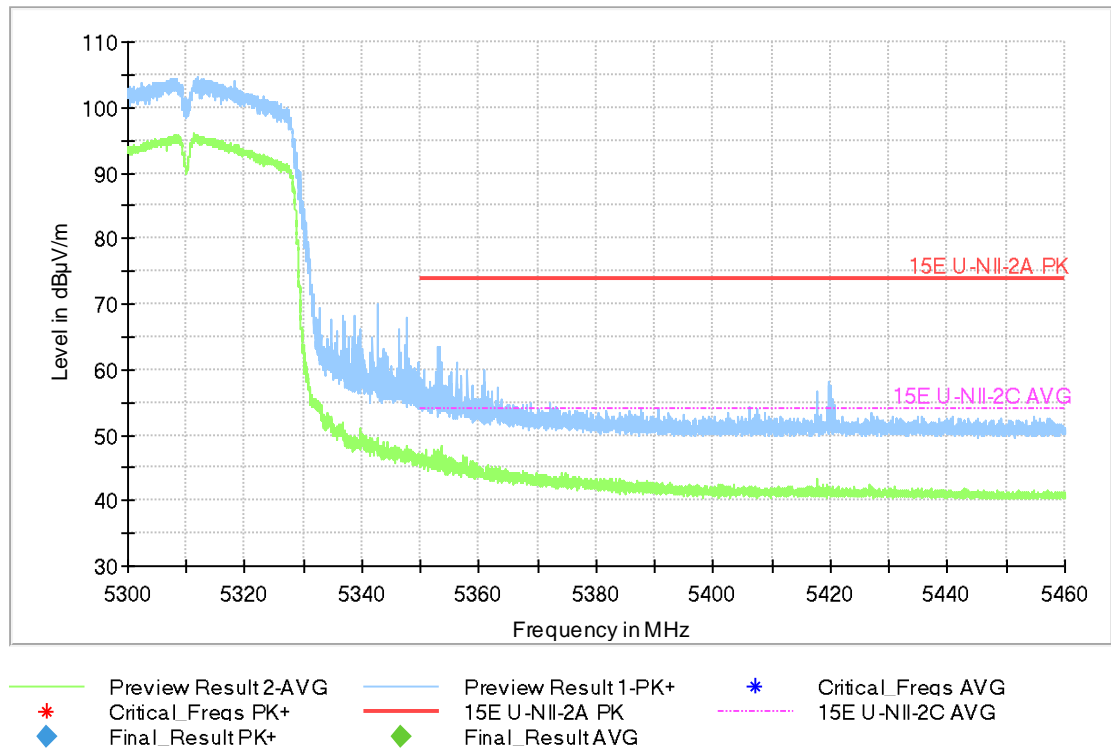
Fig.51 Band Edges (802.11ac-HT40, 5310MHz)
