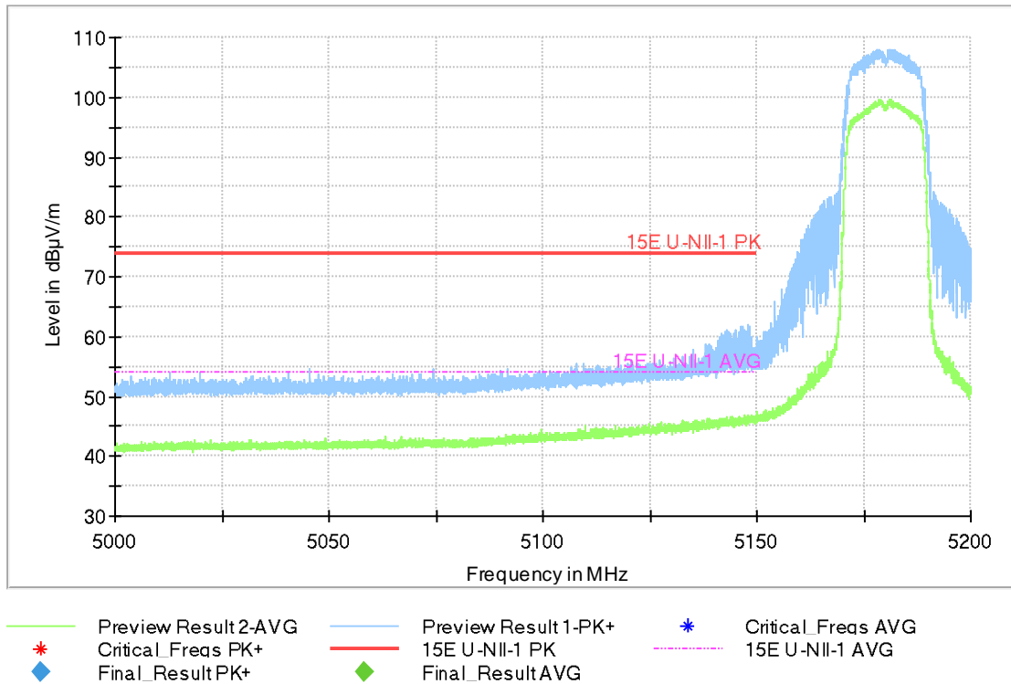
Fig.38 Band Edges (802.11n-HT20, 5180MHz)
