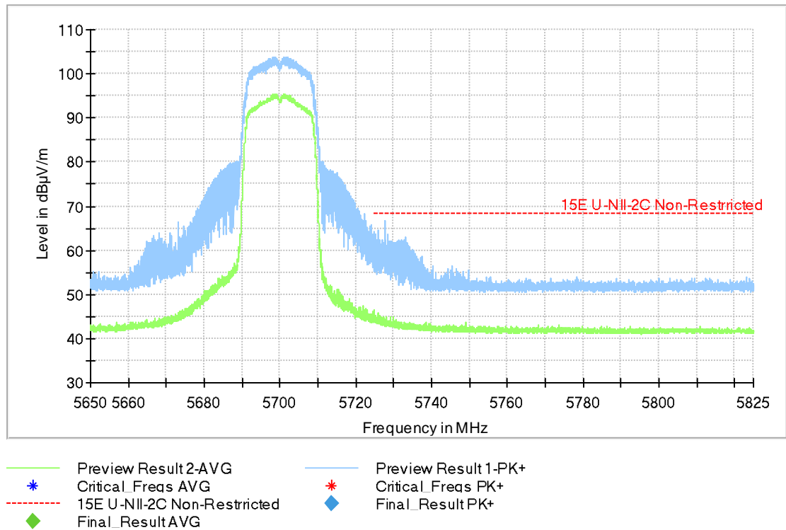
Fig.41 Band Edges (802.11n-HT20, 5700MHz)
