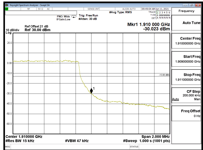
EDGE B2 1.4M CH19193 16QAM(6,0)
