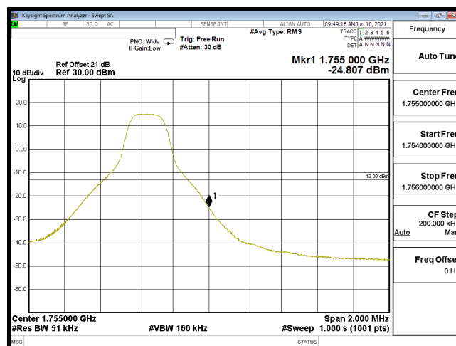
EDGE B4 5M CH20375 16QAM(1,24)
