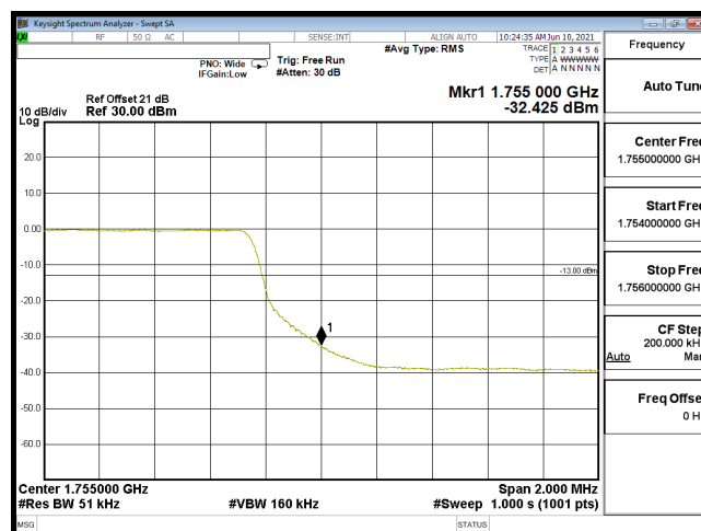
EDGE B4 5M CH20375 16QAM(25,0)
