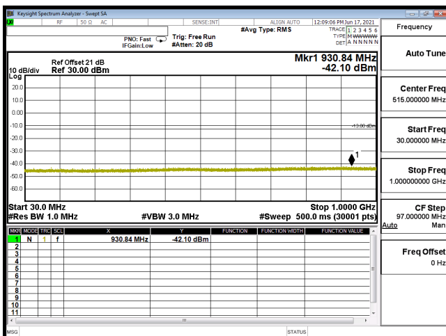
CSE B4 20M CH20175 QPSK(1,50) 30M-1G
