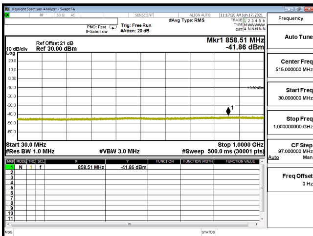
CSE B2 20M CH18700 16QAM(1,50) 30M-1G
