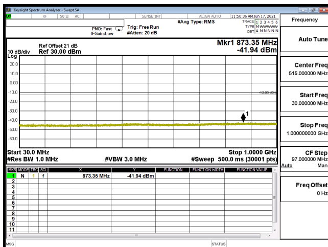
CSE B4 5M CH20375 16QAM(1,0) 30M-1G
