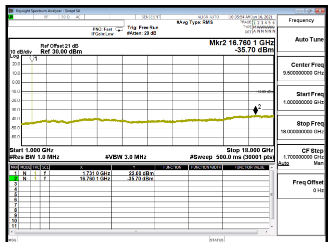
CSE B4 3M CH20175 QPSK(1,0) 1G-18G
