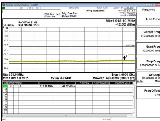
CSE B4 1.4M CH20393 16QAM(3,2) 30M-1G
