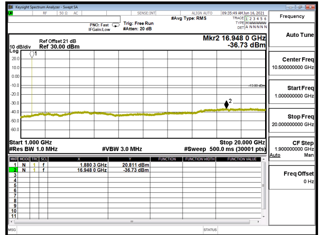
CSE B2 20M CH18900 16QAM(1,50) 1G-20G
