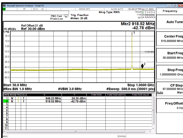
CSE B5 1.4M CH20643 16QAM(1,2) 30M-1G
