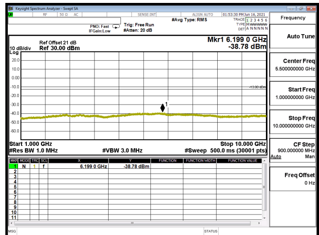
CSE B5 1.4M CH20407 16QAM(3,2) 1G-10G
