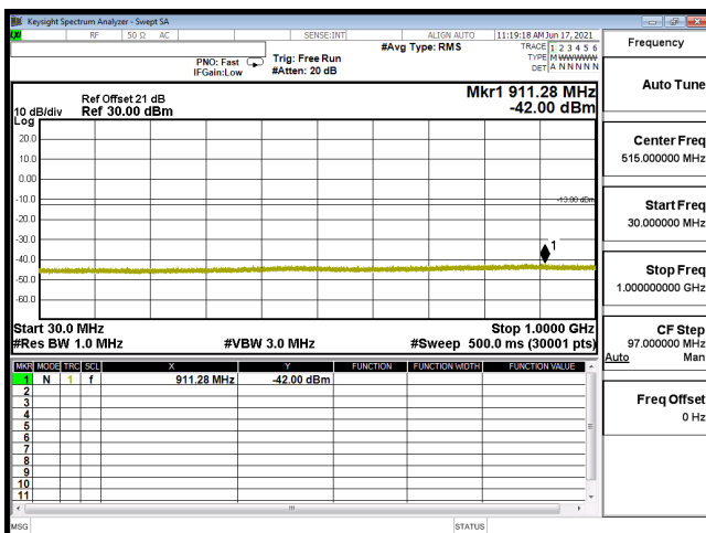
CSE B2 20M CH19100 16QAM(1,50) 30M-1G
