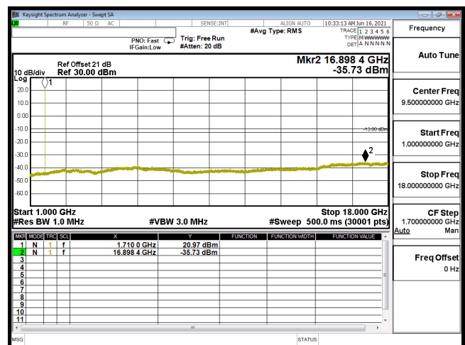
CSE B4 3M CH19965 16QAM(1,0) 1G-18G
