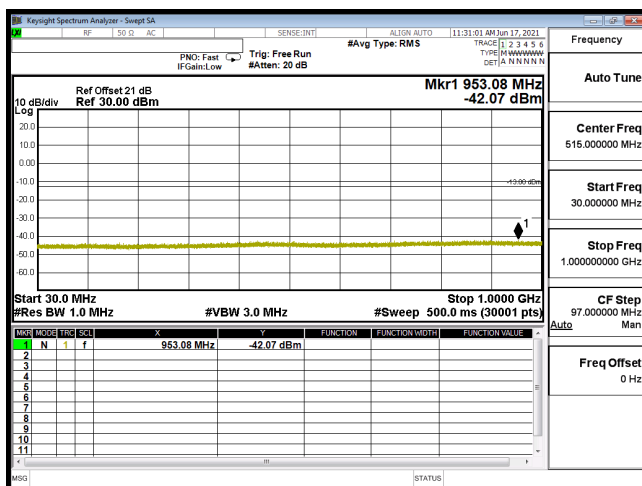
CSE B4 3M CH19965 16QAM(1,0) 30M-1G
