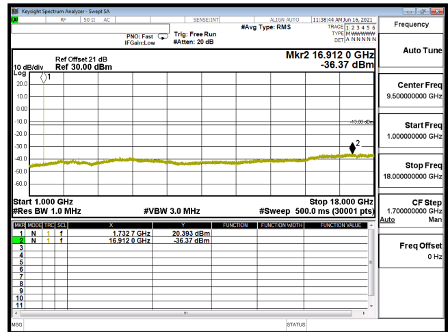
CSE B4 20M CH20175 16QAM(1,50) 1G-18G
