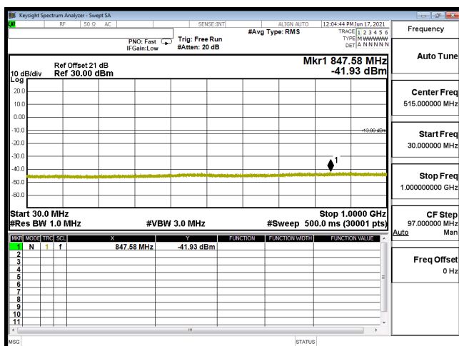
CSE B4 15M CH20175 QPSK(1,74) 30M-1G
