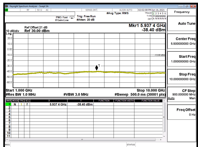
CSE B5 3M CH20635 QPSK(1,0) 1G-10G
