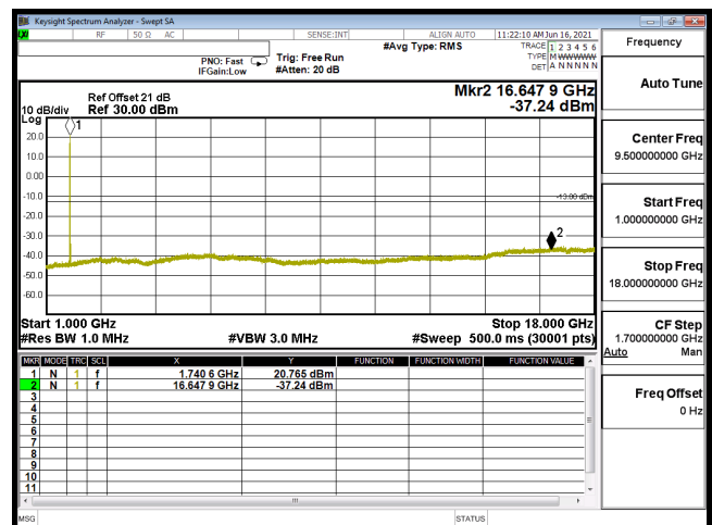
CSE B4 15M CH20325 16QAM(1,0) 1G-18G
