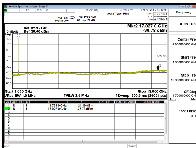
CSE B4 15M CH20175 QPSK(1,74) 1G-18G
