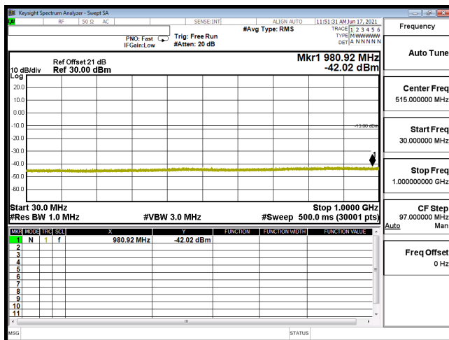
CSE B4 5M CH20375 QPSK(1,0) 30M-1G
