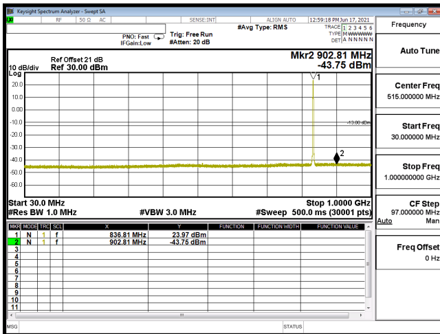
CSE B5 1.4M CH20525 16QAM(3,2) 30M-1G
