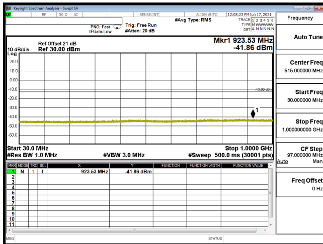
CSE B4 20M CH20175 16QAM(1,50) 30M-1G
