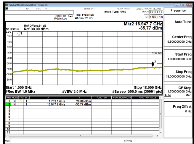
CSE B4 1.4M CH20175 16QAM(1,2) 1G-18G
