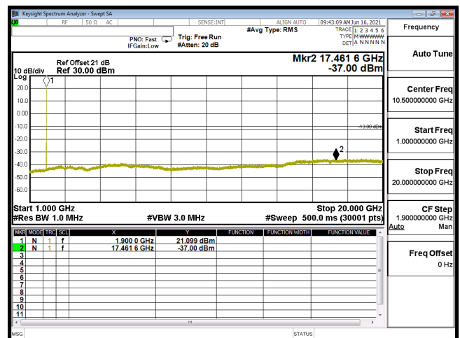
CSE B2 20M CH19100 16QAM(1,50) 1G-20G
