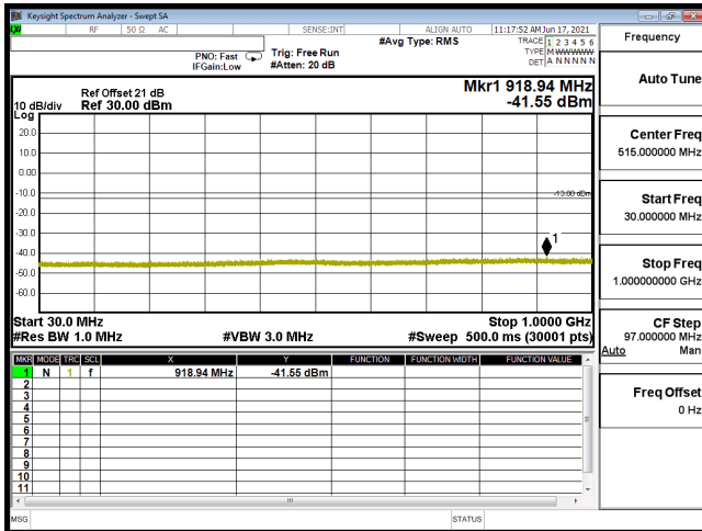
CSE B2 20M CH18900 16QAM(1,50) 30M-1G
