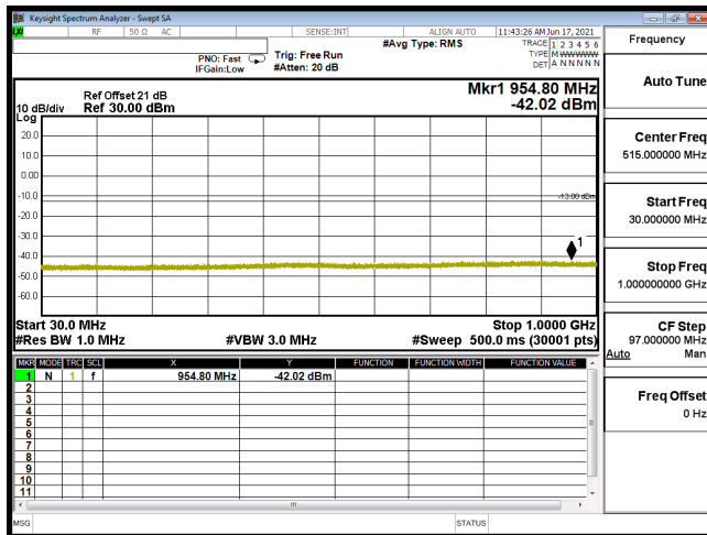
CSE B4 5M CH20175 16QAM(1,24) 30M-1G
