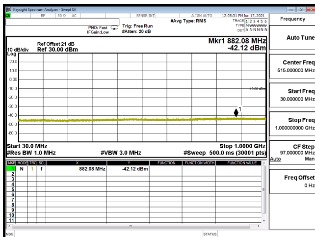
CSE B4 15M CH20325 16QAM(1,0) 30M-1G
