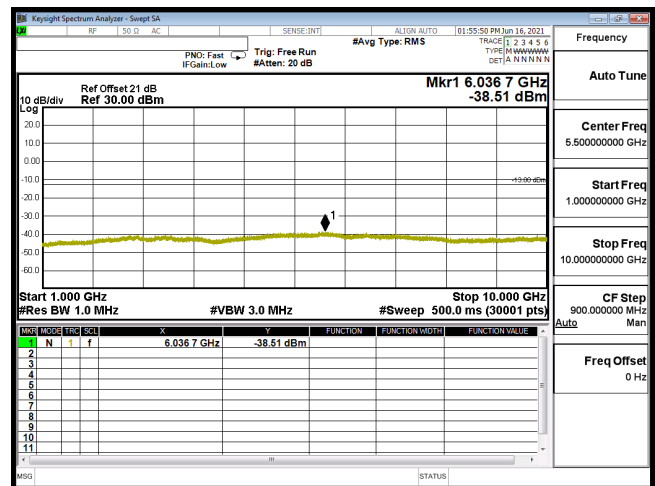
CSE B5 1.4M CH20643 QPSK(1,0) 1G-10G
