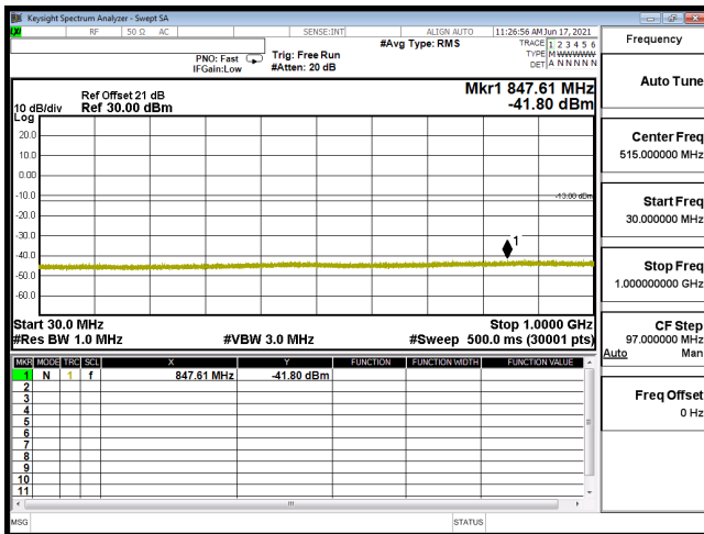
CSE B4 1.4M CH20175 16QAM(1,2) 30M-1G
