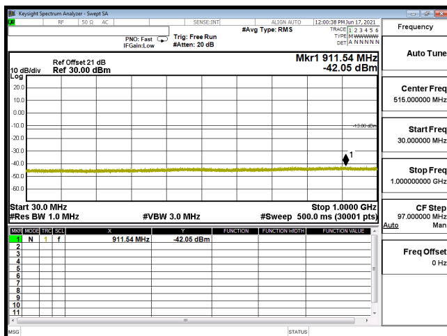
CSE B410M CH20175 QPSK(1,25) 30M-1G
