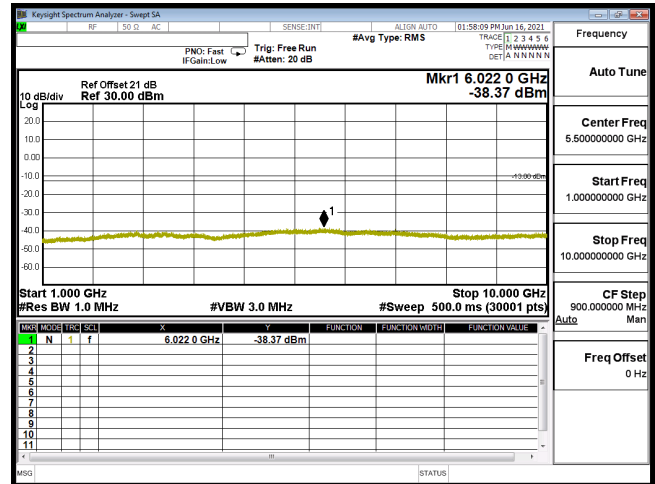
CSE B5 3M CH20415 QPSK(1,0) 1G-10G
