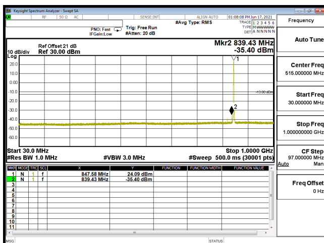
CSE B5 3M CH20635 16QAM(1,7) 30M-1G
