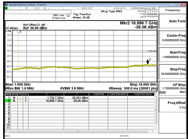
CSE B4 10M CH20175 16QAM(1,25) 1G-18G
