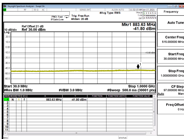
CSE B4 3M CH20175 QPSK(1,0) 30M-1G
