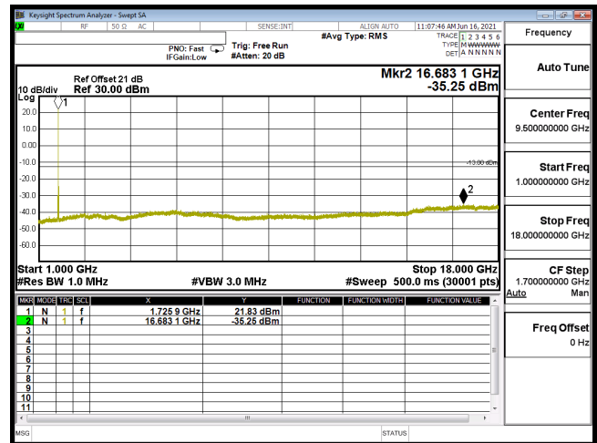
CSE B4 15M CH20175 16QAM(1,0) 1G-18G
