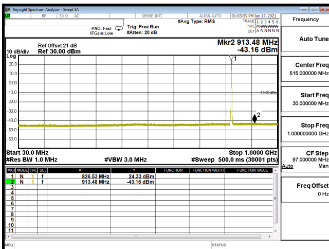
CSE B5 3M CH20415 16QAM(1,14) 30M-1G
