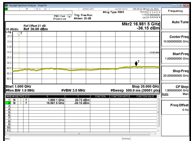
CSE B2 20M CH18700 16QAM(1,50) 1G-20G
