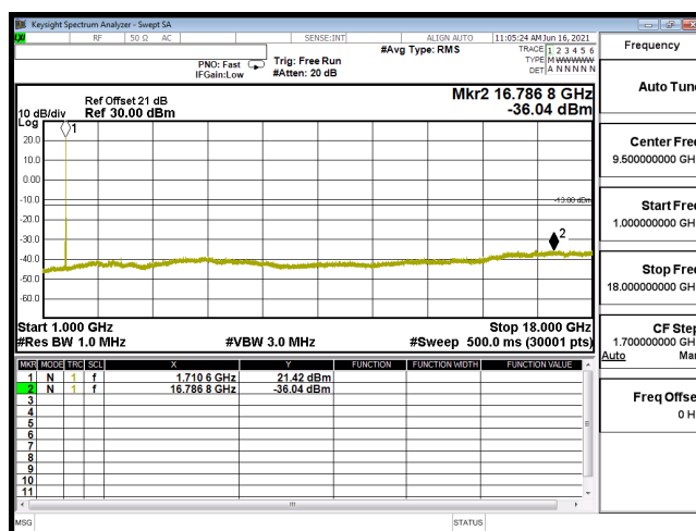
CSE B4 15M CH20025 16QAM(1,0) 1G-18G
