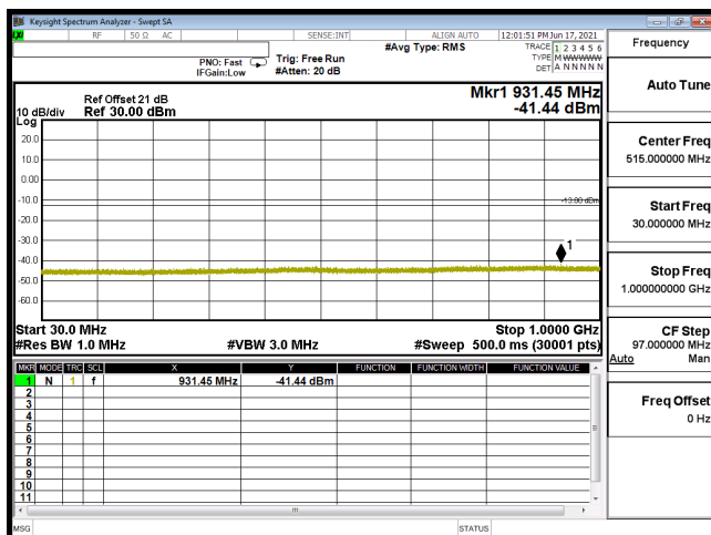
CSE B4 10M CH20350 16QAM(1,0) 30M-1G
