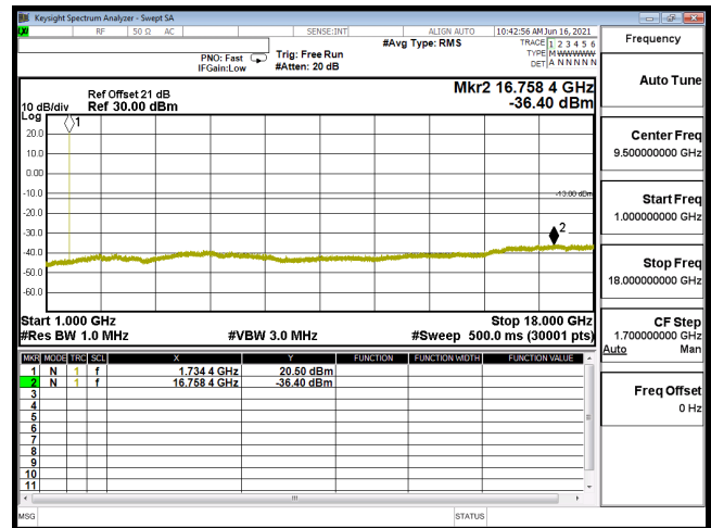
CSE B4 5M CH20175 16QAM(1,24) 1G-18G
