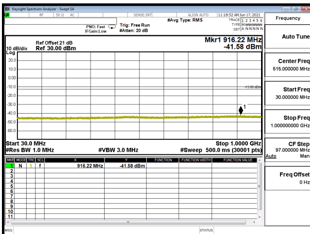
CSE B2 20M CH19100 QPSK(1,50) 30M-1G
