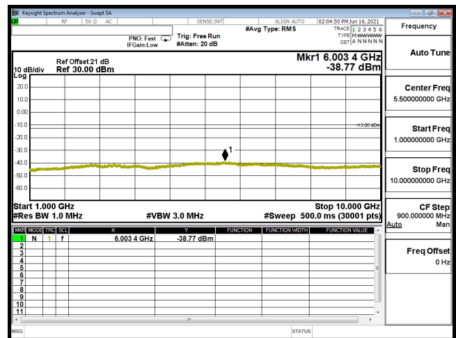
CSE B5 5M CH20425 16QAM(1,12) 1G-10G
