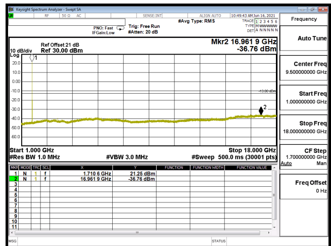
CSE B410M CH20000 16QAM(1,0) 1G-18G
