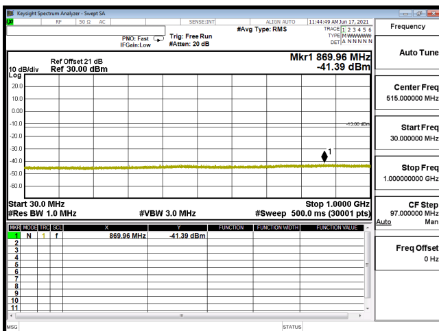
CSE B4 5M CH20175 QPSK(1,0) 30M-1G
