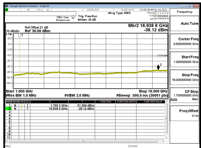
CSE B4 5M CH20375 16QAM(1,0) 1G-18G
