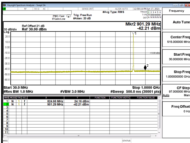
CSE B5 1.4M CH20407 16QAM(3,2) 30M-1G
