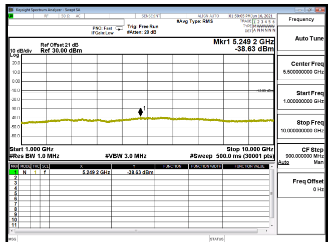
CSE B5 3M CH20525 QPSK(1,0) 1G-10G
