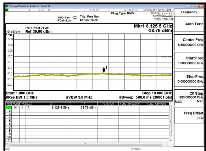
CSE B5 5M CH20525 QPSK(1,24) 1G-10G
