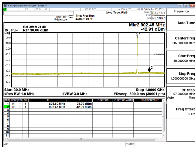
CSE B5 5M CH20425 16QAM(1,12) 30M-1G
