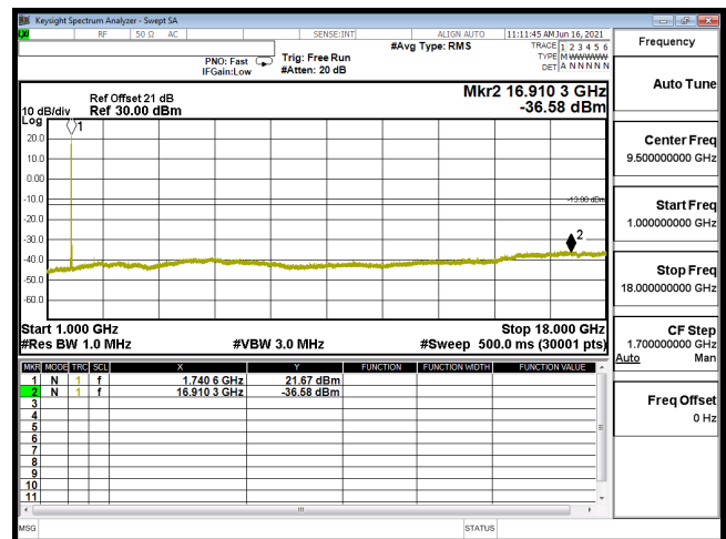
CSE B4 15M CH20325 QPSK(1,0) 1G-18G
