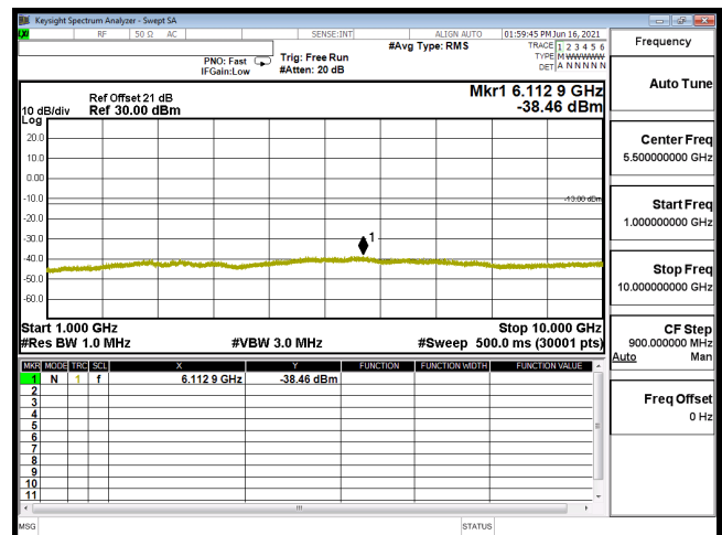
CSE B5 3M CH20525 16QAM(1,7) 1G-10G
