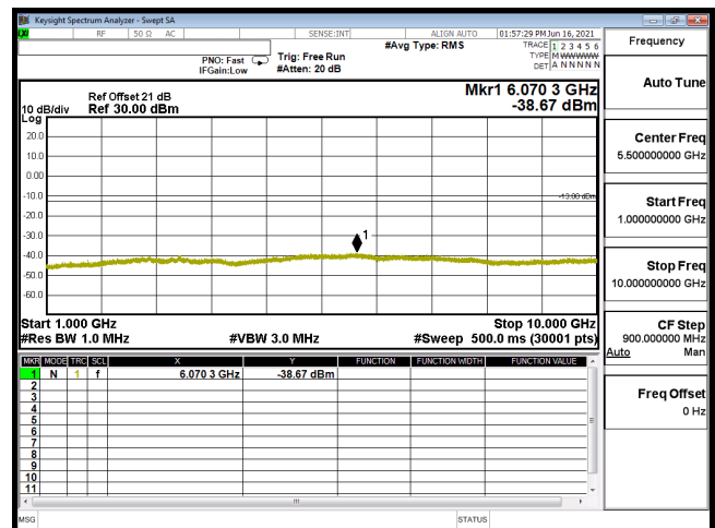
CSE B5 3M CH20415 16QAM(1,14) 1G-10G
