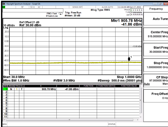
CSE B2 20M CH18700 QPSK(1,50) 30M-1G
