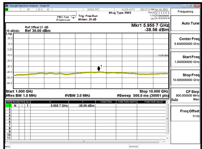
CSE B5 10M CH20450 16QAM(1,49) 1G-10G
