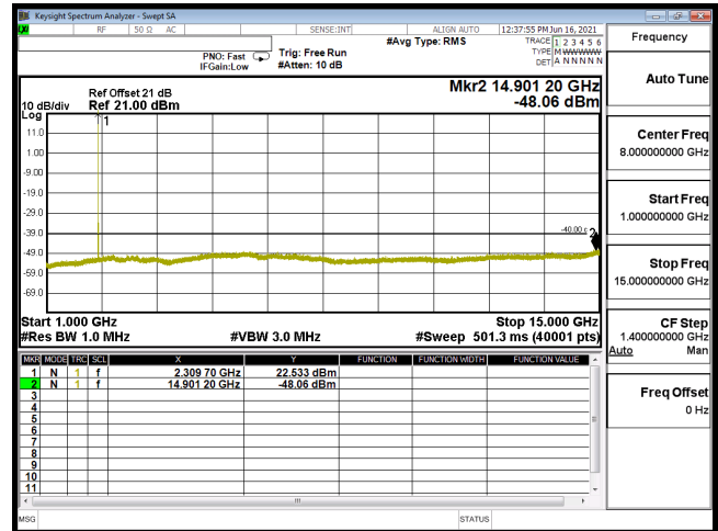
CSE B30 5M CH27685 QPSK(1,24) 1G-15G
