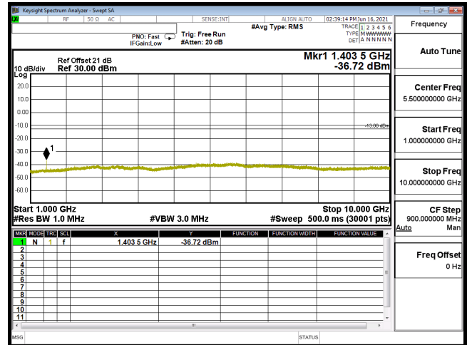
CSE B12 3M CH23025 QPSK(1,14) 1G-10G
