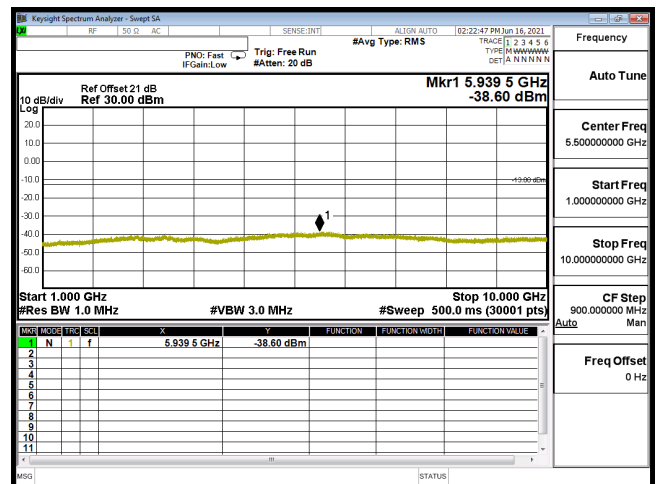
CSE B5 10M CH20600 QPSK(1,25) 1G-10G
