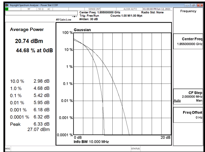
PTAR B2 10M CH18650 16QAM
