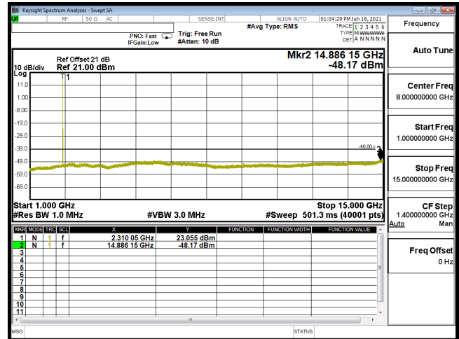
CSE B30 5M CH27710 QPSK(1,12) 1G-15G
