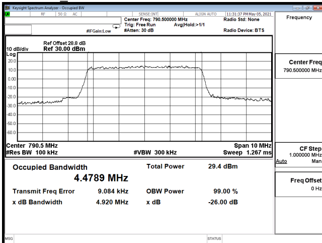
OCC-B14_5M-CH23305-64QAM
