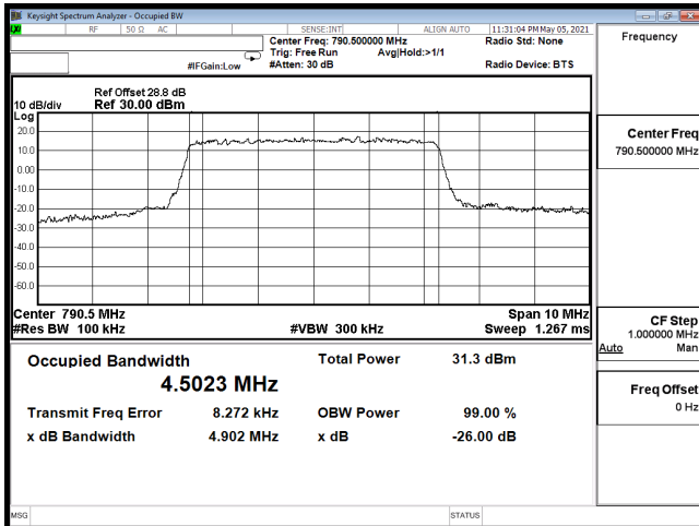
OCC-B14_5M-CH23305-QPSK
