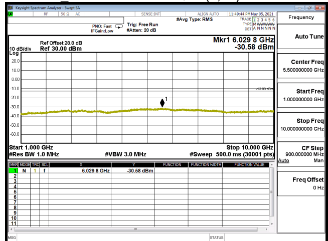
CSE-B14_10M-CH23355-64QAM(1,25)-1G-10G
