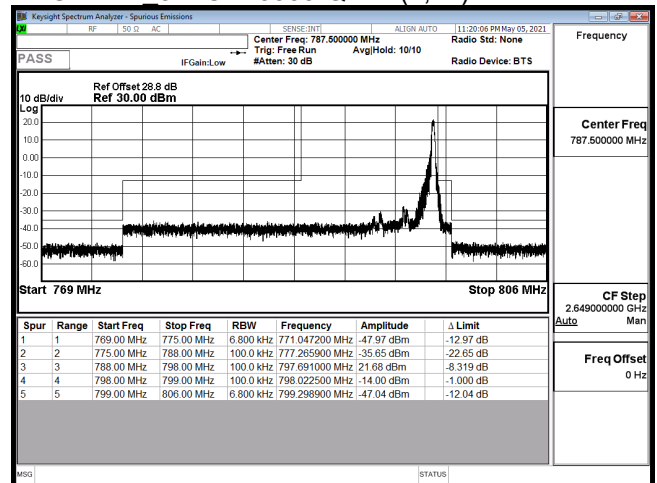
EDGE-B14 5M-CH23355-16QAM(1,24)
