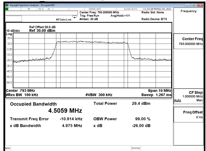
OCC-B14_5M-CH23330-64QAM
