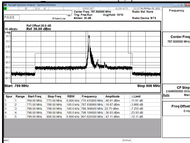
EDGE-B14 5M-CH23305-16QAM(1,0)
