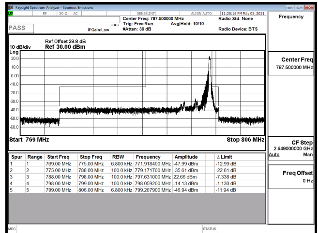
EDGE-B14 5M-CH23355-QPSK(1,24)
