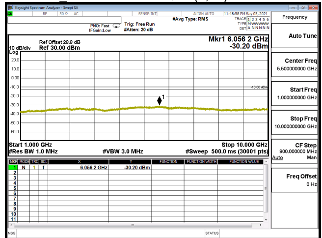
CSE-B14_5M-CH23355-64QAM(1,12)-1G-10G
