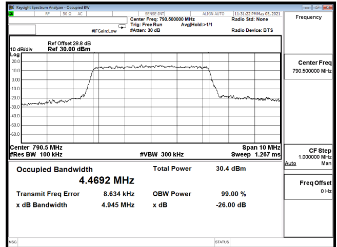
OCC-B14_5M-CH23305-16QAM
