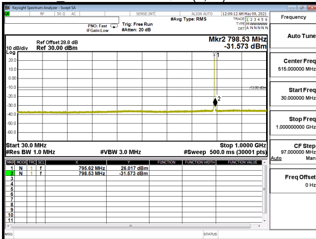
CSE-B14_5M-CH23355-64QAM(1,12)-30M-1G
