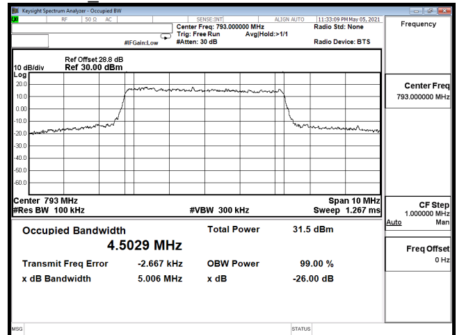
OCC-B14_5M-CH23330-QPSK
