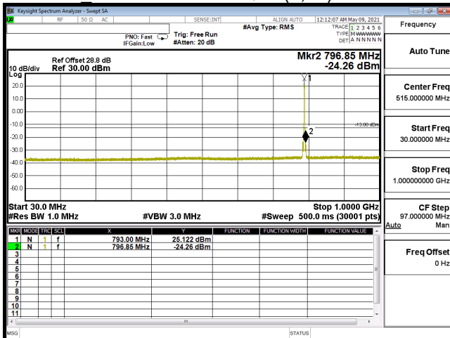
CSE-B14_10M-CH23355-64QAM(1,25)-30M-1G
