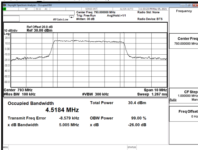
OCC-B14_5M-CH23330-16QAM
