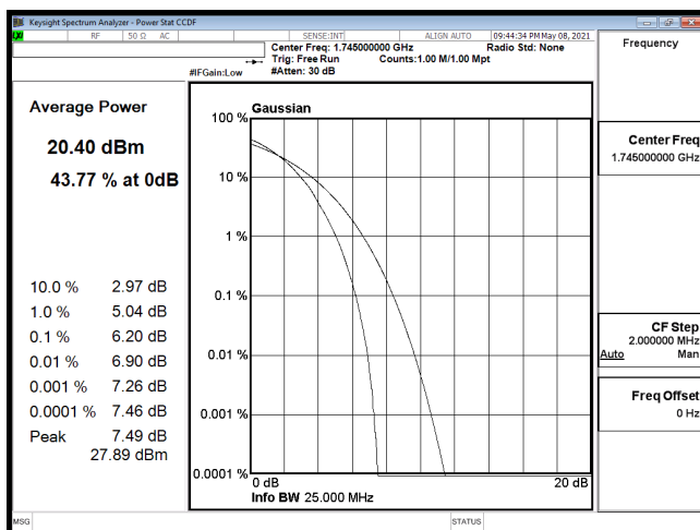
PTAR-B66_20M-CH132322-64QAM
