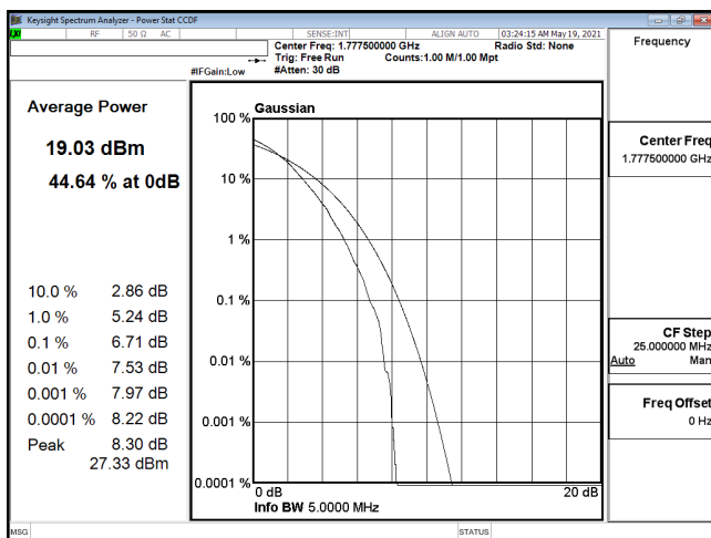
PTAR-ENDC_12A_n66-256QAM_5M_CH355500_1777.5(25,0)
