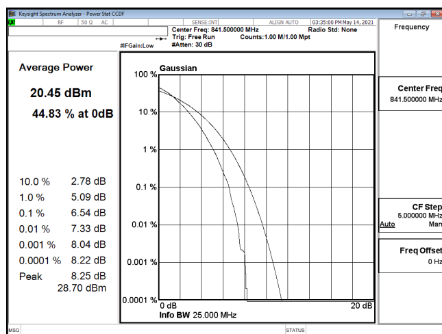
PTAR-ENDC_30A_n5-256QAM_15M_CH168300_841.5(75,0)
