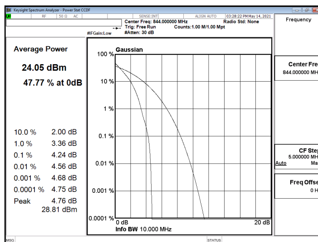
PTAR-ENDC_30A_n5-PI2-BPSK_10M_CH168800_844(50,0)
