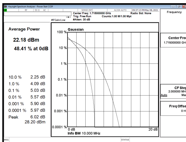
PTAR-B66_10M-CH132022-QPSK
