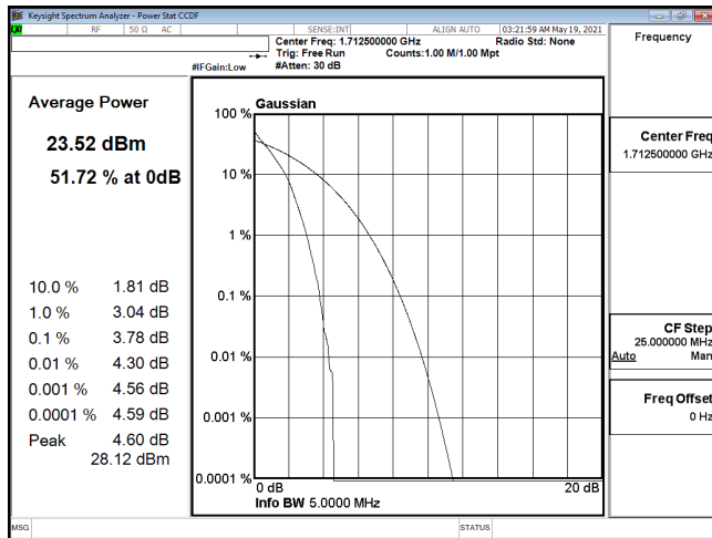
PTAR-ENDC_12A_n66-PI2-BPSK_5M_CH342500_1712.5(25,0)
