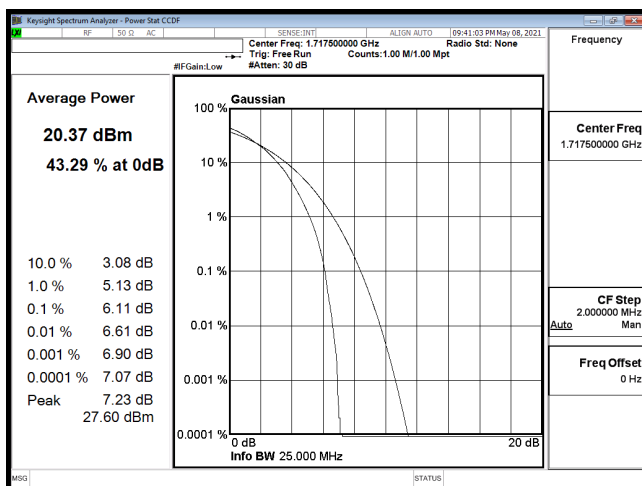
PTAR-B66_15M-CH132047-64QAM
