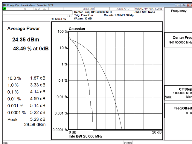
PTAR-ENDC_30A_n5-PI2-BPSK_15M_CH168300_841.5(75,0)
