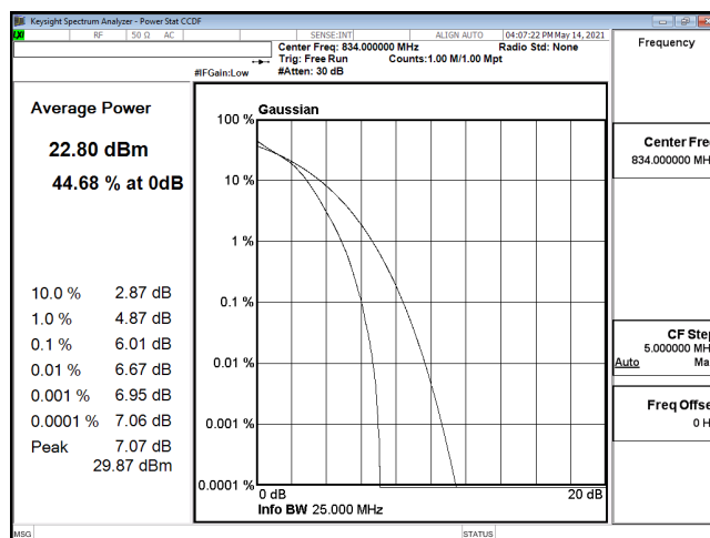
PTAR-ENDC_30A_n5-16QAM_20M_CH166800_834(100,0)
