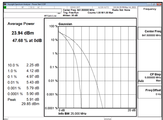
PTAR-ENDC_30A_n5-QPSK_15M_CH168300_841.5(75,0)
