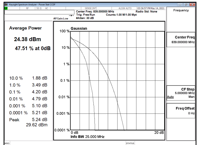
PTAR-ENDC_30A_n5-PI2-BPSK_20M_CH167800_839(100,0)
