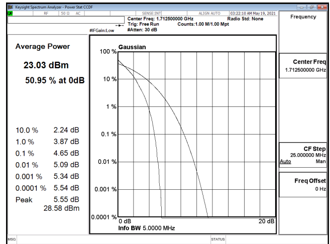
PTAR-ENDC_12A_n66-QPSK_5M_CH342500_1712.5(25,0)
