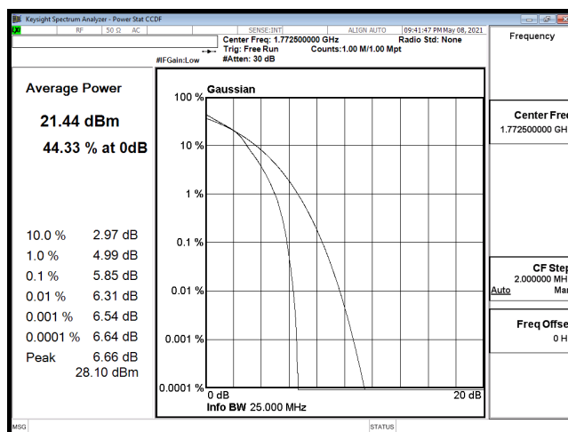
PTAR-B66_15M-CH132597-16QAM
