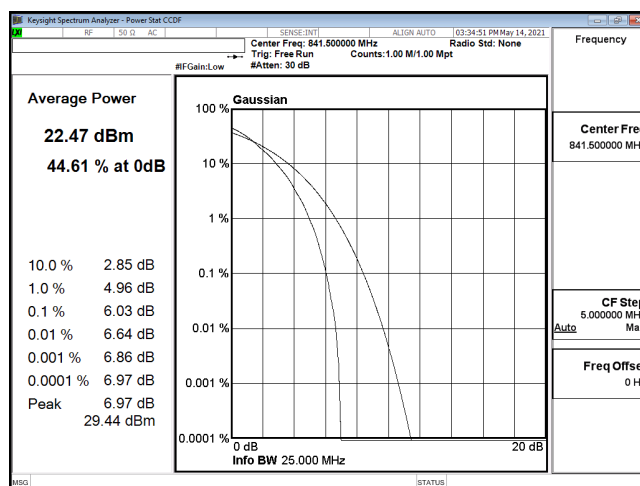
PTAR-ENDC_30A_n5-64QAM_15M_CH168300_841.5(75,0)
