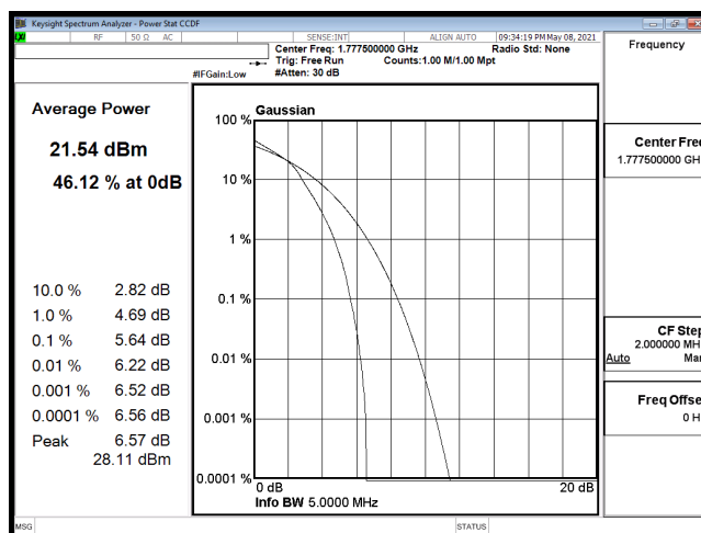
PTAR-B66_5M-CH132647-16QAM
