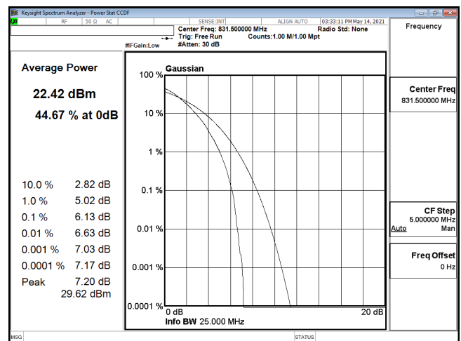
PTAR-ENDC_30A_n5-64QAM_15M_CH166300_831.5(75,0)
