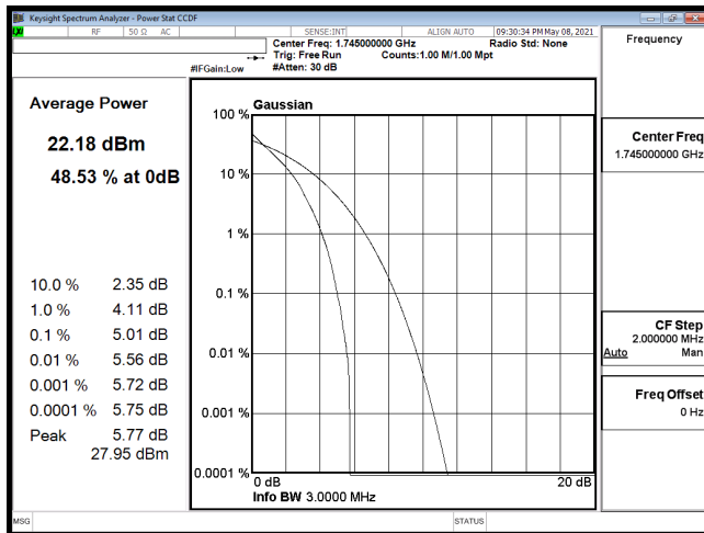
PTAR-B66_3M-CH132322-QPSK
