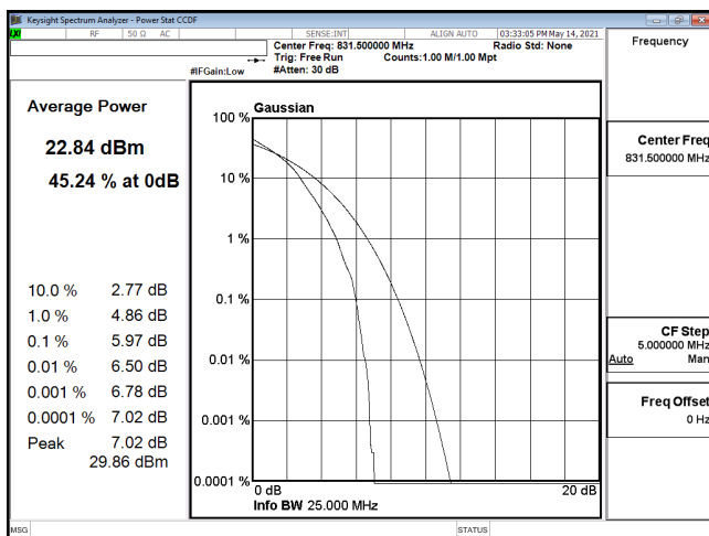
PTAR-ENDC_30A_n5-16QAM_15M_CH166300_831.5(75,0)
