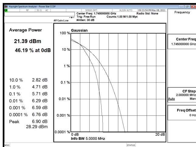
PTAR-B66_5M-CH132322-16QAM
