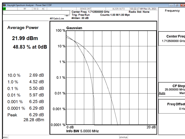
PTAR-ENDC_12A_n66-16QAM_5M_CH342500_1712.5(25,0)
