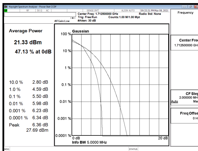
PTAR-B66_5M-CH131997-16QAM
