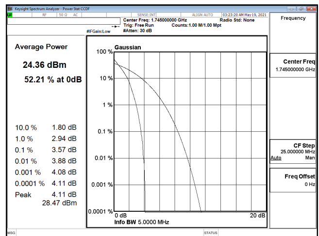
PTAR-ENDC_12A_n66-PI2-BPSK_5M_CH349000_1745(25,0)
