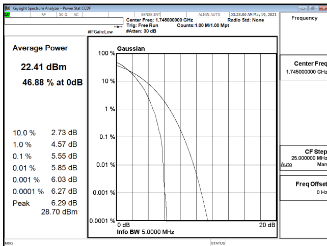
PTAR-ENDC_12A_n66-64QAM_5M_CH349000_1745(25,0)
