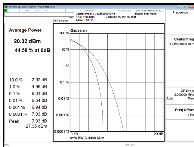
PTAR-B66_5M-CH131997-64QAM
