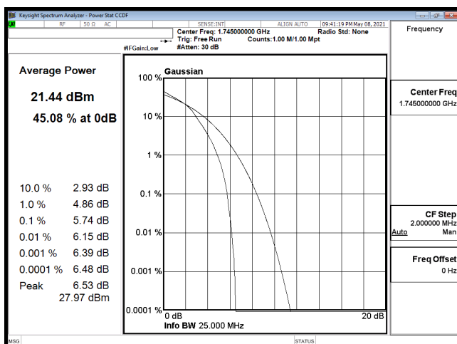
PTAR-B66_15M-CH132322-16QAM
