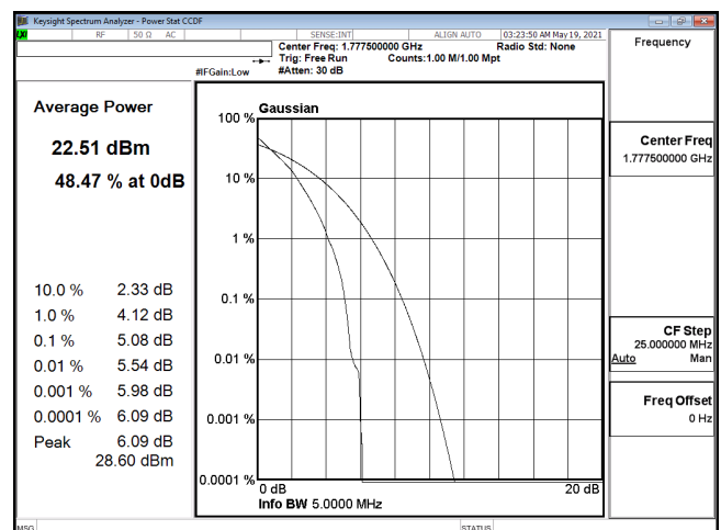
PTAR-ENDC_12A_n66-QPSK_5M_CH355500_1777.5(25,0)
