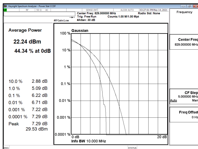
PTAR-ENDC_30A_n5-64QAM_10M_CH165800_829(50,0)
