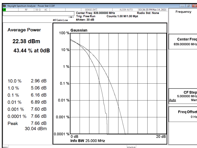
PTAR-ENDC_30A_n5-64QAM_20M_CH167800_839(100,0)
