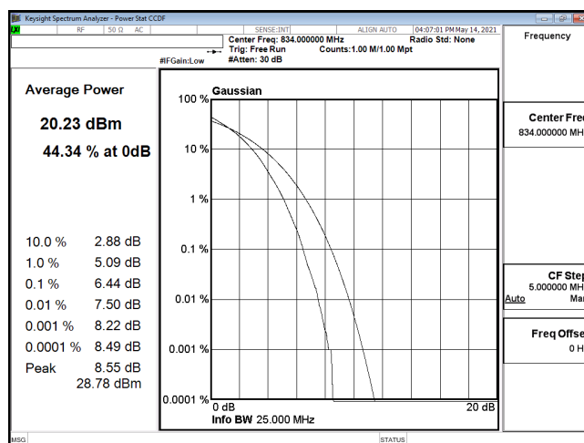
PTAR-ENDC_30A_n5-256QAM_20M_CH166800_834(100,0)
