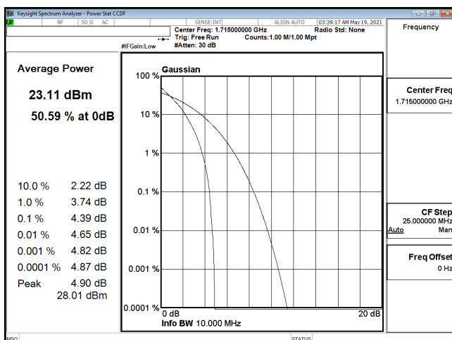
PTAR-ENDC_12A_n66-QPSK_10M_CH343000_1715(50,0)
