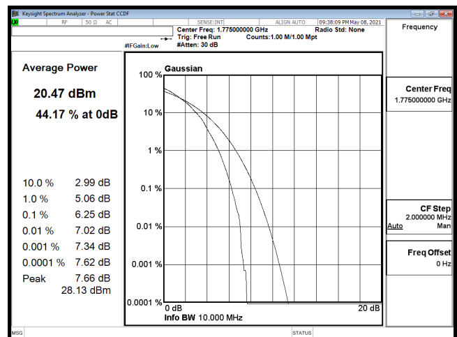
PTAR-B66_10M-CH132622-64QAM
