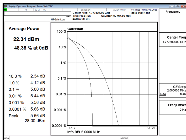
PTAR-B66_5M-CH132647-QPSK
