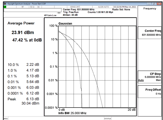
PTAR-ENDC_30A_n5-QPSK_15M_CH166300_831.5(75,0)
