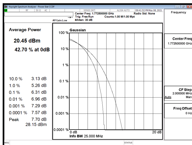
PTAR-B66_15M-CH132597-64QAM
