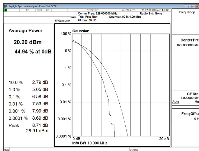
PTAR-ENDC_30A_n5-256QAM_10M_CH165800_829(50,0)
