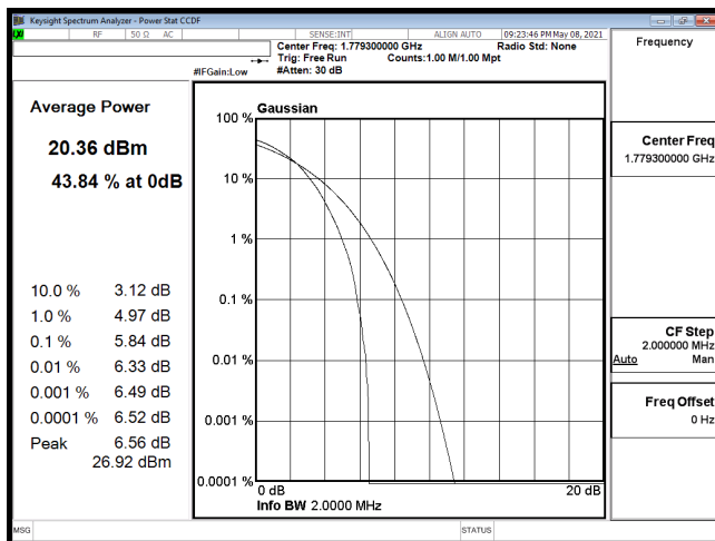
PTAR-B66_1.4M-CH132665-64QAM
