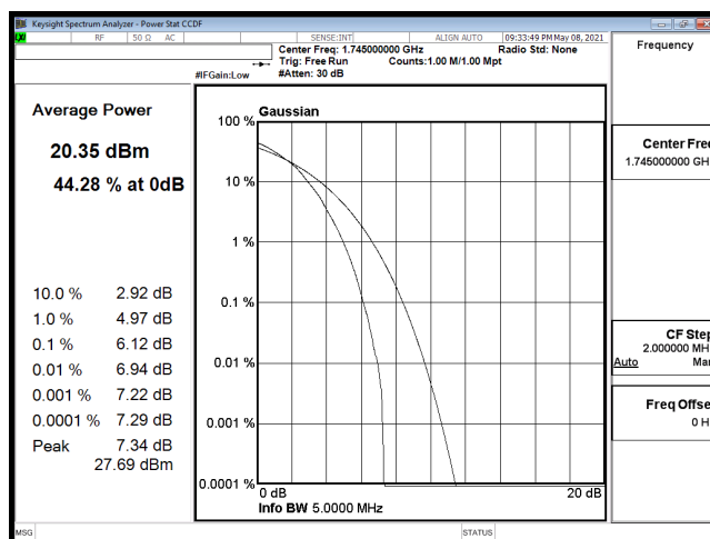
PTAR-B66_5M-CH132322-64QAM
