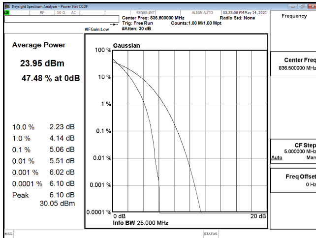
PTAR-ENDC_30A_n5-QPSK_15M_CH167300_836.5(75,0)
