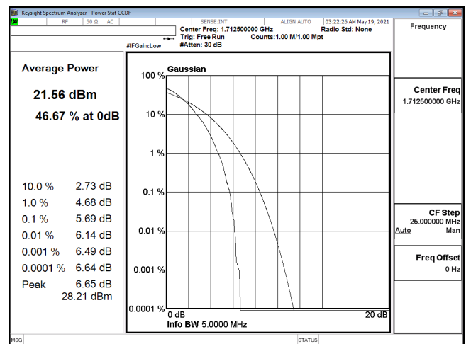
PTAR-ENDC_12A_n66-64QAM_5M_CH342500_1712.5(25,0)
