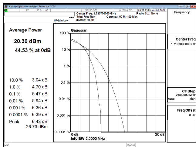
PTAR-B66_1.4M-CH131979-64QAM
