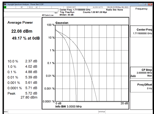
PTAR-B66_3M-CH131987-QPSK
