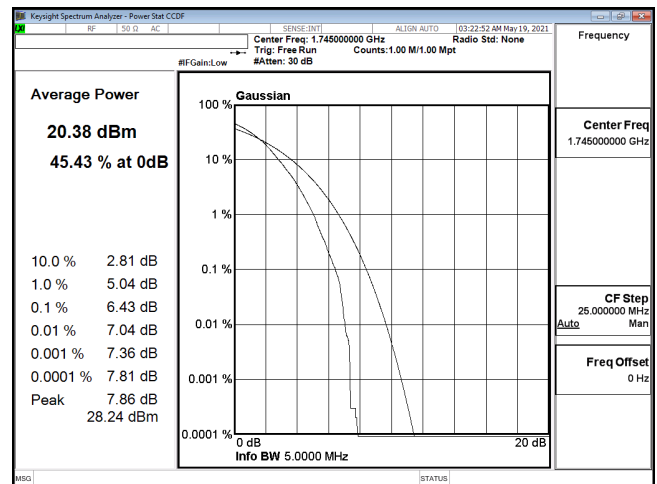
PTAR-ENDC_12A_n66-256QAM_5M_CH349000_1745(25,0)
