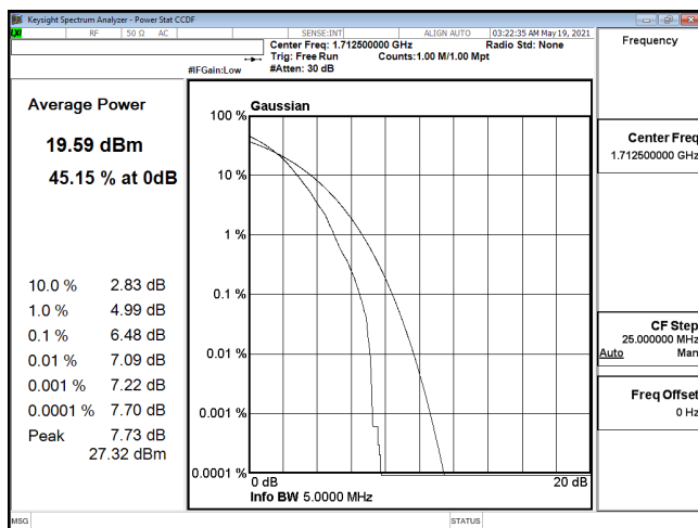
PTAR-ENDC_12A_n66-256QAM_5M_CH342500_1712.5(25,0)
