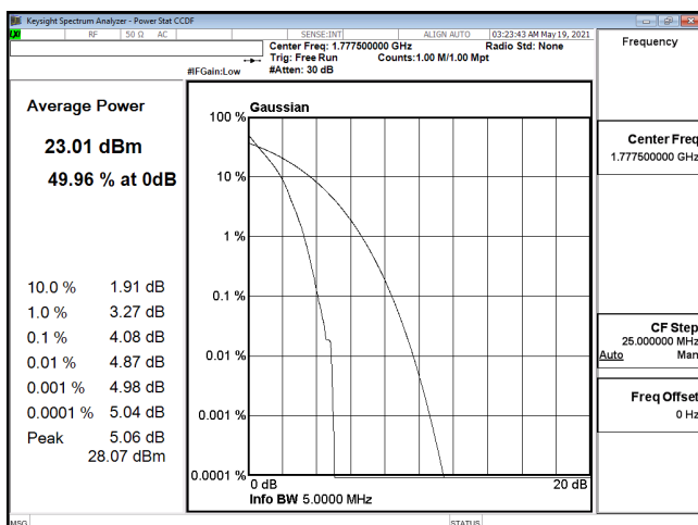
PTAR-ENDC_12A_n66-PI2-BPSK_5M_CH355500_1777.5(25,0)
