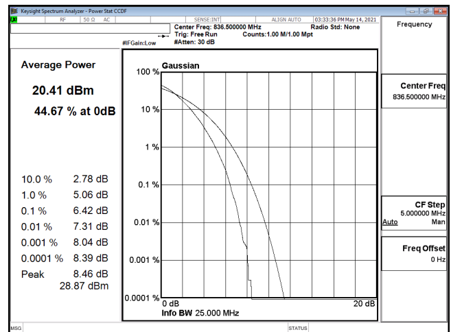
PTAR-ENDC_30A_n5-256QAM_15M_CH167300_836.5(75,0)
