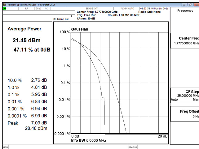
PTAR-ENDC_12A_n66-16QAM_5M_CH355500_1777.5(25,0)
