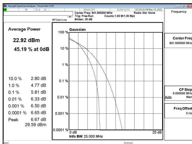
PTAR-ENDC_30A_n5-16QAM_15M_CH168300_841.5(75,0)
