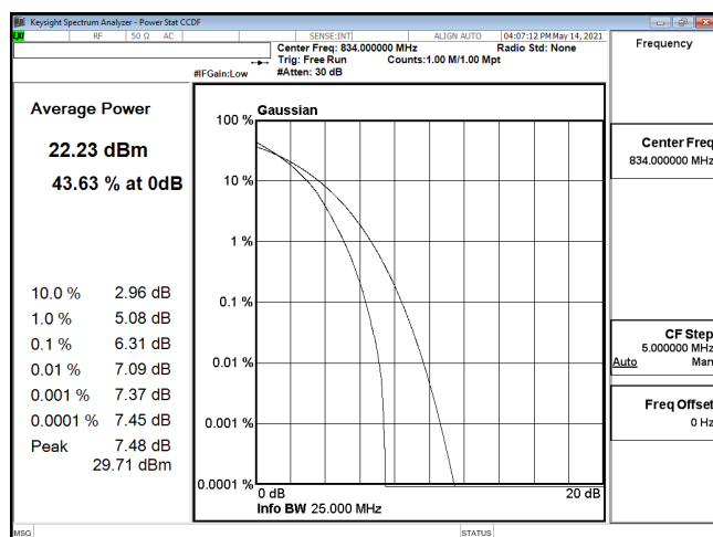
PTAR-ENDC_30A_n5-64QAM_20M_CH166800_834(100,0)
