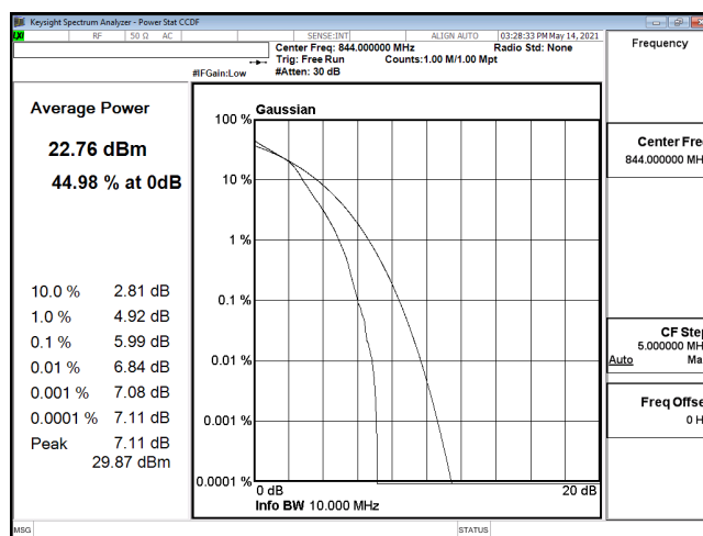
PTAR-ENDC_30A_n5-16QAM_10M_CH168800_844(50,0)
