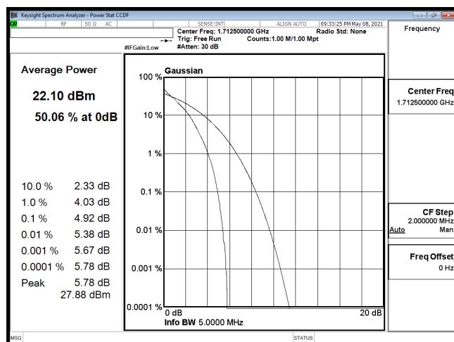
PTAR-B66_5M-CH131997-QPSK
