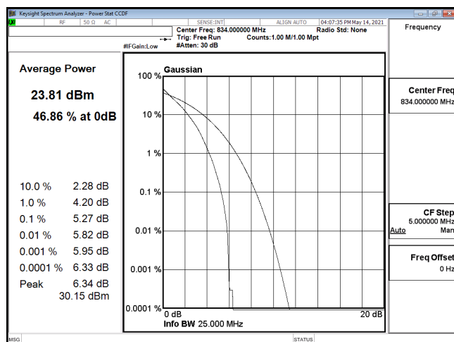
PTAR-ENDC_30A_n5-QPSK_20M_CH166800_834(100,0)
