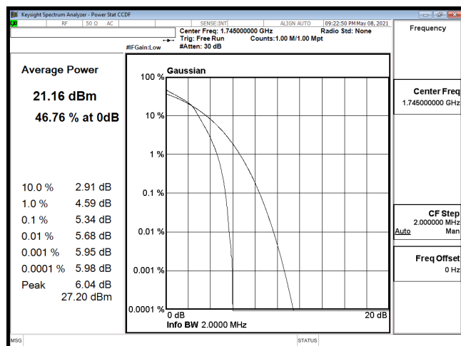
PTAR-B66_1.4M-CH132322-16QAM
