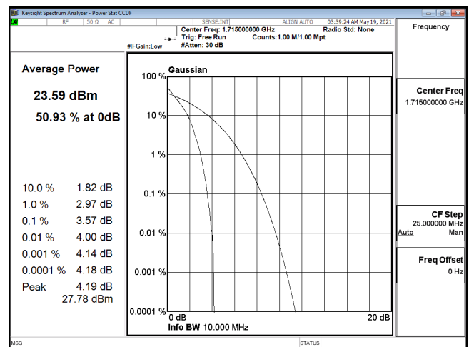
PTAR-ENDC_12A_n66-PI2-BPSK_10M_CH343000_1715(50,0)
