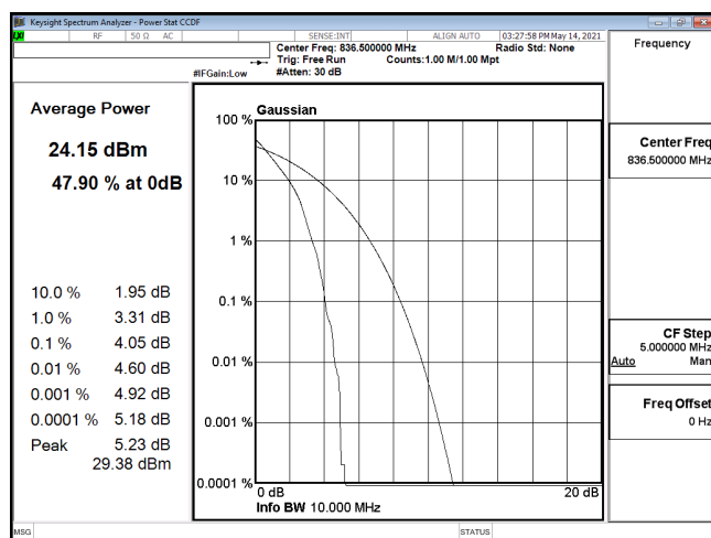
PTAR-ENDC_30A_n5-PI2-BPSK_10M_CH167300_836.5(50,0)
