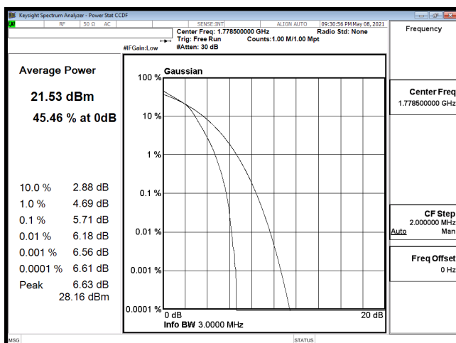
PTAR-B66_3M-CH132657-16QAM
