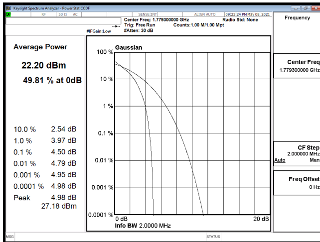
PTAR-B66_1.4M-CH132665-QPSK
