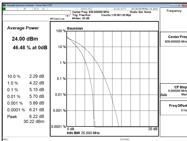
PTAR-ENDC_30A_n5-QPSK_20M_CH167800_839(100,0)
