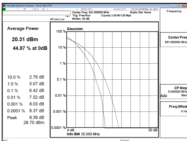
PTAR-ENDC_30A_n5-256QAM_15M_CH166300_831.5(75,0)
