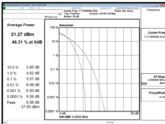
PTAR-B66_3M-CH131987-16QAM
