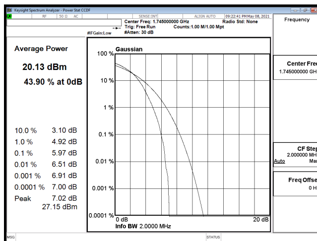
PTAR-B66_1.4M-CH132322-64QAM
