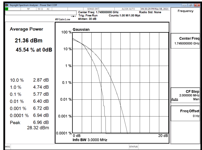
PTAR-B66_3M-CH132322-16QAM
