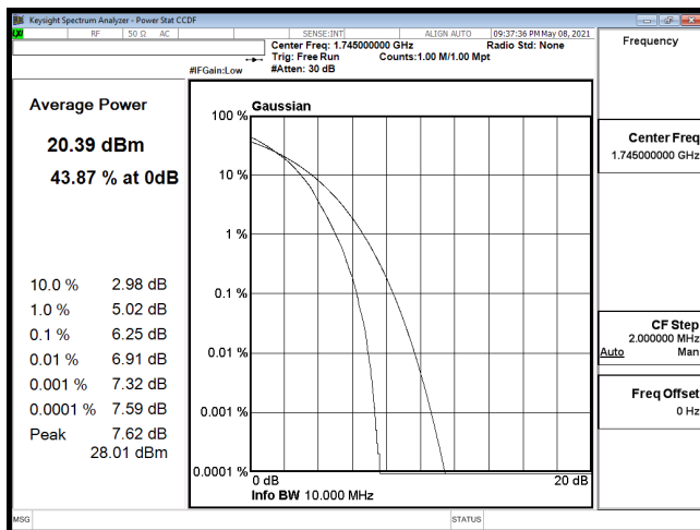
PTAR-B66_10M-CH132322-64QAM
