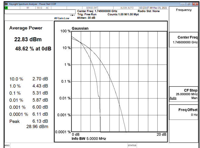
PTAR-ENDC_12A_n66-16QAM_5M_CH349000_1745(25,0)
