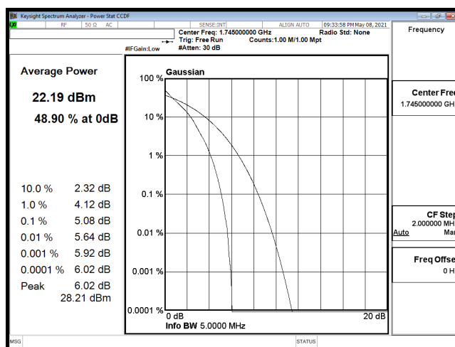
PTAR-B66_5M-CH132322-QPSK
