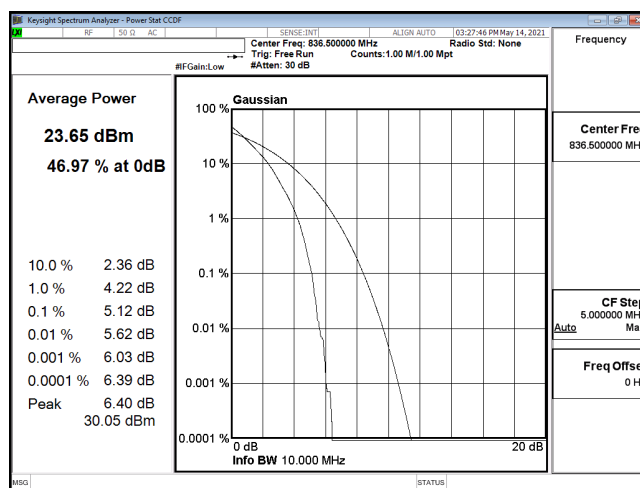
PTAR-ENDC_30A_n5-QPSK_10M_CH167300_836.5(50,0)
