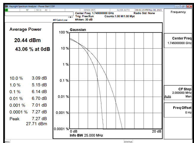
PTAR-B66_15M-CH132322-64QAM
