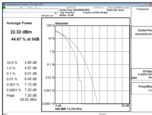
PTAR-ENDC_30A_n5-64QAM_10M_CH167300_836.5(50,0)
