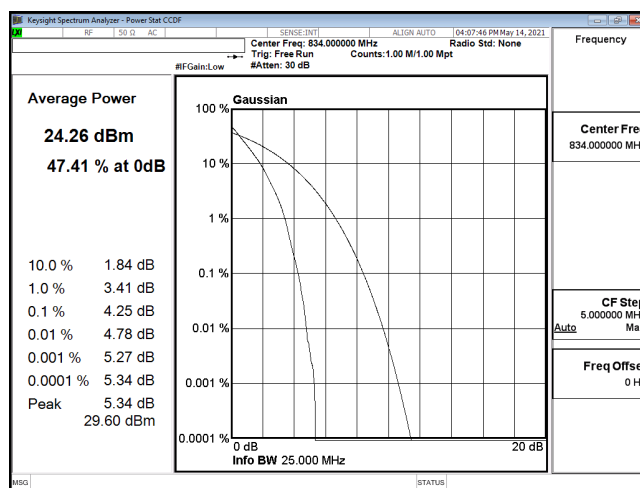
PTAR-ENDC_30A_n5-PI2-BPSK_20M_CH166800_834(100,0)
