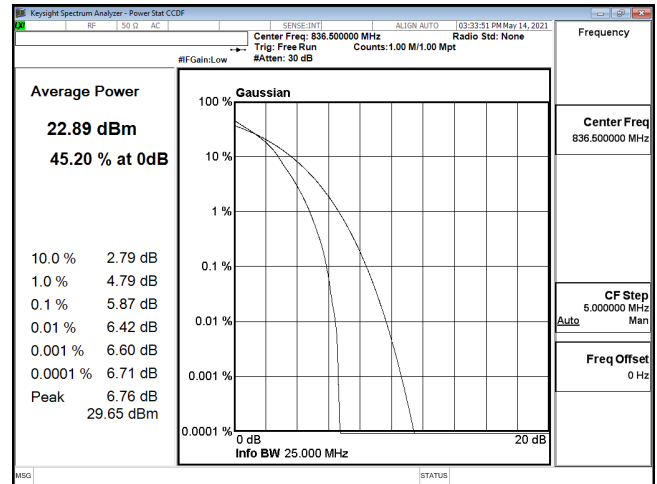
PTAR-ENDC_30A_n5-16QAM_15M_CH167300_836.5(75,0)
