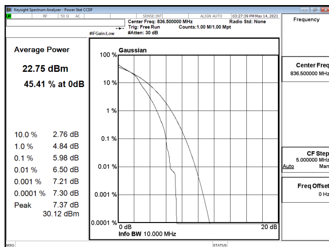
PTAR-ENDC_30A_n5-16QAM_10M_CH167300_836.5(50,0)
