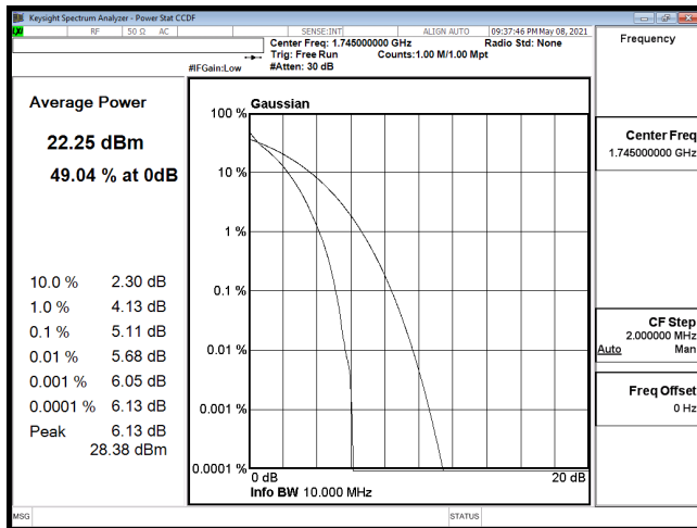
PTAR-B66_10M-CH132322-QPSK
