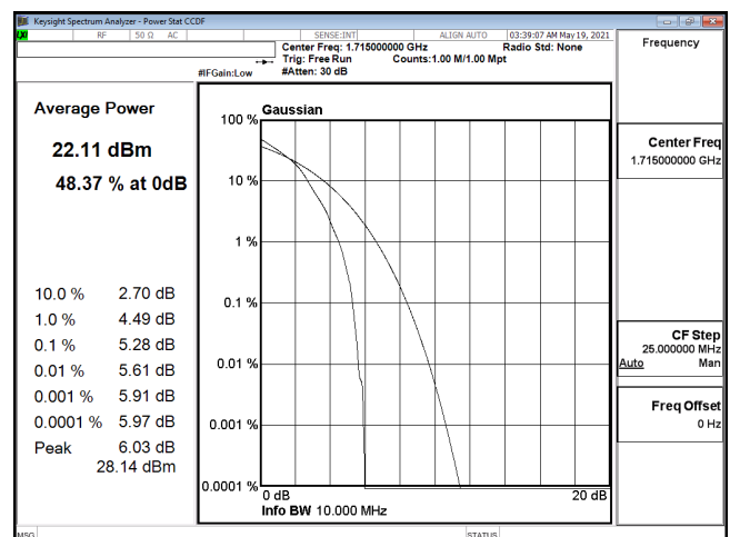
PTAR-ENDC_12A_n66-16QAM_10M_CH343000_1715(50,0)
