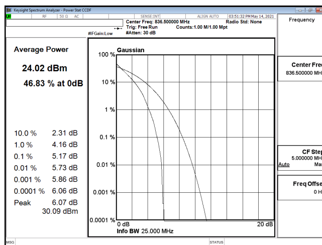
PTAR-ENDC_30A_n5-QPSK_20M_CH167300_836.5(100,0)
