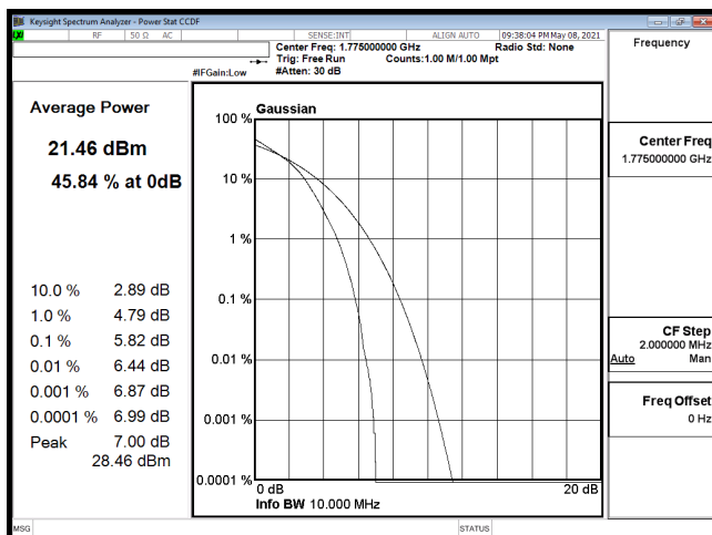
PTAR-B66_10M-CH132622-16QAM
