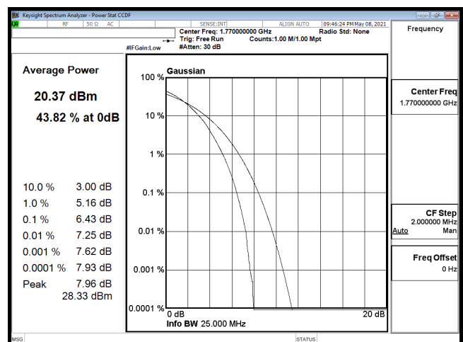
PTAR-B66_20M-CH132572-64QAM
