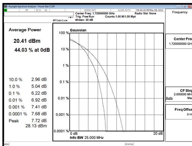
PTAR-B66_20M-CH132072-64QAM
