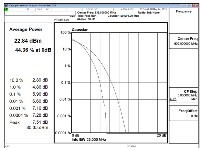
PTAR-ENDC_30A_n5-16QAM_20M_CH167800_839(100,0)
