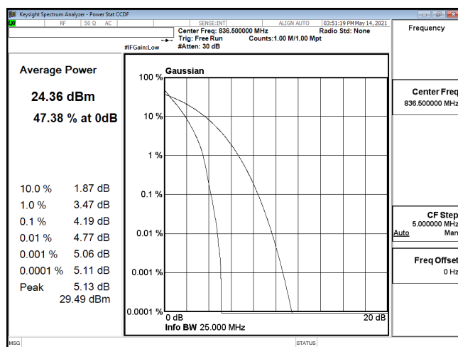
PTAR-ENDC_30A_n5-PI2-BPSK_20M_CH167300_836.5(100,0)
