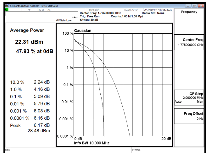
PTAR-B66_10M-CH132622-QPSK
