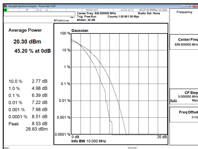
PTAR-ENDC_30A_n5-256QAM_10M_CH167300_836.5(50,0)
