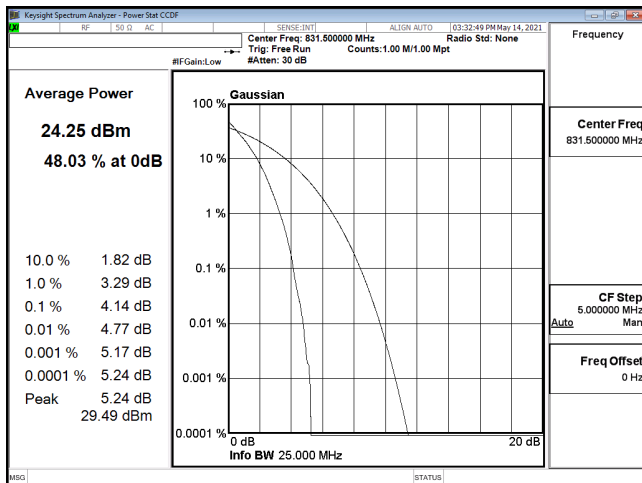
PTAR-ENDC_30A_n5-PI2-BPSK_15M_CH166300_831.5(75,0)
