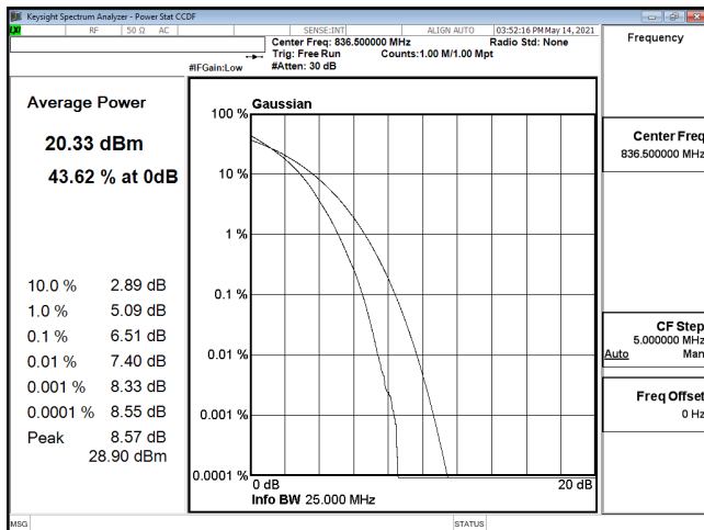
PTAR-ENDC_30A_n5-256QAM_20M_CH167300_836.5(100,0)
