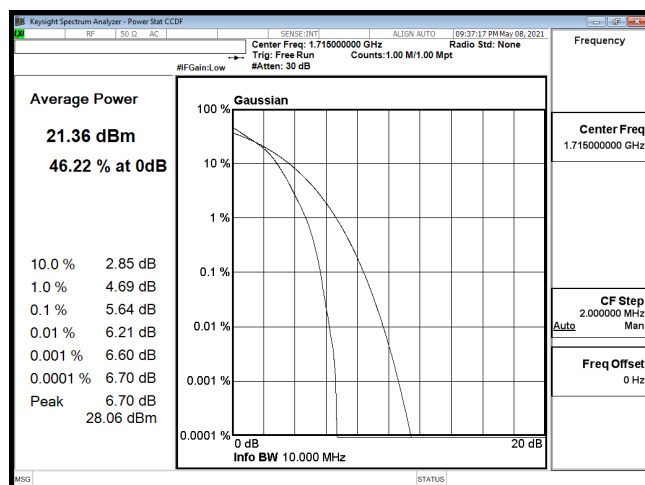
PTAR-B66_10M-CH132022-16QAM
