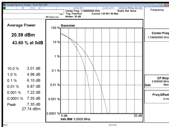
PTAR-B66_3M-CH132322-64QAM
