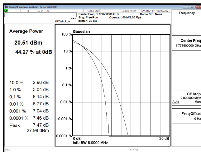
PTAR-B66_5M-CH132647-64QAM
