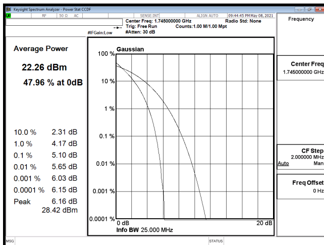
PTAR-B66_20M-CH132322-QPSK
