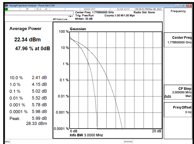
PTAR-B66_3M-CH132657-QPSK
