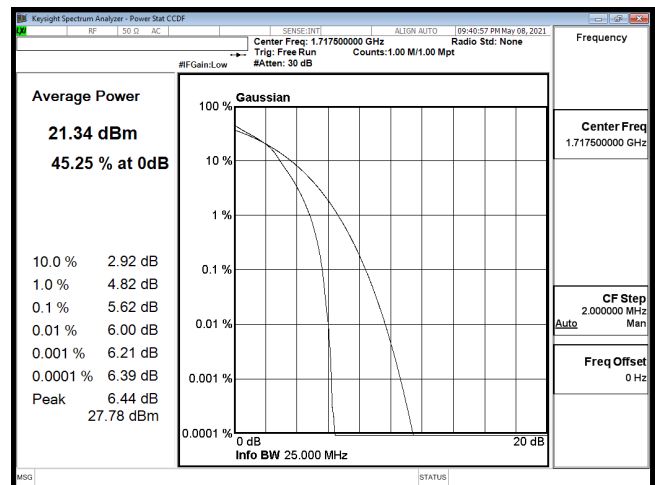
PTAR-B66_15M-CH132047-16QAM
