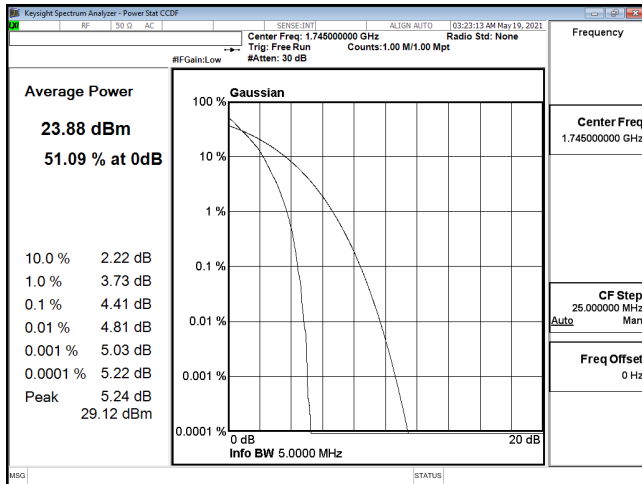
PTAR-ENDC_12A_n66-QPSK_5M_CH349000_1745(25,0)
