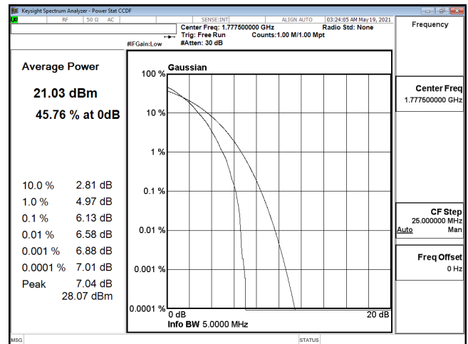
PTAR-ENDC_12A_n66-64QAM_5M_CH355500_1777.5(25,0)
