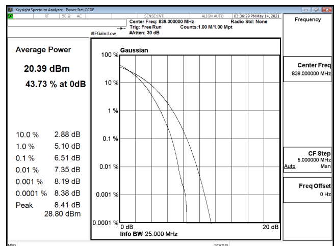
PTAR-ENDC_30A_n5-256QAM_20M_CH167800_839(100,0)
