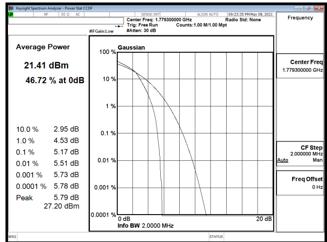
PTAR-B66_1.4M-CH132665-16QAM
