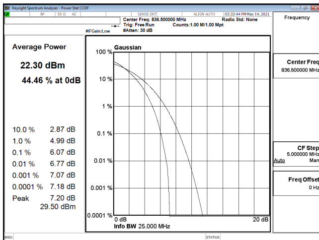
PTAR-ENDC_30A_n5-64QAM_15M_CH167300_836.5(75,0)
