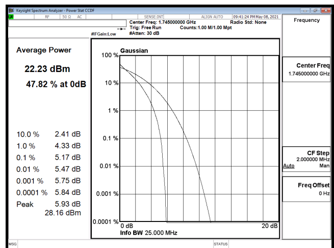
PTAR-B66_15M-CH132322-QPSK
