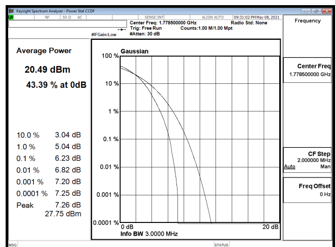
PTAR-B66_3M-CH132657-64QAM
