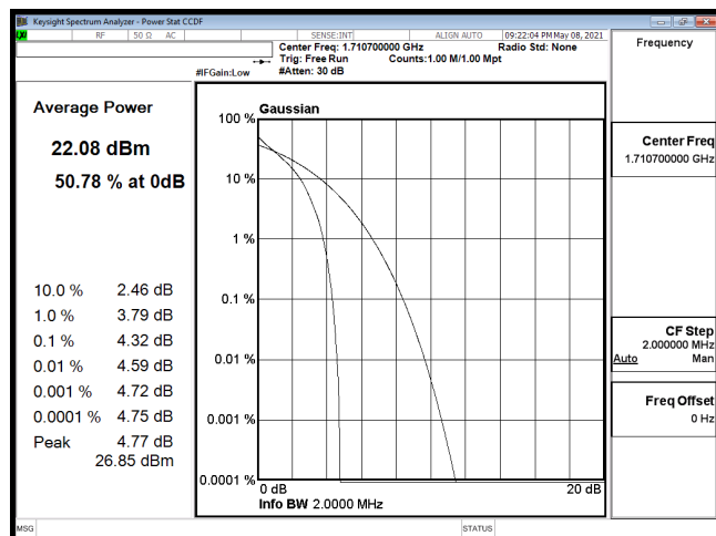
PTAR-B66_1.4M-CH131979-QPSK
