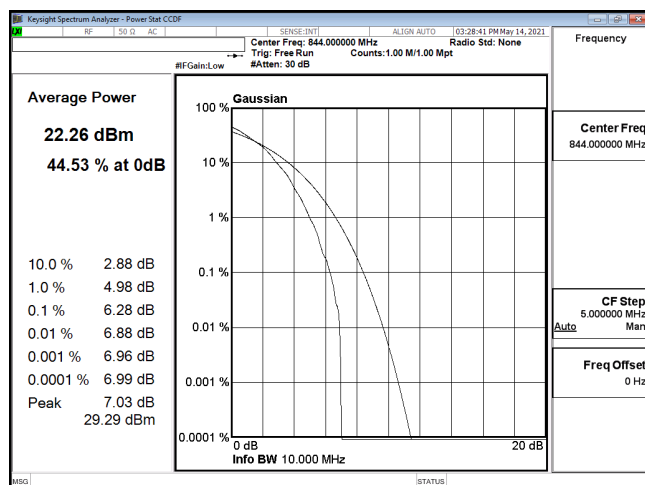
PTAR-ENDC_30A_n5-64QAM_10M_CH168800_844(50,0)
