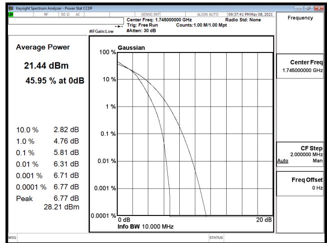
PTAR-B66_10M-CH132322-16QAM
