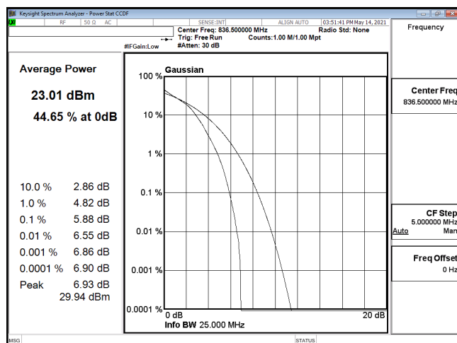
PTAR-ENDC_30A_n5-16QAM_20M_CH167300_836.5(100,0)
