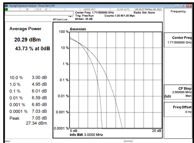
PTAR-B66_3M-CH131987-64QAM
