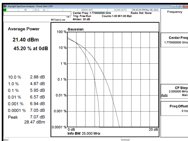
PTAR-B66_20M-CH132572-16QAM
