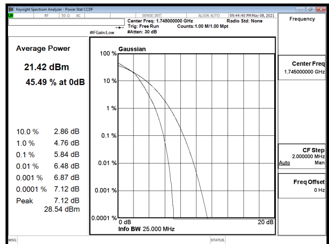
PTAR-B66_20M-CH132322-16QAM
