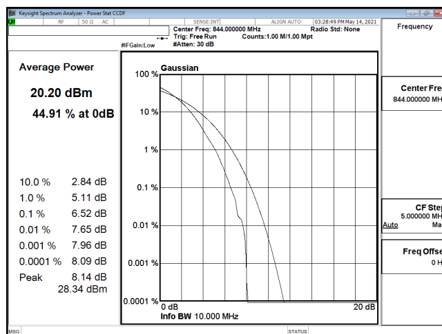
PTAR-ENDC_30A_n5-256QAM_10M_CH168800_844(50,0)
