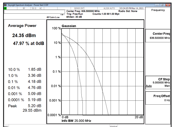
PTAR-ENDC_30A_n5-PI2-BPSK_15M_CH167300_836.5(75,0)
