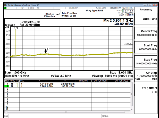
CSE-B66_1.4M-CH131979-64QAM(1,0)-1G-18G
