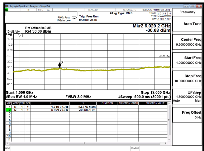
CSE-B66_1.4M-CH131979-16QAM(1,0)-1G-18G
