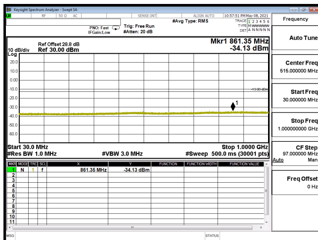
CSE-B66_1.4M-CH131979-16QAM(1,0)-30M-1G
