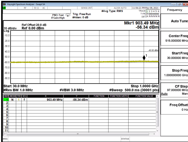
CSE-B30_5M-CH27735-QPSK(1,12)-30M-1G
