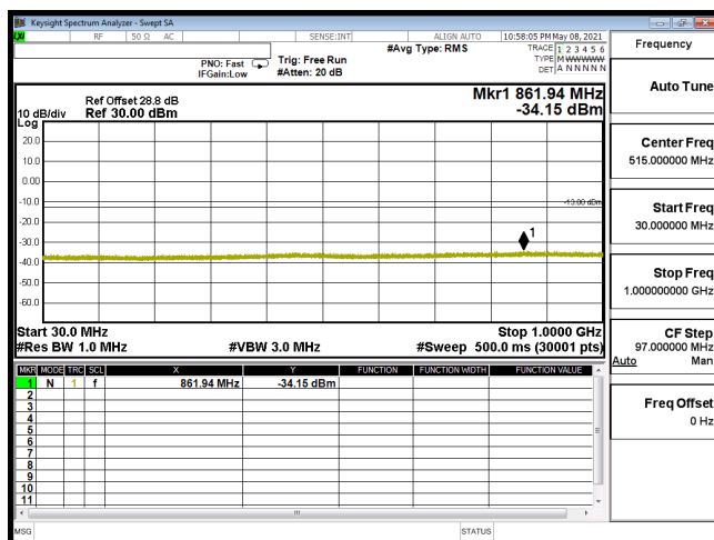
CSE-B66_1.4M-CH131979-64QAM(1,0)-30M-1G
