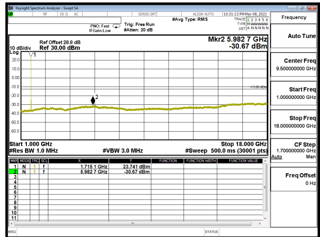
CSE-B66_10M-CH132022-QPSK(1,25)-1G-18G
