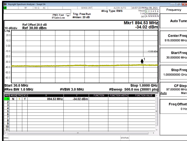
CSE-B66_1.4M-CH131979-QPSK(1,5)-30M-1G
