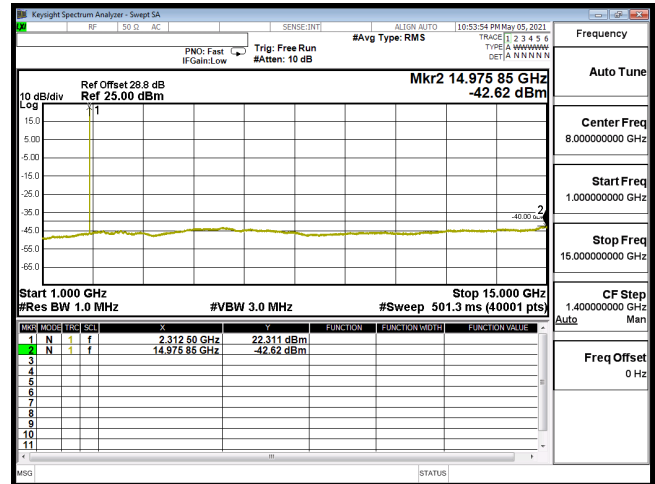
CSE-B30_5M-CH27735-QPSK(1,12)-1G-15G
