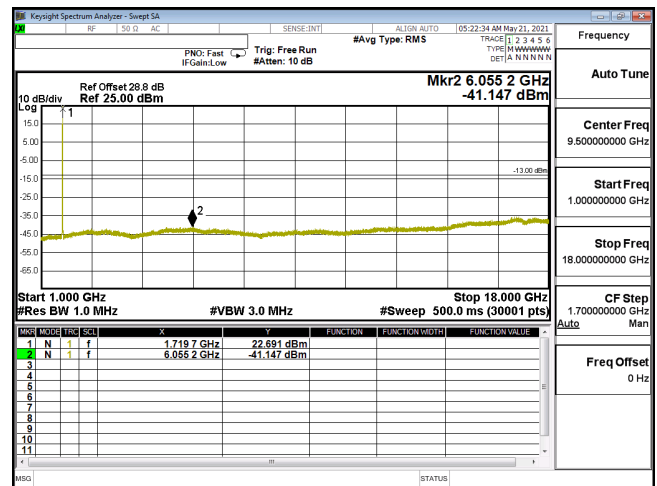
CSE-ENDC_12A_n66_QPSK_20M_CH344000_1720(1,53)-1G-18G
