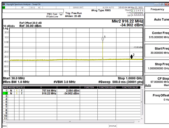
CSE-ENDC_12A_n66_16QAM_10M_CH349000_1745(1,26)-30M-1G
