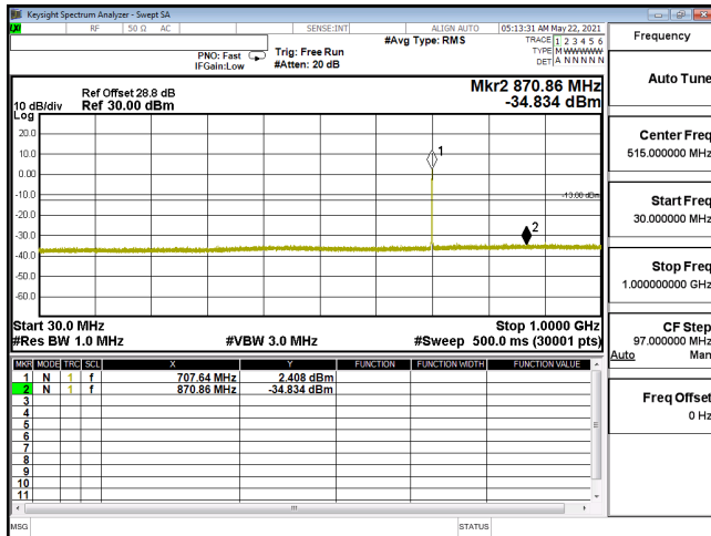
CSE-ENDC_12A_n66_16QAM_15M_CH354500_1772.5(1,39)-30M-1G
