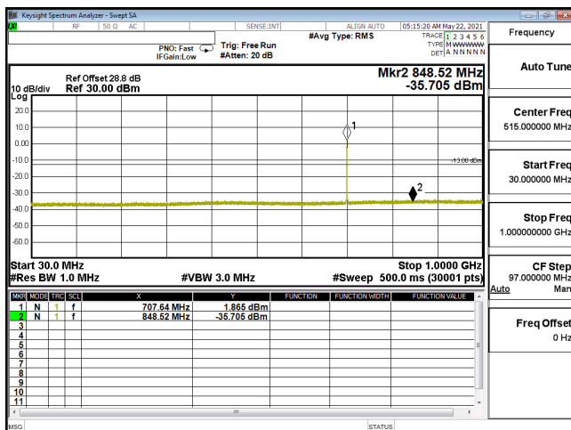
CSE-ENDC_12A_n66_16QAM_20M_CH344000_1720(1,53)-30M-1G
