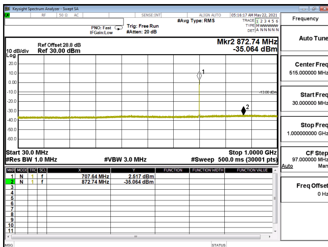
CSE-ENDC_12A_n66_PI2-BPSK_20M_CH349000_1745(1,53)-30M-1G
