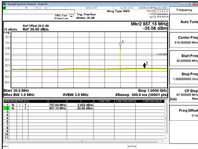
CSE-ENDC_12A_n66_P12-BPSK_10M_CH343000_1715(1,26)-30M-1G
