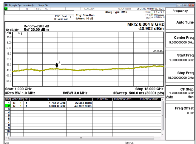
CSE-ENDC_12A_n66_64QAM_20M_CH349000_1745(1,53)-1G-18G
