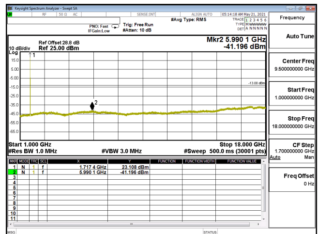
CSE-ENDC_12A_n66_16QAM_15M_CH343500_1717.5(1,39)-1G-18G
