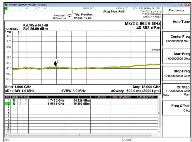
CSE-ENDC_12A_n66_16QAM_15M_CH349000_1745(1,39)-1G-18G
