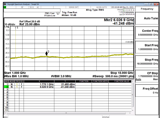
CSE-ENDC_12A_n66_256QAM_20M_CH354000_1770(1,53)-1G-18G
