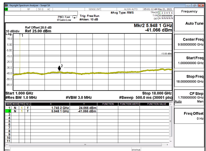
CSE-ENDC_12A_n66_64QAM_10M_CH349000_1745(1,26)-1G-18G
