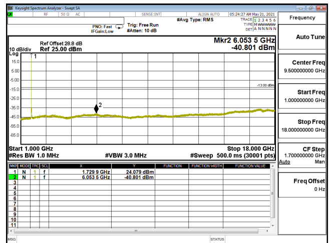
CSE-ENDC_12A_n66_QPSK_40M_CH346000_1730(1,108)-1G-18G
