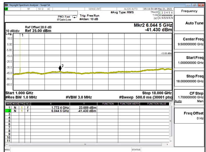
CSE-ENDC_12A_n66_PI2-BPSK_15M_CH354500_1772.5(1,39)-1G-18G
