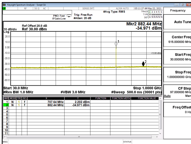
CSE-ENDC_12A_n66_16QAM_15M_CH349000_1745(1,39)-30M-1G
