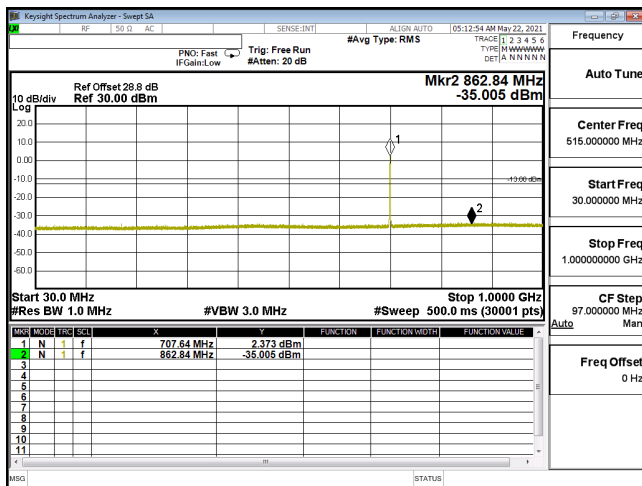
CSE-ENDC_12A_n66_PI2-BPSK_15M_CH354500_1772.5(1,39)-30M-1G
