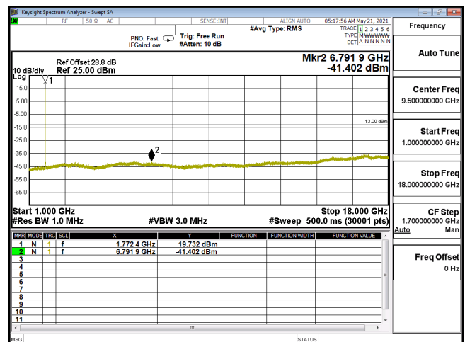
CSE-ENDC_12A_n66_256QAM_15M_CH354500_1772.5(1,39)-1G-18G
