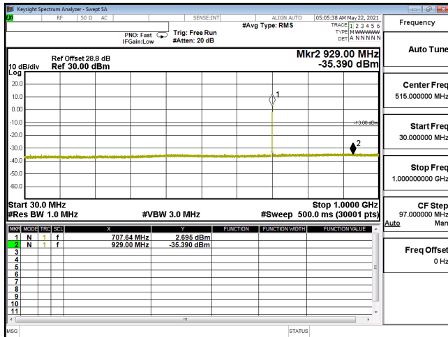
CSE-ENDC_12A_n66_16QAM_10M_CH355000_1775(1,26)-30M-1G
