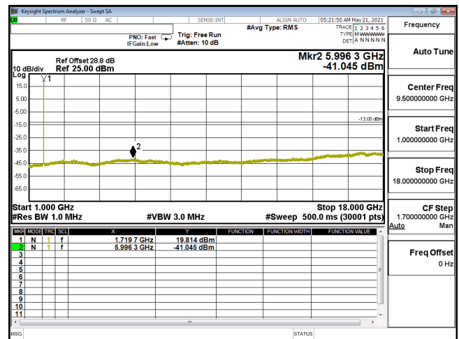
CSE-ENDC_12A_n66_256QAM_20M_CH344000_1720(1,53)-1G-18G
