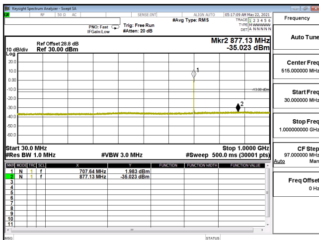
CSE-ENDC_12A_n66_64QAM_20M_CH349000_1745(1,53)-30M-1G
