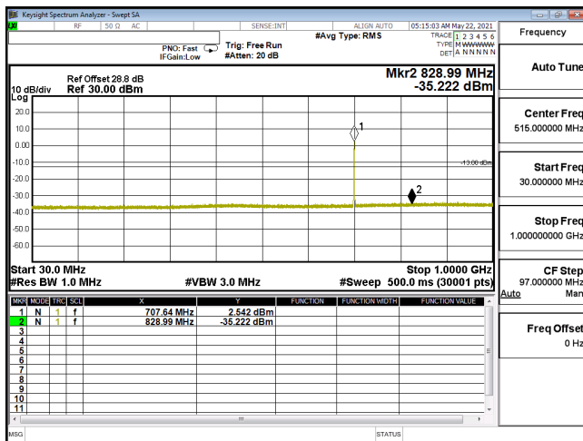
CSE-ENDC_12A_n66_QPSK_20M_CH344000_1720(1,53)-30M-1G
