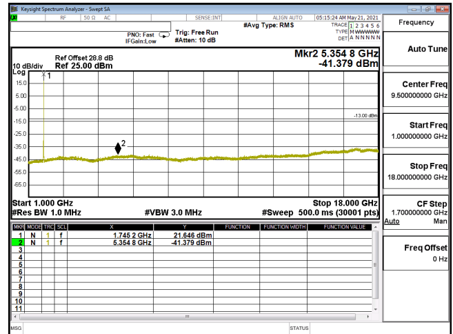
CSE-ENDC_12A_n66_256QAM_15M_CH349000_1745(1,39)-1G-18G
