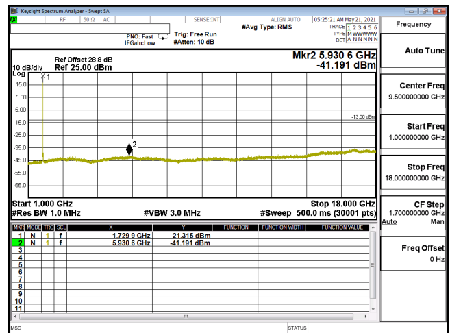
CSE-ENDC_12A_n66_256QAM_40M_CH346000_1730(1,108)-1G-18G
