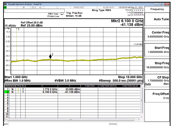
CSE-ENDC_12A_n66_PI2-BPSK_10M_CH355000_1775(1,26)-1G-18G
