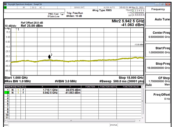
CSE-ENDC_12A_n66_QPSK_10M_CH343000_1715(1,26)-1G-18G
