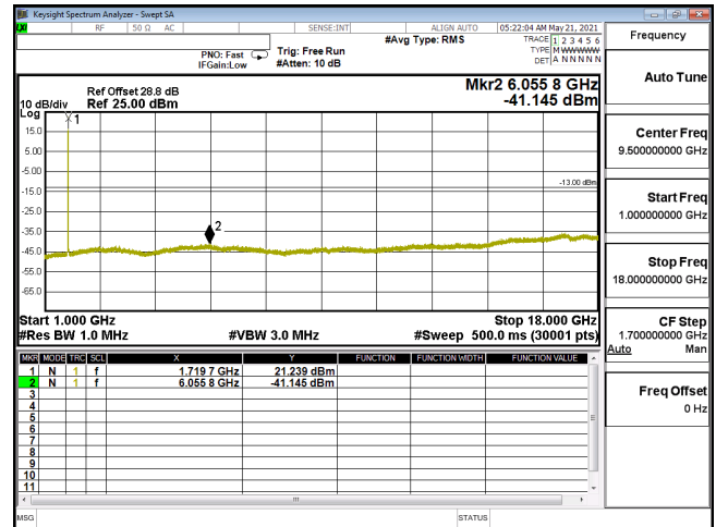
CSE-ENDC_12A_n66_64QAM_20M_CH344000_1720(1,53)-1G-18G
