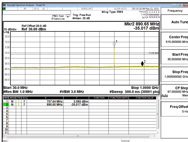
CSE-ENDC_12A_n66_PI2-BPSK_15M_CH349000_1745(1,39)-30M-1G
