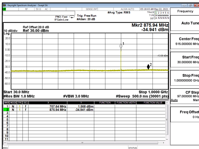
CSE-ENDC_12A_n66_QPSK_20M_CH354000_1770(1,53)-30M-1G
