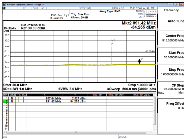
CSE-ENDC_12A_n66_16QAM_40M_CH349000_1745(1,108)-30M-1G
