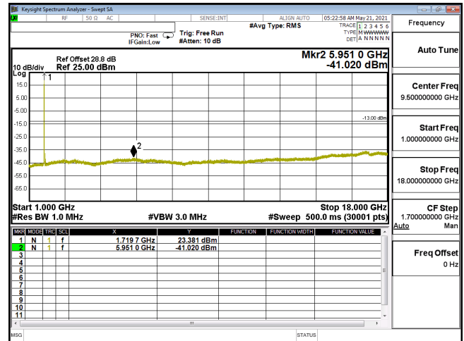
CSE-ENDC_12A_n66_P12-BPSK_20M_CH344000_1720(1,53)-1G-18G
