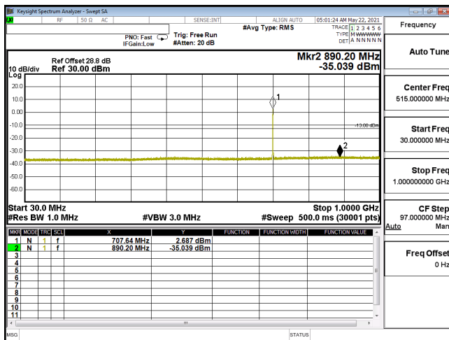
CSE-ENDC_12A_n66_256QAM_10M_CH343000_1715(1,26)-30M-1G
