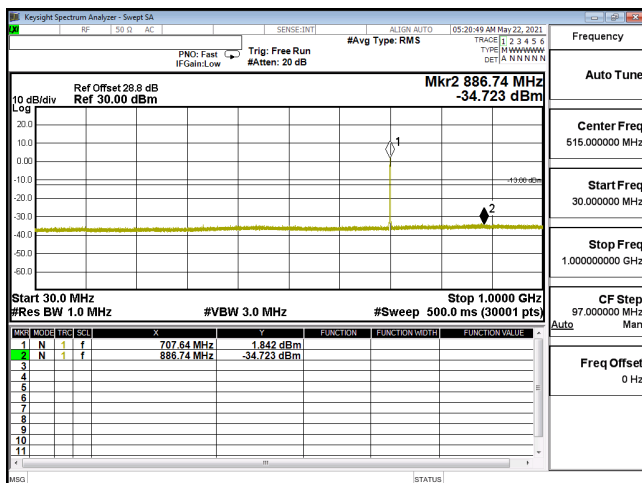
CSE-ENDC_12A_n66_PI2-BPSK_40M_CH349000_1745(1,108)-30M-1G
