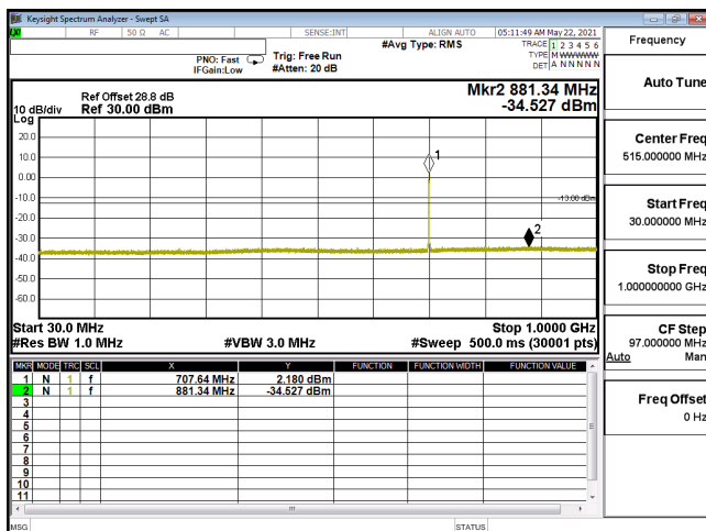
CSE-ENDC_12A_n66_64QAM_15M_CH349000_1745(1,39)-30M-1G
