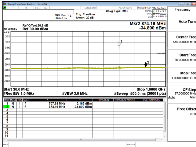
CSE-ENDC_12A_n66_64QAM_10M_CH343000_1715(1,26)-30M-1G
