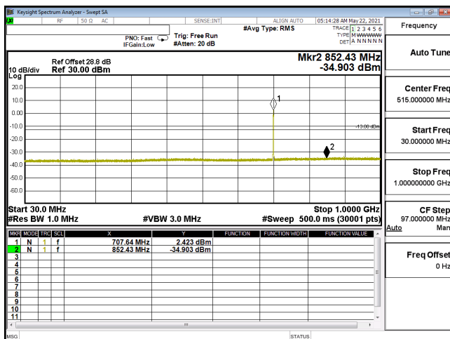
CSE-ENDC_12A_n66_256QAM_15M_CH354500_1772.5(1,39)-30M-1G
