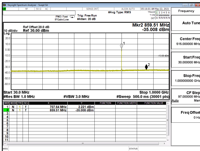
CSE-ENDC_12A_n66_256QAM_20M_CH344000_1720(1,53)-30M-1G
