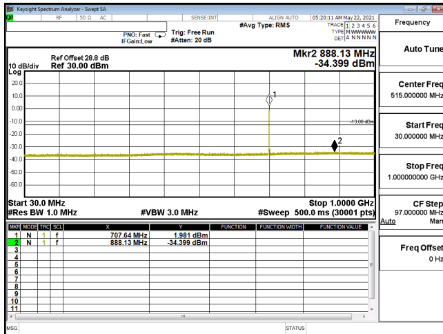
CSE-ENDC_12A_n66_64QAM_40M_CH346000_1730(1,108)-30M-1G
