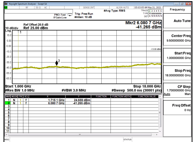
CSE-ENDC_12A_n66_P12-BPSK_10M_CH343000_1715(1,26)-1G-18G
