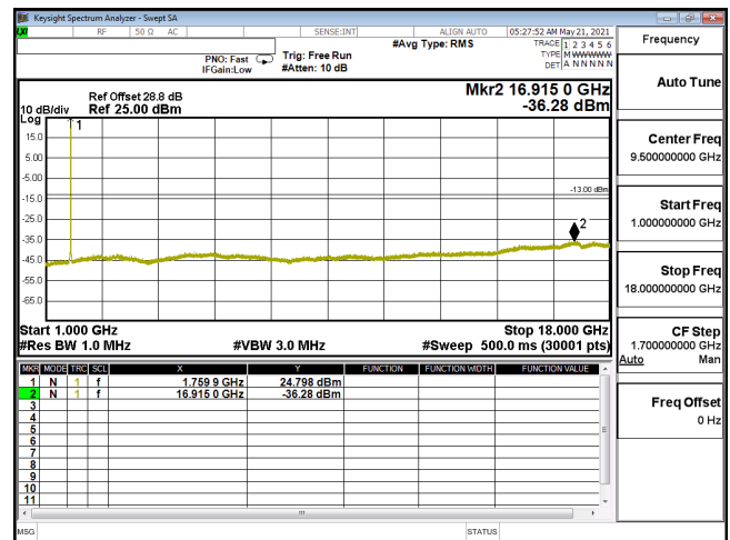
CSE-ENDC_12A_n66_PI2-BPSK_40M_CH352000_1760(1,108)-1G-18G
