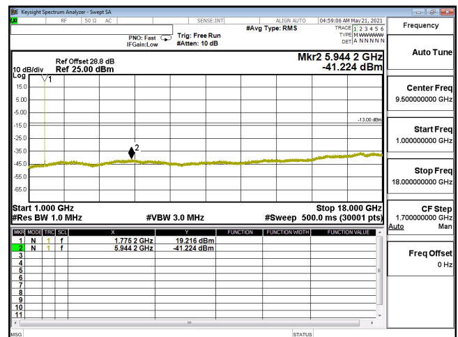
CSE-ENDC_12A_n66_256QAM_10M_CH355000_1775(1,26)-1G-18G
