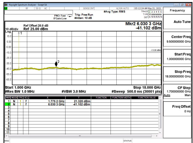
CSE-ENDC_12A_n66_64QAM_10M_CH355000_1775(1,26)-1G-18G
