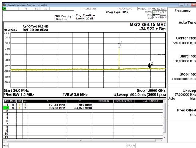
CSE-ENDC_12A_n66_64QAM_20M_CH354000_1770(1,53)-30M-1G
