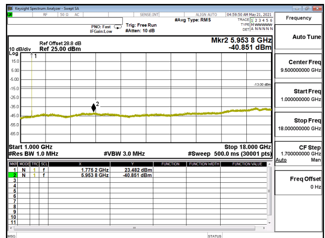
CSE-ENDC_12A_n66_QPSK_10M_CH355000_1775(1,26)-1G-18G
