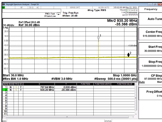
CSE-ENDC_12A_n66_PI2-BPSK_10M_CH349000_1745(1,26)-30M-1G
