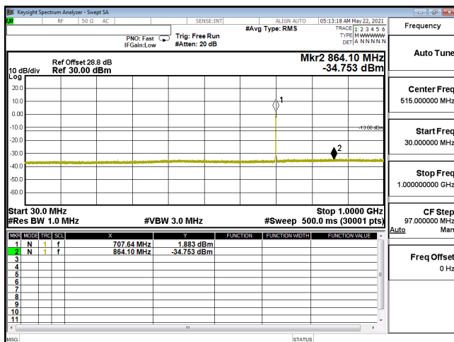
CSE-ENDC_12A_n66_QPSK_15M_CH354500_1772.5(1,39)-30M-1G
