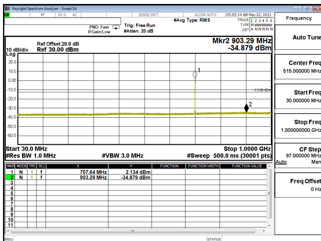
CSE-ENDC_12A_n66_QPSK_10M_CH355000_1775(1,26)-30M-1G
