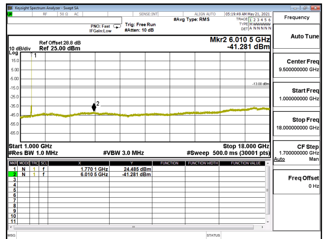
CSE-ENDC_12A_n66_PI2-BPSK_20M_CH354000_1770(1,53)-1G-18G
