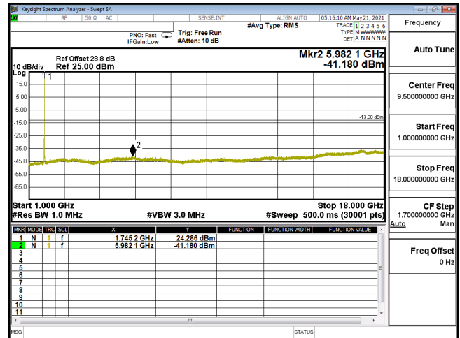
CSE-ENDC_12A_n66_QPSK_15M_CH349000_1745(1,39)-1G-18G
