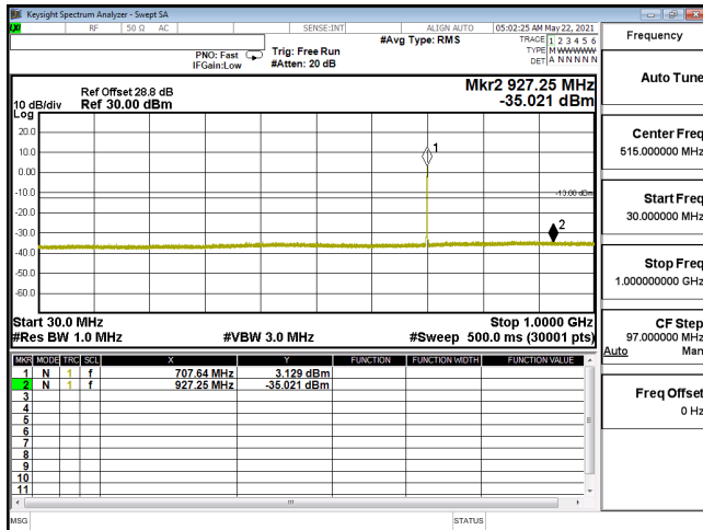
CSE-ENDC_12A_n66_QPSK_10M_CH349000_1745(1,26)-30M-1G
