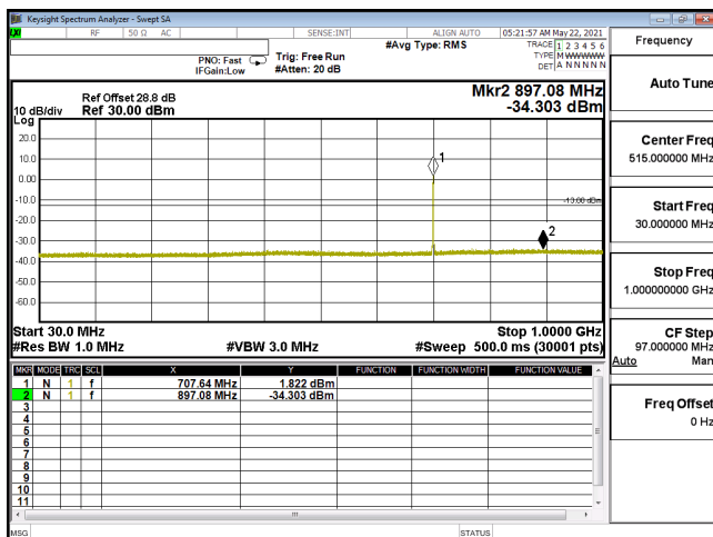
CSE-ENDC_12A_n66_64QAM_40M_CH349000_1745(1,108)-30M-1G
