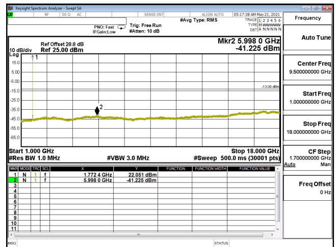
CSE-ENDC_12A_n66_64QAM_15M_CH354500_1772.5(1,39)-1G-18G
