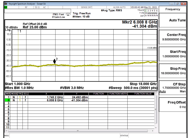
CSE-ENDC_12A_n66_QPSK_10M_CH349000_1745(1,26)-1G-18G
