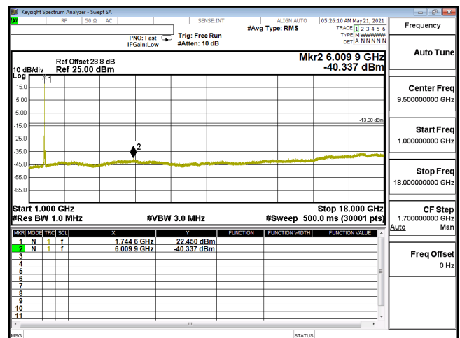
CSE-ENDC_12A_n66_64QAM_40M_CH349000_1745(1,108)-1G-18G
