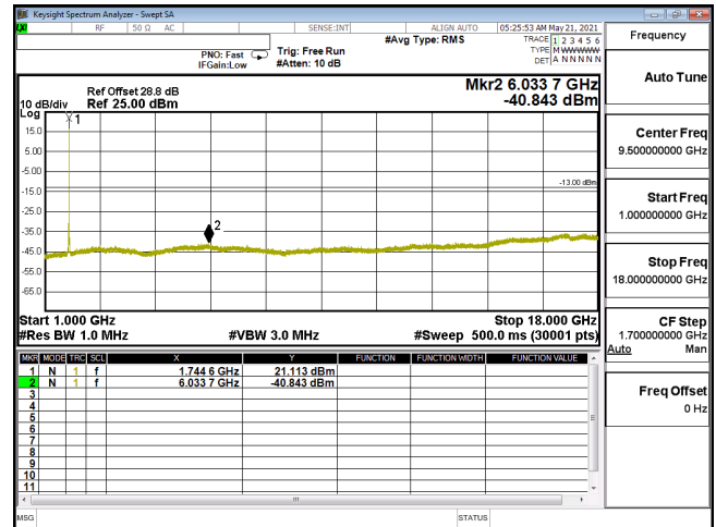
CSE-ENDC_12A_n66_256QAM_40M_CH349000_1745(1,108)-1G-18G
