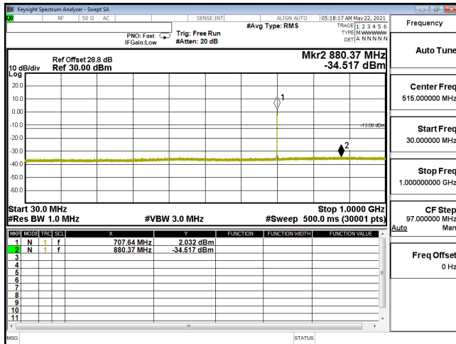
CSE-ENDC_12A_n66_16QAM_20M_CH354000_1770(1,53)-30M-1G
