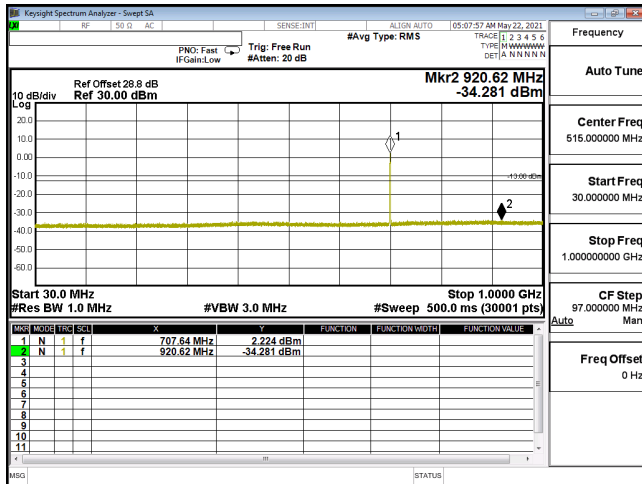
CSE-ENDC_12A_n66_P12-BPSK_15M_CH343500_1717.5(1,39)-30M-1G
