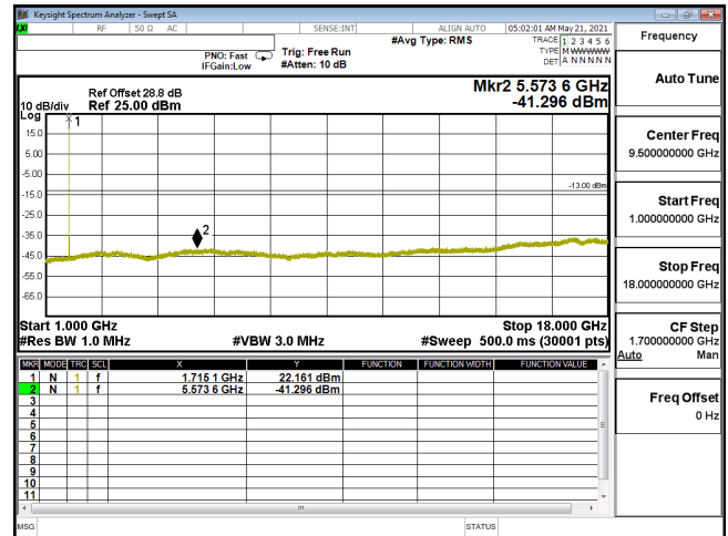
CSE-ENDC_12A_n66_64QAM_10M_CH343000_1715(1,26)-1G-18G
