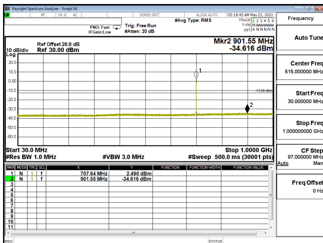
CSE-ENDC_12A_n66_256QAM_20M_CH354000_1770(1,53)-30M-1G
