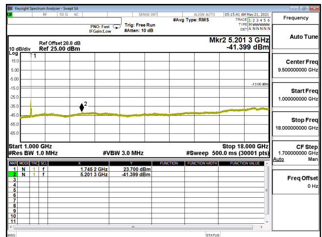
CSE-ENDC_12A_n66_64QAM_15M_CH349000_1745(1,39)-1G-18G
