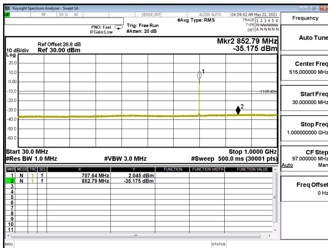
CSE-ENDC_12A_n66_QPSK_10M_CH343000_1715(1,26)-30M-1G
