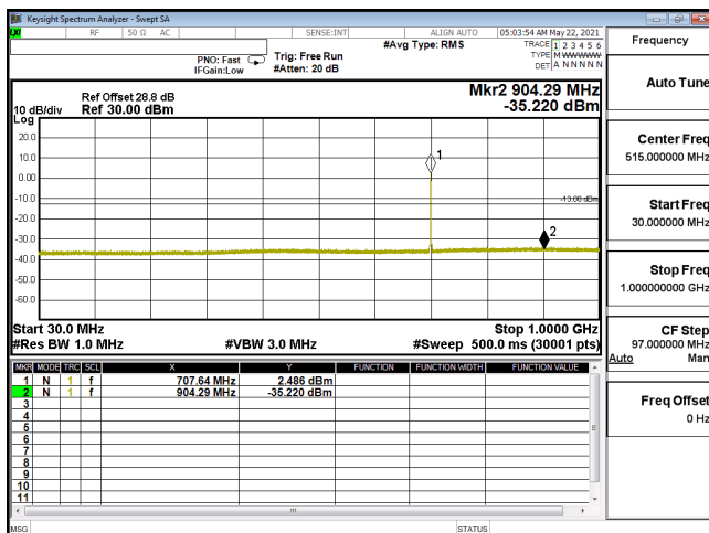
CSE-ENDC_12A_n66_64QAM_10M_CH349000_1745(1,26)-30M-1G
