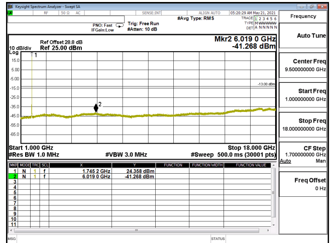
CSE-ENDC_12A_n66_QPSK_20M_CH349000_1745(1,53)-1G-18G
