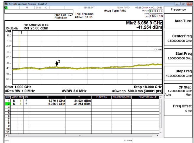
CSE-ENDC_12A_n66_16QAM_20M_CH354000_1770(1,53)-1G-18G
