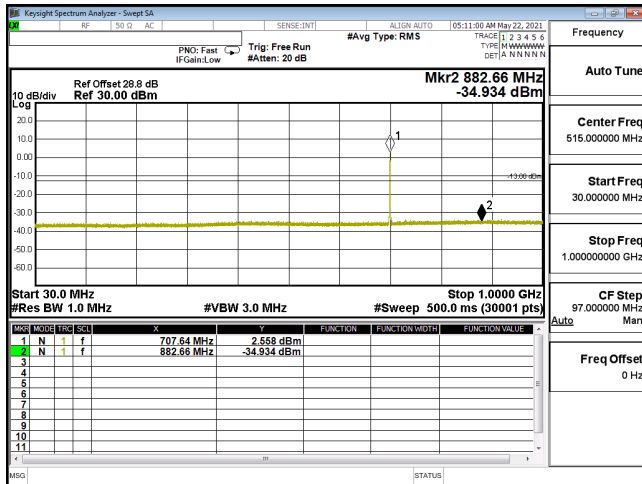
CSE-ENDC_12A_n66_QPSK_15M_CH349000_1745(1,39)-30M-1G
