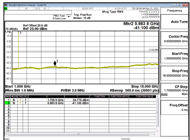
CSE-ENDC_12A_n66_QPSK_40M_CH352000_1760(1,108)-1G-18G
