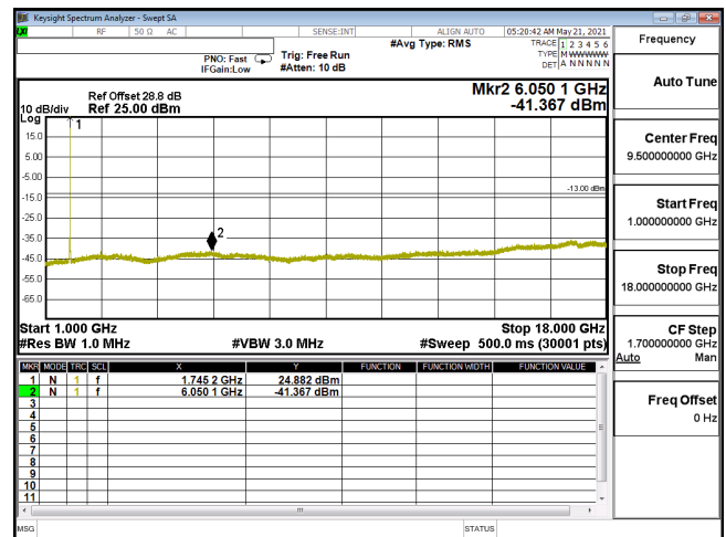
CSE-ENDC_12A_n66_16QAM_20M_CH349000_1745(1,53)-1G-18G
