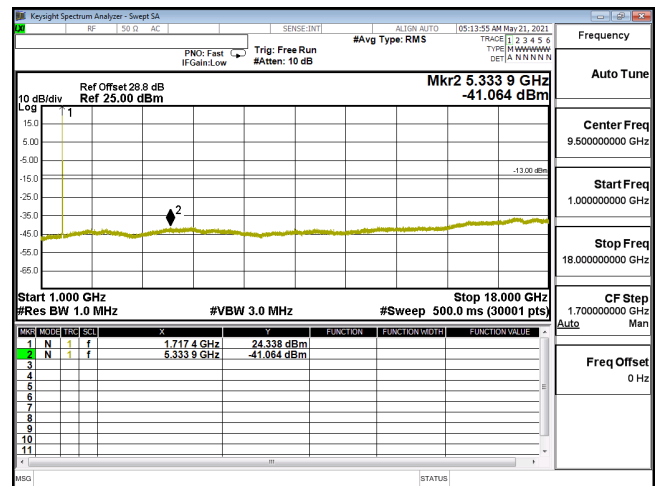
CSE-ENDC_12A_n66_QPSK_15M_CH343500_1717.5(1,39)-1G-18G
