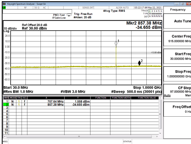
CSE-ENDC_12A_n66_256QAM_40M_CH349000_1745(1,108)-30M-1G
