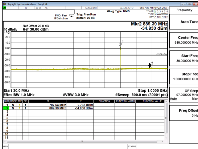
CSE-ENDC_12A_n66_256QAM_20M_CH349000_1745(1,53)-30M-1G
