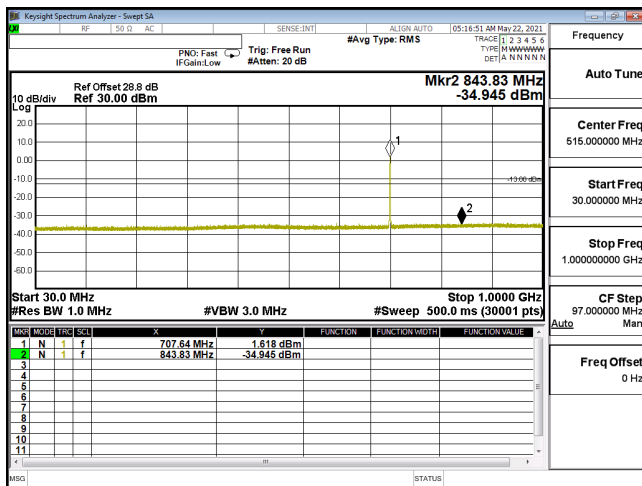
CSE-ENDC_12A_n66_16QAM_20M_CH349000_1745(1,53)-30M-1G
