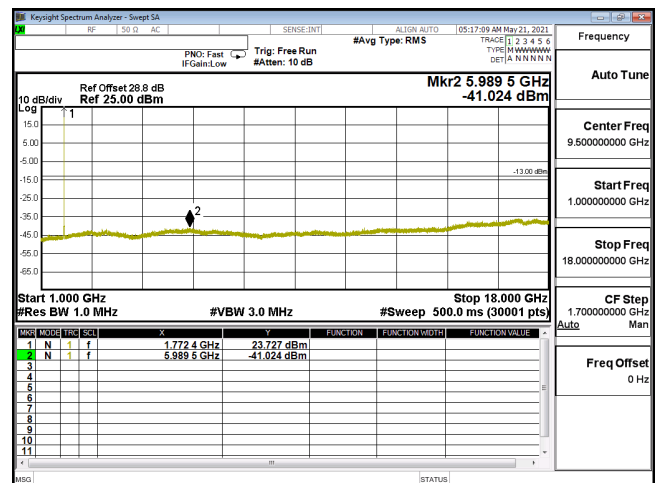
CSE-ENDC_12A_n66_QPSK_15M_CH354500_1772.5(1,39)-1G-18G
