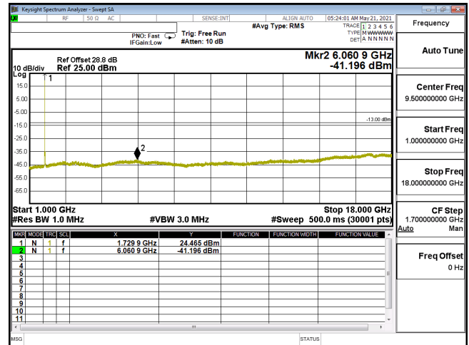
CSE-ENDC_12A_n66_P12-BPSK_40M_CH346000_1730(1,108)-1G-18G
