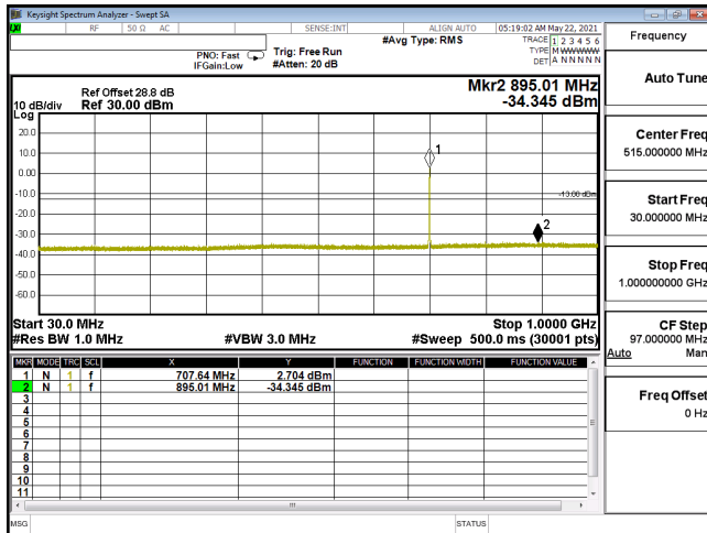
CSE-ENDC_12A_n66_P12-BPSK_40M_CH346000_1730(1,108)-30M-1G
