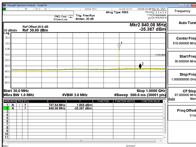
CSE-ENDC_12A_n66_16QAM_10M_CH343000_1715(1,26)-30M-1G
