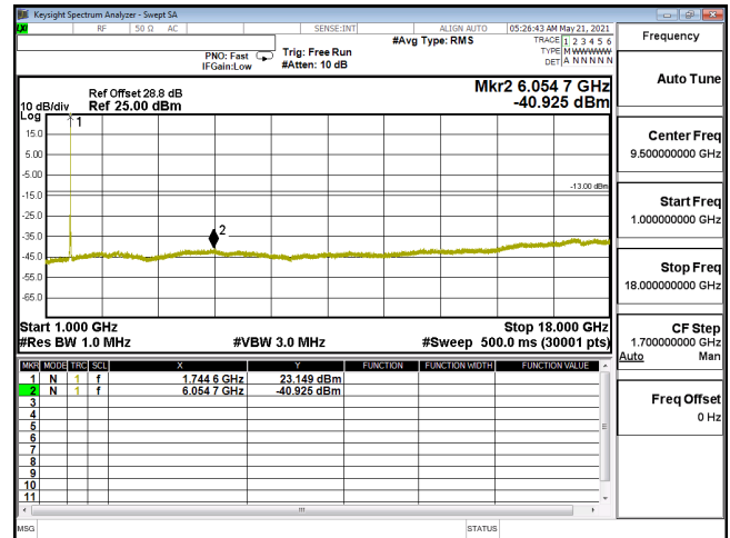
CSE-ENDC_12A_n66_QPSK_40M_CH349000_1745(1,108)-1G-18G
