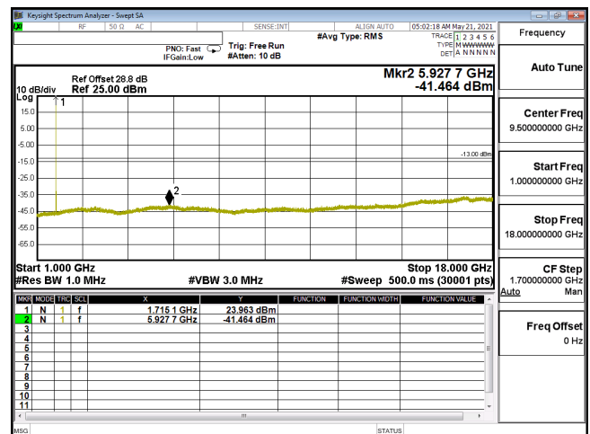
CSE-ENDC_12A_n66_16QAM_10M_CH343000_1715(1,26)-1G-18G
