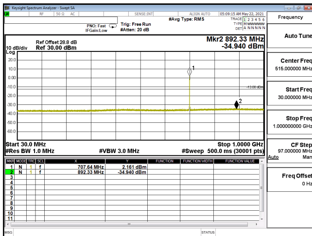
CSE-ENDC_12A_n66_QPSK_15M_CH343500_1717.5(1,39)-30M-1G
