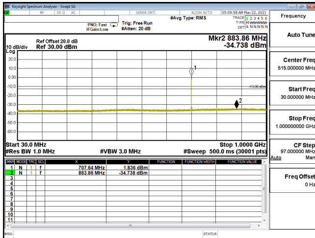
CSE-ENDC_12A_n66_64QAM_15M_CH343500_1717.5(1,39)-30M-1G
