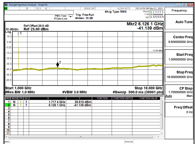
CSE-ENDC_12A_n66_256QAM_15M_CH343500_1717.5(1,39)-1G-18G
