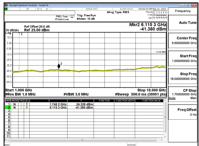
CSE-ENDC_12A_n66_PI2-BPSK_10M_CH349000_1745(1,26)-1G-18G
