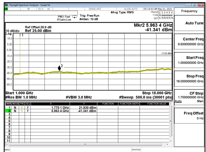
CSE-ENDC_12A_n66_64QAM_20M_CH354000_1770(1,53)-1G-18G
