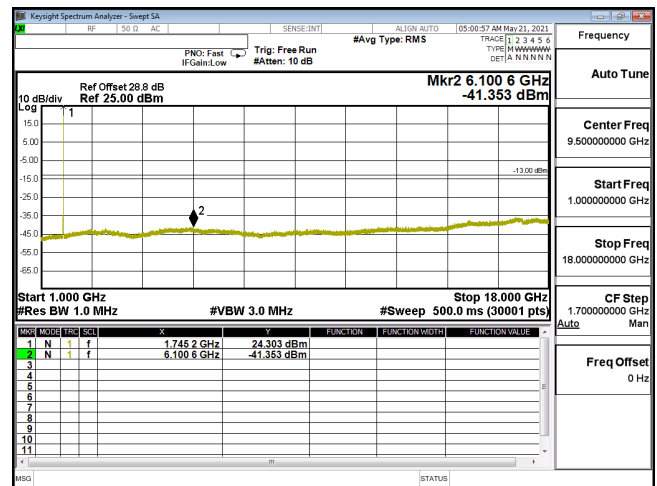
CSE-ENDC_12A_n66_16QAM_10M_CH349000_1745(1,26)-1G-18G
