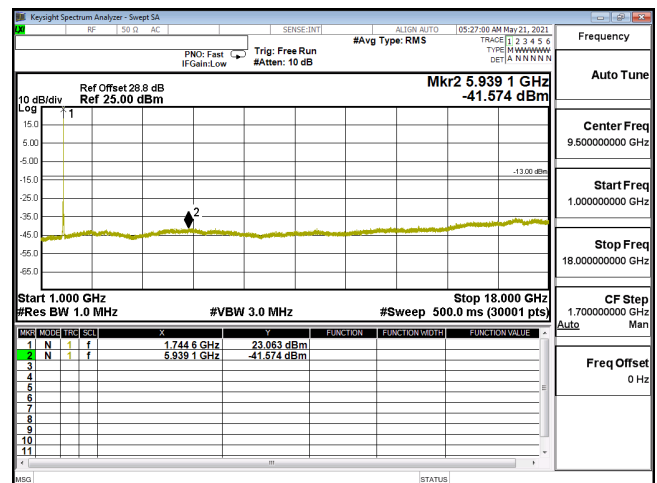
CSE-ENDC_12A_n66_PI2-BPSK_40M_CH349000_1745(1,108)-1G-18G
