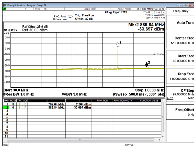
CSE-ENDC_12A_n66_16QAM_40M_CH346000_1730(1,108)-30M-1G
