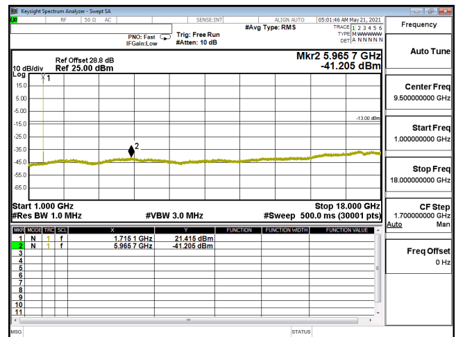
CSE-ENDC_12A_n66_256QAM_10M_CH343000_1715(1,26)-1G-18G
