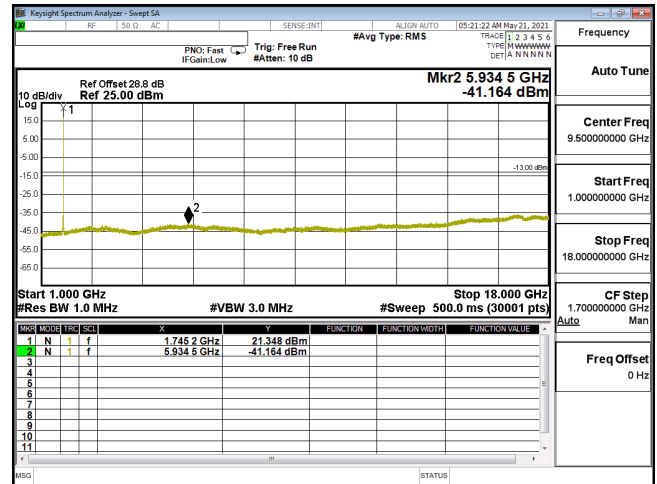
CSE-ENDC_12A_n66_256QAM_20M_CH349000_1745(1,53)-1G-18G
