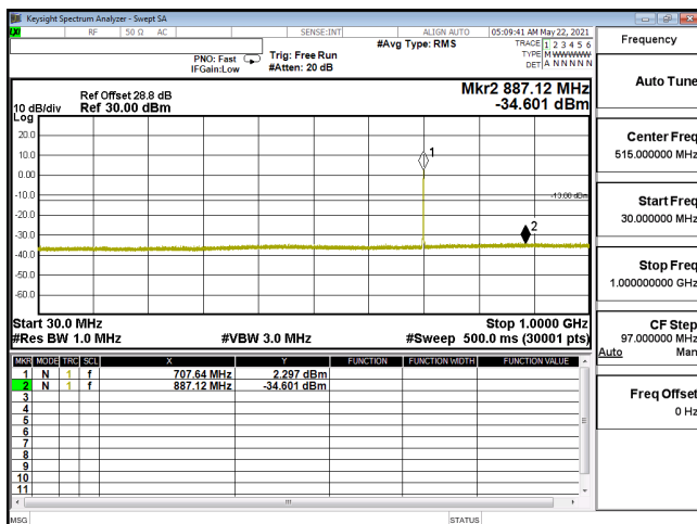
CSE-ENDC_12A_n66_16QAM_15M_CH343500_1717.5(1,39)-30M-1G
