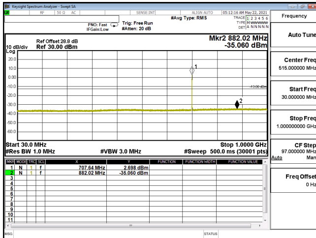
CSE-ENDC_12A_n66_256QAM_15M_CH349000_1745(1,39)-30M-1G
