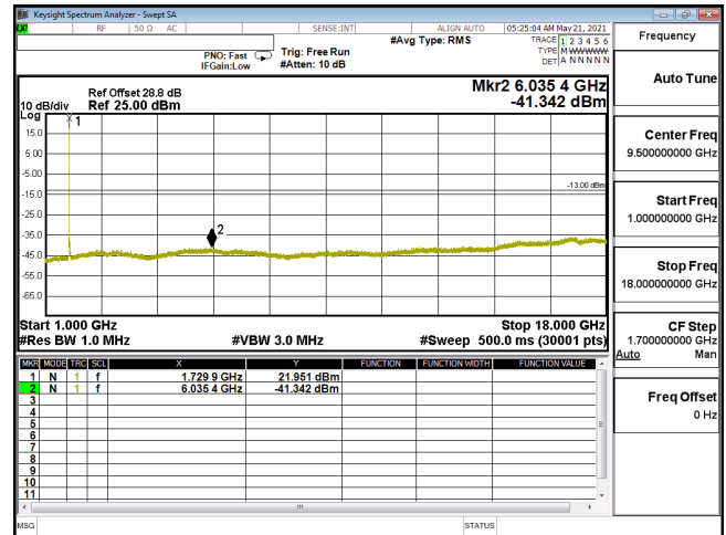
CSE-ENDC_12A_n66_64QAM_40M_CH346000_1730(1,108)-1G-18G
