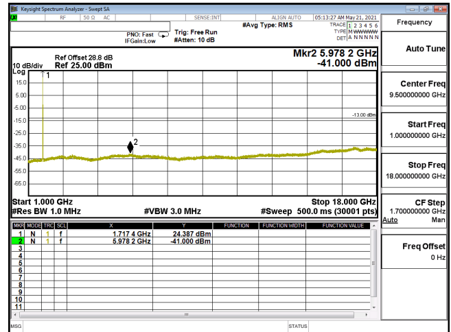
CSE-ENDC_12A_n66_P12-BPSK_15M_CH343500_1717.5(1,39)-1G-18G
