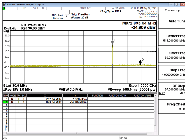
CSE-ENDC_12A_n66_QPSK_40M_CH346000_1730(1,108)-30M-1G
