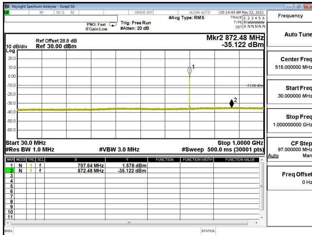
CSE-ENDC_12A_n66_P12-BPSK_20M_CH344000_1720(1,53)-30M-1G
