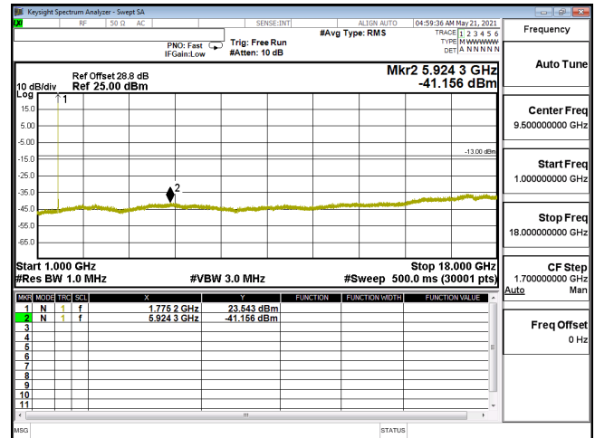
CSE-ENDC_12A_n66_16QAM_10M_CH355000_1775(1,26)-1G-18G
