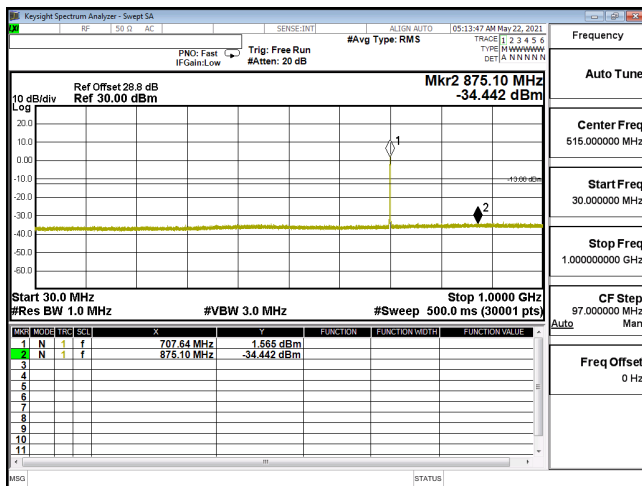
CSE-ENDC_12A_n66_64QAM_15M_CH354500_1772.5(1,39)-30M-1G
