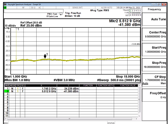
CSE-ENDC_12A_n66_PI2-BPSK_20M_CH349000_1745(1,53)-1G-18G
