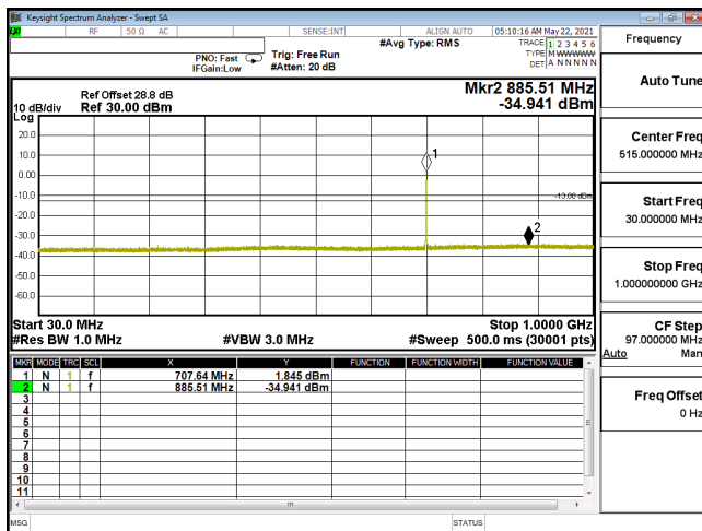
CSE-ENDC_12A_n66_256QAM_15M_CH343500_1717.5(1,39)-30M-1G
