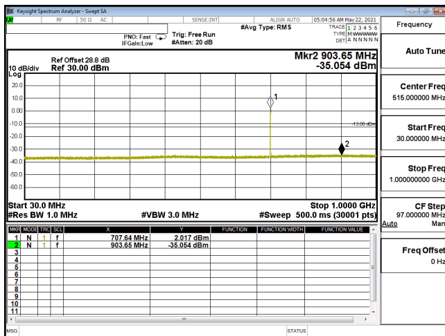
CSE-ENDC_12A_n66_PI2-BPSK_10M_CH355000_1775(1,26)-30M-1G
