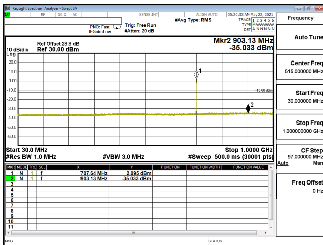
CSE-ENDC_12A_n66_256QAM_40M_CH346000_1730(1,108)-30M-1G
