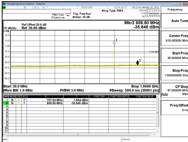
CSE-ENDC_12A_n66_64QAM_20M_CH344000_1720(1,53)-30M-1G
