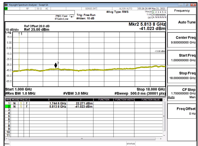
CSE-ENDC_12A_n66_16QAM_40M_CH349000_1745(1,108)-1G-18G
