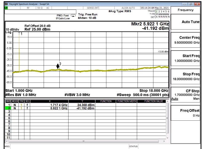
CSE-ENDC_12A_n66_64QAM_15M_CH343500_1717.5(1,39)-1G-18G
