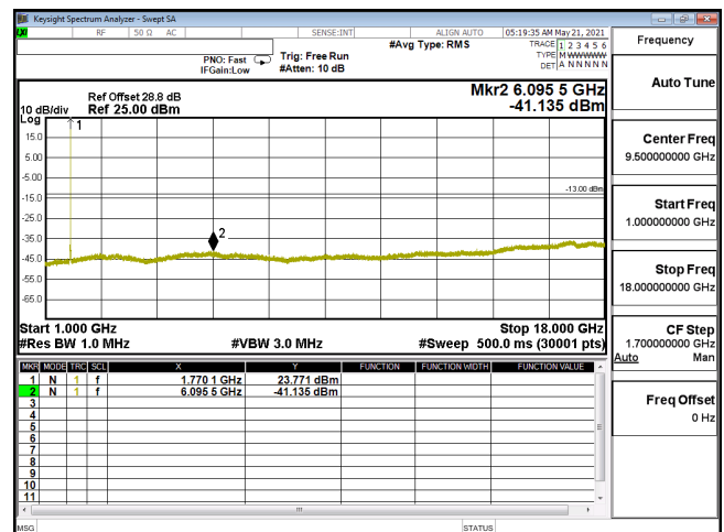
CSE-ENDC_12A_n66_QPSK_20M_CH354000_1770(1,53)-1G-18G
