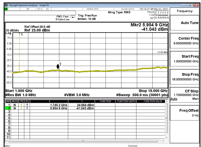
CSE-ENDC_12A_n66_PI2-BPSK_15M_CH349000_1745(1,39)-1G-18G
