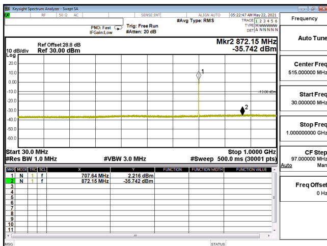
CSE-ENDC_12A_n66_QPSK_40M_CH352000_1760(1,108)-30M-1G
