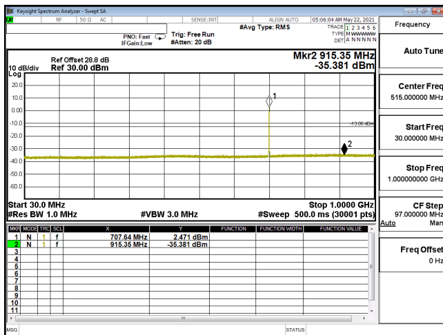
CSE-ENDC_12A_n66_64QAM_10M_CH355000_1775(1,26)-30M-1G
