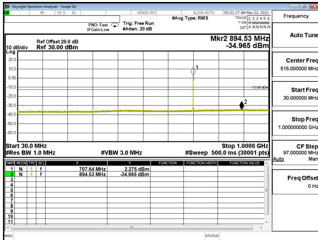
CSE-ENDC_12A_n66_QPSK_40M_CH349000_1745(1,108)-30M-1G
