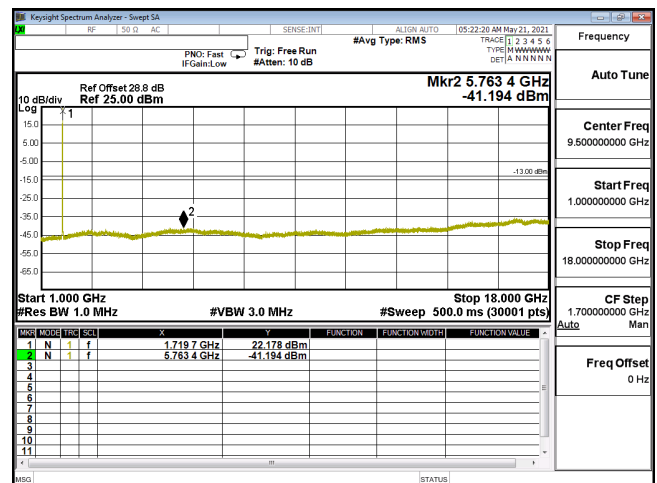
CSE-ENDC_12A_n66_16QAM_20M_CH344000_1720(1,53)-1G-18G
