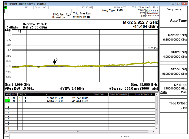
CSE-ENDC_12A_n66_256QAM_10M_CH349000_1745(1,26)-1G-18G
