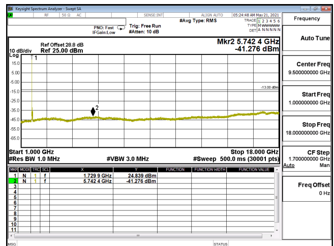
CSE-ENDC_12A_n66_16QAM_40M_CH346000_1730(1,108)-1G-18G
