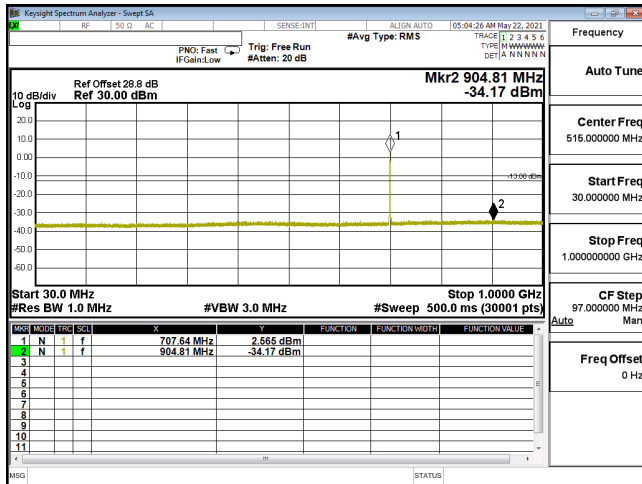
CSE-ENDC_12A_n66_256QAM_10M_CH349000_1745(1,26)-30M-1G
