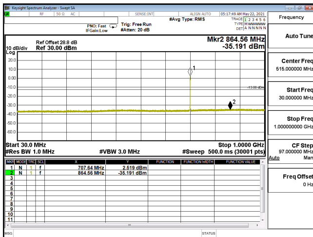
CSE-ENDC_12A_n66_PI2-BPSK_20M_CH354000_1770(1,53)-30M-1G
