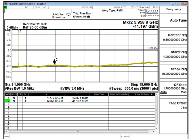
CSE-ENDC_12A_n66_16QAM_15M_CH354500_1772.5(1,39)-1G-18G
