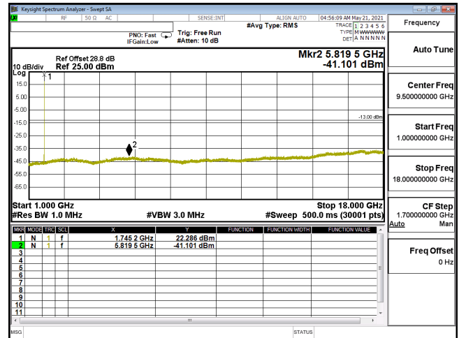
CSE-ENDC_12A_n66_256QAM_5M_CH349000_1745(1,12)-1G-18G
