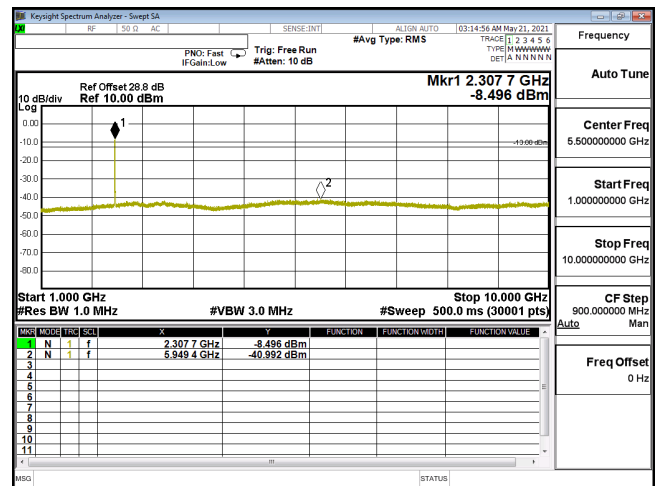
CSE-ENDC_30A_n5-16QAM_15M_CH167300_836.5(1,39)-1G-10G
