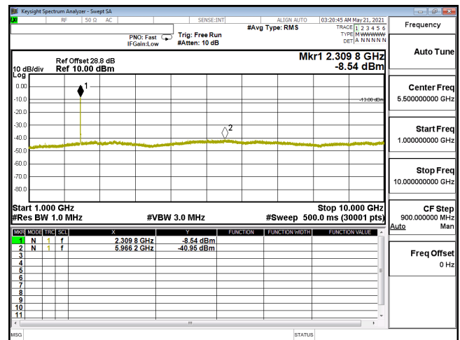
CSE-ENDC_30A_n5-256QAM_20M_CH166800_834(1,53)-1G-10G
