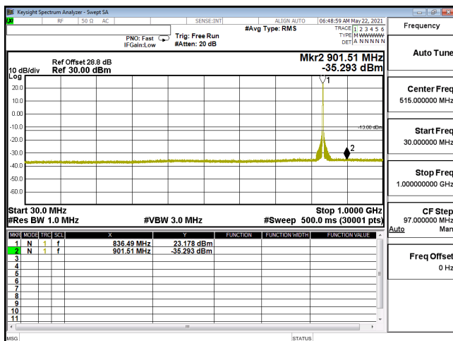
CSE-ENDC_30A_n5-64QAM_20M_CH167300_836.5(1,53)-30M-1G
