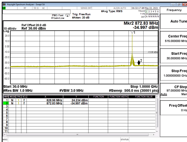
CSE-ENDC_30A_n5-64QAM_10M_CH165800_829(1,26)-30M-1G
