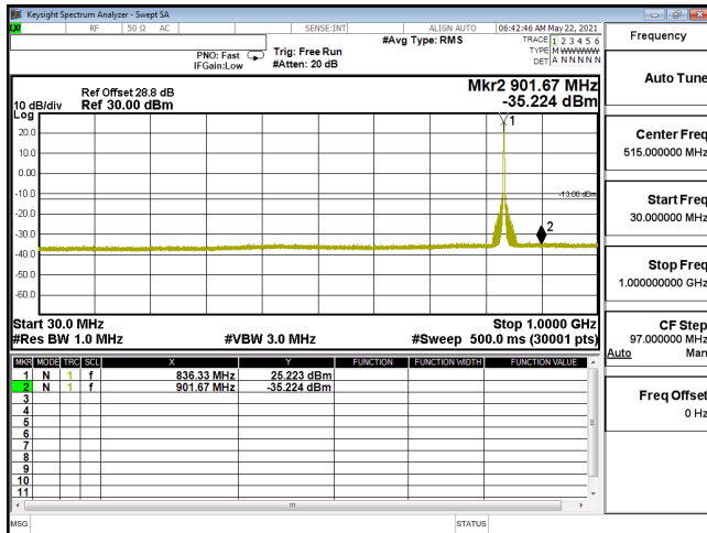
CSE-ENDC_30A_n5-QPSK_15M_CH167300_836.5(1,39)-30M-1G
