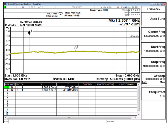
CSE-ENDC_30A_n5-256QAM_15M_CH166300_831.5(1,39)-1G-10G
