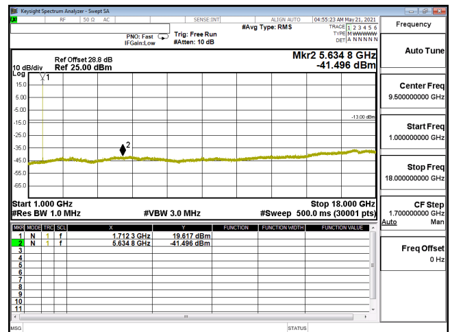
CSE-ENDC_12A_n66_256QAM_5M_CH342500_1712.5(1,12)-1G-18G
