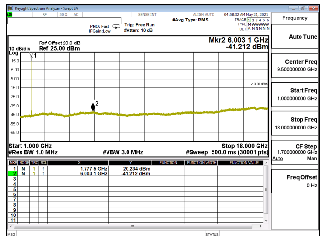
CSE-ENDC_12A_n66_256QAM_5M_CH355500_1777.5(1,12)-1G-18G
