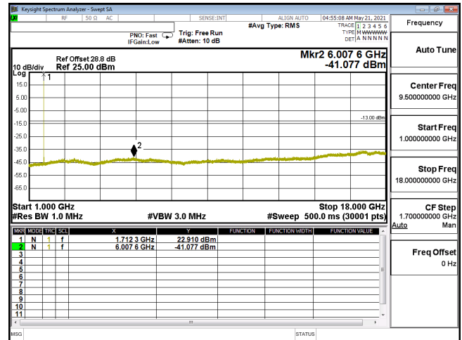
CSE-ENDC_12A_n66_64QAM_5M_CH342500_1712.5(1,12)-1G-18G
