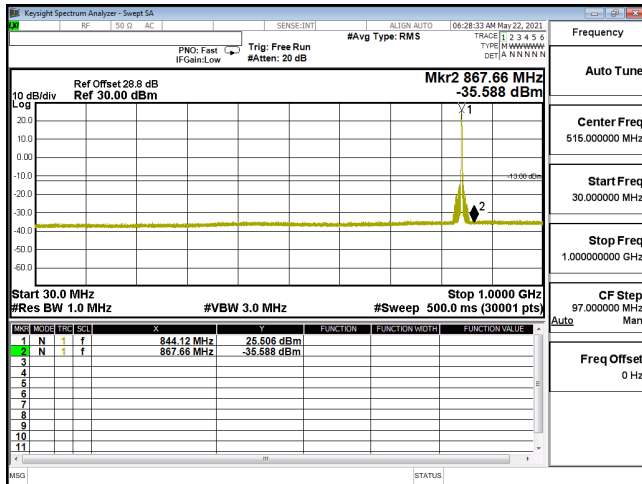
CSE-ENDC_30A_n5-16QAM_10M_CH168800_844(1,26)-30M-1G
