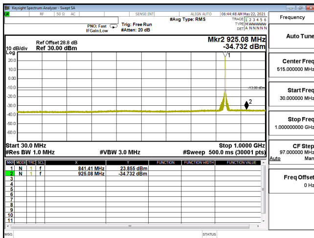
CSE-ENDC_30A_n5-64QAM_15M_CH168300_841.5(1,39)-30M-1G
