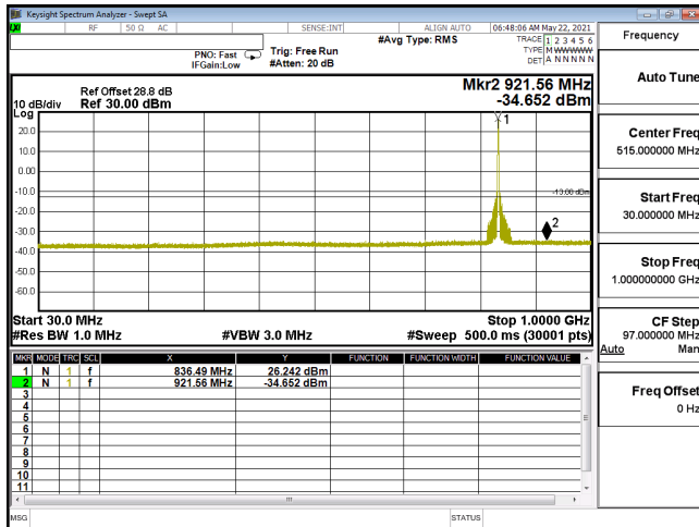
CSE-ENDC_30A_n5-QPSK_20M_CH167300_836.5(1,53)-30M-1G
