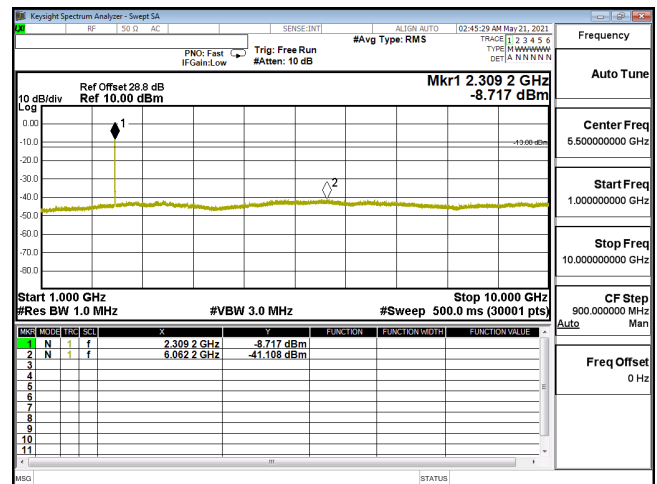
CSE-ENDC_30A_n5-16QAM_10M_CH167300_836.5(1,26)-1G-10G
