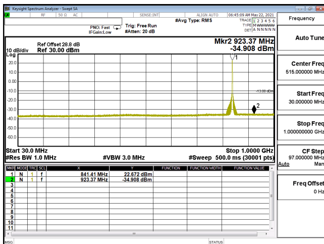
CSE-ENDC_30A_n5-256QAM_15M_CH168300_841.5(1,39)-30M-1G
