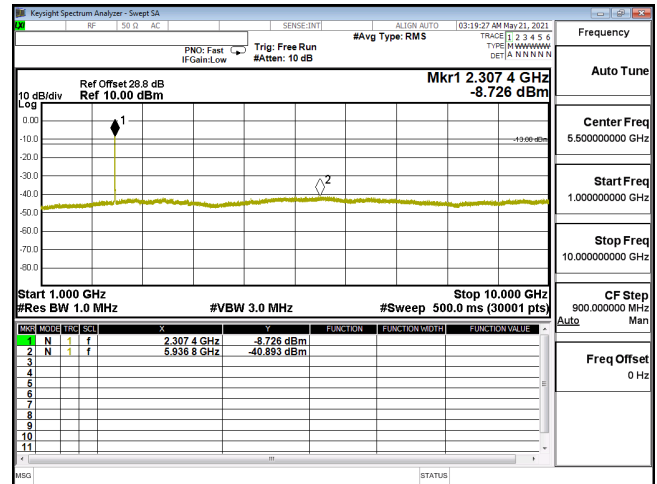
CSE-ENDC_30A_n5-QPSK_20M_CH167300_836.5(1,53)-1G-10G
