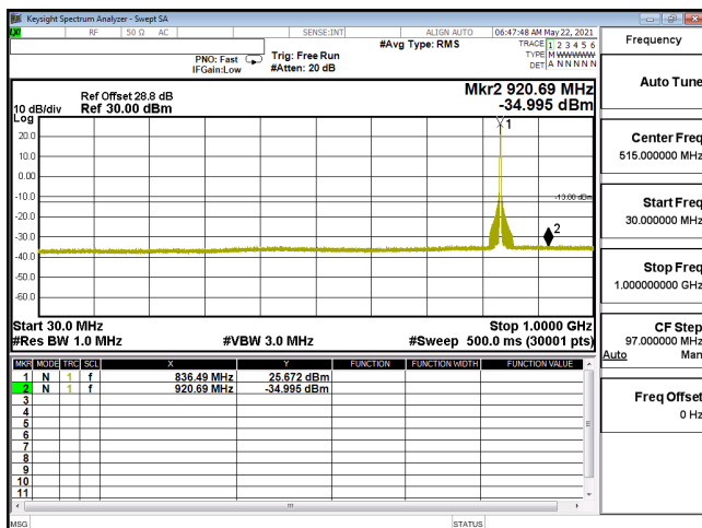
CSE-ENDC_30A_n5-PI2-BPSK_20M_CH167300_836.5(1,53)-30M-1G
