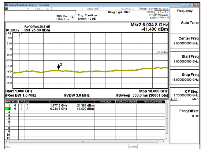
CSE-ENDC_12A_n66_64QAM_5M_CH355500_1777.5(1,12)-1G-18G
