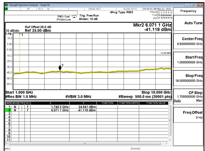
CSE-ENDC_12A_n66_16QAM_5M_CH349000_1745(1,12)-1G-18G
