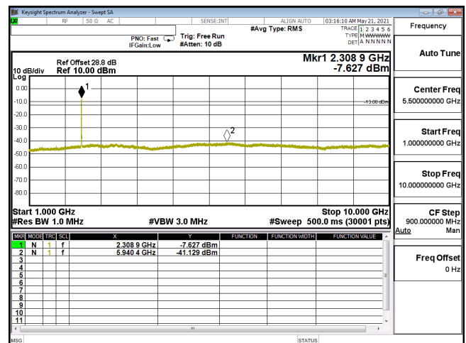
CSE-ENDC_30A_n5-QPSK_15M_CH168300_841.5(1,39)-1G-10G
