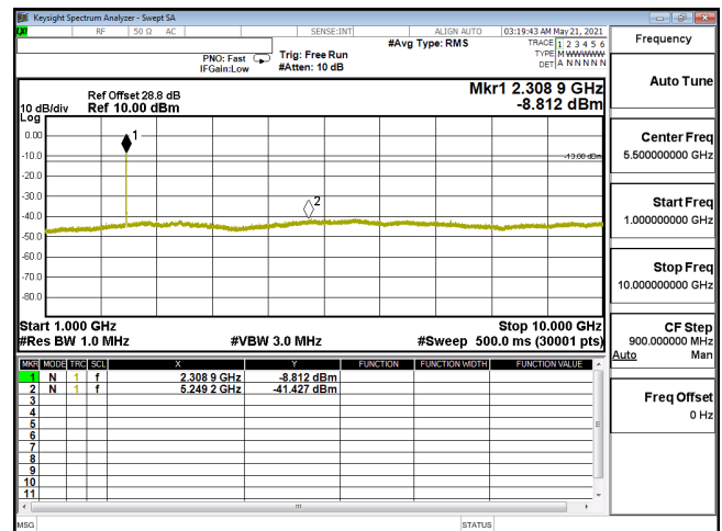
CSE-ENDC_30A_n5-16QAM_20M_CH167300_836.5(1,53)-1G-10G
