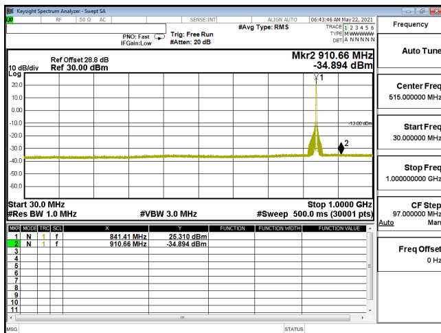
CSE-ENDC_30A_n5-PI2-BPSK_15M_CH168300_841.5(1,39)-30M-1G
