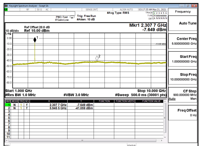
CSE-ENDC_30A_n5-256QAM_20M_CH167800_839(1,53)-1G-10G
