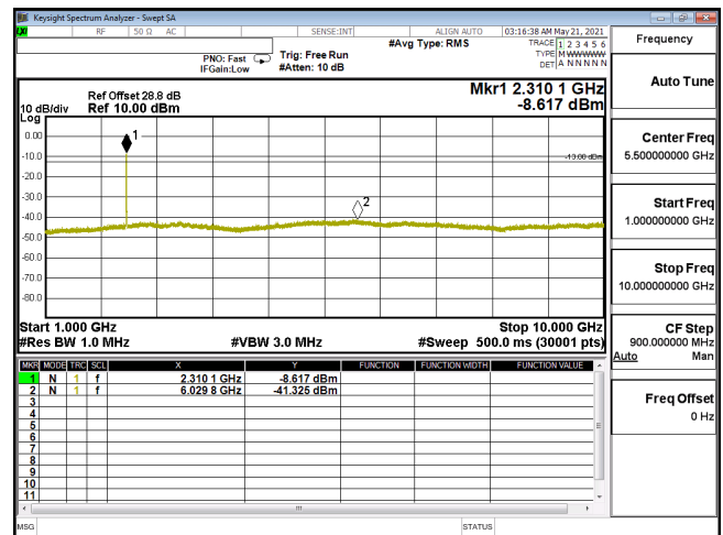
CSE-ENDC_30A_n5-64QAM_15M_CH168300_841.5(1,39)-1G-10G
