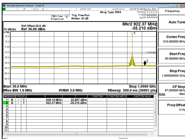
CSE-ENDC_30A_n5-256QAM_20M_CH167800_839(1,53)-30M-1G
