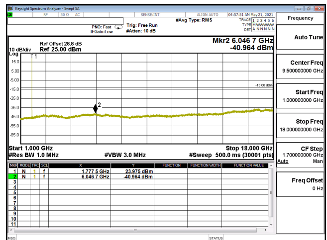
CSE-ENDC_12A_n66_QPSK_5M_CH355500_1777.5(1,12)-1G-18G
