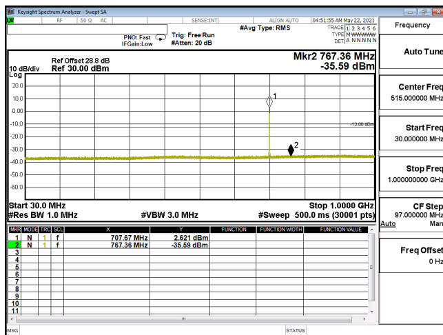
CSE-ENDC_12A_n66_QPSK_5M_CH342500_1712.5(1,12)-30M-1G
