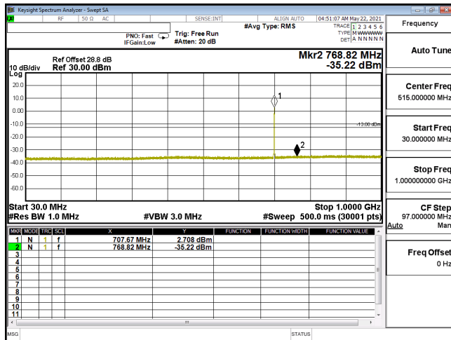
CSE-ENDC_12A_n66_PI2-BPSK_5M_CH342500_1712.5(1,12)-30M-1G
