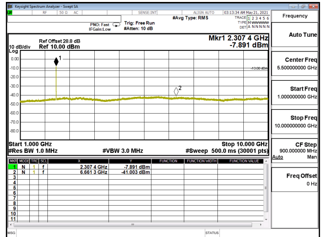
CSE-ENDC_30A_n5-64QAM_15M_CH166300_831.5(1,39)-1G-10G
