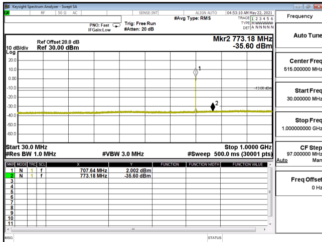
CSE-ENDC_12A_n66_64QAM_5M_CH342500_1712.5(1,12)-30M-1G
