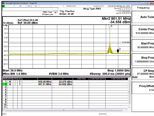
CSE-ENDC_30A_n5-256QAM_20M_CH167300_836.5(1,53)-30M-1G
