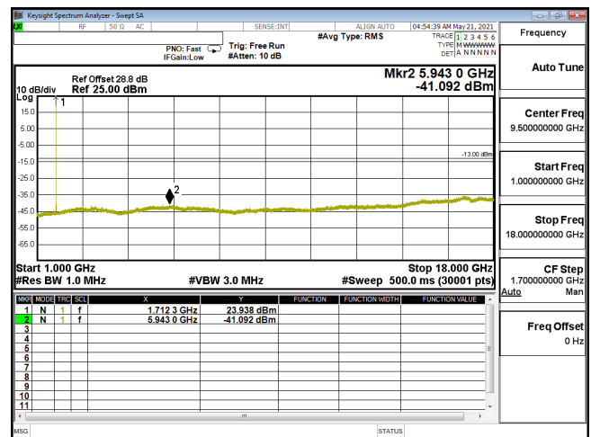
CSE-ENDC_12A_n66_QPSK_5M_CH342500_1712.5(1,12)-1G-18G
