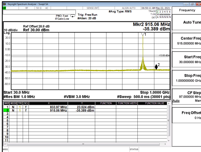
CSE-ENDC_30A_n5-64QAM_20M_CH166800_834(1,53)-30M-1G
