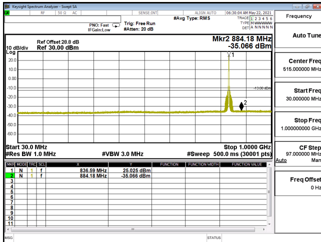
CSE-ENDC_30A_n5-QPSK_10M_CH167300_836.5(1,26)-30M-1G
