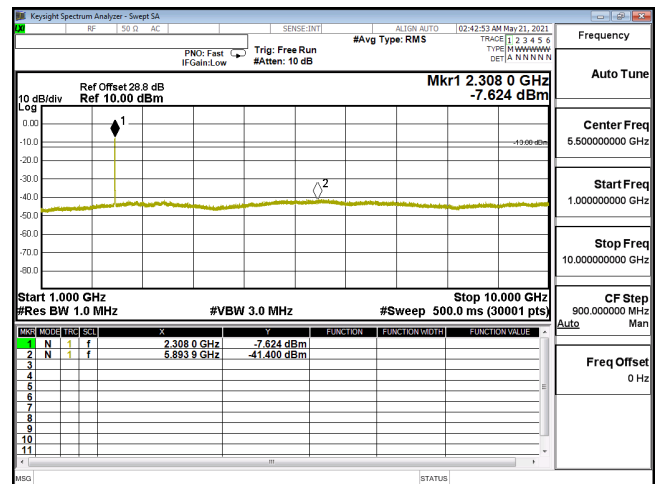
CSE-ENDC_30A_n5-64QAM_10M_CH168800_844(1,26)-1G-10G
