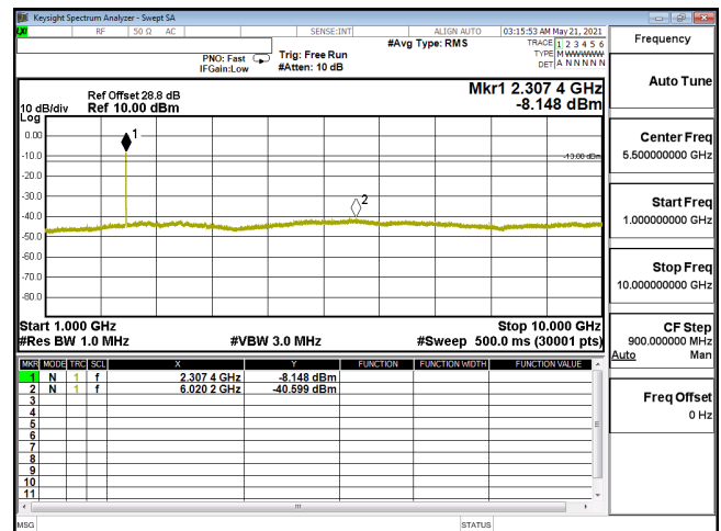
CSE-ENDC_30A_n5-PI2-BPSK_15M_CH168300_841.5(1,39)-1G-10G
