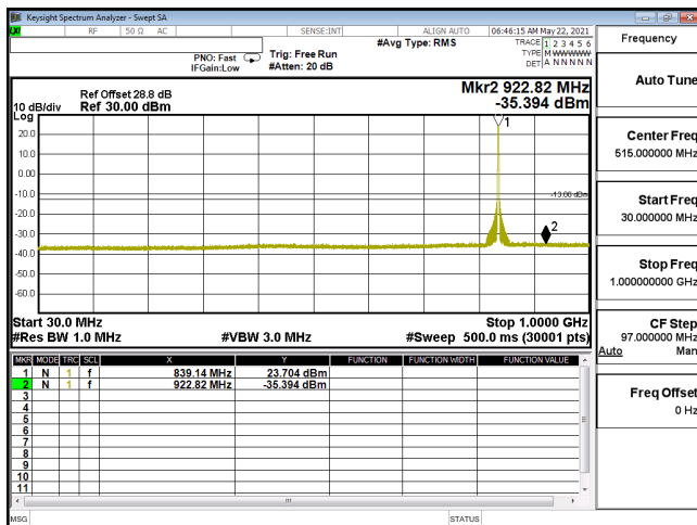
CSE-ENDC_30A_n5-64QAM_20M_CH167800_839(1,53)-30M-1G
