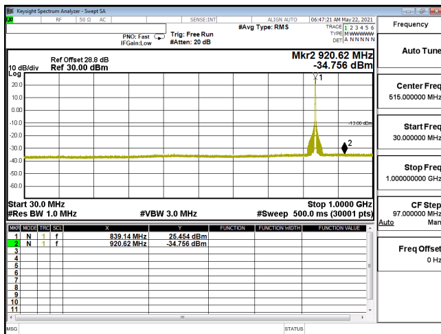
CSE-ENDC_30A_n5-PI2-BPSK_20M_CH167800_839(1,53)-30M-1G
