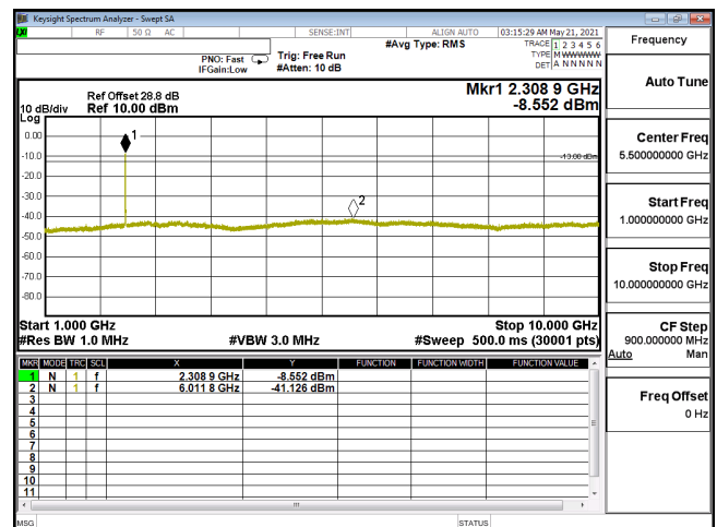
CSE-ENDC_30A_n5-PI2-BPSK_15M_CH167300_836.5(1,39)-1G-10G
