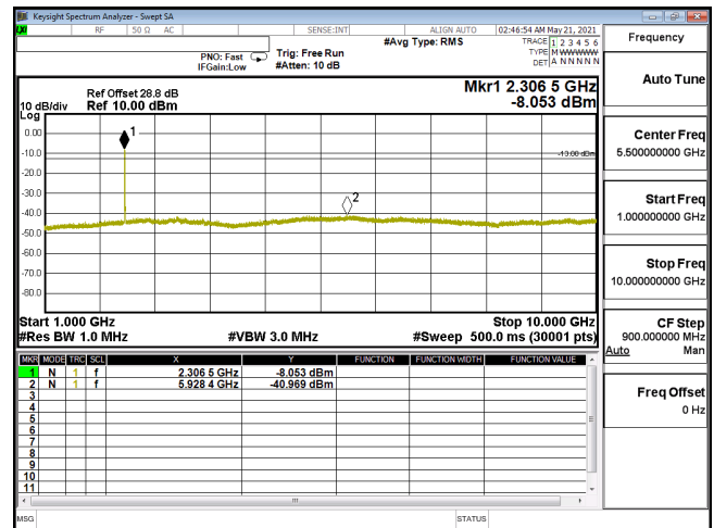
CSE-ENDC_30A_n5-64QAM_10M_CH165800_829(1,26)-1G-10G
