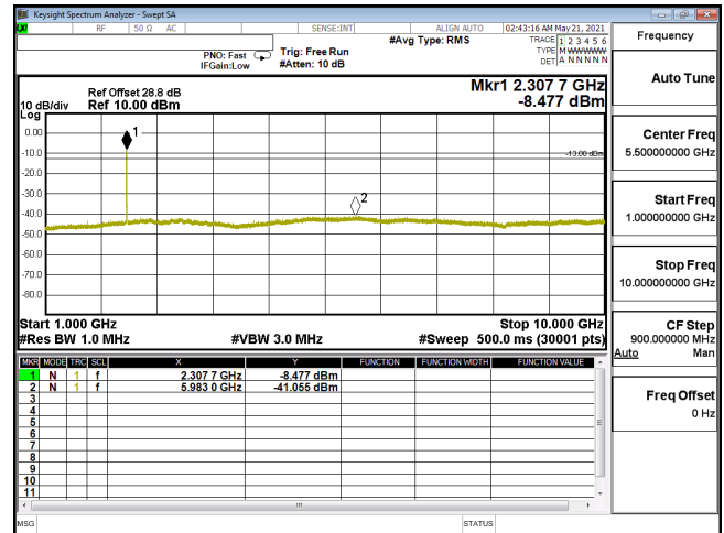
CSE-ENDC_30A_n5-16QAM_10M_CH168800_844(1,26)-1G-10G
