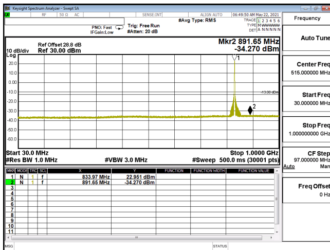
CSE-ENDC_30A_n5-256QAM_20M_CH166800_834(1,53)-30M-1G
