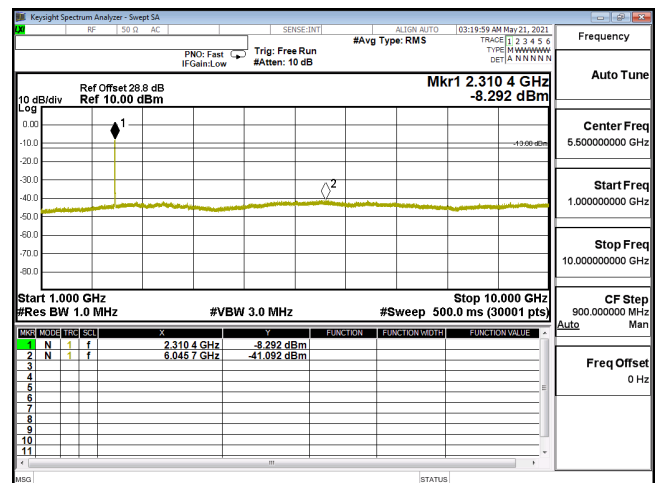
CSE-ENDC_30A_n5-64QAM_20M_CH167300_836.5(1,53)-1G-10G
