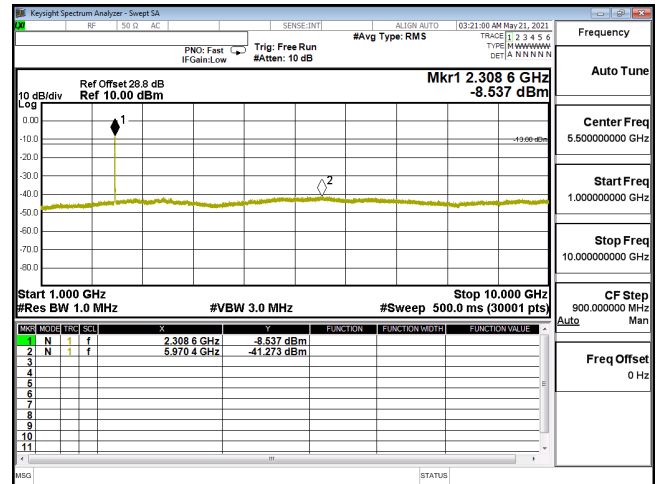
CSE-ENDC_30A_n5-64QAM_20M_CH166800_834(1,53)-1G-10G
