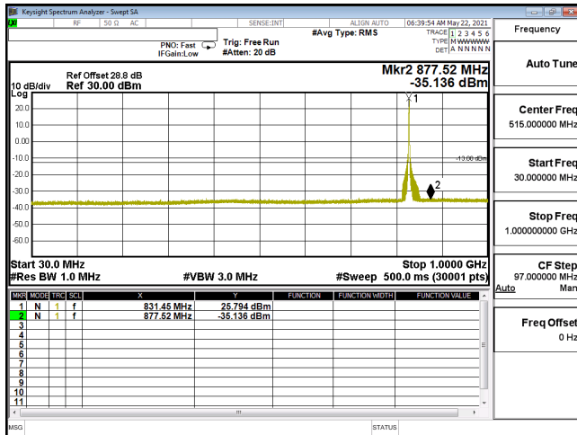
CSE-ENDC_30A_n5-PI2-BPSK_15M_CH166300_831.5(1,39)-30M-1G
