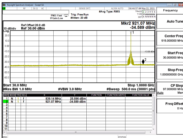
CSE-ENDC_30A_n5-QPSK_20M_CH167800_839(1,53)-30M-1G
