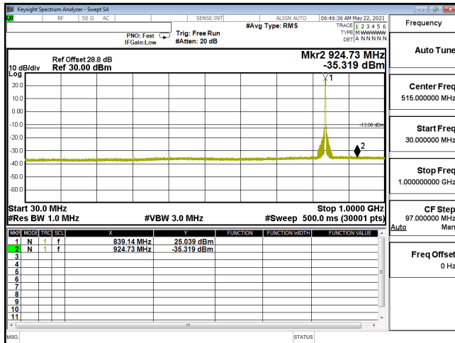
CSE-ENDC_30A_n5-16QAM_20M_CH167800_839(1,53)-30M-1G
