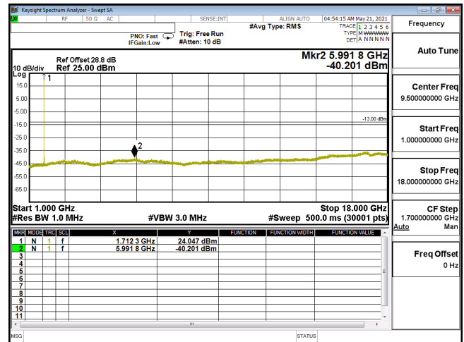
CSE-ENDC_12A_n66_PI2-BPSK_5M_CH342500_1712.5(1,12)-1G-18G
