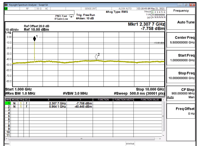
CSE-ENDC_30A_n5-PI2-BPSK_20M_CH167800_839(1,53)-1G-10G
