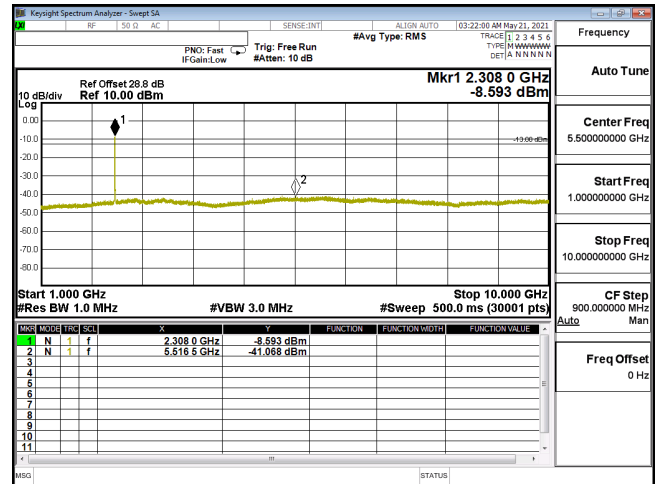
CSE-ENDC_30A_n5-PI2-BPSK_20M_CH166800_834(1,53)-1G-10G
