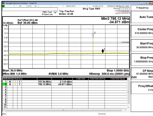
CSE-ENDC_12A_n66_QPSK_5M_CH349000_1745(1,12)-30M-1G
