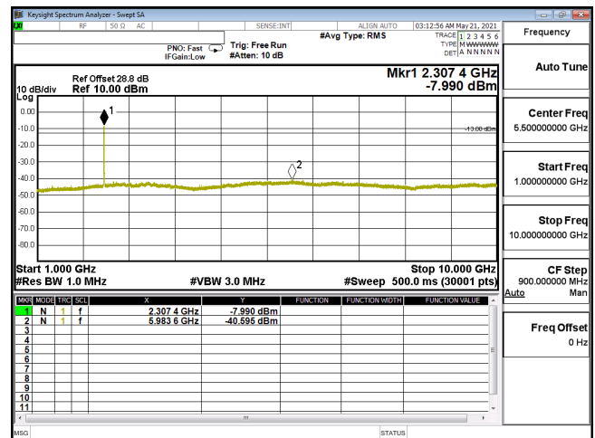
CSE-ENDC_30A_n5-QPSK_15M_CH166300_831.5(1,39)-1G-10G
