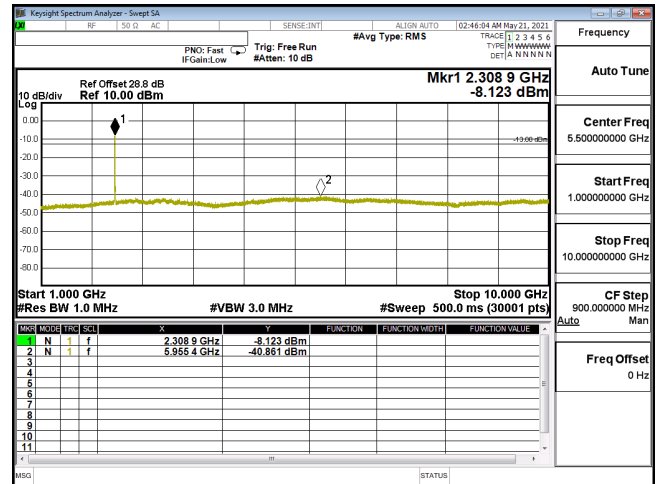
CSE-ENDC_30A_n5-256QAM_10M_CH167300_836.5(1,26)-1G-10G
