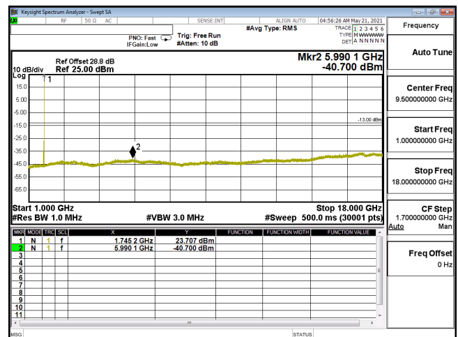
CSE-ENDC_12A_n66_64QAM_5M_CH349000_1745(1,12)-1G-18G
