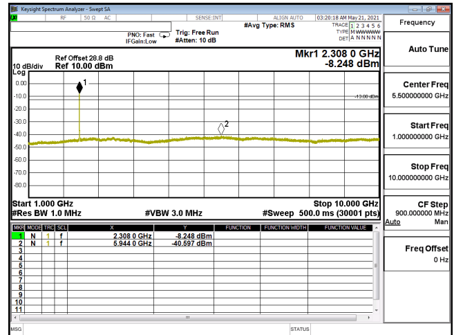
CSE-ENDC_30A_n5-256QAM_20M_CH167300_836.5(1,53)-1G-10G
