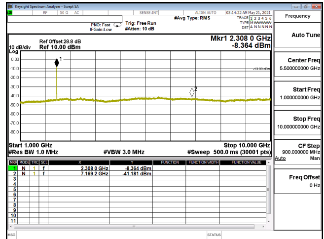
CSE-ENDC_30A_n5-256QAM_15M_CH167300_836.5(1,39)-1G-10G
