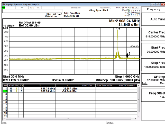
CSE-ENDC_30A_n5-64QAM_15M_CH167300_836.5(1,39)-30M-1G
