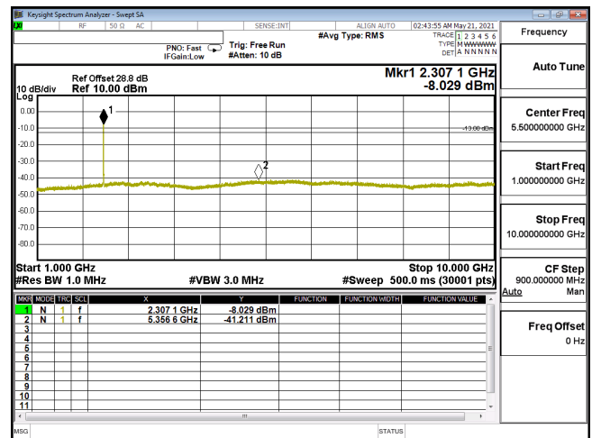
CSE-ENDC_30A_n5-PI2-BPSK_10M_CH168800_844(1,26)-1G-10G
