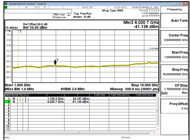
CSE-ENDC_12A_n66_QPSK_5M_CH349000_1745(1,12)-1G-18G
