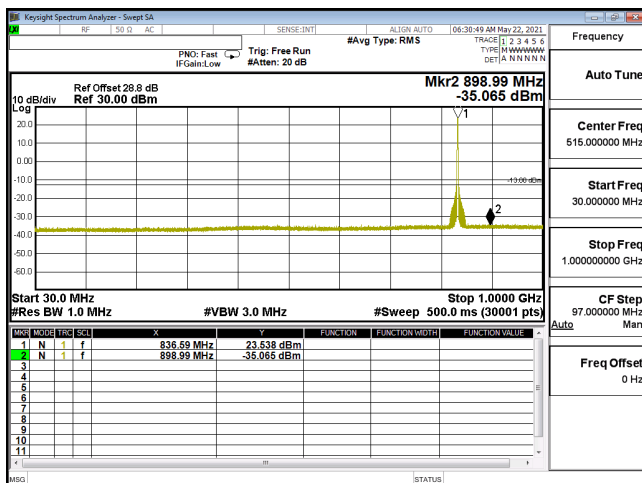
CSE-ENDC_30A_n5-64QAM_10M_CH167300_836.5(1,26)-30M-1G
