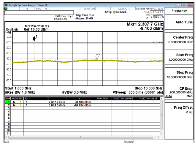
CSE-ENDC_30A_n5-64QAM_10M_CH167300_836.5(1,26)-1G-10G
