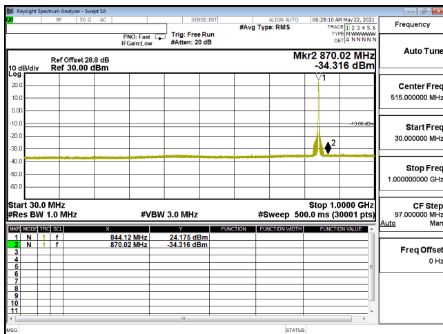
CSE-ENDC_30A_n5-64QAM_10M_CH168800_844(1,26)-30M-1G
