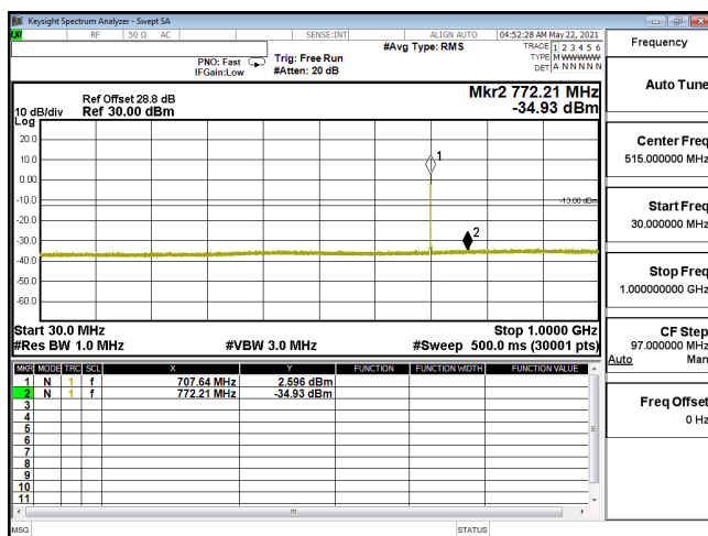
CSE-ENDC_12A_n66_16QAM_5M_CH342500_1712.5(1,12)-30M-1G
