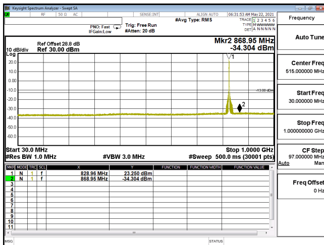
CSE-ENDC_30A_n5-256QAM_10M_CH165800_829(1,26)-30M-1G
