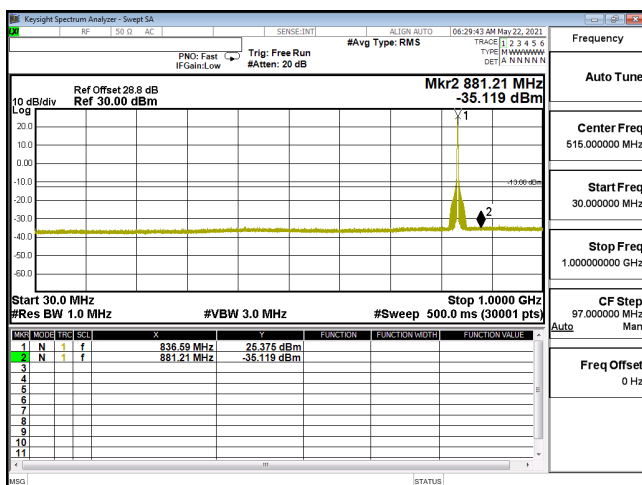
CSE-ENDC_30A_n5-PI2-BPSK_10M_CH167300_836.5(1,26)-30M-1G
