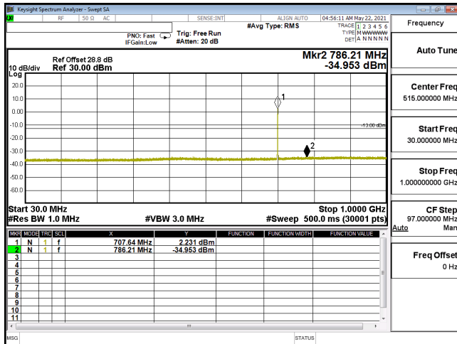
CSE-ENDC_12A_n66_256QAM_5M_CH349000_1745(1,12)-30M-1G
