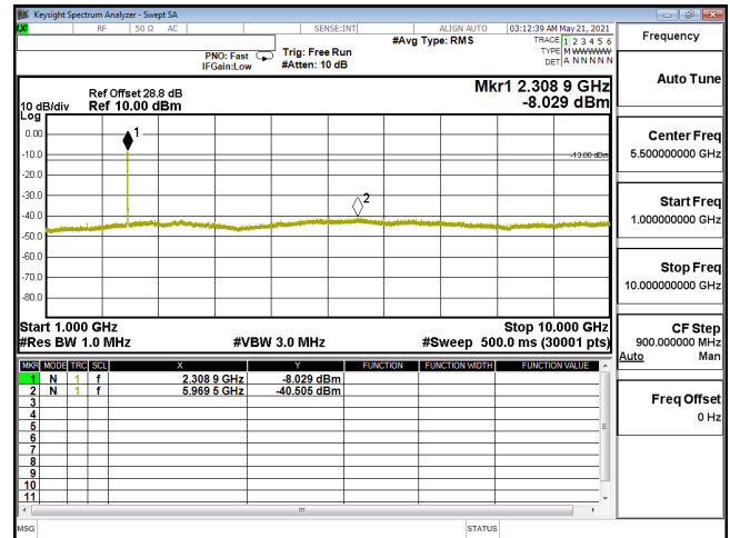
CSE-ENDC_30A_n5-PI2-BPSK_15M_CH166300_831.5(1,39)-1G-10G
