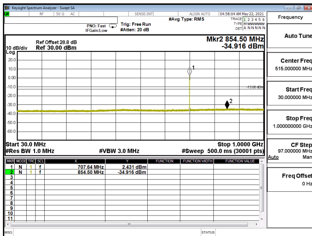
CSE-ENDC_12A_n66_64QAM_5M_CH355500_1777.5(1,12)-30M-1G
