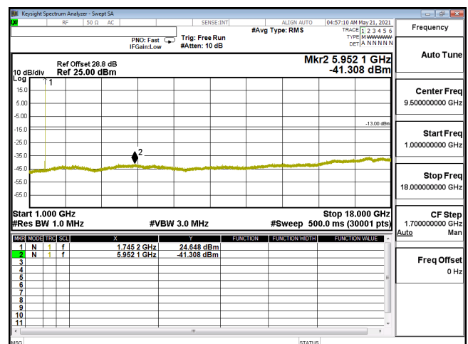
CSE-ENDC_12A_n66_PI2-BPSK_5M_CH349000_1745(1,12)-1G-18G
