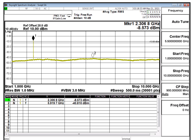
CSE-ENDC_30A_n5-QPSK_20M_CH167800_839(1,53)-1G-10G
