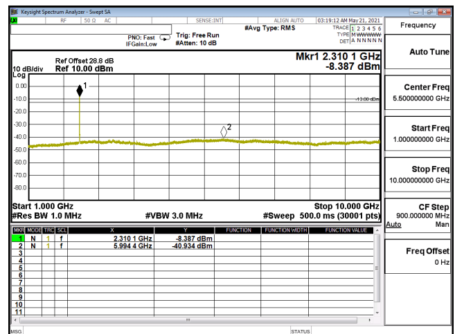
CSE-ENDC_30A_n5-PI2-BPSK_20M_CH167300_836.5(1,53)-1G-10G
