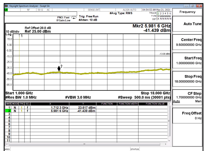
CSE-ENDC_12A_n66_16QAM_5M_CH342500_1712.5(1,12)-1G-18G
