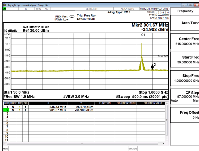
CSE-ENDC_30A_n5-16QAM_15M_CH167300_836.5(1,39)-30M-1G
