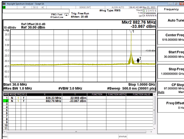
CSE-ENDC_30A_n5-256QAM_15M_CH167300_836.5(1,39)-30M-1G
