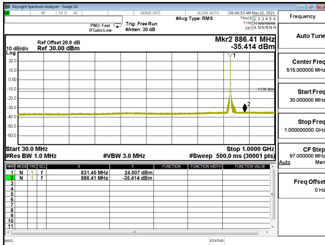
CSE-ENDC_30A_n5-64QAM_15M_CH166300_831.5(1,39)-30M-1G
