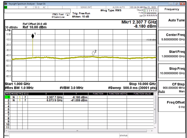
CSE-ENDC_30A_n5-16QAM_15M_CH168300_841.5(1,39)-1G-10G
