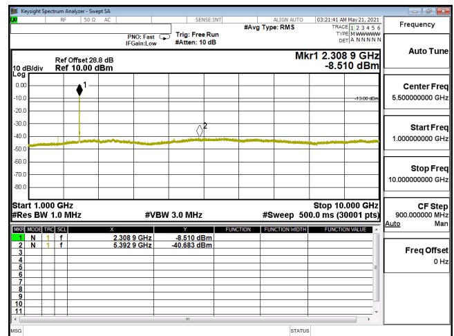
CSE-ENDC_30A_n5-QPSK_20M_CH166800_834(1,53)-1G-10G
