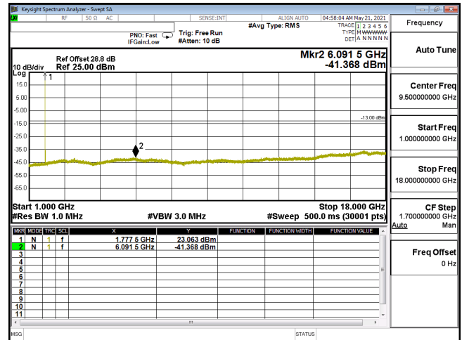
CSE-ENDC_12A_n66_16QAM_5M_CH355500_1777.5(1,12)-1G-18G
