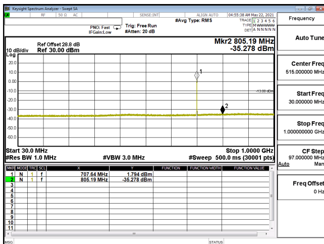
CSE-ENDC_12A_n66_64QAM_5M_CH349000_1745(1,12)-30M-1G
