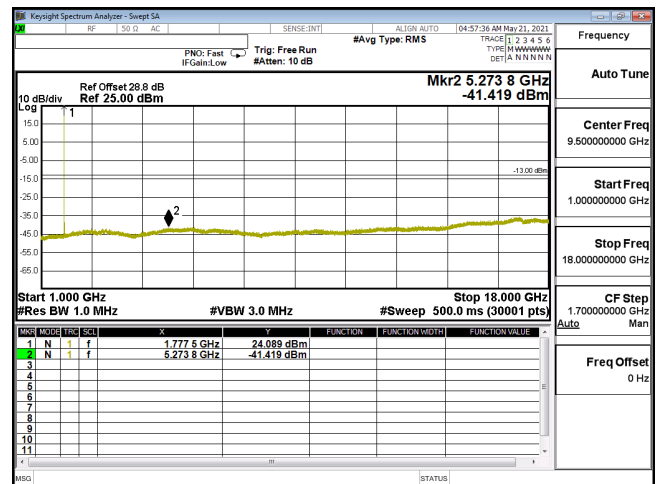
CSE-ENDC_12A_n66_PI2-BPSK_5M_CH355500_1777.5(1,12)-1G-18G
