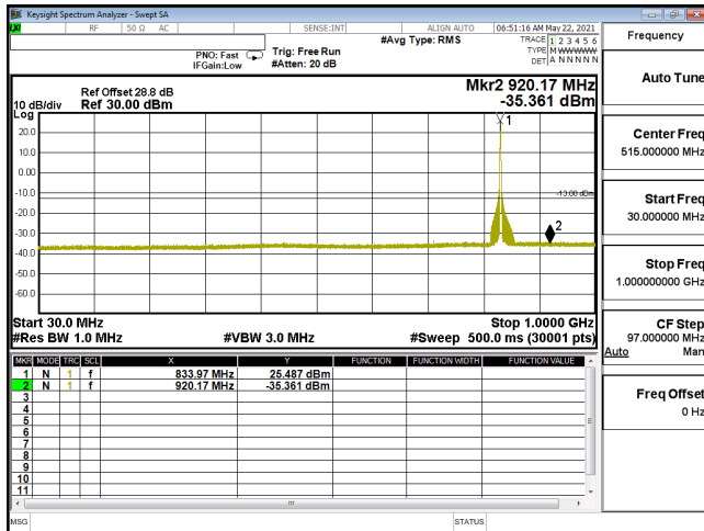
CSE-ENDC_30A_n5-PI2-BPSK_20M_CH166800_834(1,53)-30M-1G
