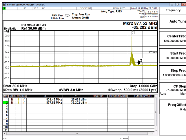
CSE-ENDC_30A_n5-QPSK_15M_CH166300_831.5(1,39)-30M-1G
