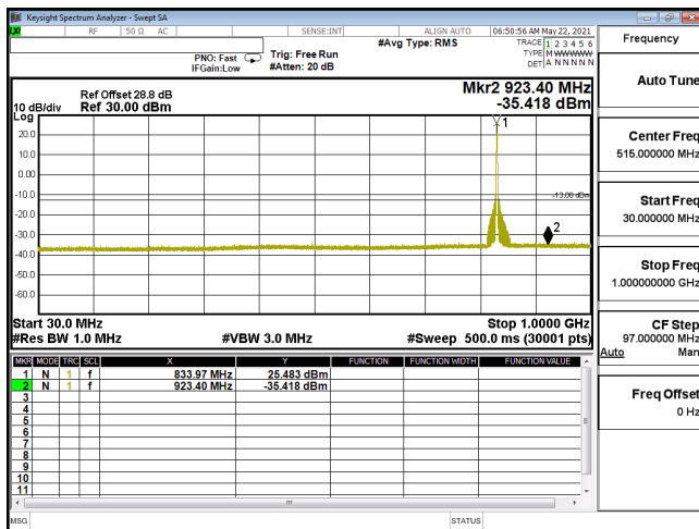
CSE-ENDC_30A_n5-QPSK_20M_CH166800_834(1,53)-30M-1G
