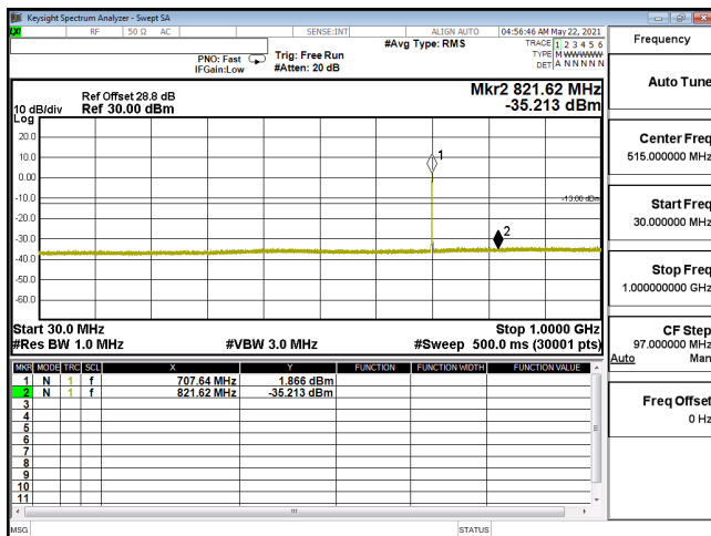
CSE-ENDC_12A_n66_PI2-BPSK_5M_CH355500_1777.5(1,12)-30M-1G
