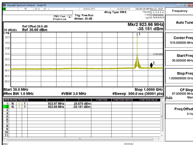
CSE-ENDC_30A_n5-16QAM_20M_CH166800_834(1,53)-30M-1G
