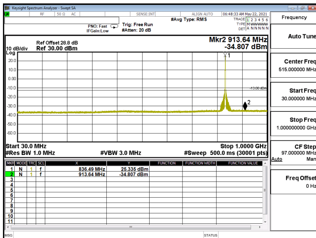
CSE-ENDC_30A_n5-16QAM_20M_CH167300_836.5(1,53)-30M-1G
