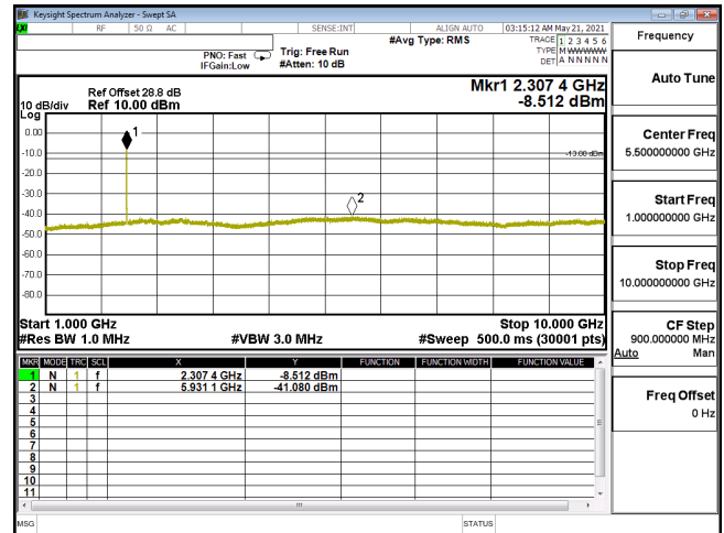
CSE-ENDC_30A_n5-QPSK_15M_CH167300_836.5(1,39)-1G-10G
