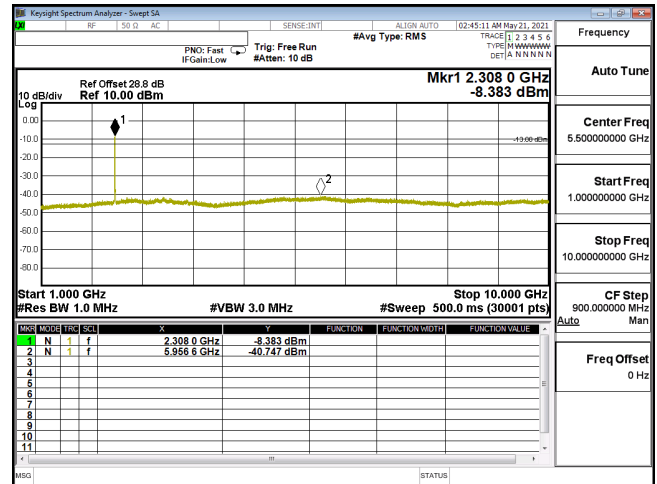
CSE-ENDC_30A_n5-QPSK_10M_CH167300_836.5(1,26)-1G-10G
