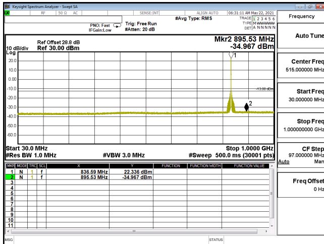
CSE-ENDC_30A_n5-256QAM_10M_CH167300_836.5(1,26)-30M-1G
