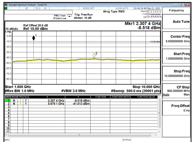
CSE-ENDC_30A_n5-256QAM_10M_CH165800_829(1,26)-1G-10G
