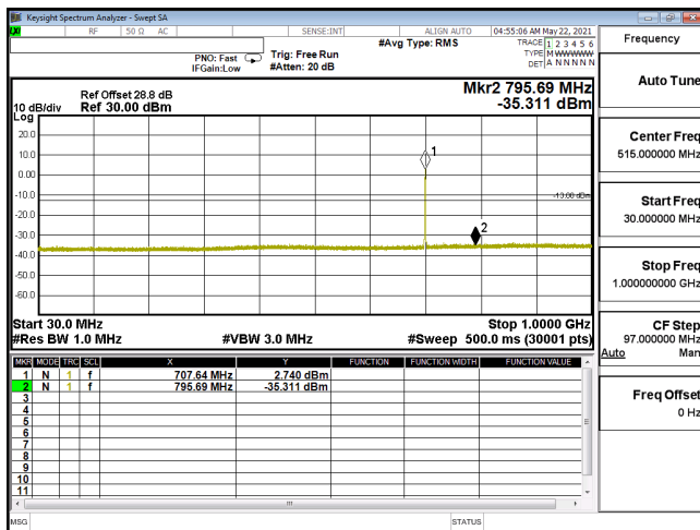
CSE-ENDC_12A_n66_16QAM_5M_CH349000_1745(1,12)-30M-1G
