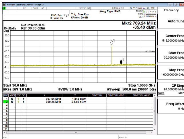
CSE-ENDC_12A_n66_256QAM_5M_CH342500_1712.5(1,12)-30M-1G
