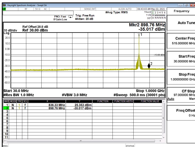
CSE-ENDC_30A_n5-PI2-BPSK_15M_CH167300_836.5(1,39)-30M-1G
