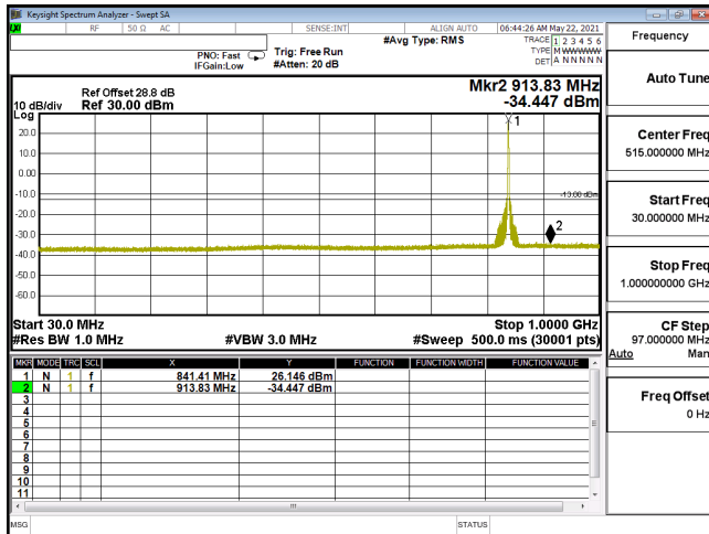
CSE-ENDC_30A_n5-16QAM_15M_CH168300_841.5(1,39)-30M-1G
