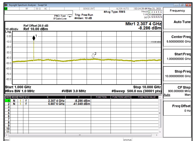
CSE-ENDC_30A_n5-64QAM_15M_CH167300_836.5(1,39)-1G-10G
