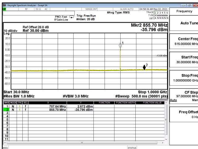
CSE-ENDC_12A_n66_256QAM_5M_CH355500_1777.5(1,12)-30M-1G
