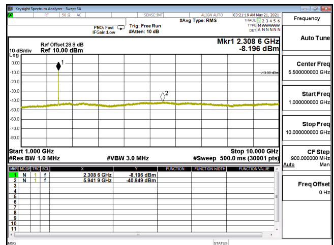
CSE-ENDC_30A_n5-16QAM_20M_CH166800_834(1,53)-1G-10G
