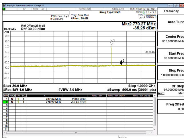
CSE-ENDC_12A_n66_PI2-BPSK_5M_CH349000_1745(1,12)-30M-1G
