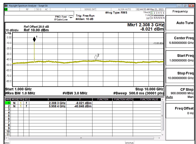
CSE-ENDC_30A_n5-PI2-BPSK_10M_CH167300_836.5(1,26)-1G-10G
