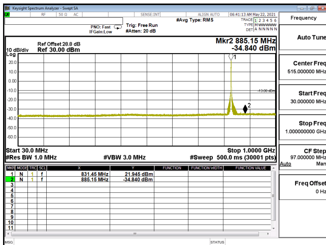
CSE-ENDC_30A_n5-256QAM_15M_CH166300_831.5(1,39)-30M-1G
