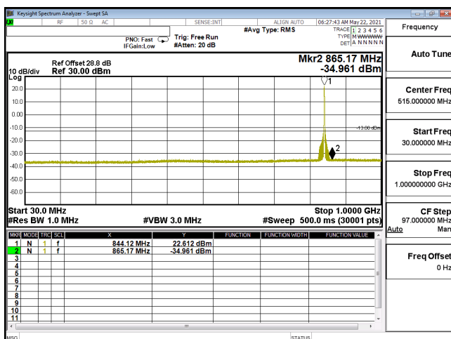
CSE-ENDC_30A_n5-256QAM_10M_CH168800_844(1,26)-30M-1G
