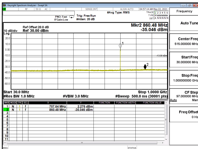
CSE-ENDC_12A_n66_QPSK_5M_CH355500_1777.5(1,12)-30M-1G
