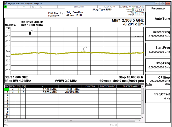
CSE-ENDC_30A_n5-16QAM_20M_CH167800_839(1,53)-1G-10G
