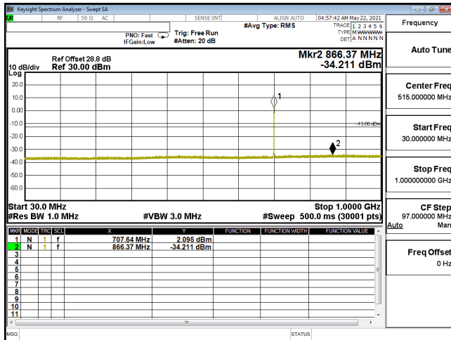
CSE-ENDC_12A_n66_16QAM_5M_CH355500_1777.5(1,12)-30M-1G
