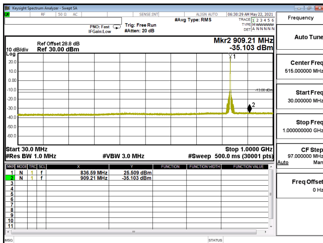
CSE-ENDC_30A_n5-16QAM_10M_CH167300_836.5(1,26)-30M-1G
