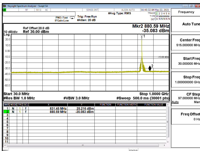
CSE-ENDC_30A_n5-16QAM_15M_CH166300_831.5(1,39)-30M-1G
