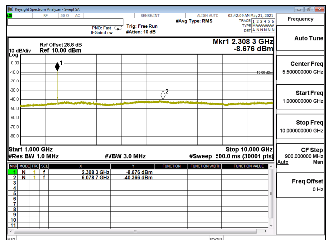
CSE-ENDC_30A_n5-256QAM_10M_CH168800_844(1,26)-1G-10G
