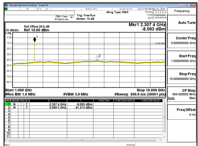
CSE-ENDC_30A_n5-256QAM_15M_CH168300_841.5(1,39)-1G-10G
