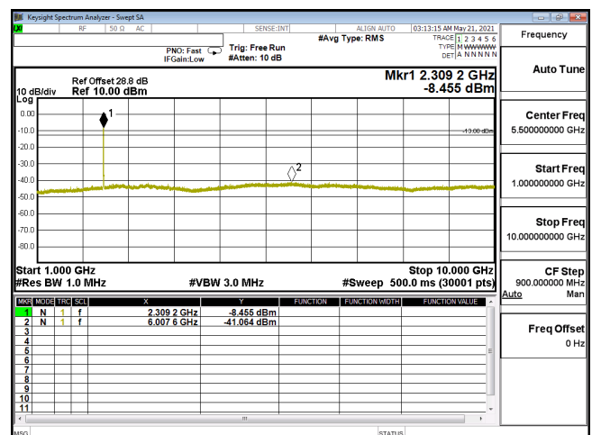
CSE-ENDC_30A_n5-16QAM_15M_CH166300_831.5(1,39)-1G-10G
