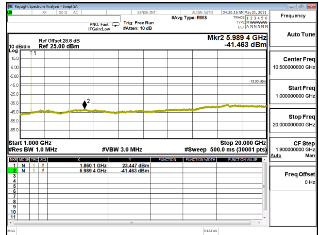
CSE-ENDC_5A_n2_P12-BPSK_20M_CH372000_1860(1,53)-1G-20G
