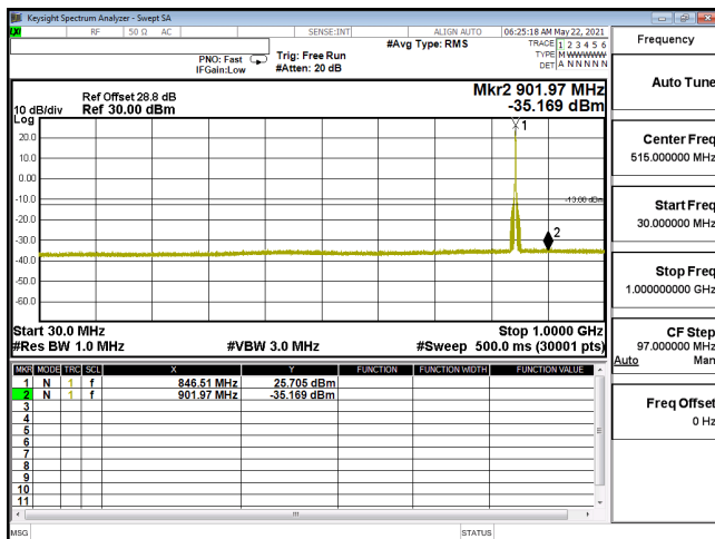
CSE-ENDC_30A_n5-PI2-BPSK_5M_CH169300_846.5(1,12)-30M-1G
