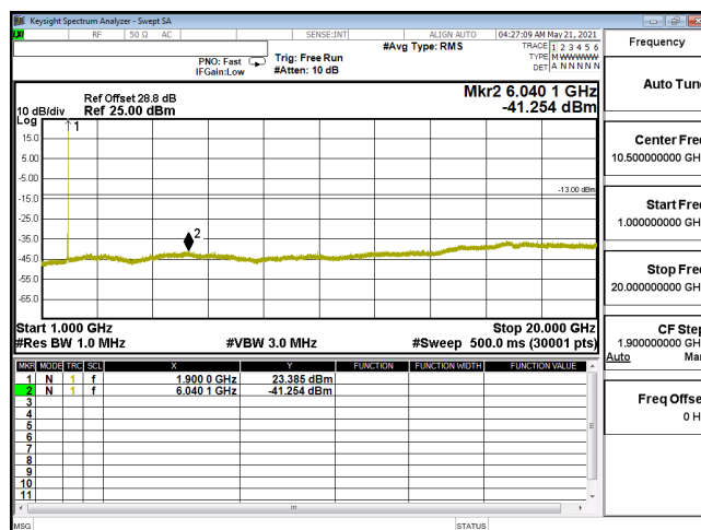
CSE-ENDC_5A_n2_QPSK_20M_CH380000_1900(1,53)-1G-20G
