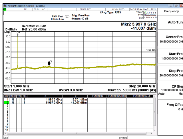
CSE-ENDC_5A_n2_256QAM_20M_CH376000_1880(1,53)-1G-20G
