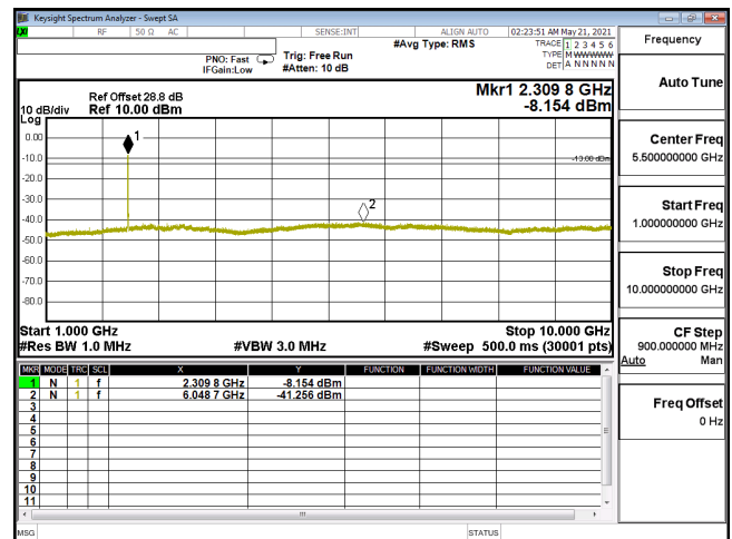
CSE-ENDC_30A_n5-PI2-BPSK_5M_CH169300_846.5(1,12)-1G-10G
