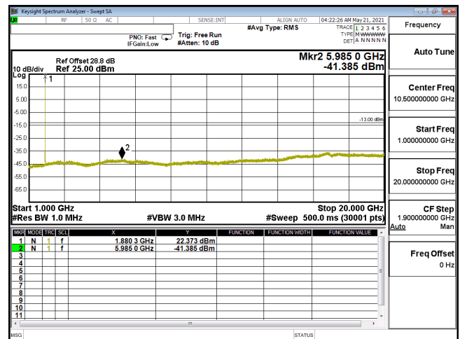
CSE-ENDC_5A_n2_16QAM_15M_CH376000_1880(1,39)-1G-20G
