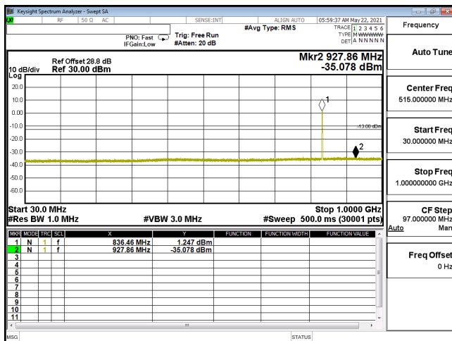
CSE-ENDC_5A_n2_16QAM_15M_CH376000_1880(1,39)-30M-1G
