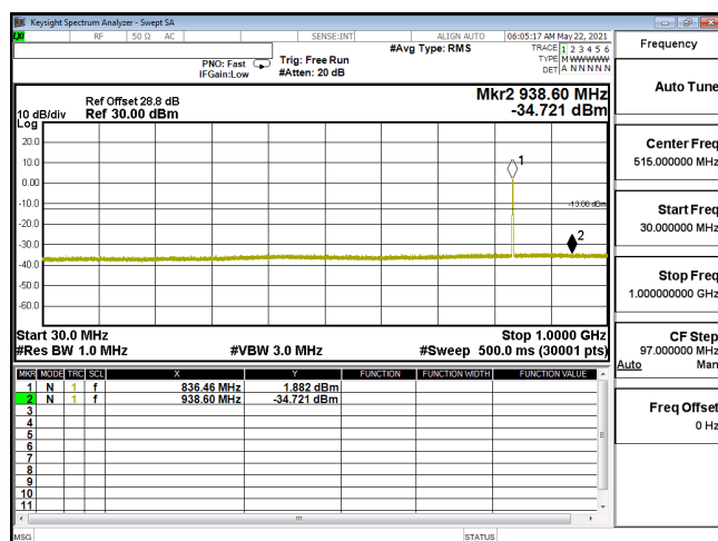
CSE-ENDC_5A_n2_256QAM_20M_CH376000_1880(1,53)-30M-1G
