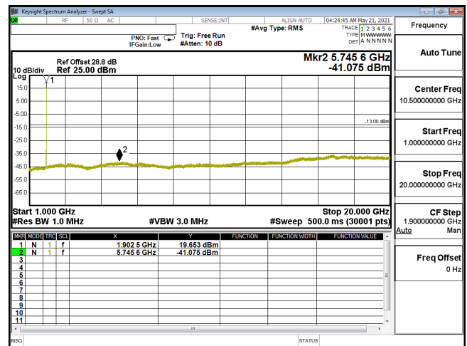
CSE-ENDC_5A_n2_64QAM_15M_CH380500_1902.5(1,39)-1G-20G
