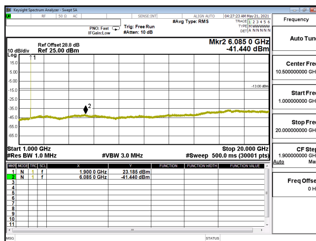
CSE-ENDC_5A_n2_PI2-BPSK_20M_CH380000_1900(1,53)-1G-20G
