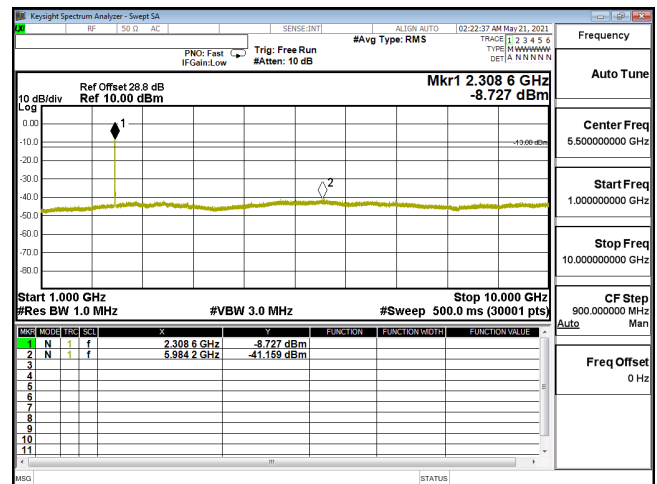
CSE-ENDC_30A_n5-16QAM_5M_CH167300_836.5(1,12)-1G-10G
