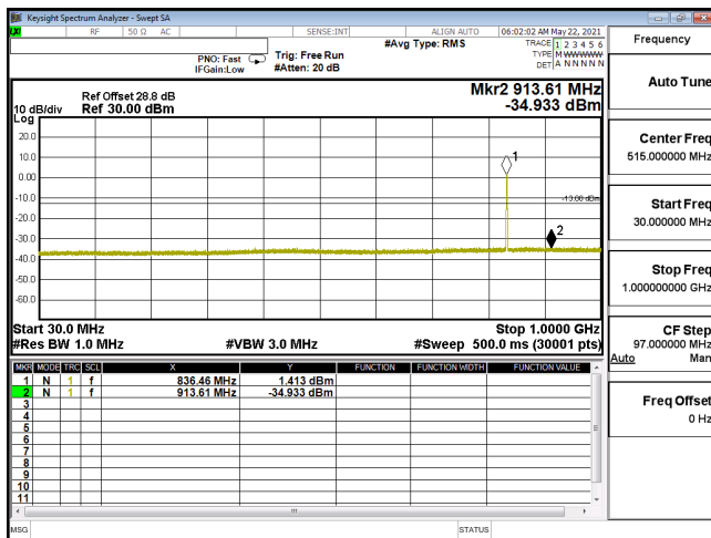
CSE-ENDC_5A_n2_64QAM_15M_CH380500_1902.5(1,39)-30M-1G
