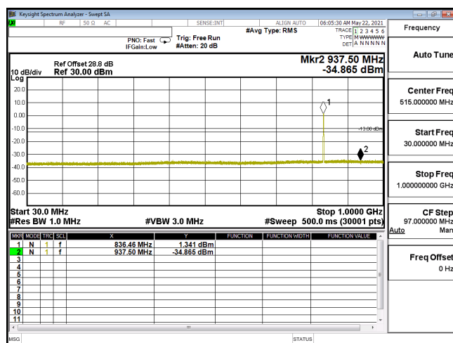
CSE-ENDC_5A_n2_PI2-BPSK_20M_CH380000_1900(1,53)-30M-1G
