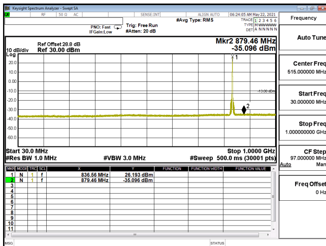
CSE-ENDC_30A_n5-16QAM_5M_CH167300_836.5(1,12)-30M-1G
