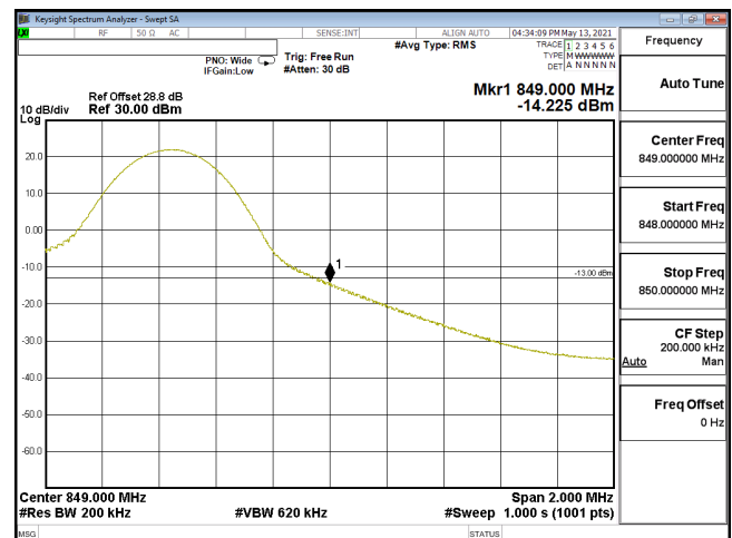
EDGE-ENDC_30A_n5-16QAM_20M_CH167800_839(1,105)_SCS15KHz
