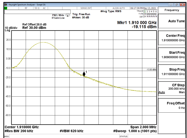
EDGE-ENDC_5A_n2-64QAM_20M_CH380000_1900(1,105)_SCS15KHz
