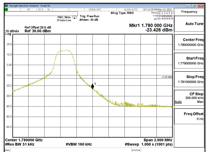
EDGE-ENDC_12A_n66-256QAM_5M_CH355500_1777.5(1,24)_SCS15KHz
