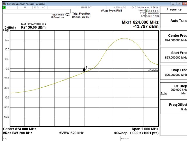
EDGE-ENDC_30A_n5-64QAM_20M_CH166800_834(1,0)_SCS15KHz
