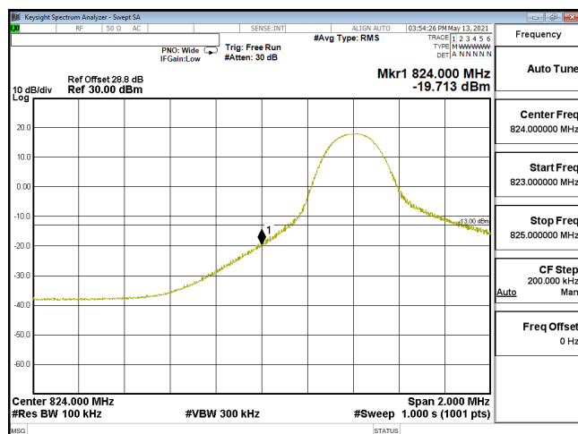
EDGE-ENDC_30A_n5-256QAM_10M_CH165800_829(1,0)_SCS15KHz
