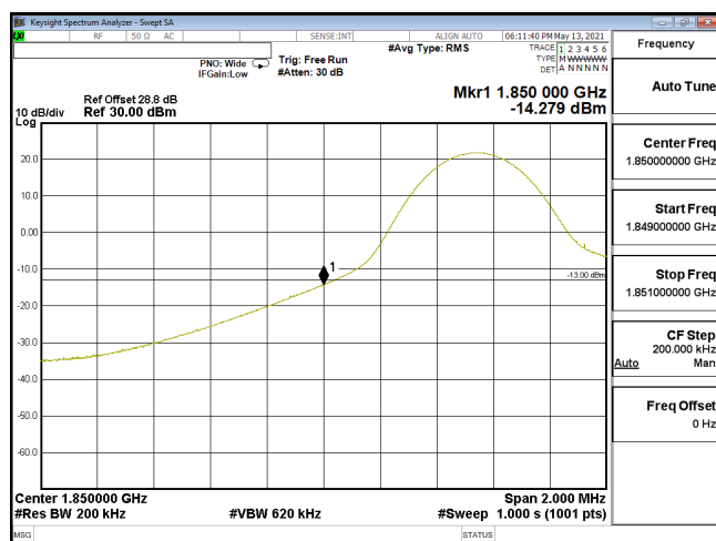
EDGE-ENDC_5A_n2-QPSK_20M_CH372000_1860(1,0)_SCS15KHz
