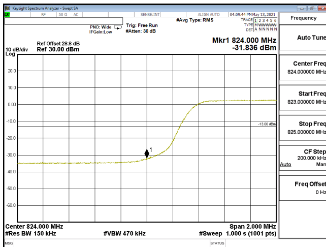
EDGE-ENDC_30A_n5-64QAM_15M_CH166300_831.5(75,0)_SCS15KHz
