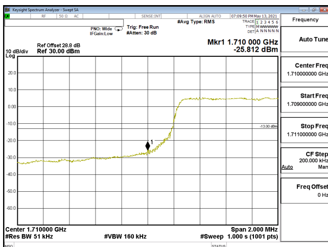
EDGE-ENDC_12A_n66-PI2-BPSK_5M_CH342500_1712.5(25,0)_SCS15KHz
