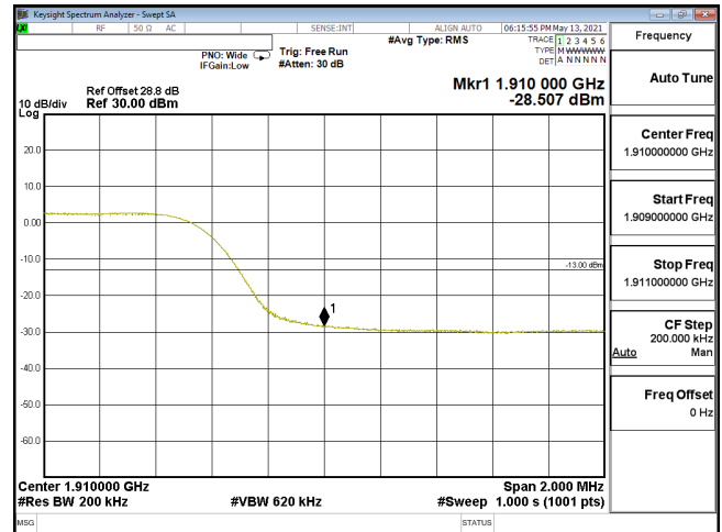
EDGE-ENDC_5A_n2-QPSK_20M_CH380000_1900(100,6)_SCS15KHz
