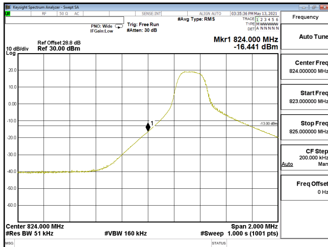
EDGE-ENDC_30A_n5-PI2-BPSK_5M_CH165300_826.5(1,0)_SCS15KHz
