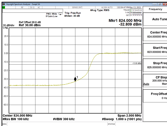
EDGE-ENDC_30A_n5-256QAM_10M_CH165800_829(50,0)_SCS15KHz
