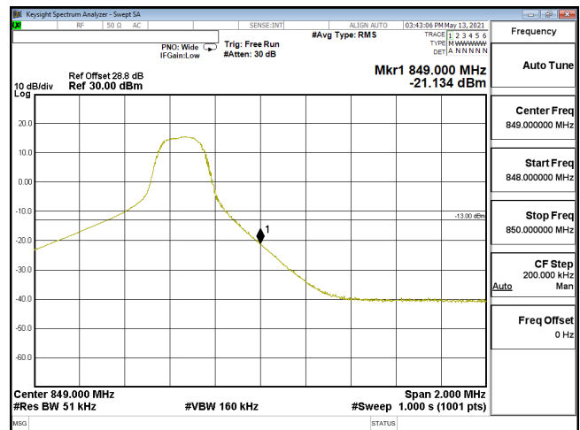
EDGE-ENDC_30A_n5-256QAM_5M_CH169300_846.5(1,24)_SCS15KHz
