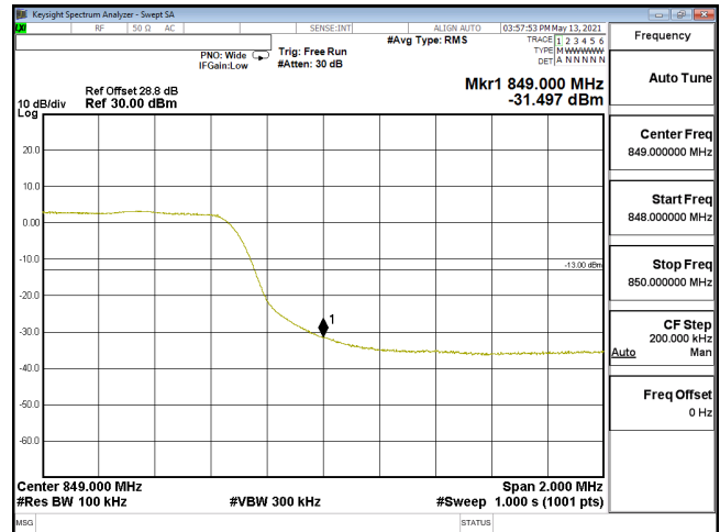
EDGE-ENDC_30A_n5-64QAM_10M_CH168800_844(50,2)_SCS15KHz
