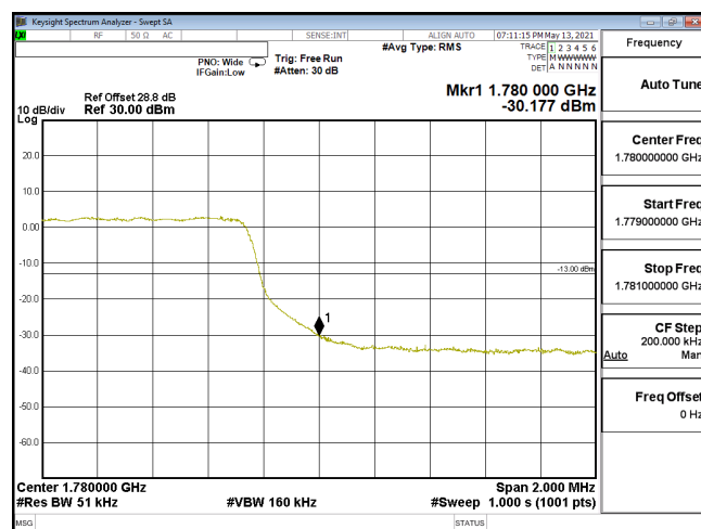
EDGE-ENDC_12A_n66-16QAM_5M_CH355500_1777.5(25,0)_SCS15KHz
