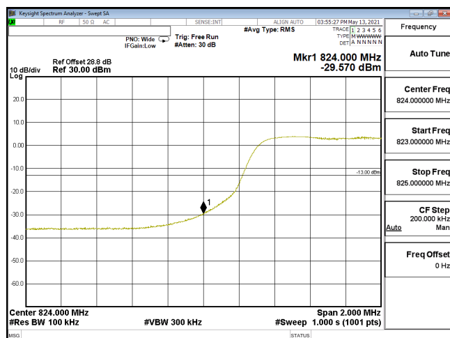
EDGE-ENDC_30A_n5-16QAM_10M_CH165800_829(50,0)_SCS15KHz
