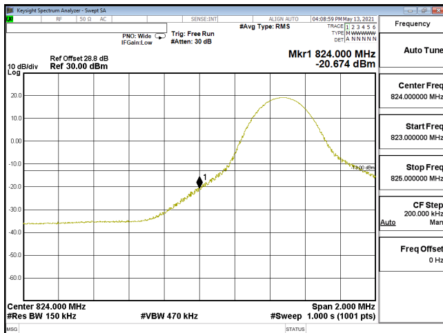
EDGE-ENDC_30A_n5-256QAM_15M_CH166300_831.5(1,0)_SCS15KHz
