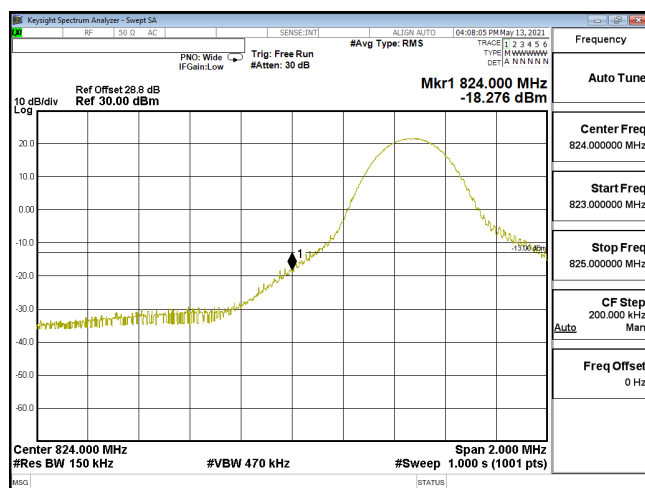
EDGE-ENDC_30A_n5-16QAM_15M_CH166300_831.5(1,0)_SCS15KHz
