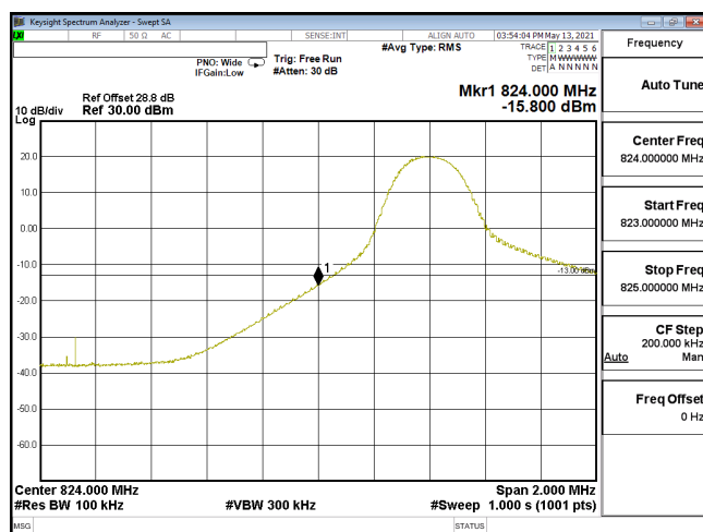
EDGE-ENDC_30A_n5-64QAM_10M_CH165800_829(1,0)_SCS15KHz
