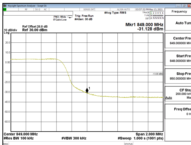
EDGE-ENDC_30A_n5-16QAM_10M_CH168800_844(50,2)_SCS15KHz
