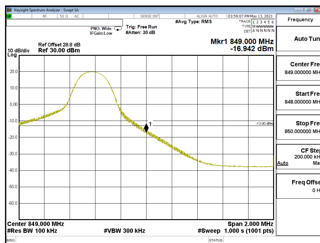
EDGE-ENDC_30A_n5-64QAM_10M_CH168800_844(1,51)_SCS15KHz
