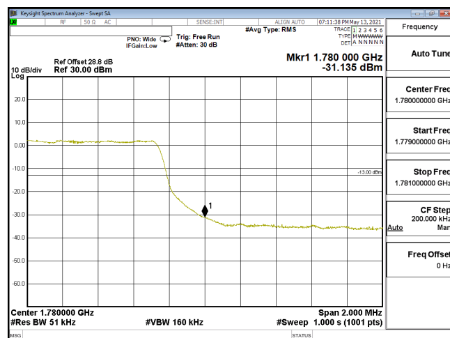
EDGE-ENDC_12A_n66-64QAM_5M_CH355500_1777.5(25,0)_SCS15KHz
