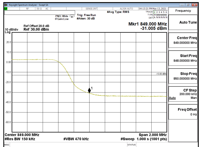
EDGE-ENDC_30A_n5-64QAM_15M_CH168300_841.5(75,4)_SCS15KHz
