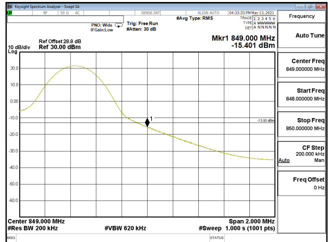
EDGE-ENDC_30A_n5-64QAM_20M_CH167800_839(1,105)_SCS15KHz
