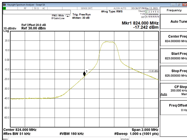
EDGE-ENDC_30A_n5-QPSK_5M_CH165300_826.5(1,0)_SCS15KHz
