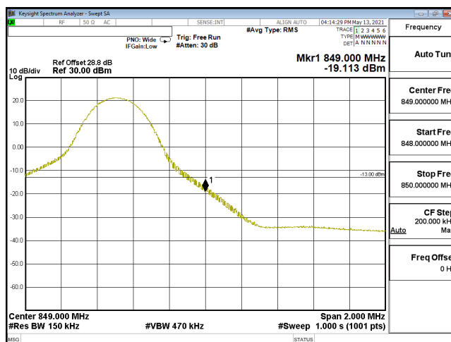
EDGE-ENDC_30A_n5-64QAM_15M_CH168300_841.5(1,78)_SCS15KHz
