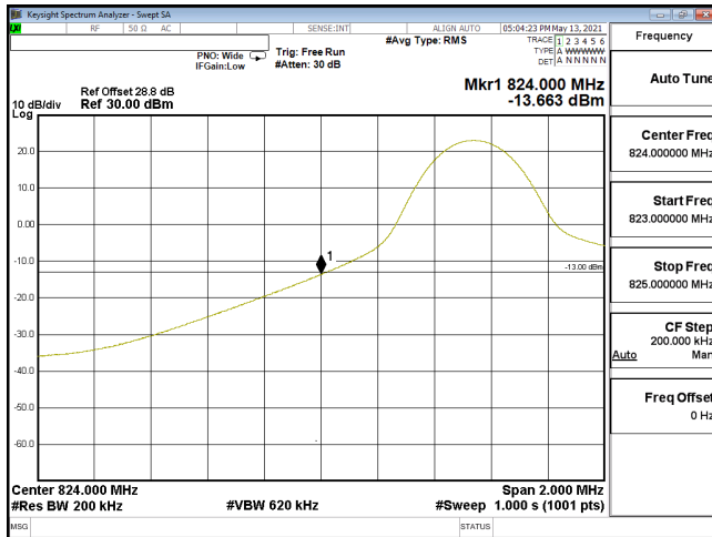
EDGE-ENDC_30A_n5-PI2-BPSK_20M_CH166800_834(1,0)_SCS15KHz
