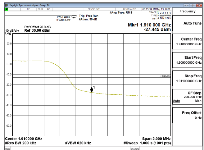
EDGE-ENDC_5A_n2-256QAM_20M_CH380000_1900(1,105)_SCS15KHz
