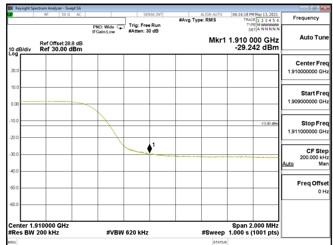
EDGE-ENDC_5A_n2-16QAM_20M_CH380000_1900(100,6)_SCS15KHz
