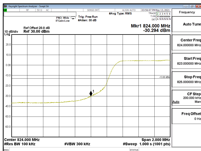
EDGE-ENDC_30A_n5-PI2-BPSK_10M_CH165800_829(50,0)_SCS15KHz
