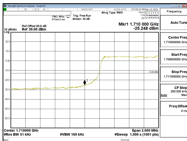
EDGE-ENDC_12A_n66-QPSK_5M_CH342500_1712.5(25,0)_SCS15KHz
