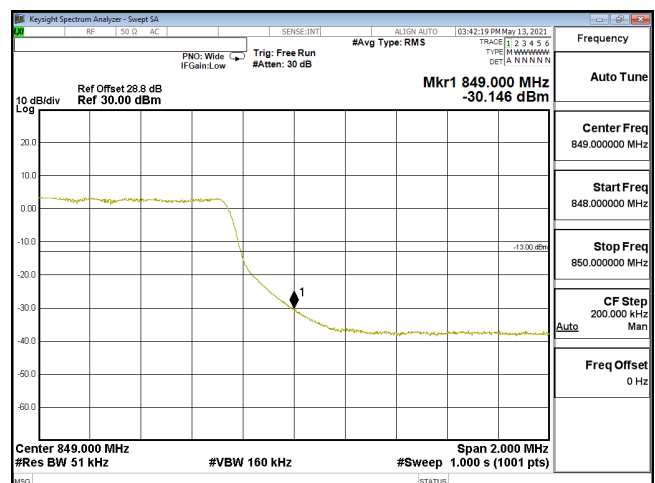
EDGE-ENDC_30A_n5-64QAM_5M_CH169300_846.5(25,0)_SCS15KHz
