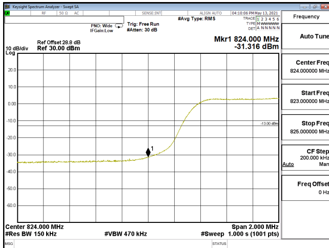
EDGE-ENDC_30A_n5-16QAM_15M_CH166300_831.5(75,0)_SCS15KHz
