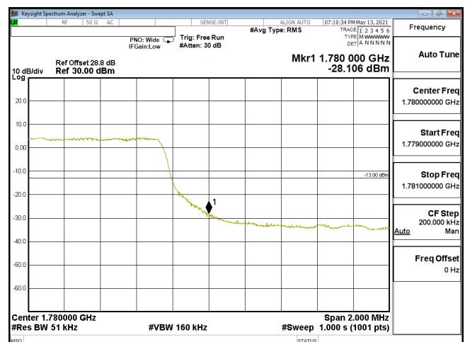
EDGE-ENDC_12A_n66-PI2-BPSK_5M_CH355500_1777.5(25,0)_SCS15KHz
