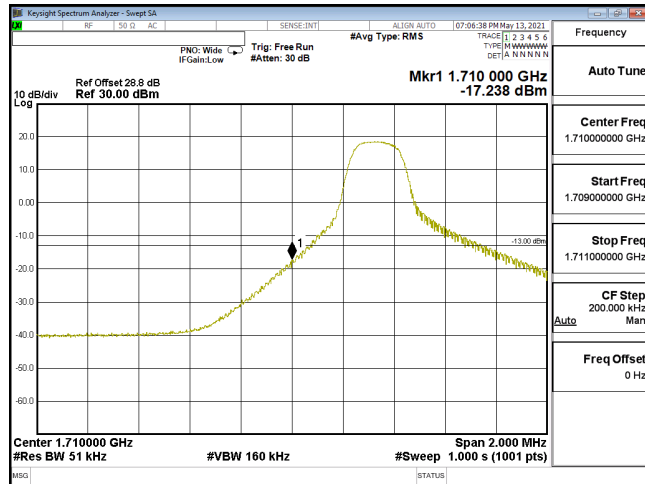
EDGE-ENDC_12A_n66-PI2-BPSK_5M_CH342500_1712.5(1,0)_SCS15KHz
