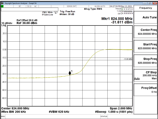
EDGE-ENDC_30A_n5-256QAM_20M_CH166800_834(100,0)_SCS15KHz
