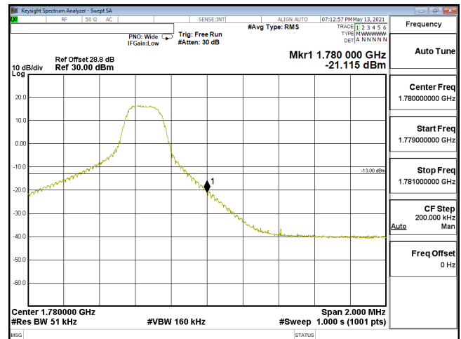
EDGE-ENDC_12A_n66-64QAM_5M_CH355500_1777.5(1,24)_SCS15KHz
