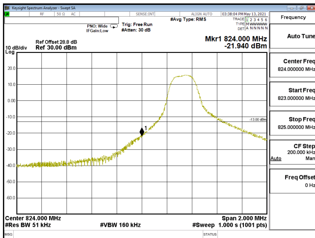
EDGE-ENDC_30A_n5-256QAM_5M_CH165300_826.5(1,0)_SCS15KHz
