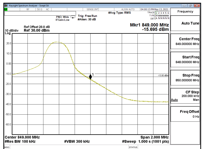
EDGE-ENDC 30A n5-PI2-BPSK 10M_CH168800_844(1,51)_SCS15KHz
