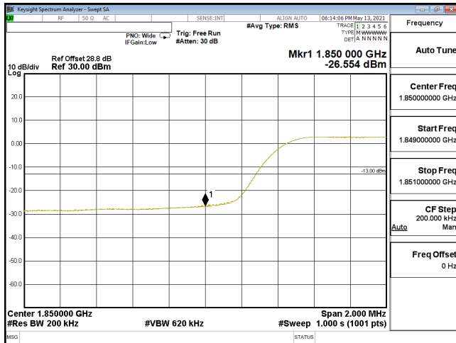
EDGE-ENDC_5A_n2-QPSK_20M_CH372000_1860(100,0)_SCS15KHz
