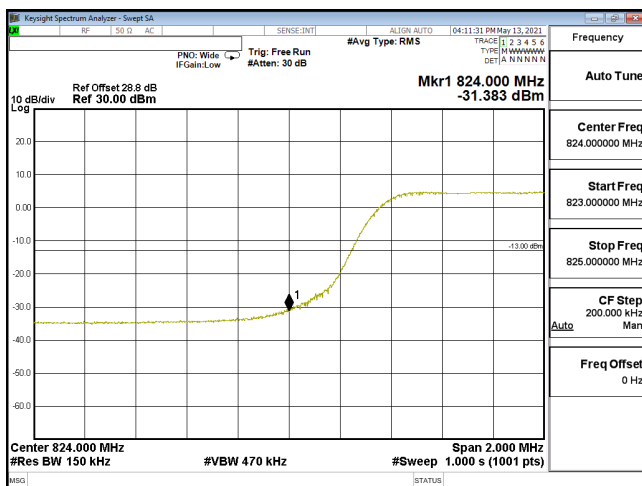
EDGE-ENDC_30A_n5-PI2-BPSK_15M_CH166300_831.5(75,0)_SCS15KHz
