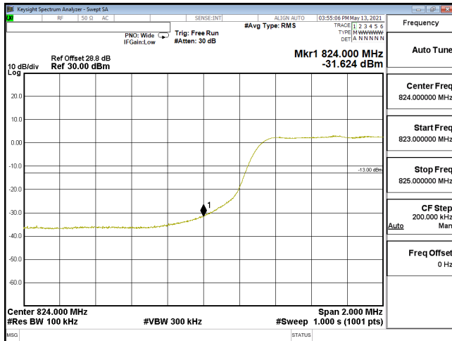
EDGE-ENDC_30A_n5-64QAM_10M_CH165800_829(50,0)_SCS15KHz
