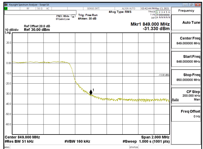
EDGE-ENDC 30A n5-256QAM 5M CH169300 846.5(25,0) SCS15KHz
