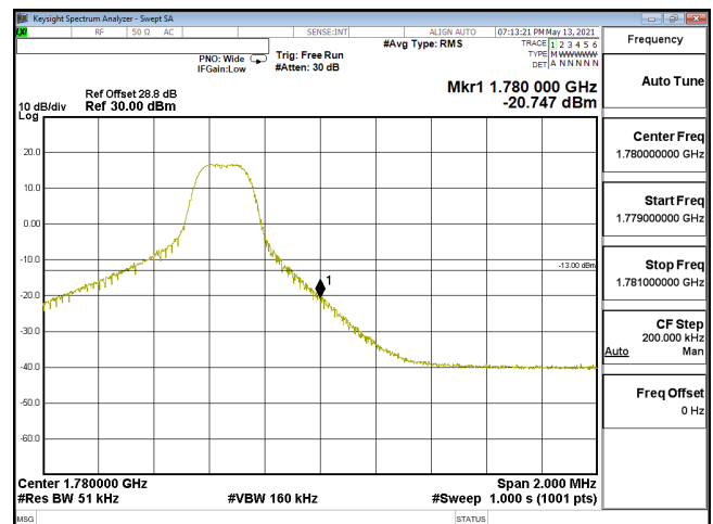
EDGE-ENDC_12A_n66-16QAM_5M_CH355500_1777.5(1,24)_SCS15KHz
