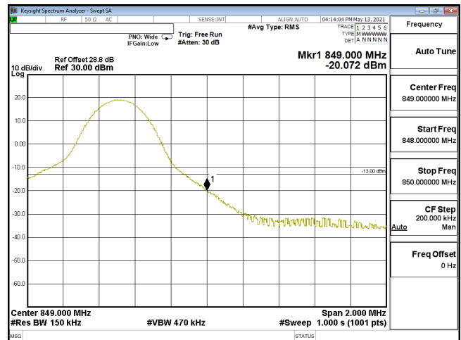
EDGE-ENDC_30A_n5-256QAM_15M_CH168300_841.5(1,78)_SCS15KHz
