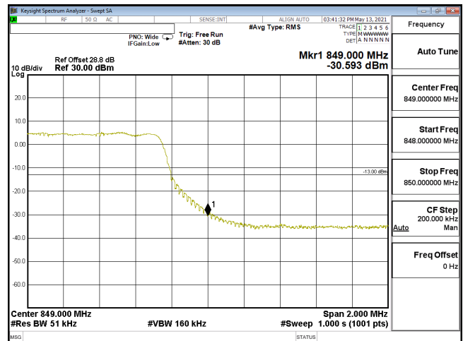
EDGE-ENDC_30A_n5-QPSK_5M_CH169300_846.5(25,0)_SCS15KHz
