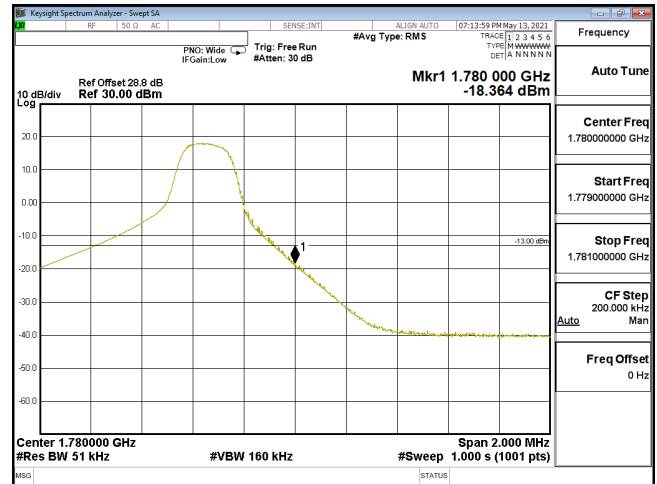
EDGE-ENDC_12A_n66-PI2-BPSK_5M_CH355500_1777.5(1,24)_SCS15KHz
