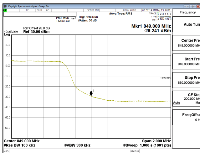
EDGE-ENDC_30A_n5-QPSK_10M_CH168800_844(50,2)_SCS15KHz
