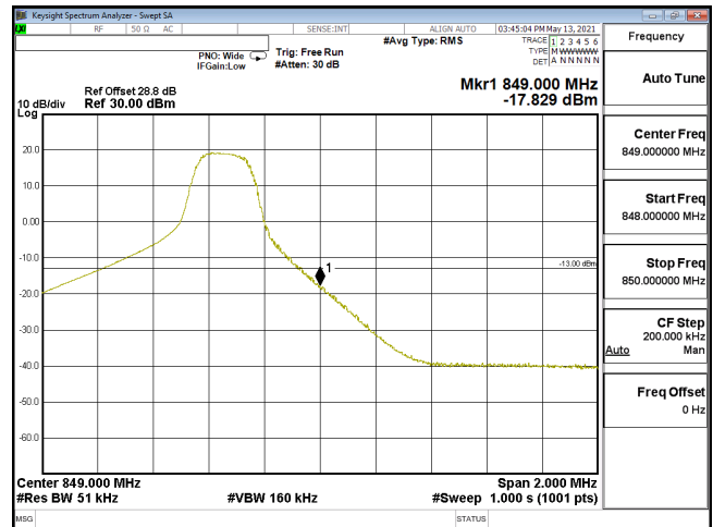
EDGE-ENDC_30A_n5-PI2-BPSK_5M_CH169300_846.5(1,24)_SCS15KHz
