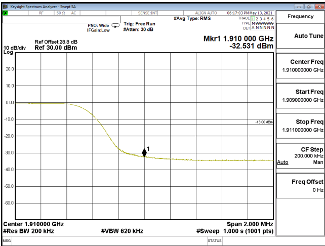
EDGE-ENDC_5A_n2-256QAM_20M_CH380000_1900(100,6)_SCS15KHz
