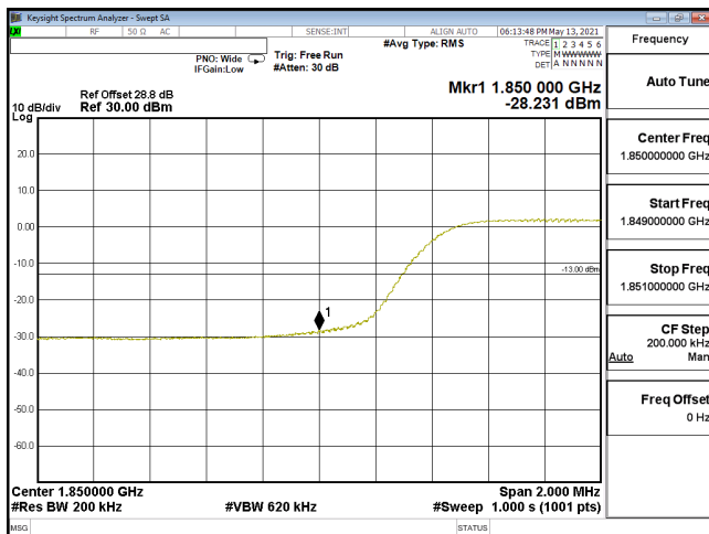
EDGE-ENDC_5A_n2-16QAM_20M_CH372000_1860(100,0)_SCS15KHz
