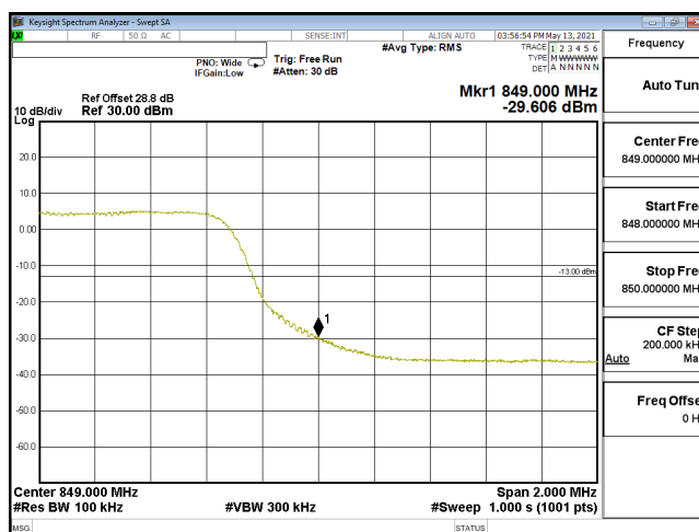
EDGE-ENDC_30A_n5-PI2-BPSK_10M_CH168800_844(50,2)_SCS15KHz
