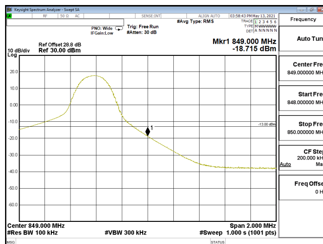
EDGE-ENDC_30A_n5-256QAM_10M_CH168800_844(1,51)_SCS15KHz
