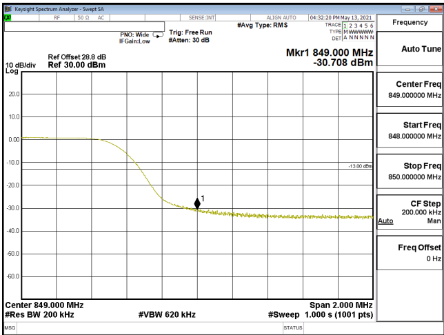
EDGE-ENDC_30A_n5-256QAM_20M_CH167800_839(100,6)_SCS15KHz
