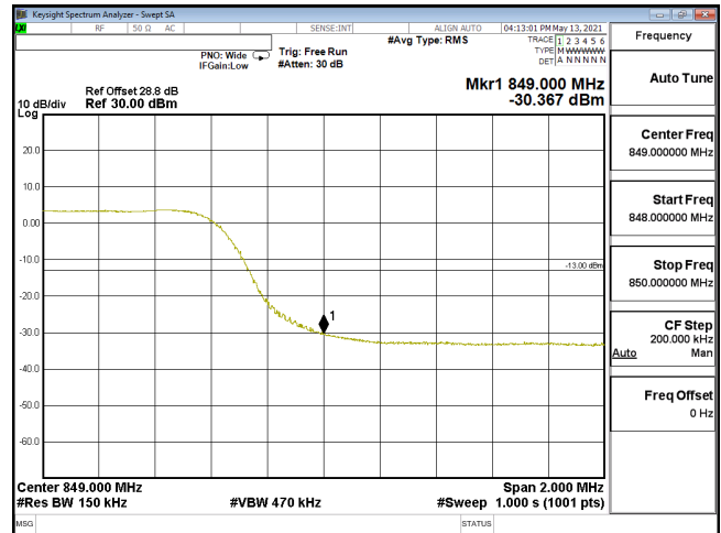
EDGE-ENDC_30A_n5-16QAM_15M_CH168300_841.5(75,4)_SCS15KHz
