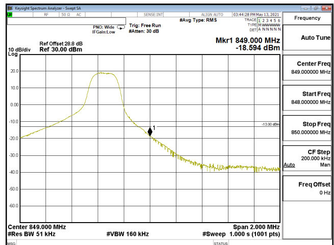
EDGE-ENDC_30A_n5-QPSK_5M_CH169300_846.5(1,24)_SCS15KHz
