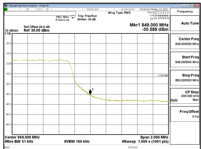
EDGE-ENDC_30A_n5-16QAM_5M_CH169300_846.5(25,0)_SCS15KHz
