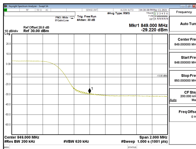
EDGE-ENDC 30A n5-16QAM 20M CH167800 839(100,6) SCS15KHz
