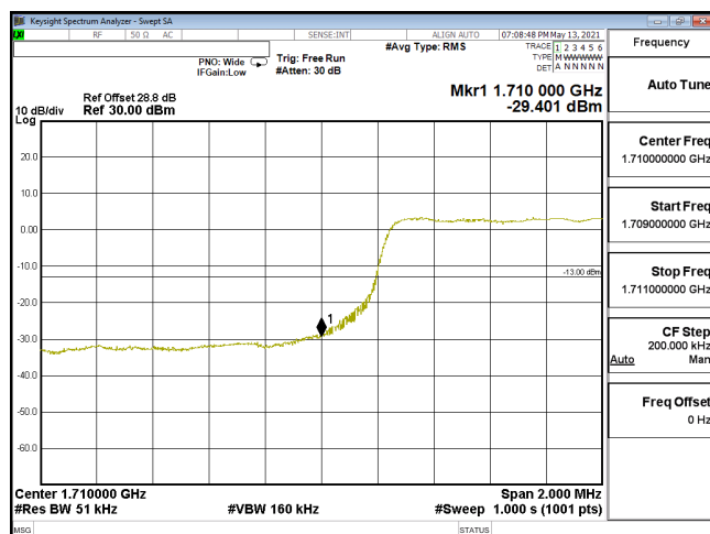
EDGE-ENDC_12A_n66-64QAM_5M_CH342500_1712.5(25,0)_SCS15KHz
