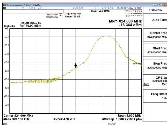
EDGE-ENDC_30A_n5-64QAM_15M_CH166300_831.5(1,0)_SCS15KHz
