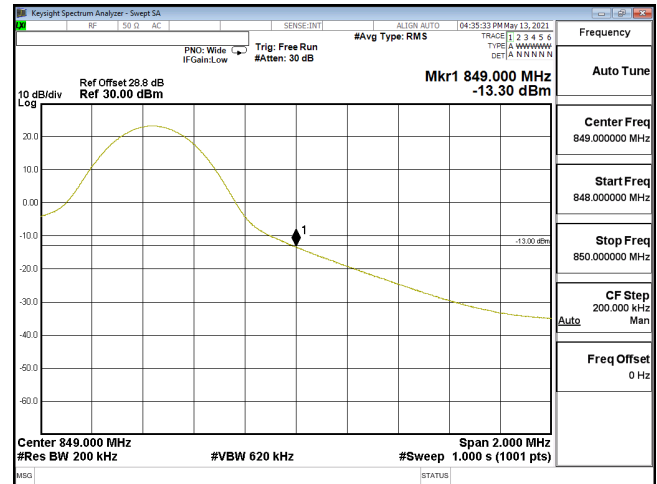
EDGE-ENDC_30A_n5-PI2-BPSK_20M_CH167800_839(1,105)_SCS15KHz
