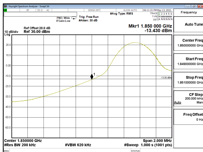
EDGE-ENDC_5A_n2-PI2-BPSK_20M_CH372000_1860(1,0)_SCS15KHz
