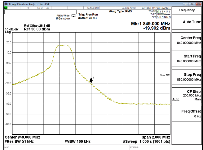
EDGE-ENDC_30A_n5-64QAM_5M_CH169300_846.5(1,24)_SCS15KHz
