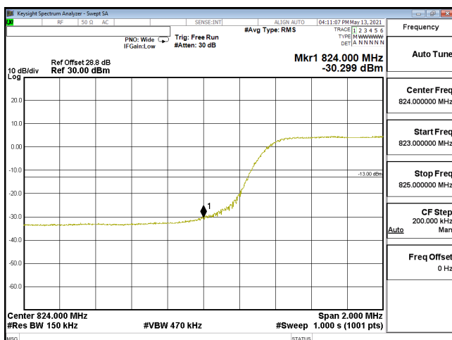
EDGE-ENDC_30A_n5-QPSK_15M_CH166300_831.5(75,0)_SCS15KHz
