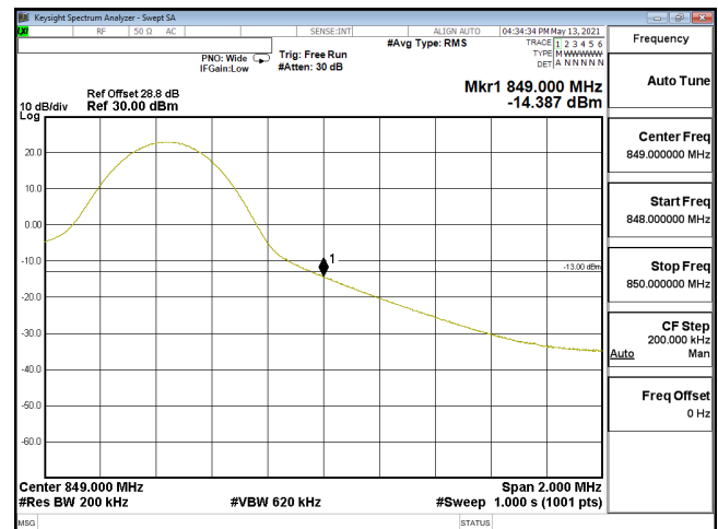
EDGE-ENDC_30A_n5-QPSK_20M_CH167800_839(1,105)_SCS15KHz
