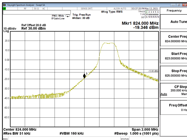
EDGE-ENDC_30A_n5-16QAM_5M_CH165300_826.5(1,0)_SCS15KHz
