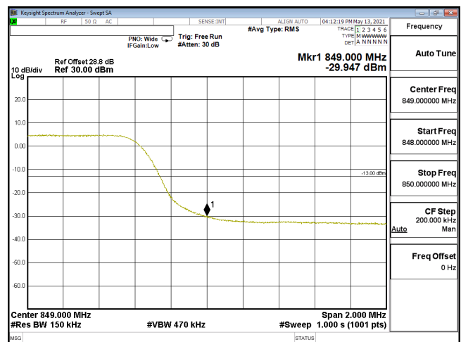
EDGE-ENDC_30A_n5-PI2-BPSK_15M_CH168300_841.5(75,4)_SCS15KHz
