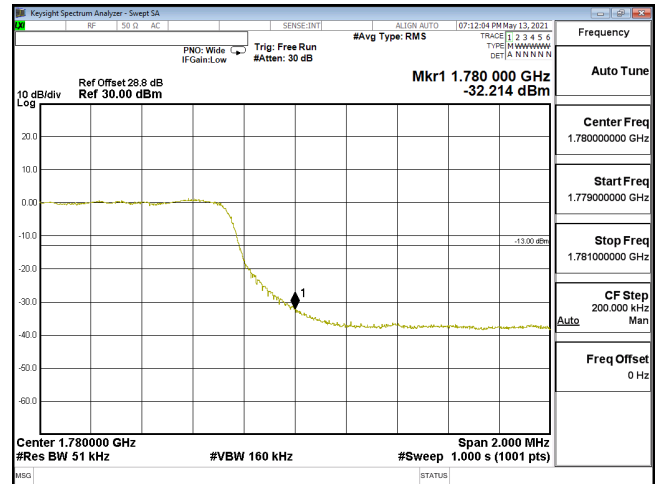
EDGE-ENDC_12A_n66-256QAM_5M_CH355500_1777.5(25,0)_SCS15KHz
