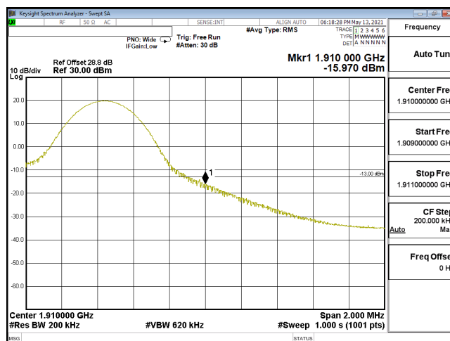
EDGE-ENDC_5A_n2-16QAM_20M_CH380000_1900(1,105)_SCS15KHz
