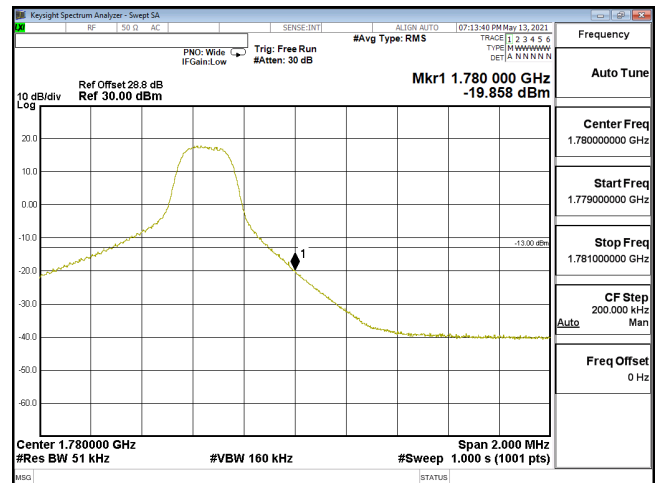
EDGE-ENDC_12A_n66-QPSK_5M_CH355500_1777.5(1,24)_SCS15KHz
