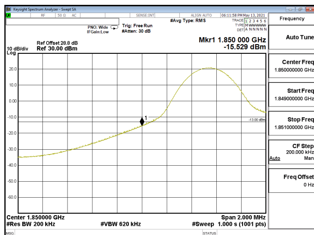
EDGE-ENDC_5A_n2-16QAM_20M_CH372000_1860(1,0)_SCS15KHz
