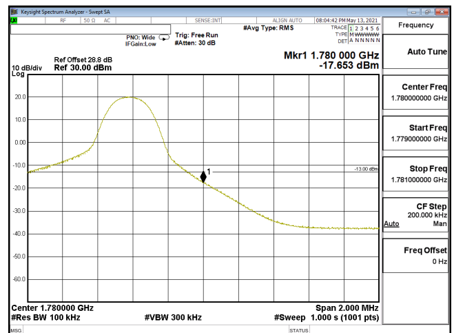
EDGE-ENDC_12A_n66-QPSK_10M_CH355000_1715(1,51)_SCS15KHz
