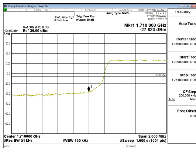
EDGE-ENDC_12A_n66-16QAM_5M_CH342500_1712.5(25,0)_SCS15KHz
