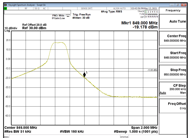
EDGE-ENDC_30A_n5-16QAM_5M_CH169300_846.5(1,24)_SCS15KHz
