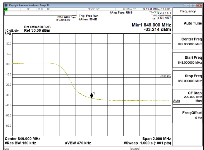
EDGE-ENDC_30A_n5-256QAM_15M_CH168300_841.5(75,4)_SCS15KHz
