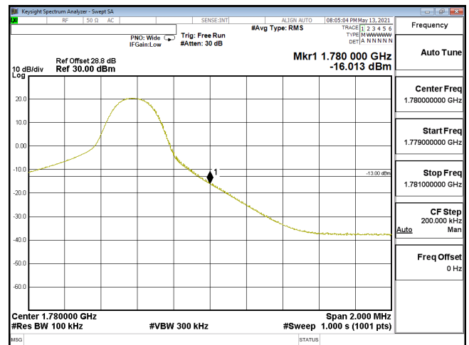
EDGE-ENDC_12A_n66-PI2-BPSK_10M_CH355000_1715(1,51)_SCS15KHz
