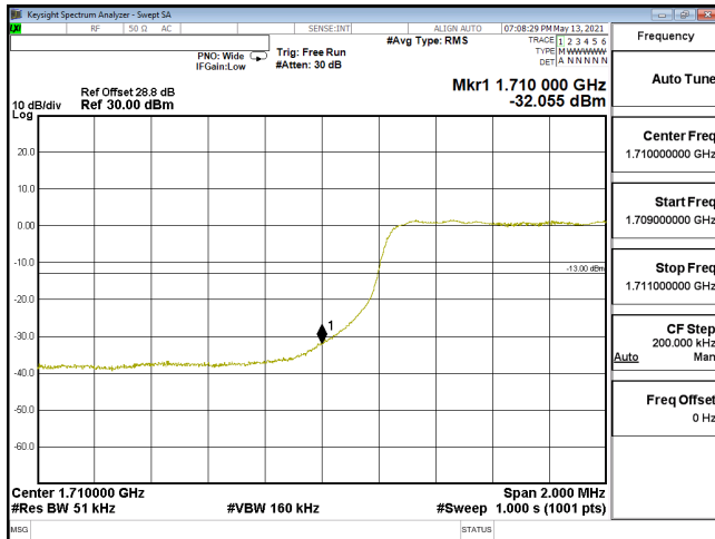
EDGE-ENDC_12A_n66-256QAM_5M_CH342500_1712.5(25,0)_SCS15KHz
