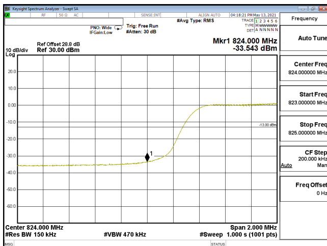
EDGE-ENDC_30A_n5-256QAM_15M_CH166300_831.5(75,0)_SCS15KHz
