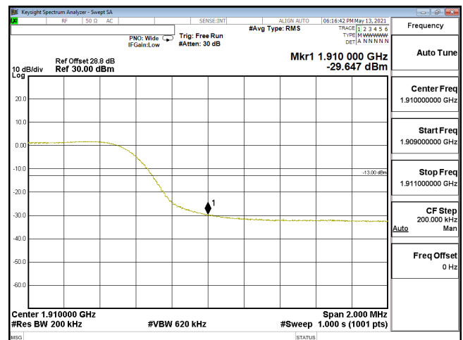
EDGE-ENDC_5A_n2-64QAM_20M_CH380000_1900(100,6)_SCS15KHz
