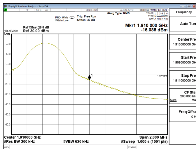
EDGE-ENDC_5A_n2-QPSK_20M_CH380000_1900(1,105)_SCS15KHz
