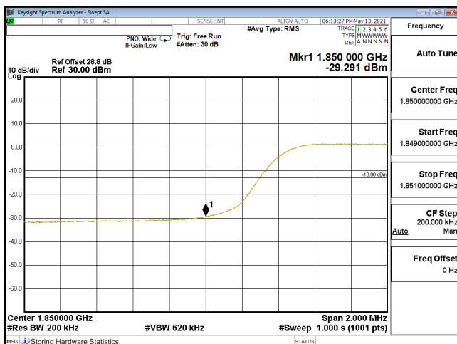
EDGE-ENDC_5A_n2-64QAM_20M_CH372000_1860(100,0)_SCS15KHz
