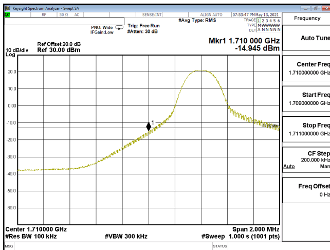
EDGE-ENDC_12A_n66-PI2-BPSK_10M_CH343000_1715(1,0)_SCS15KHz
