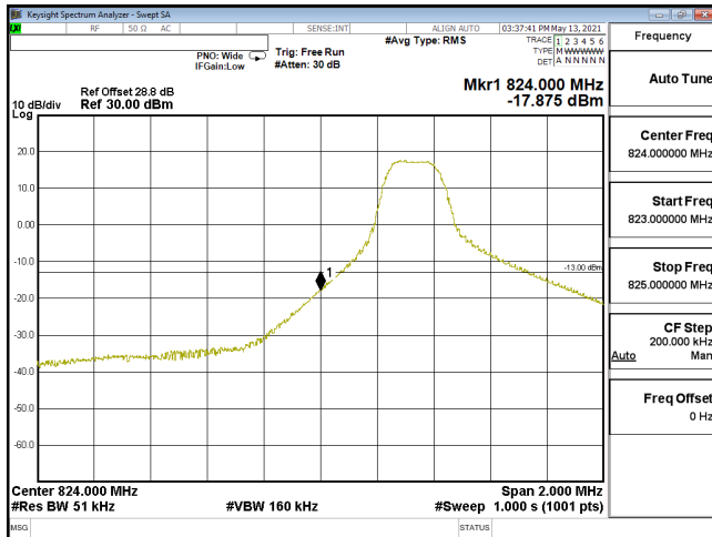
EDGE-ENDC_30A_n5-64QAM_5M_CH165300_826.5(1,0)_SCS15KHz
