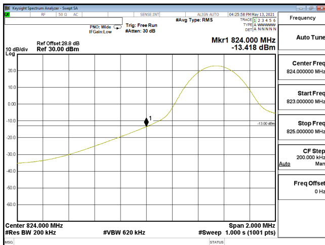
EDGE-ENDC_30A_n5-QPSK_20M_CH166800_834(1,0)_SCS15KHz
