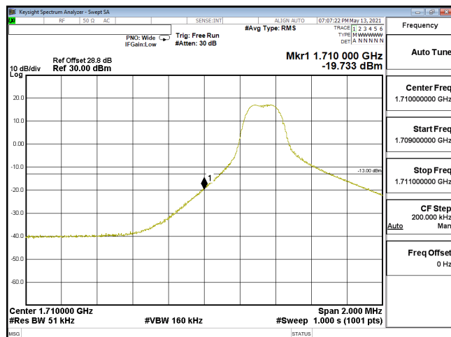
EDGE-ENDC_12A_n66-16QAM_5M_CH342500_1712.5(1,0)_SCS15KHz
