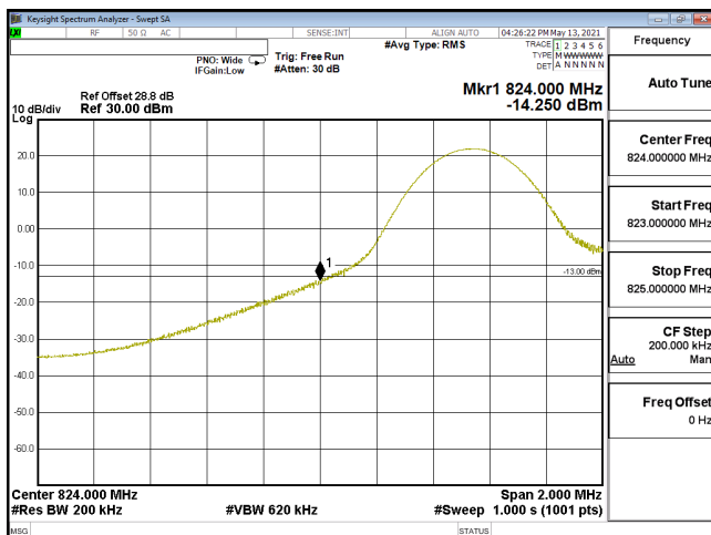
EDGE-ENDC_30A_n5-16QAM_20M_CH166800_834(1,0)_SCS15KHz
