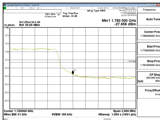
EDGE-ENDC_12A_n66-QPSK_5M_CH355500_1777.5(25,0)_SCS15KHz
