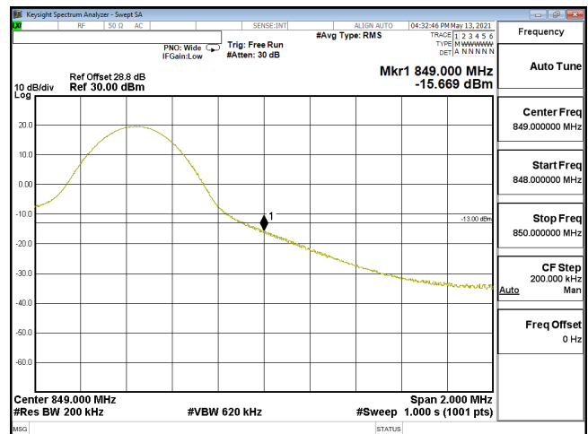
EDGE-ENDC_30A_n5-256QAM_20M_CH167800_839(1,105)_SCS15KHz
