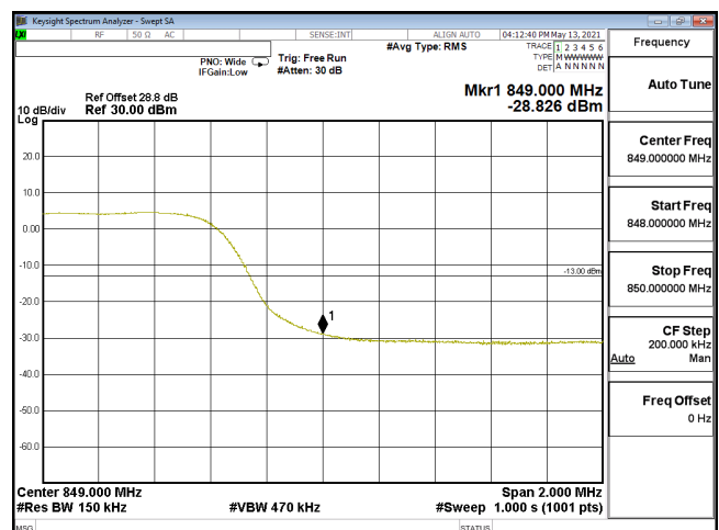
EDGE-ENDC_30A_n5-QPSK_15M_CH168300_841.5(75,4)_SCS15KHz
