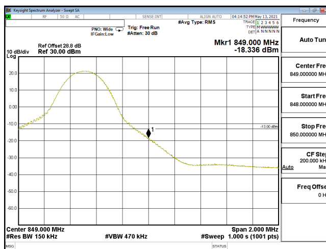
EDGE-ENDC_30A_n5-16QAM_15M_CH168300_841.5(1,78)_SCS15KHz
