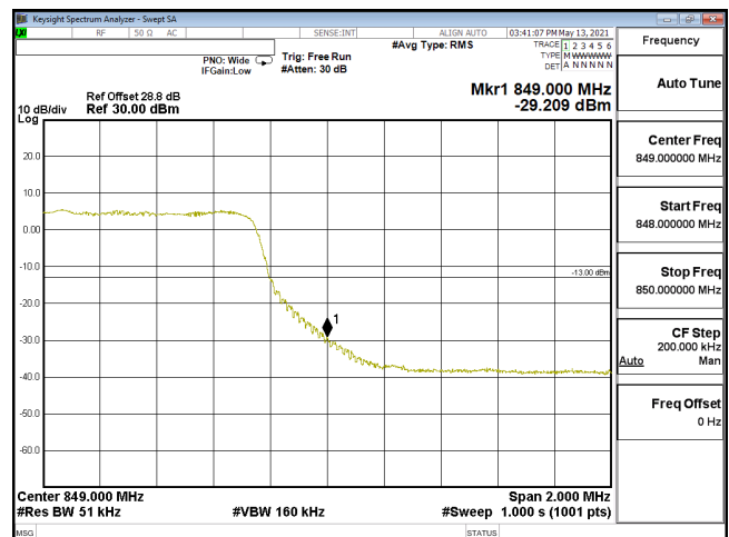
EDGE-ENDC_30A_n5-PI2-BPSK_5M_CH169300_846.5(25,0)_SCS15KHz
