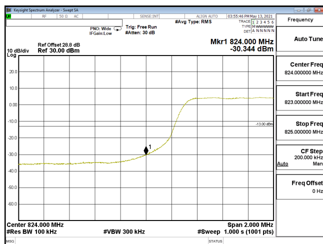
EDGE-ENDC_30A_n5-QPSK_10M_CH165800_829(50,0)_SCS15KHz
