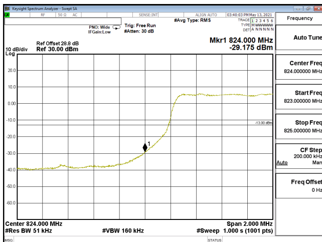
EDGE-ENDC_30A_n5-PI2-BPSK_5M_CH165300_826.5(25,0)_SCS15KHz
