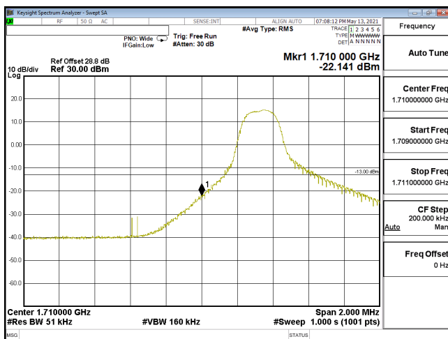
EDGE-ENDC_12A_n66-256QAM_5M_CH342500_1712.5(1,0)_SCS15KHz
