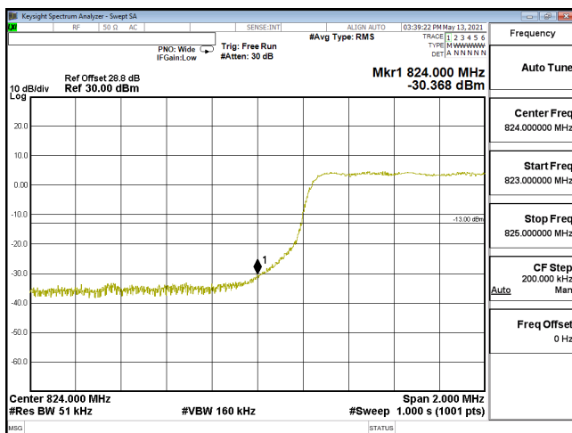
EDGE-ENDC_30A_n5-16QAM_5M_CH165300_826.5(25,0)_SCS15KHz
