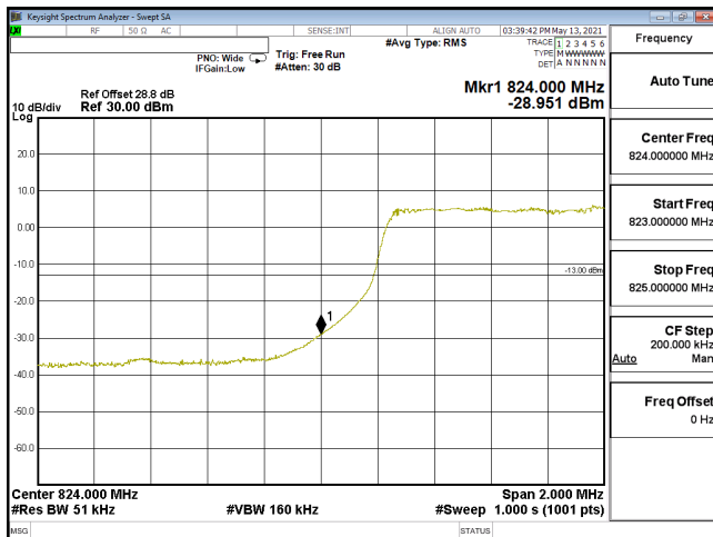
EDGE-ENDC_30A_n5-QPSK_5M_CH165300_826.5(25,0)_SCS15KHz
