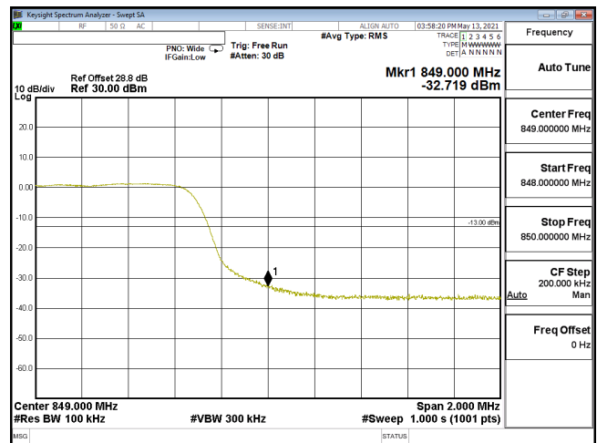
EDGE-ENDC_30A_n5-256QAM_10M_CH168800_844(50,2)_SCS15KHz
