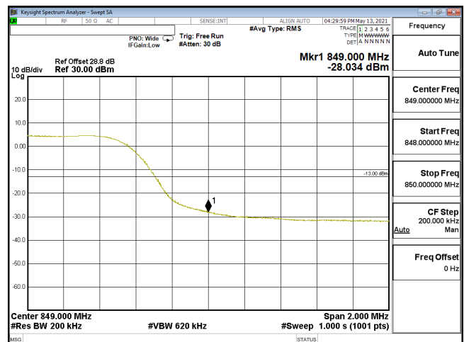
EDGE-ENDC_30A_n5-PI2-BPSK_20M_CH167800_839(100,6)_SCS15KHz
