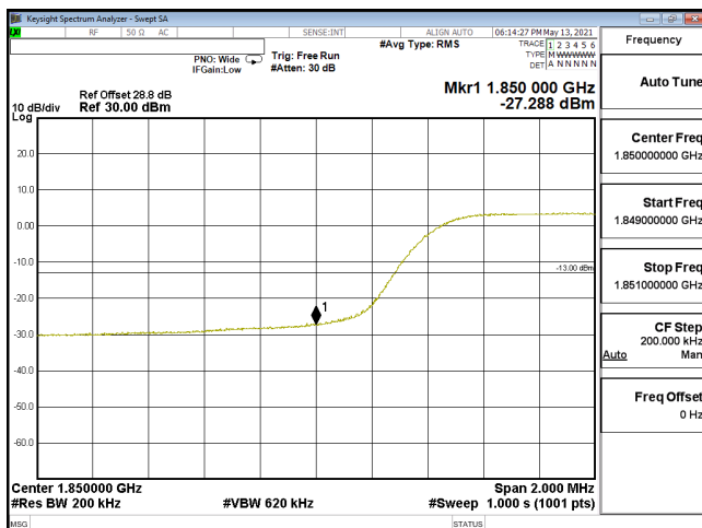
EDGE-ENDC_5A_n2-256QAM_20M_CH372000_1860(1,0)_SCS15KHz
