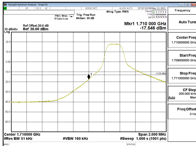
EDGE-ENDC_12A_n66-QPSK_5M_CH342500_1712.5(1,0)_SCS15KHz
