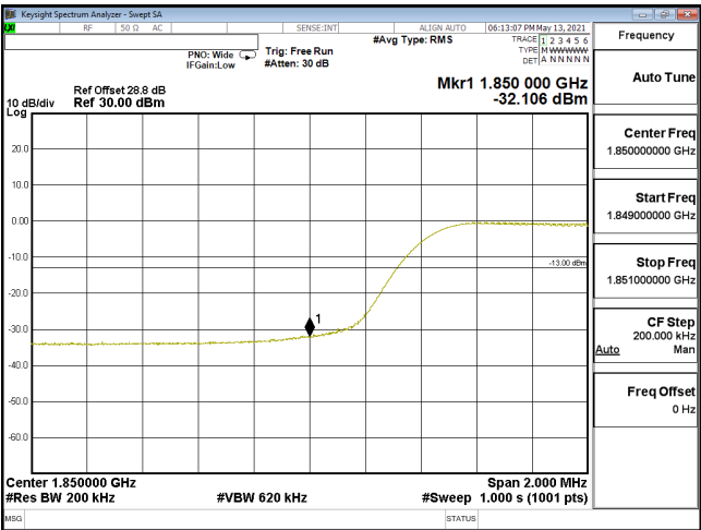
EDGE-ENDC_5A_n2-256QAM_20M_CH372000_1860(100,0)_SCS15KHz
