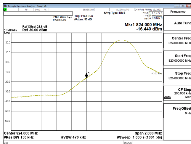
EDGE-ENDC_30A_n5-QPSK_15M_CH166300_831.5(1,0)_SCS15KHz
