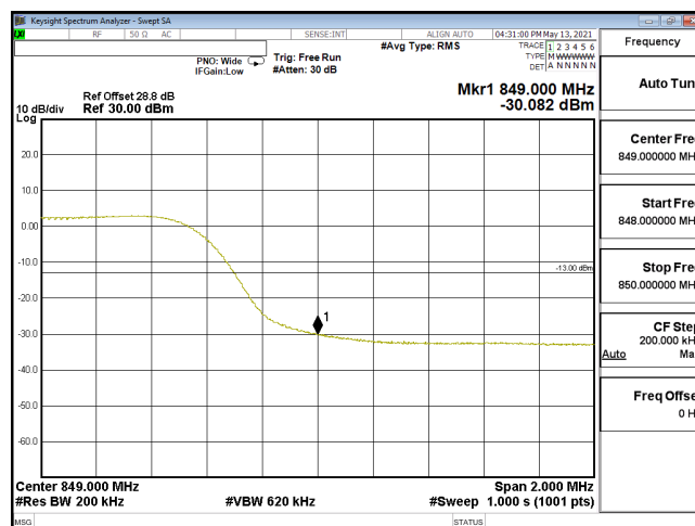
EDGE-ENDC 30A n5-64QAM 20M CH167800 839(100,6) SCS15KHz
