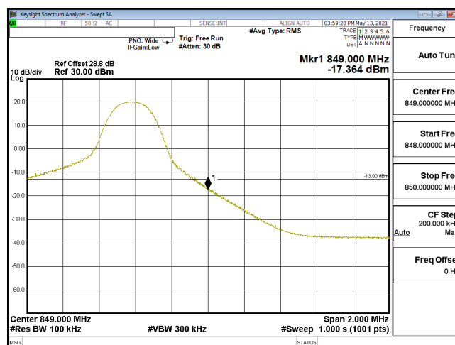
EDGE-ENDC_30A_n5-16QAM_10M_CH168800_844(1,51)_SCS15KHz
