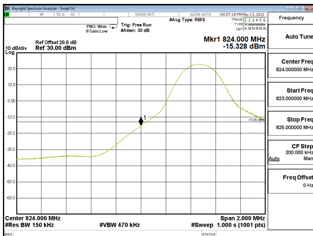
EDGE-ENDC_30A_n5-PI2-BPSK_15M_CH166300_831.5(1,0)_SCS15KHz
