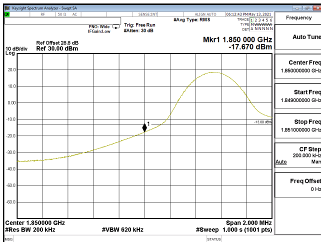
EDGE-ENDC_5A_n2-64QAM_20M_CH372000_1860(1,0)_SCS15KHz
