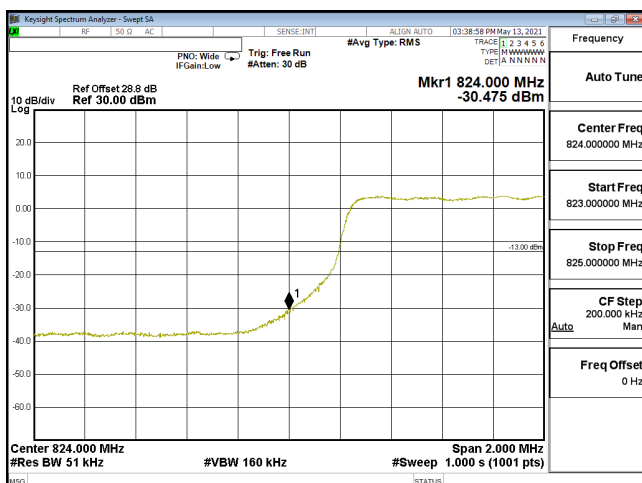
EDGE-ENDC_30A_n5-64QAM_5M_CH165300_826.5(25,0)_SCS15KHz
