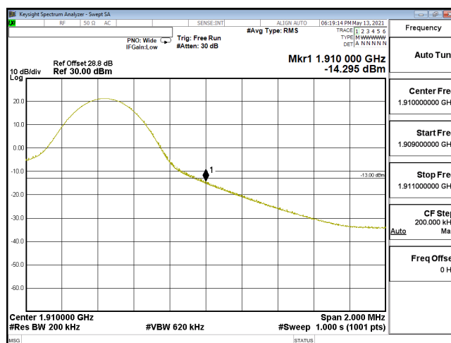
EDGE-ENDC_5A_n2-PI2-BPSK_20M_CH380000_1900(1,105)_SCS15KHz
