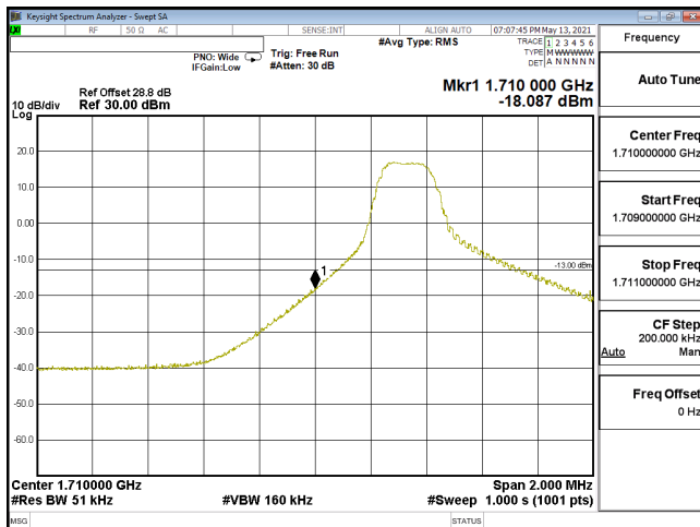
EDGE-ENDC_12A_n66-64QAM_5M_CH342500_1712.5(1,0)_SCS15KHz
