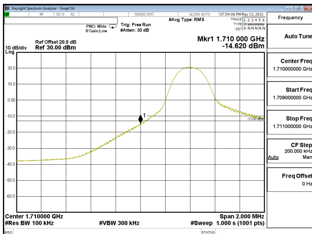
EDGE-ENDC_12A_n66-QPSK_10M_CH343000_1715(1,0)_SCS15KHz
