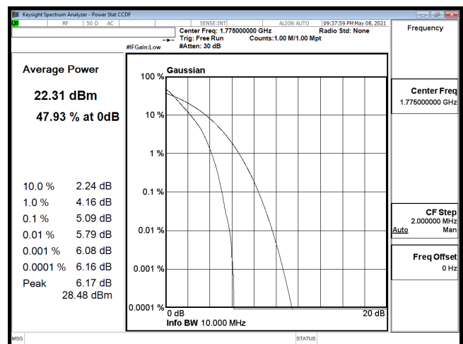
PTAR-B66_10M-CH132622-16QAM
