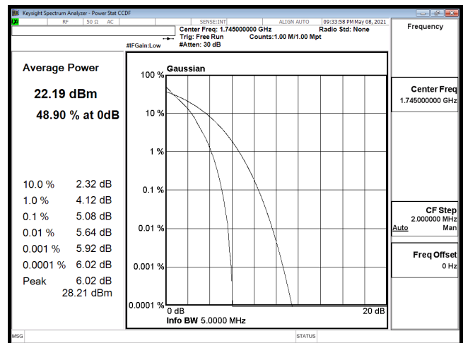
PTAR-B66_5M-CH132322-QPSK
