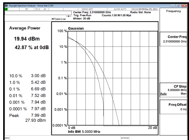
PTAR-B30_5M-CH27710-64QAM
