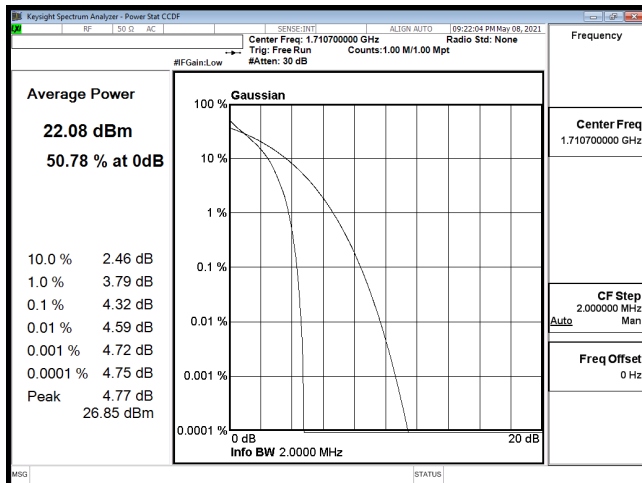
PTAR-B66_1.4M-CH131979-QPSK
