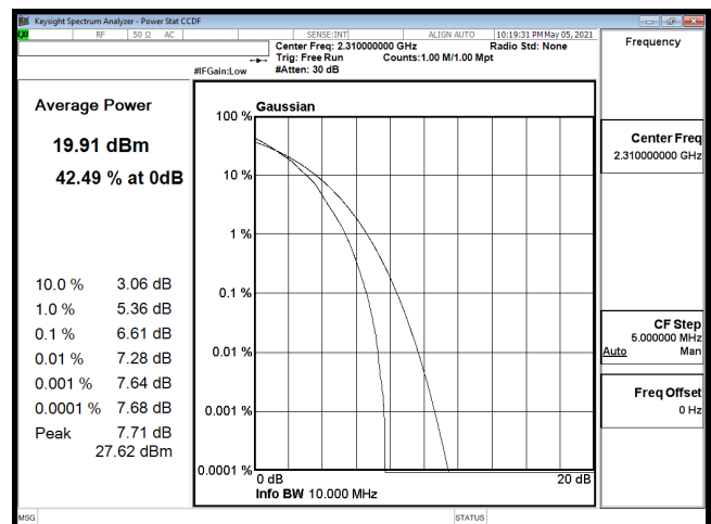
PTAR-B30_10M-CH27710-64QAM
