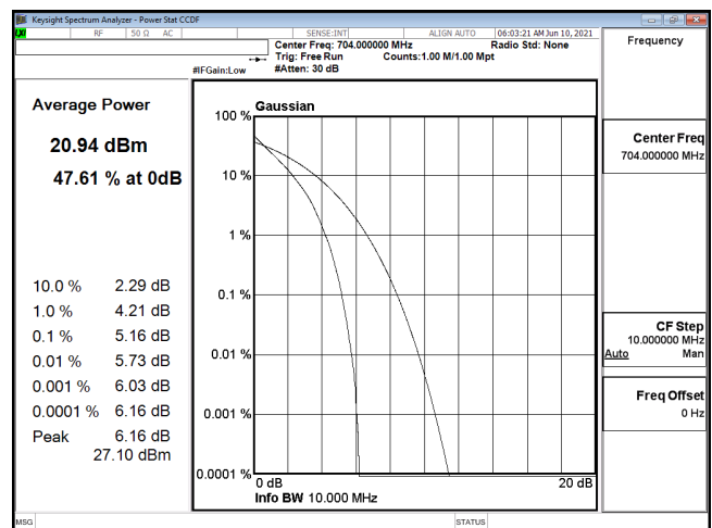
PTAR-B12_10M-CH23060-QPSK
