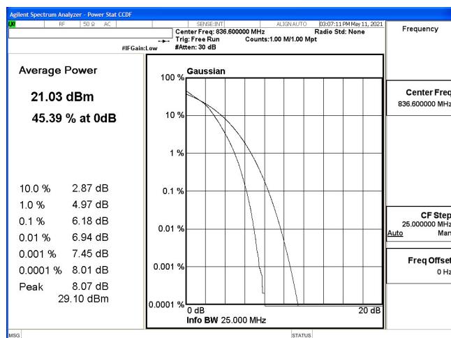
PTAR(10M+10M)-2ULCA_5B-16QAM_831.6(50,0)+841.5(50,0)
