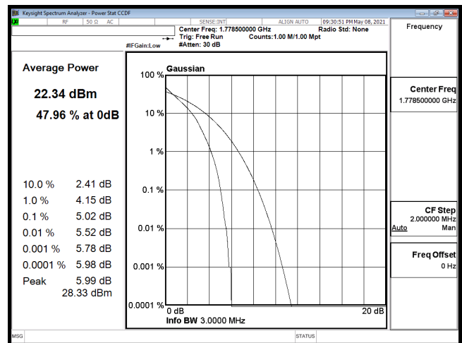
PTAR-B66_3M-CH132657-QPSK
