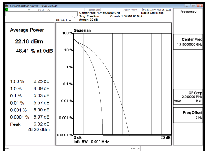
PTAR-B66_10M-CH132022-QPSK
