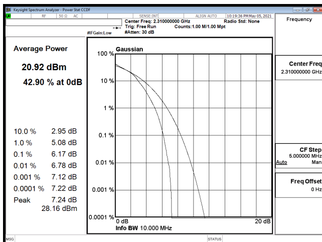
PTAR-B30_10M-CH27710-16QAM
