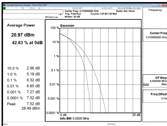
PTAR-B30_5M-CH27710-16QAM
