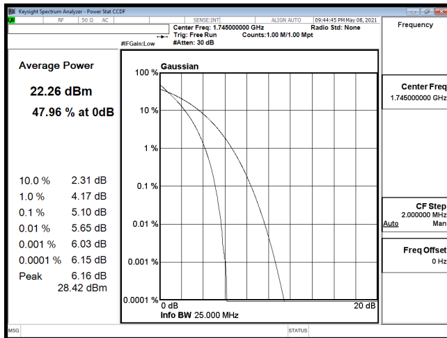
PTAR-B66_20M-CH132322-QPSK
