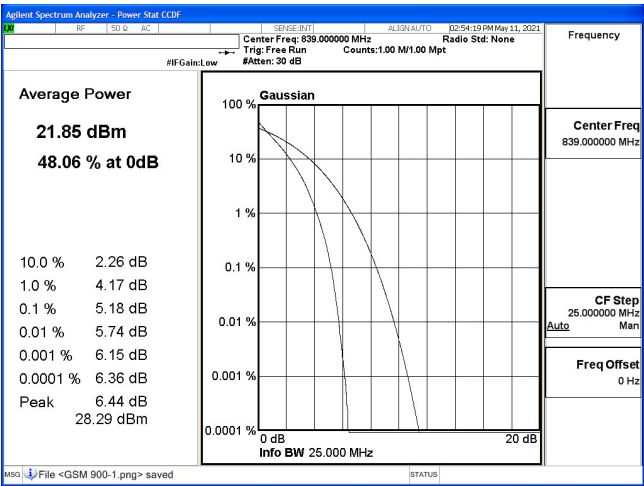
PTAR(10M+10M)-2ULCA_5B-QPSK_834.1(50,0)+844(50,0)
