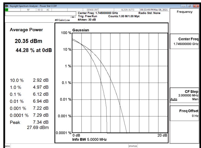
PTAR-B66_5M-CH132322-64QAM
