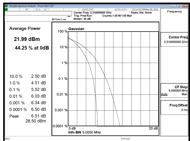
PTAR-B30_5M-CH27710-QPSK
