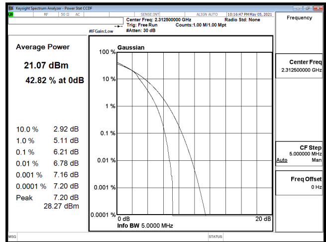
PTAR-B30_5M-CH27735-16QAM
