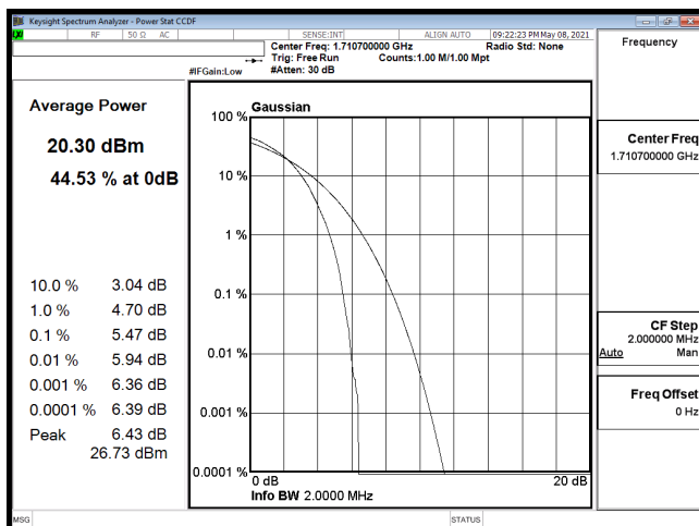
PTAR-B66_1.4M-CH131979-64QAM
