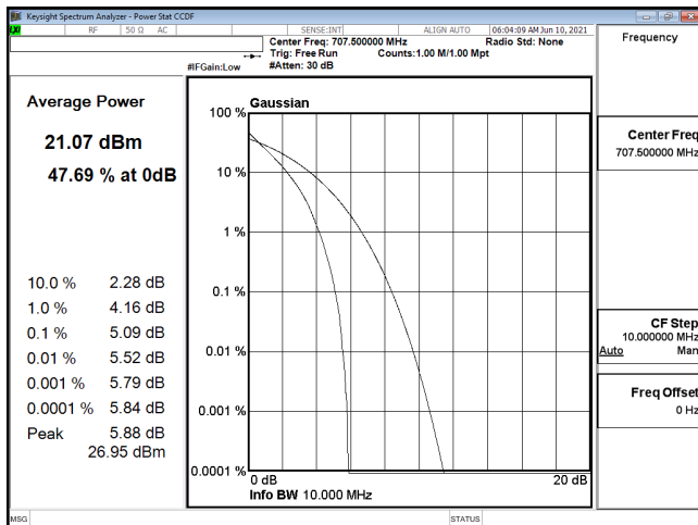
PTAR-B12_10M-CH23095-QPSK
