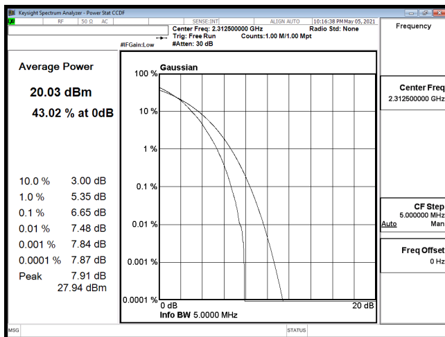
PTAR-B30_5M-CH27735-64QAM
