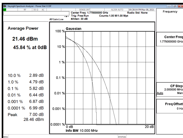
PTAR-B66_10M-CH132622-QPSK
