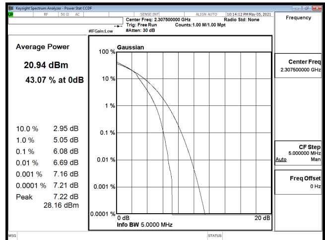
PTAR-B30_5M-CH27685-16QAM
