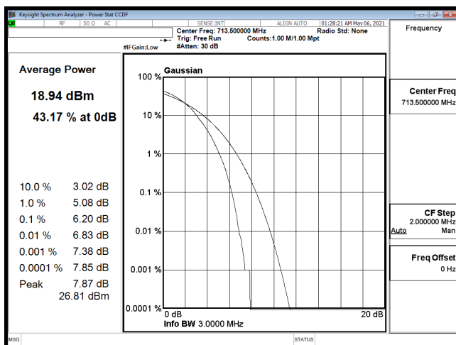
PTAR-B12_5M-CH23155-64QAM
