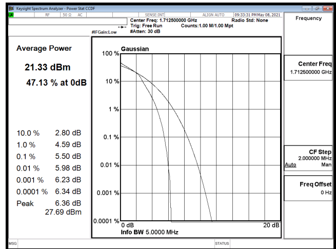
PTAR-B66_5M-CH131997-16QAM
