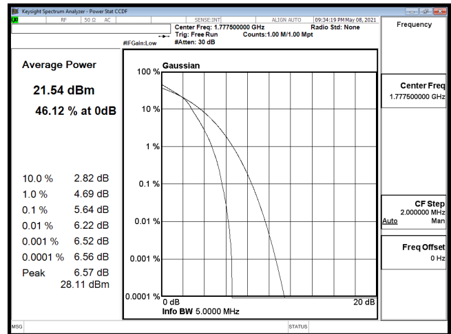
PTAR-B66_5M-CH132647-16QAM
