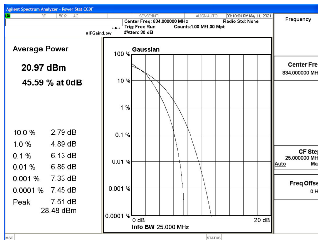
PTAR(10M+10M)-2ULCA_5B-16QAM_829(50,0)+838.9(50,0)
