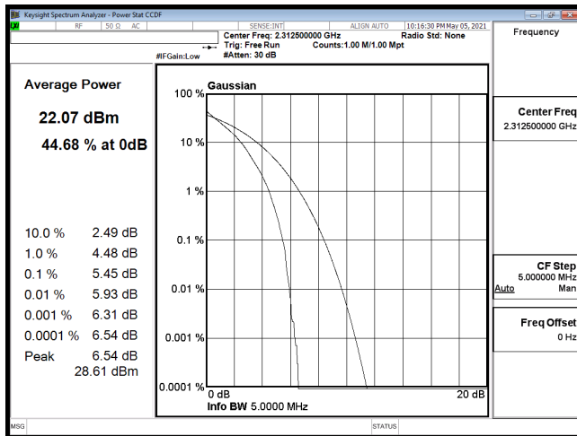
PTAR-B30_5M-CH27735-QPSK
