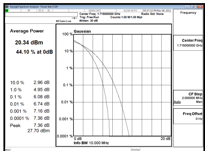
PTAR-B66_10M-CH132022-64QAM
