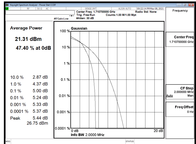
PTAR-B66_1.4M-CH131979-16QAM
