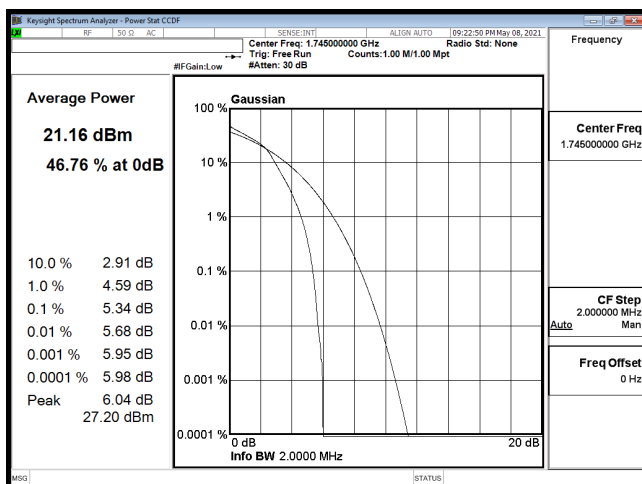
PTAR-B66_1.4M-CH132322-16QAM
