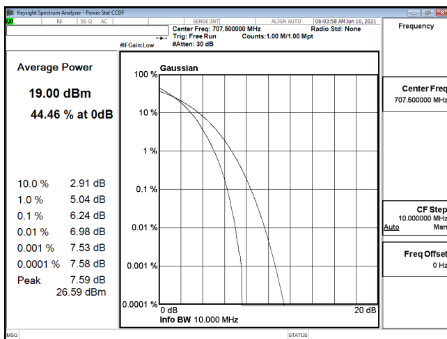
PTAR-B12_10M-CH23095-64QAM
