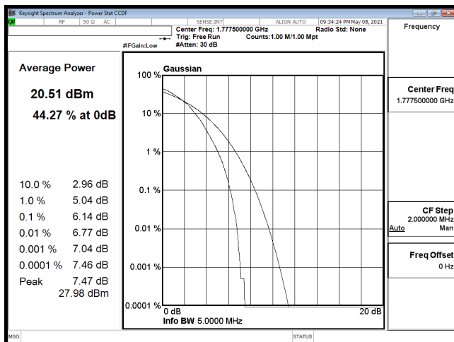
PTAR-B66_5M-CH132647-64QAM
