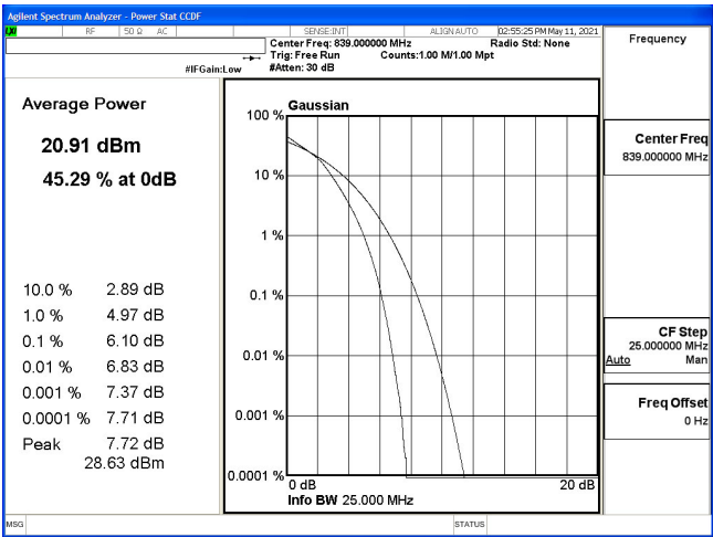
PTAR(10M+10M)-2ULCA_5B-16QAM_834.1(50,0)+844(50,0)
