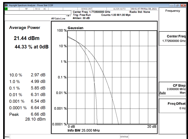
PTAR-B66_15M-CH132597-16QAM
