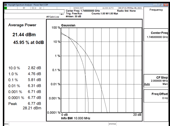
PTAR-B66_10M-CH132322-16QAM
