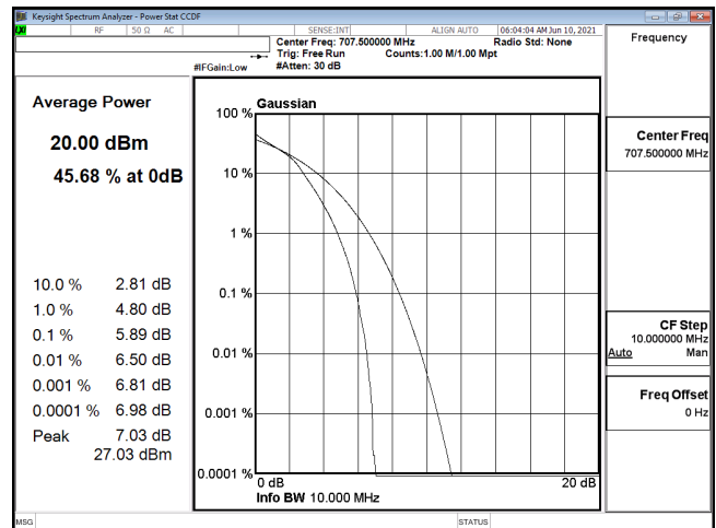
PTAR-B12_10M-CH23095-16QAM
