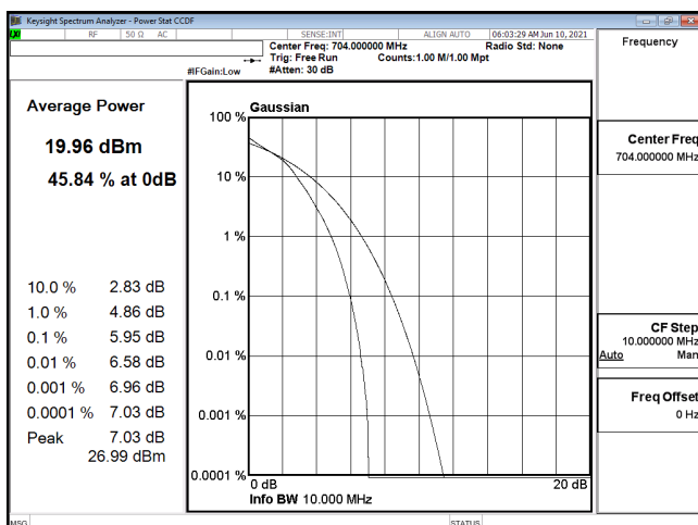
PTAR-B12_10M-CH23060-16QAM
