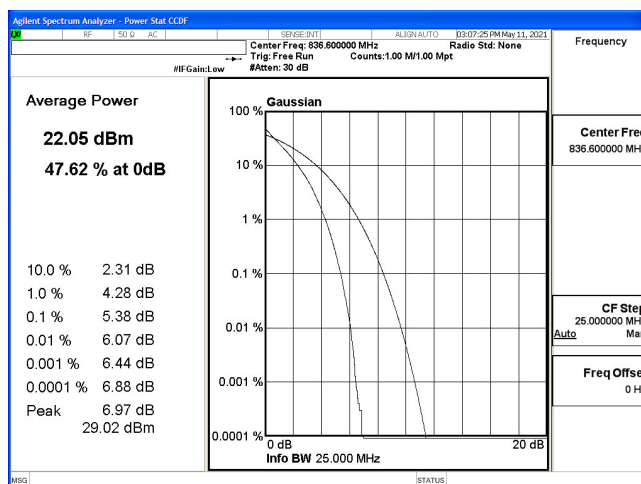
PTAR(10M+10M)-2ULCA_5B-QPSK_831.6(50,0)+841.5(50,0)
