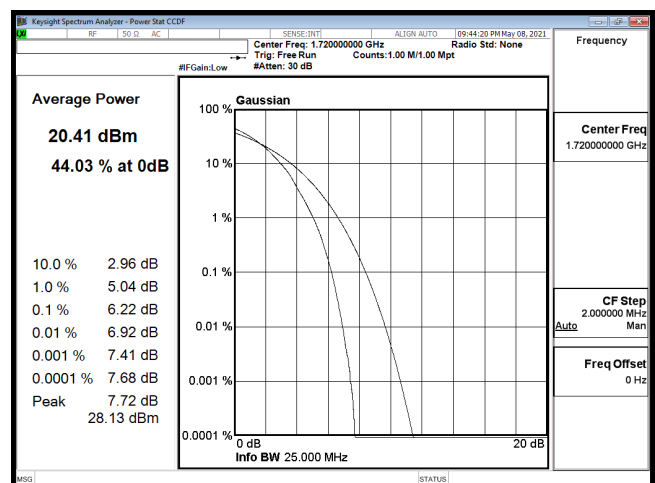
PTAR-B66_20M-CH132072-64QAM
