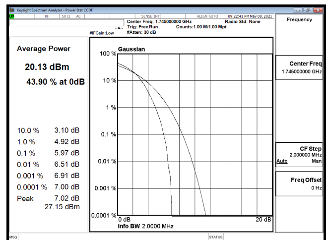
PTAR-B66_1.4M-CH132322-64QAM
