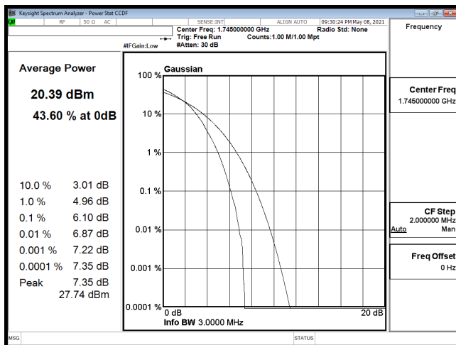
PTAR-B66_3M-CH132322-64QAM
