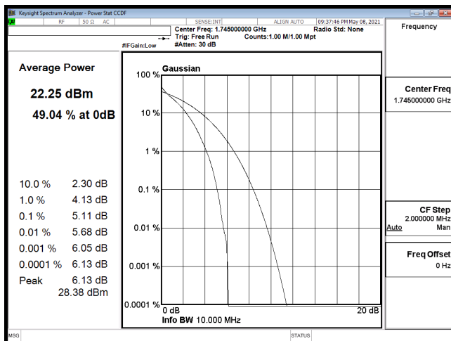
PTAR-B66_10M-CH132322-QPSK
