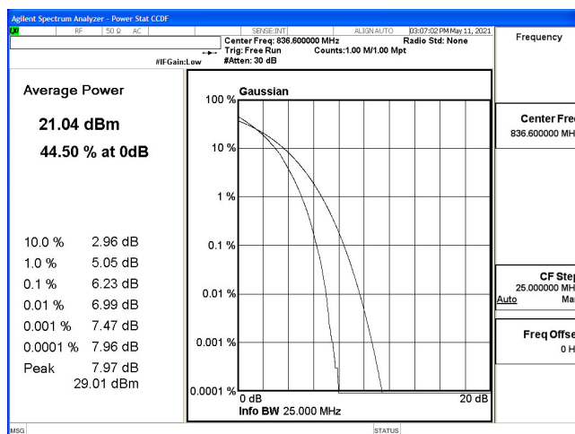
PTAR(10M+10M)-2ULCA_5B-64QAM_831.6(50,0)+841.5(50,0)
