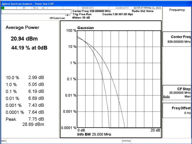
PTAR(10M+10M)-2ULCA_5B-64QAM_834.1(50,0)+844(50,0)
