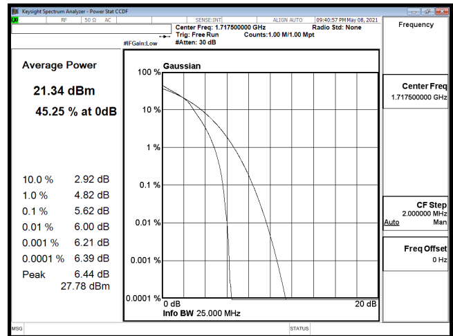
PTAR-B66_15M-CH132047-16QAM
