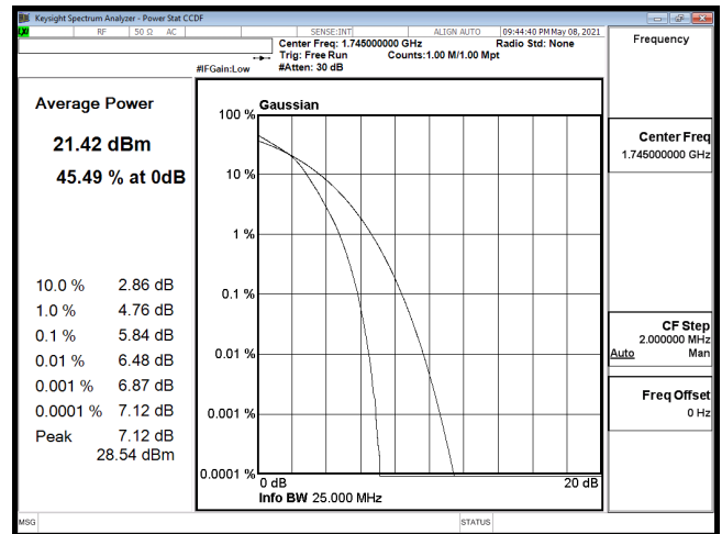
PTAR-B66_20M-CH132322-16QAM
