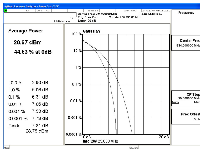
PTAR(10M+10M)-2ULCA_5B-64QAM_829(50,0)+838.9(50,0)
