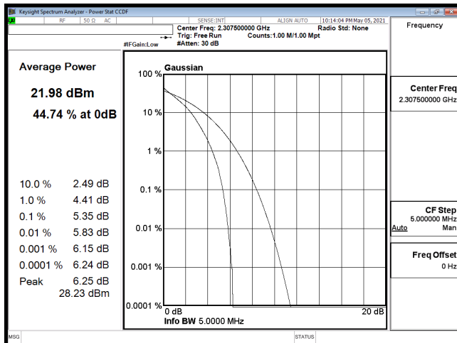
PTAR-B30_5M-CH27685-QPSK
