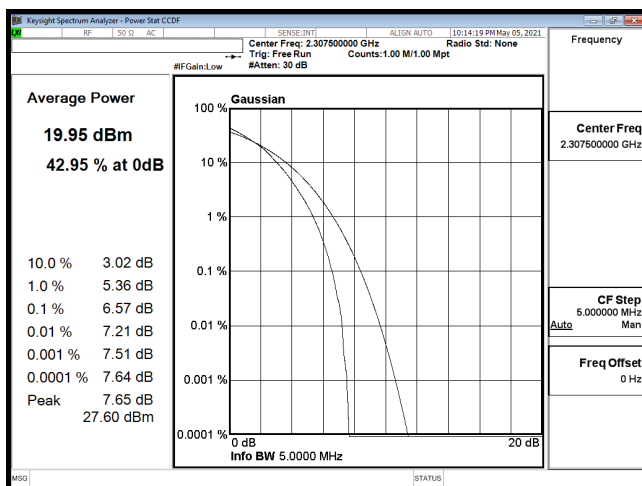
PTAR-B30_5M-CH27685-64QAM
