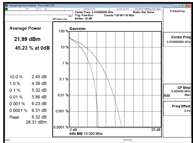
PTAR-B30_10M-CH27710-QPSK
