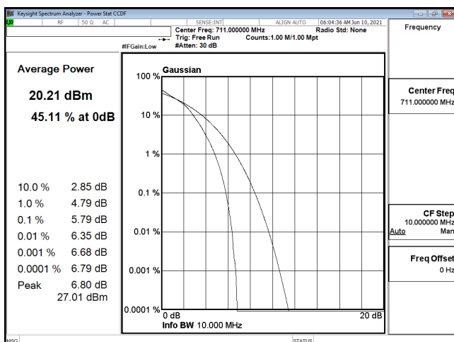
PTAR-B12_10M-CH23130-16QAM
