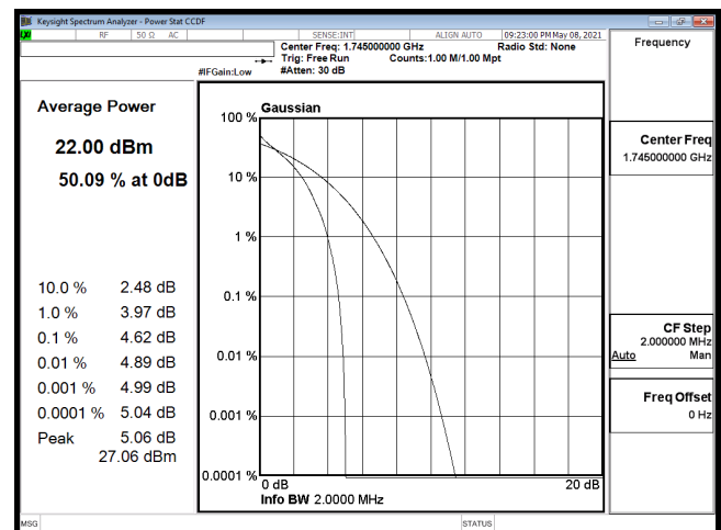
PTAR-B66_1.4M-CH132322-QPSK
