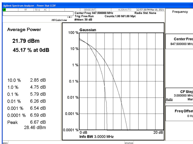
PTAR-B5_3M-CH20635-16QAM
