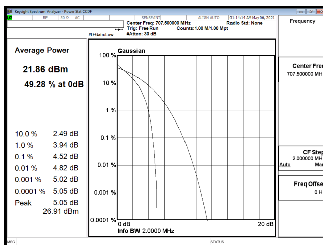
PTAR-B12_1.4M-CH23095-QPSK
