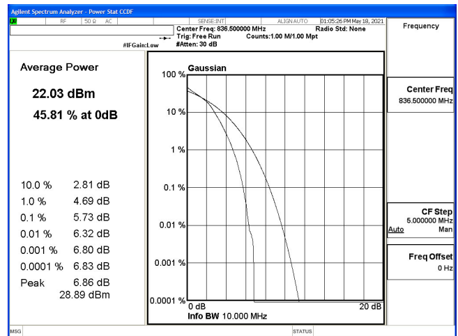
PTAR-B5_10M-CH20525-16QAM
