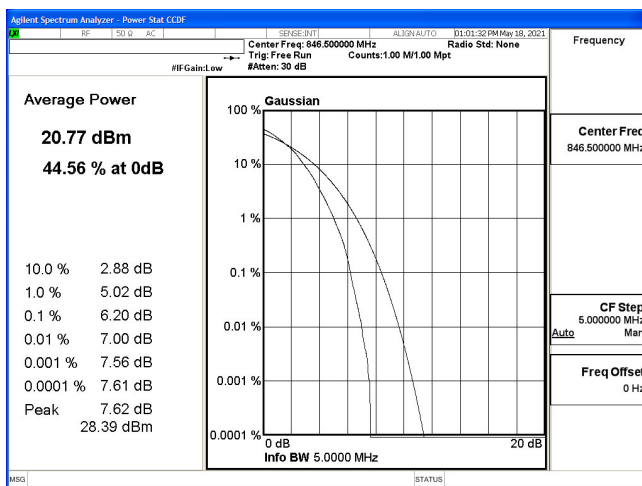
PTAR-B5_5M-CH20625-64QAM
