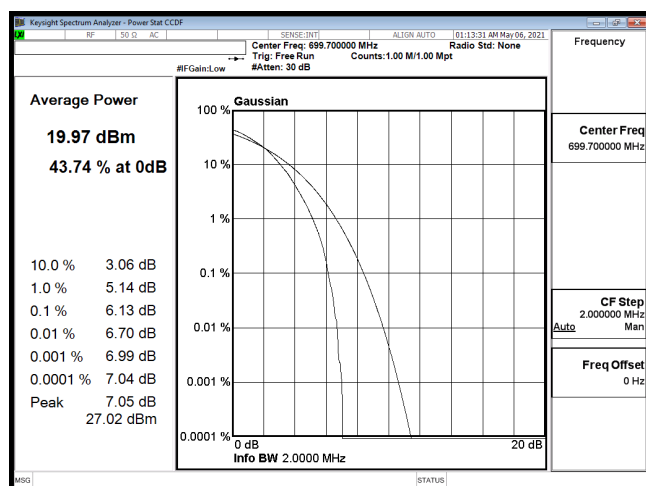
PTAR-B12_1.4M-CH23017-64QAM
