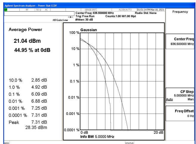
PTAR-B5_5M-CH20525-64QAM
