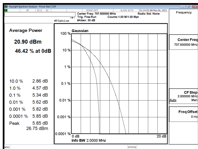
PTAR-B12_1.4M-CH23095-16QAM
