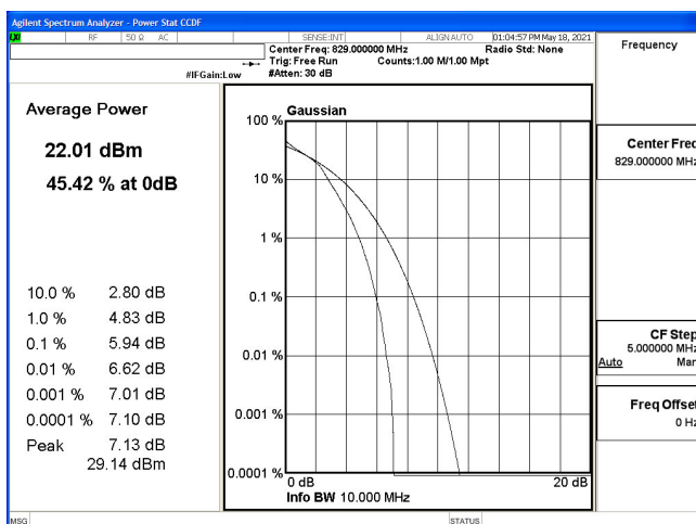
PTAR-B5_10M-CH20450-16QAM
