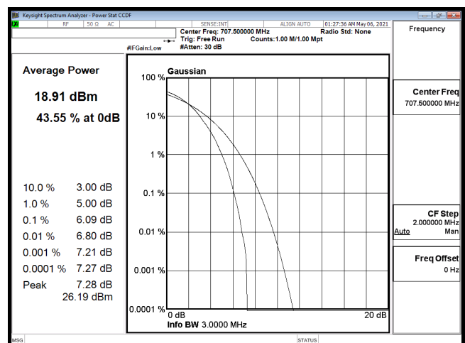
PTAR-B12_5M-CH23095-16QAM
