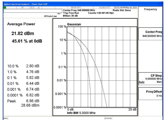
PTAR-B5_5M-CH20625-16QAM
