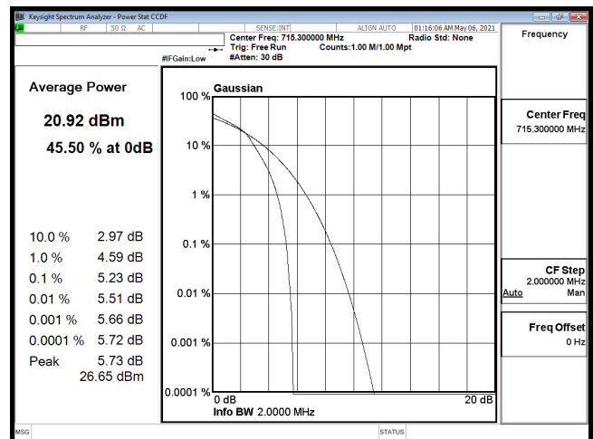
PTAR-B12_1.4M-CH23173-16QAM
