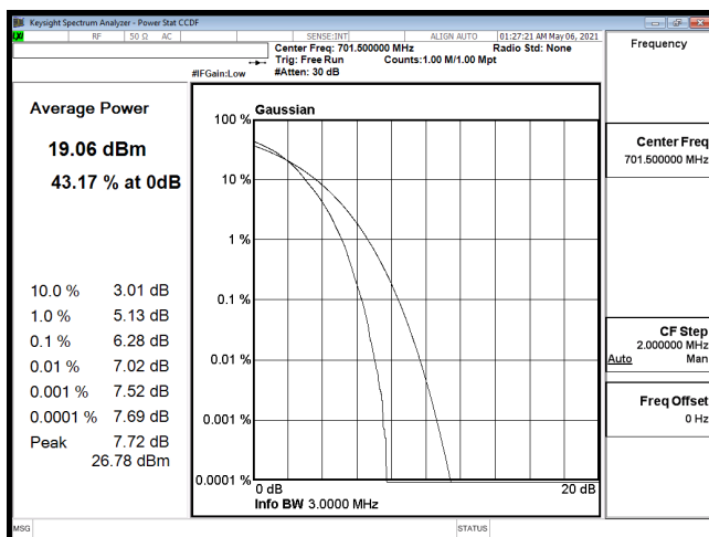
PTAR-B12_5M-CH23035-64QAM
