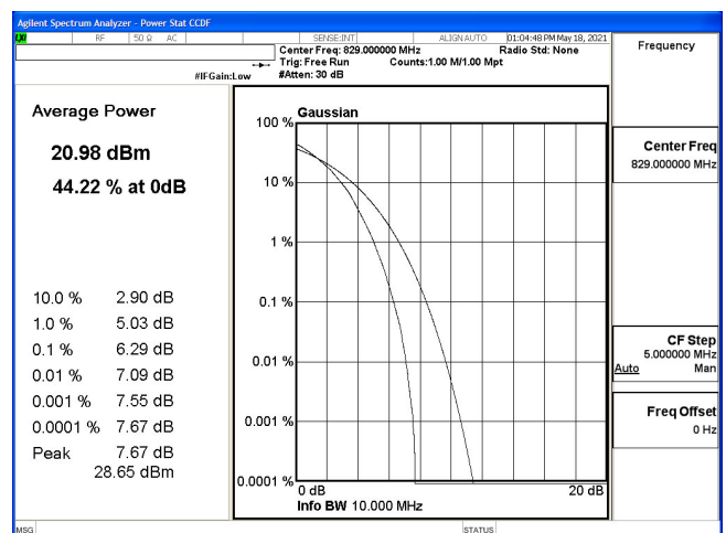
PTAR-B5_10M-CH20450-64QAM
