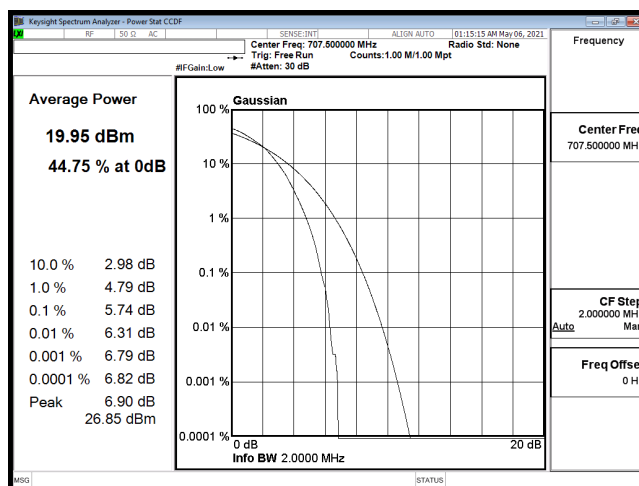
PTAR-B12_1.4M-CH23095-64QAM
