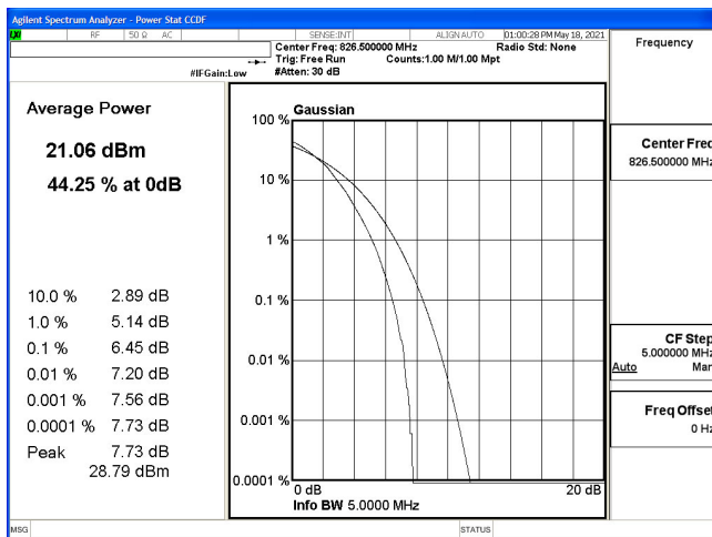
PTAR-B5_5M-CH20425-64QAM
