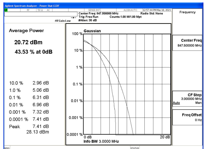
PTAR-B5_3M-CH20635-64QAM
