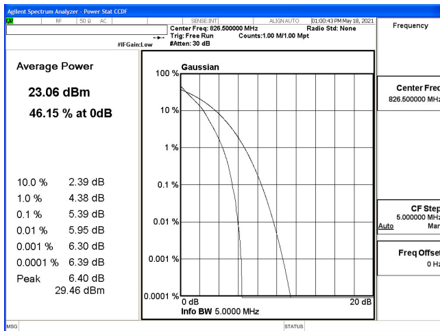
PTAR-B5_5M-CH20425-QPSK
