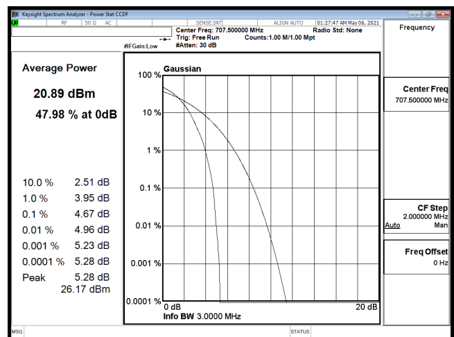
PTAR-B12_5M-CH23095-16QAM
