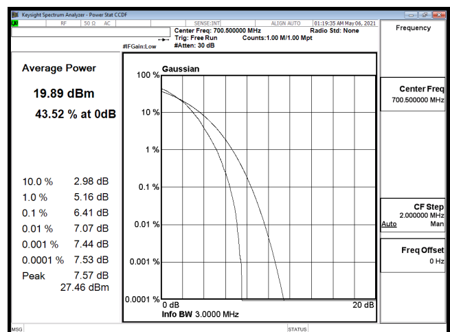
PTAR-B12_3M-CH23025-64QAM
