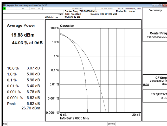
PTAR-B12_1.4M-CH23173-64QAM
