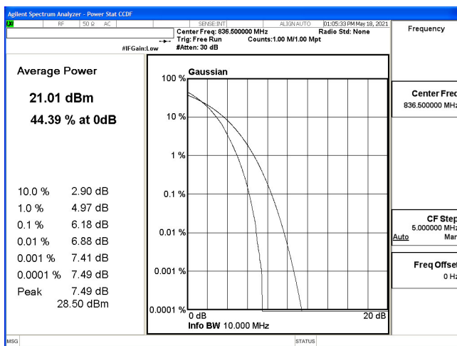
PTAR-B5_10M-CH20525-64QAM
