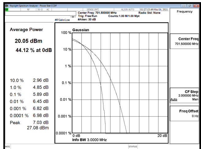
PTAR-B12_5M-CH23035-16QAM
