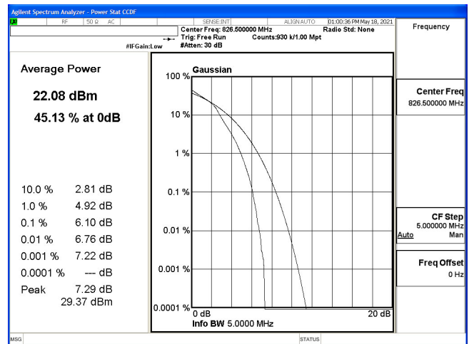
PTAR-B5_5M-CH20425-16QAM
