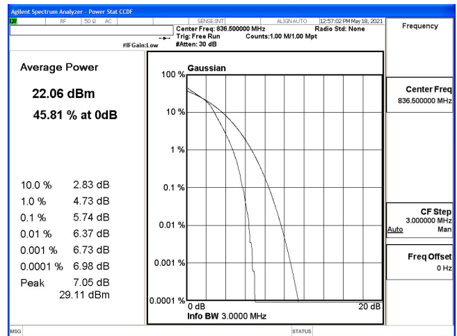
PTAR-B5_3M-CH20525-16QAM
