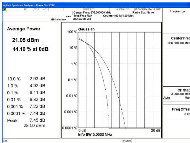
PTAR-B5_3M-CH20525-64QAM
