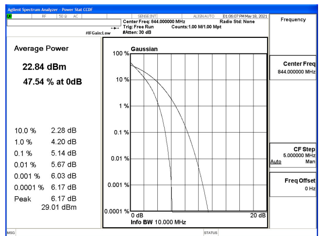
PTAR-B5_10M-CH20600-QPSK
