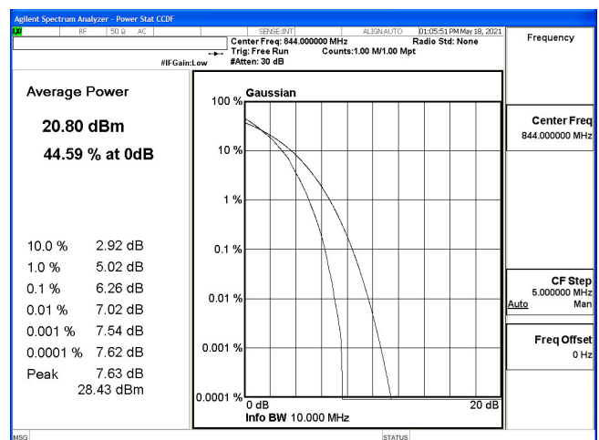
PTAR-B5_10M-CH20600-64QAM
