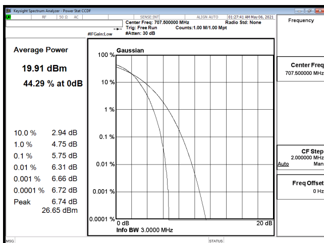
PTAR-B12_5M-CH23095-64QAM
