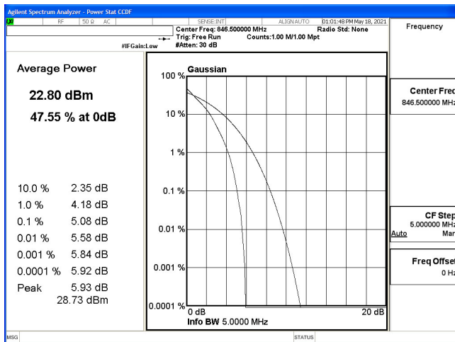
PTAR-B5_5M-CH20625-QPSK
