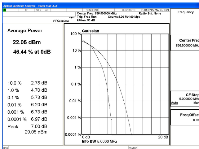
PTAR-B5_5M-CH20525-16QAM
