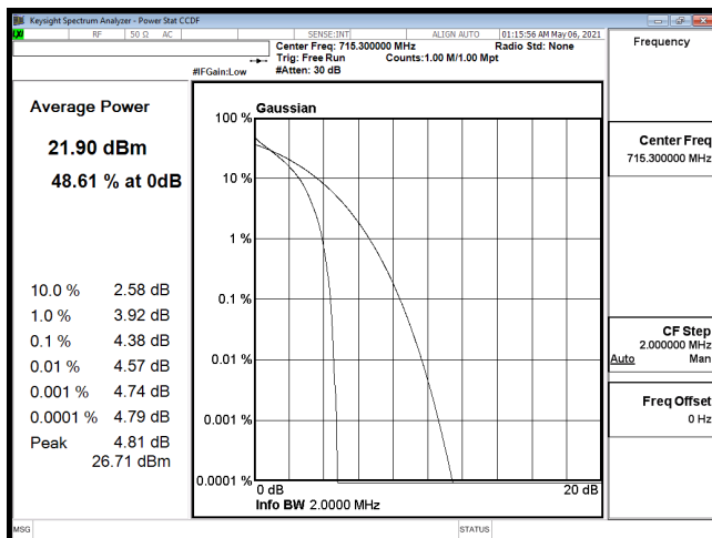
PTAR-B12_1.4M-CH23173-QPSK
