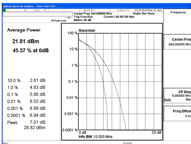
PTAR-B5_10M-CH20600-16QAM
