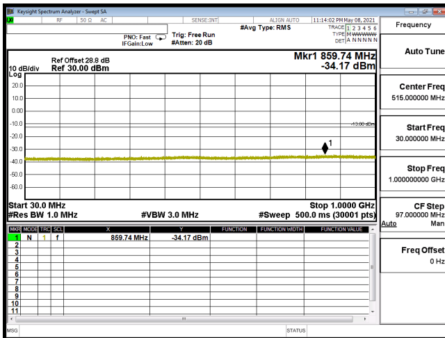
CSE-B66_10M-CH132322-QPSK(1,25)-30M-1G
