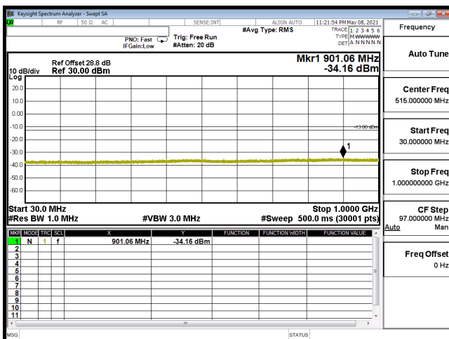
CSE-B66_20M-CH132072-64QAM(1,50)-1G
