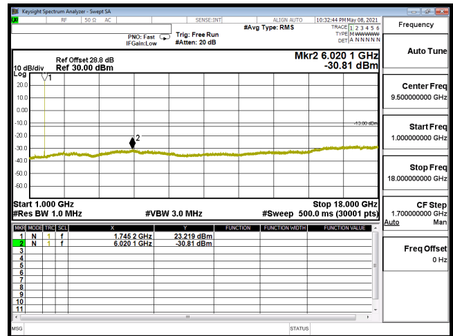
CSE-B66_10M-CH132322-QPSK(1,25)-1G-18G
