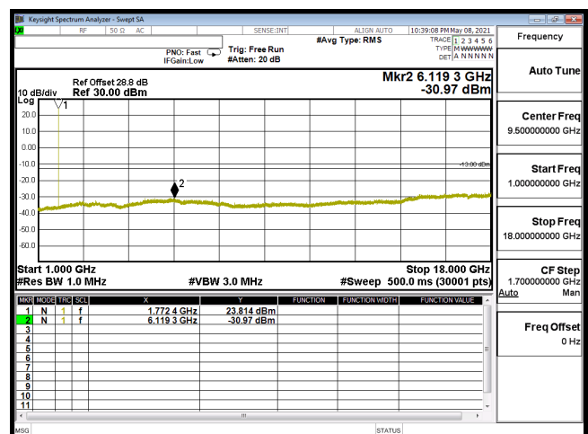
CSE-B66_15M-CH132597-64QAM(1,37)-1G-18G
