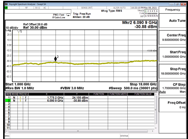
CSE-B66_10M-CH132622-QPSK(1,25)-1G-18G
