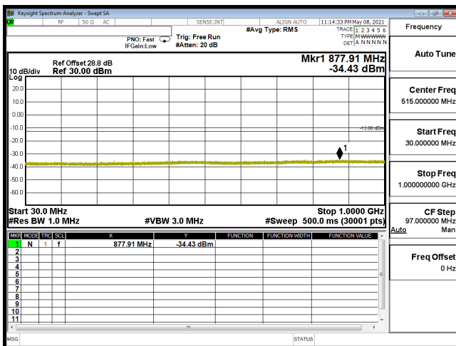
CSE-B66_10M-CH132622-16QAM(1,25)-30M-1G
