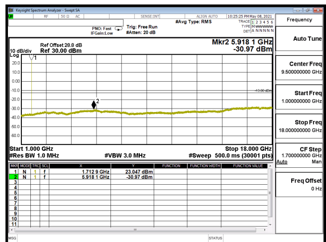
CSE-B66_5M-CH131997-16QAM(1,12)-1G-18G
