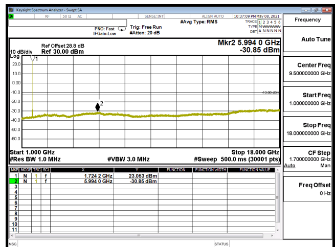
CSE-B66_15M-CH132047-64QAM(1,74)-1G-18G
