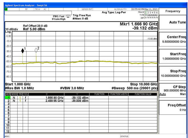
CSE(10M+10M)-2ULCA_5B-64QAM_829(1,49)+838.9(1,0)-1G-10G
