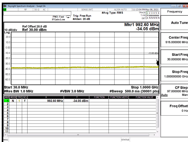
CSE-B66_10M-CH132022-16QAM(1,25)-30M-1G
