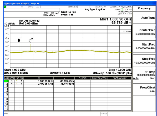
CSE(10M+10M)-2ULCA_5B-QPSK_829(1,49)+838.9(1,0)-1G-10G
