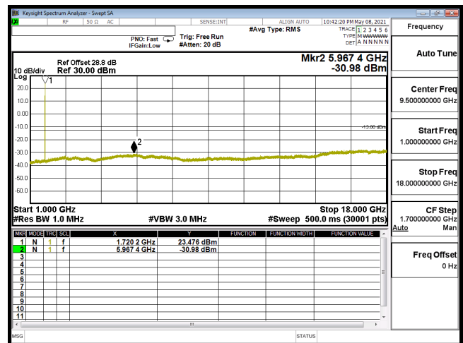
CSE-B66_20M-CH132072-16QAM(1,50)-1G-18G
