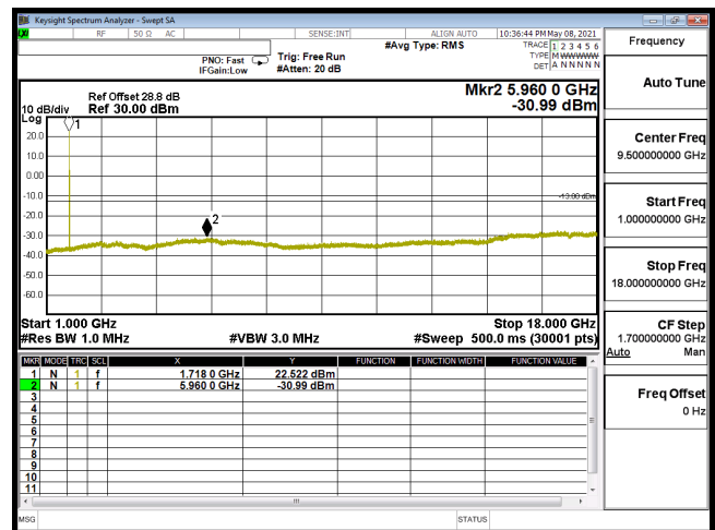
CSE-B66_15M-CH132047-16QAM(1,37)-1G-18G
