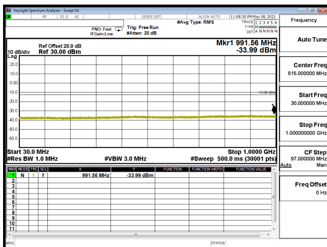
CSE-B66_5M-CH131997-16QAM(1,12)-30M-1G
