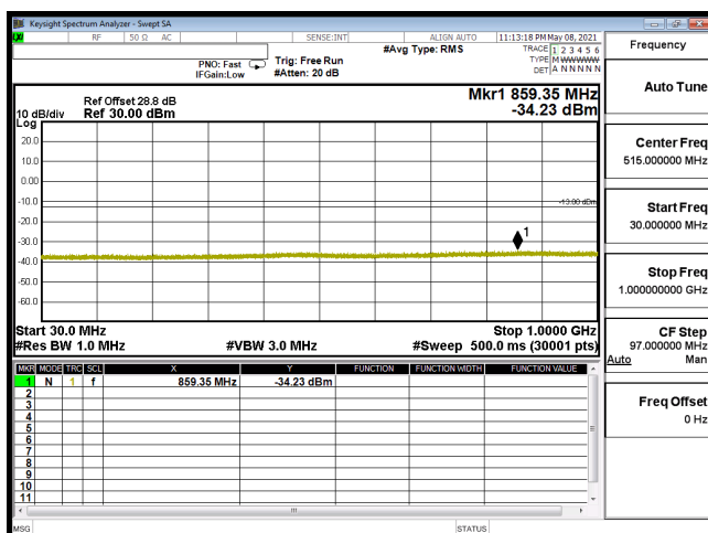
CSE-B66_10M-CH132022-64QAM(1,25)-30M-1G
