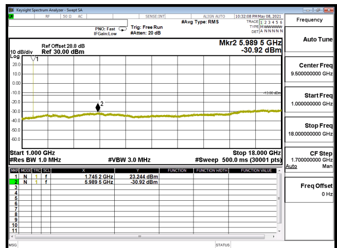
CSE-B66_10M-CH132322-64QAM(1,25)-1G-18G
