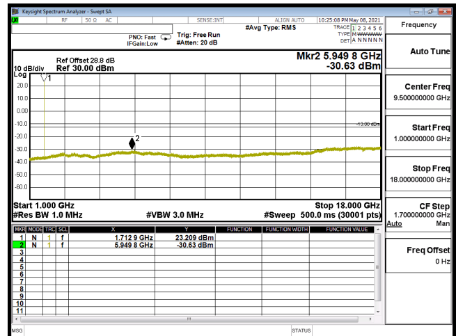
CSE-B66_5M-CH131997-QPSK(1,12)-1G-18G
