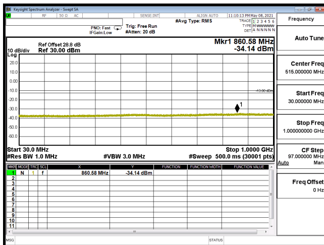
CSE-B66_5M-CH132647-16QAM(1,0)-30M-1G
