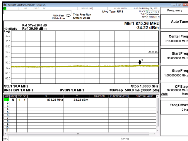
CSE-B66_10M-CH132022-QPSK(1,25)-30M-1G
