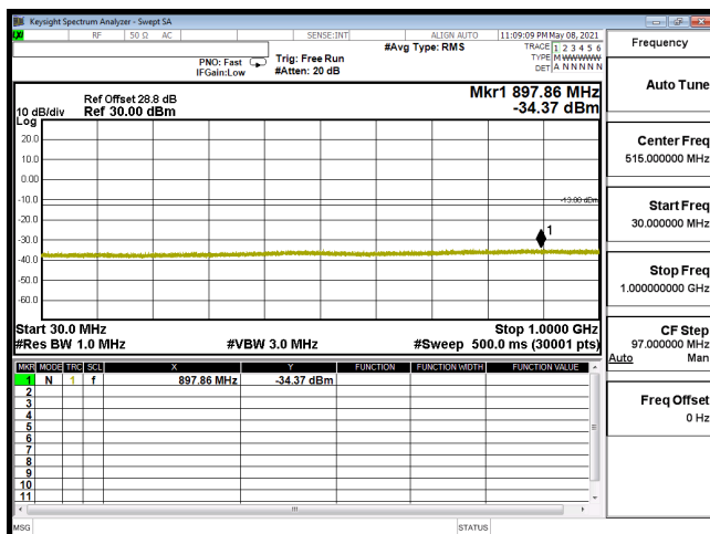
CSE-B66_5M-CH132322-64QAM(1,12)-30M-1G
