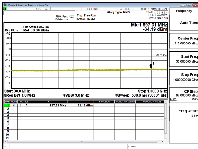
CSE-B66_5M-CH131997-QPSK(1,12)-30M-1G
