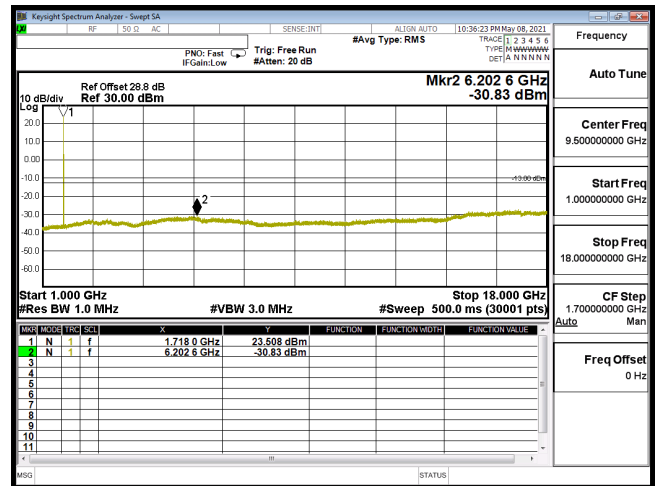
CSE-B66_15M-CH132047-QPSK(1,37)-1G-18G
