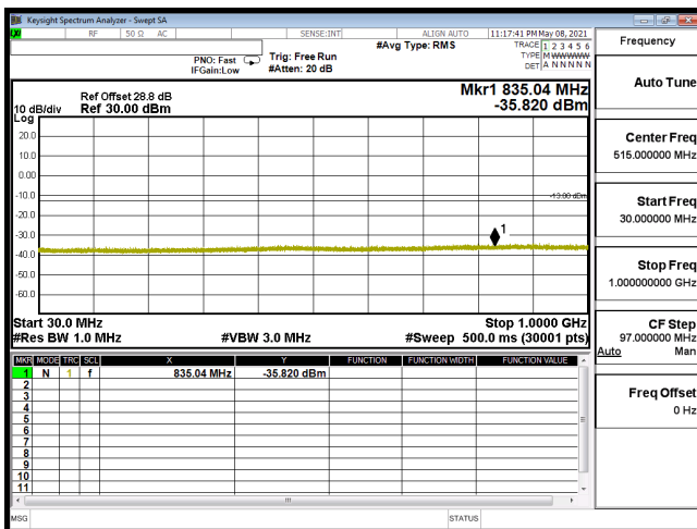
CSE-B66_15M-CH132322-16QAM(1,37)-30M-1G
