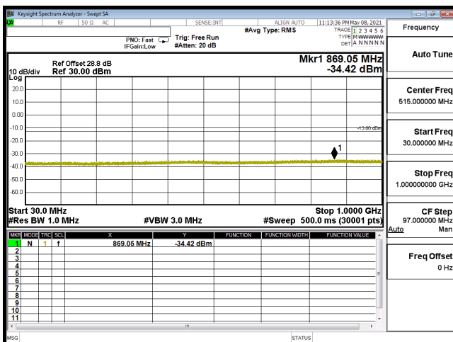
CSE-B66_10M-CH132322-64QAM(1,25)-30M-1G
