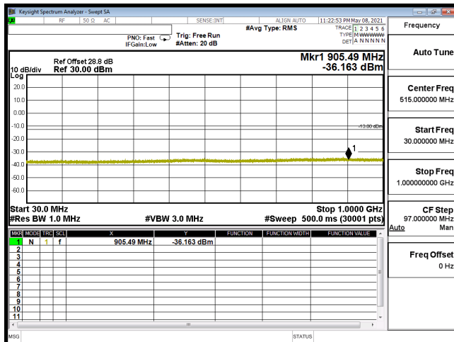
CSE-B66_20M-CH132572-QPSK(1,50)-30M-1G
