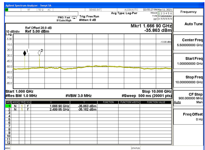
CSE(10M+10M)-2ULCA_5B-16QAM_829(1,49)+838.9(1,0)-1G-10G
