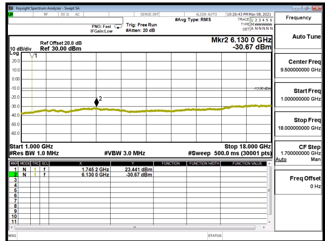
CSE-B66_5M-CH132322-QPSK(1,12)-1G-18G
