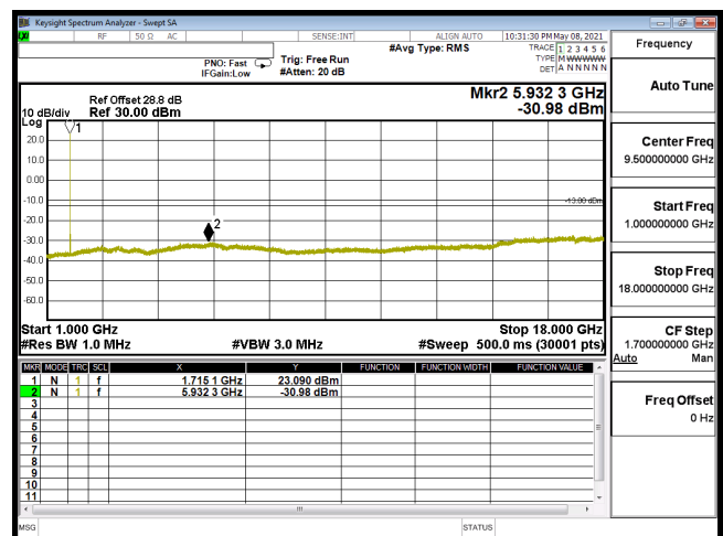
CSE-B66_10M-CH132022-16QAM(1,25)-1G-18G
