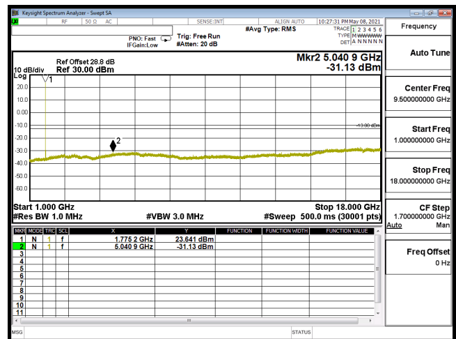
CSE-B66_5M-CH132647-16QAM(1,0)-1G-18G
