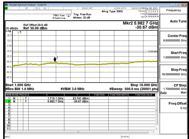
CSE-B66_10M-CH132022-QPSK(1,25)-1G-18G
