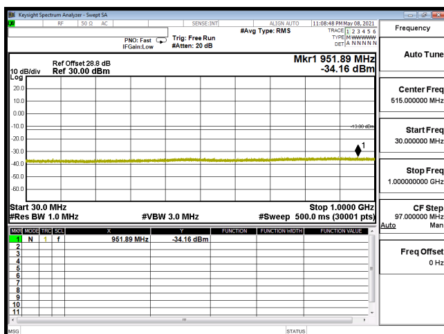
CSE-B66_5M-CH131997-64QAM(1,24)-30M-1G
