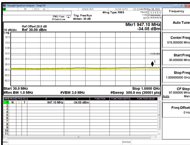
CSE-B66_10M-CH132322-16QAM(1,25)-30M-1G
