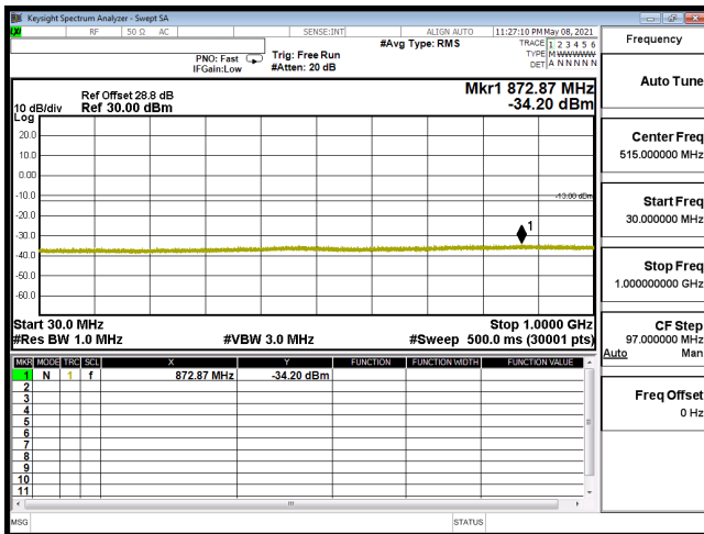
CSE-B66_15M-CH132322-QPSK(1,37)-30M-1G
