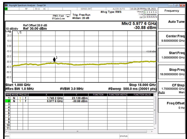
CSE-B66_5M-CH132322-16QAM(1,12)-1G-18G
