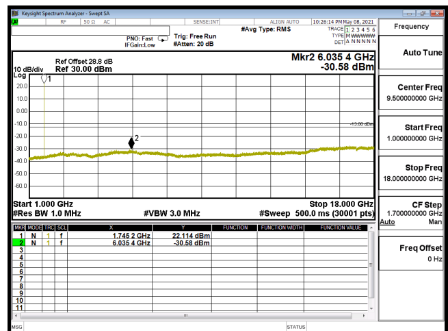
CSE-B66_5M-CH132322-64QAM(1,12)-1G-18G
