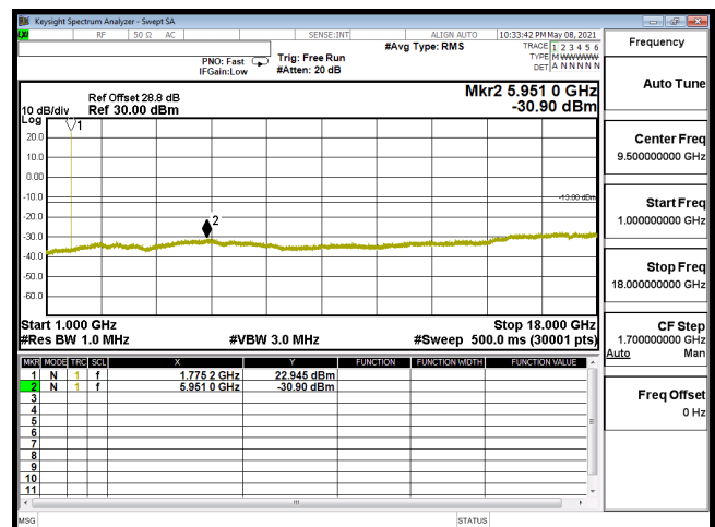
CSE-B66_10M-CH132622-64QAM(1,25)-1G-18G
