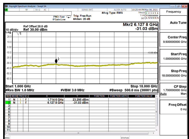
CSE-B66_5M-CH131997-64QAM(1,24)-1G-18G
