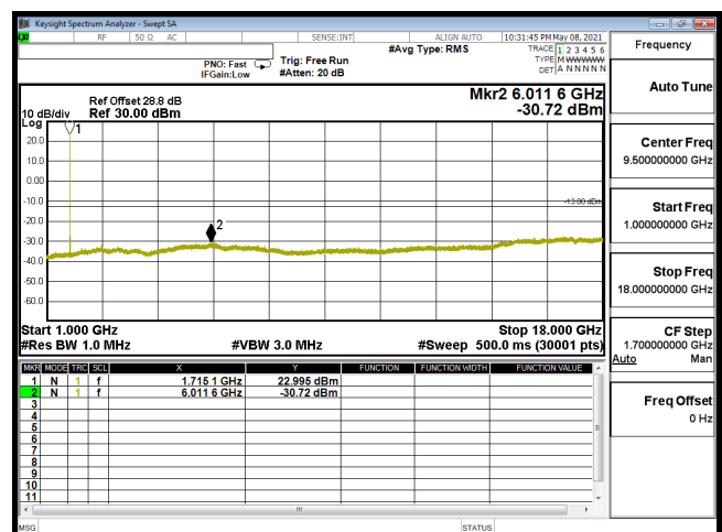
CSE-B66_10M-CH132022-64QAM(1,25)-1G-18G
