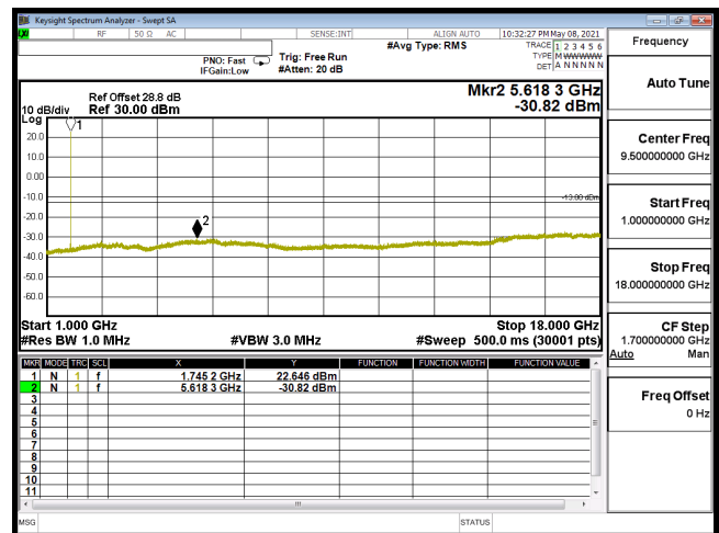
CSE-B66_10M-CH132322-16QAM(1,25)-1G-18G
