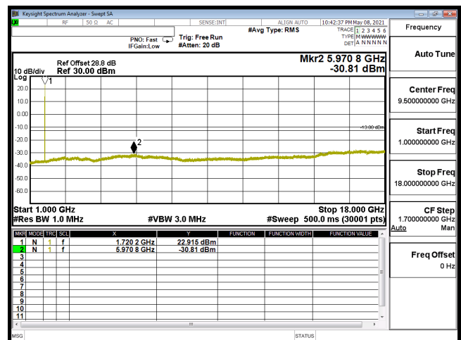
CSE-B66_20M-CH132072-64QAM(1,50)-1G-18G
