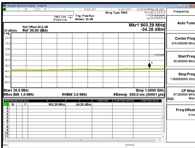
CSE-B66_20M-CH132072-16QAM(1,50)-30M-1G
