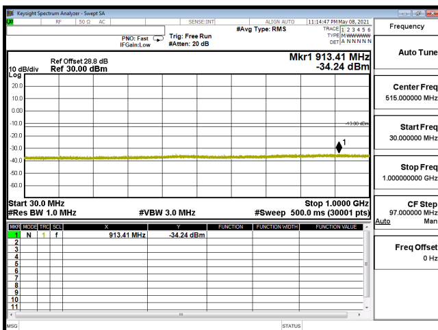
CSE-B66_10M-CH132622-64QAM(1,25)-30M-1G
