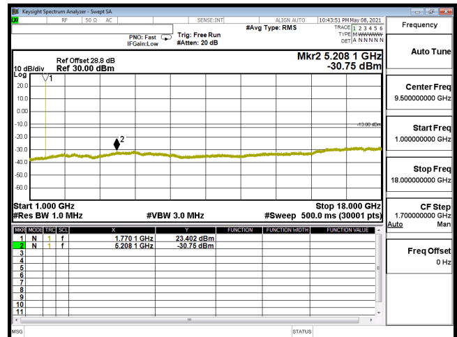
CSE-B66_20M-CH132572-QPSK(1,50)-1G-18G
