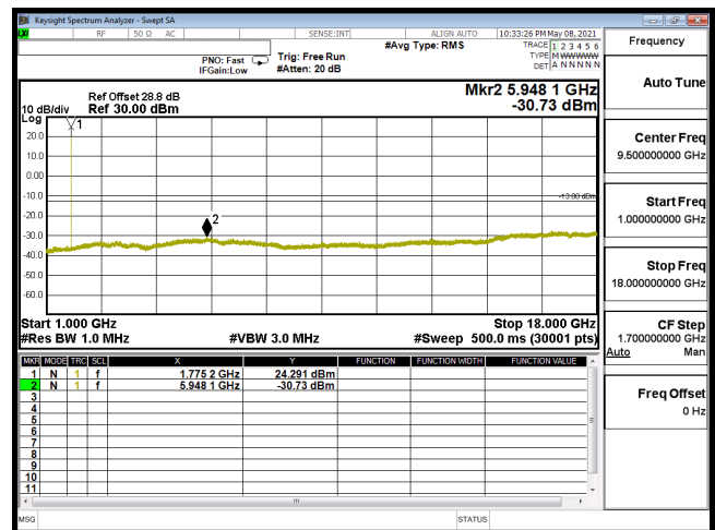
CSE-B66_10M-CH132622-16QAM(1,25)-1G-18G
