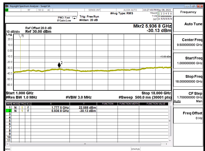
CSE-B66_5M-CH132647-64QAM(1,12)-1G-18G
