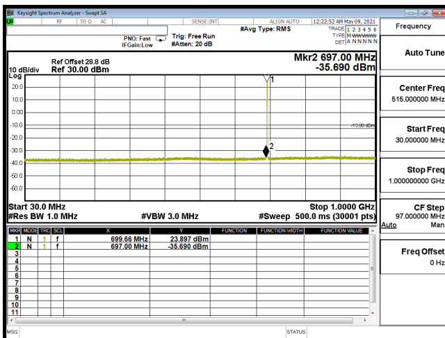
CSE-B12_1.4M-CH23017-64QAM(1,2)-30M-1G
