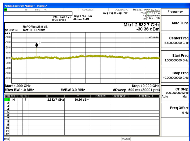
CSE-B5_5M-CH20625-16QAM(1,0)-1G-10G
