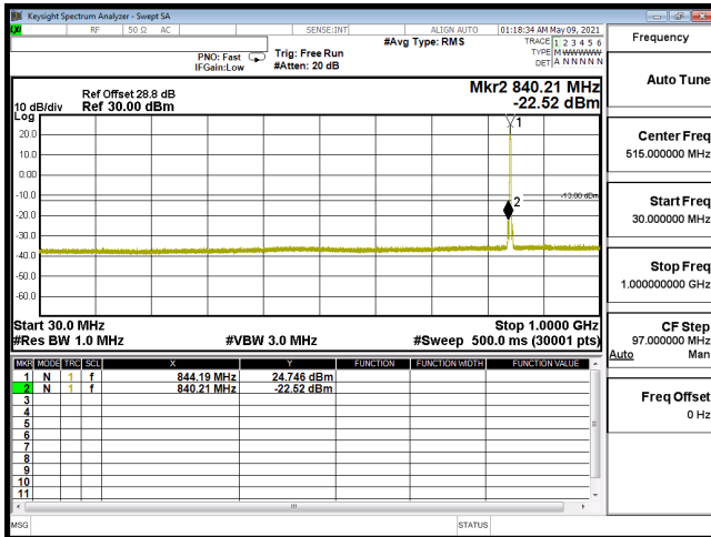
CSE-B5_10M-CH20600-QPSK(1,25)-30M-1G
