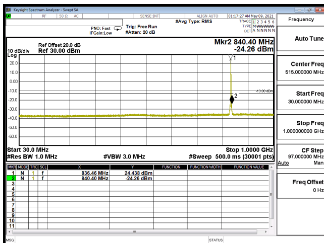
CSE-B5_10M-CH20525-64QAM(1,25)-30M-1G
