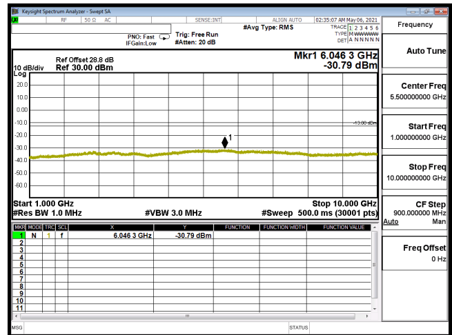
CSE-B12_3M-CH23025-QPSK(1,7)-1G-10G
