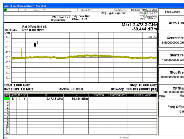
CSE-B5_10M-CH20450-64QAM(1,0)-1G-10G
