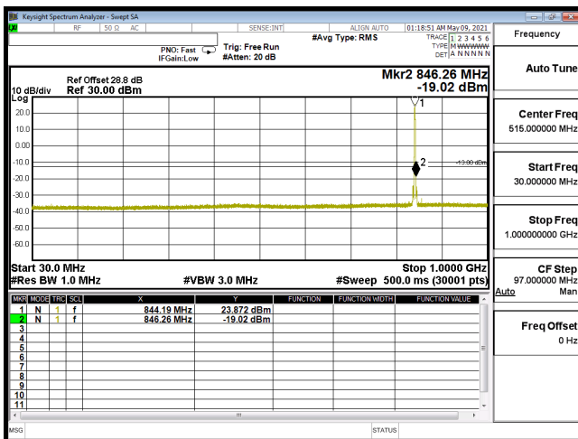
CSE-B5_10M-CH20600-16QAM(1,25)-30M-1G
