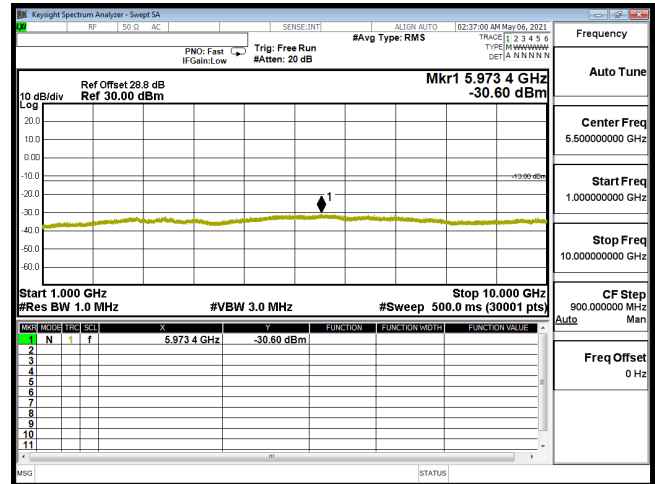
CSE-B12_3M-CH23095-QPSK(1,14)-1G-10G
