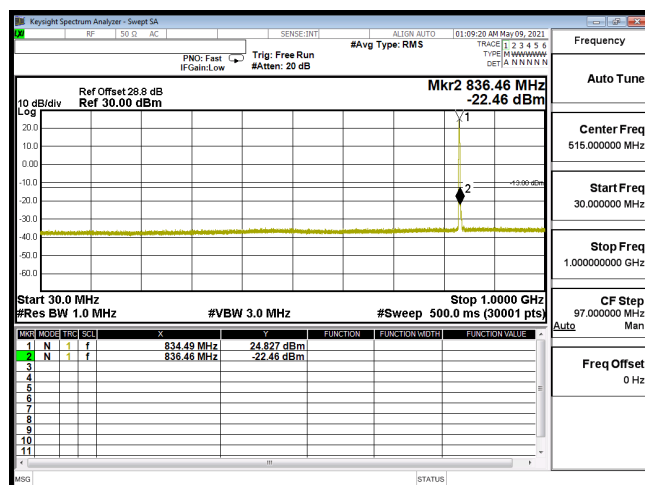
CSE-B5_5M-CH20525-64QAM(1,0)-30M-1G
