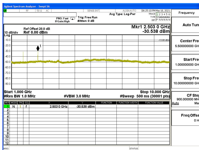
CSE-B5_5M-CH20525-64QAM(1,0)-1G-10G
