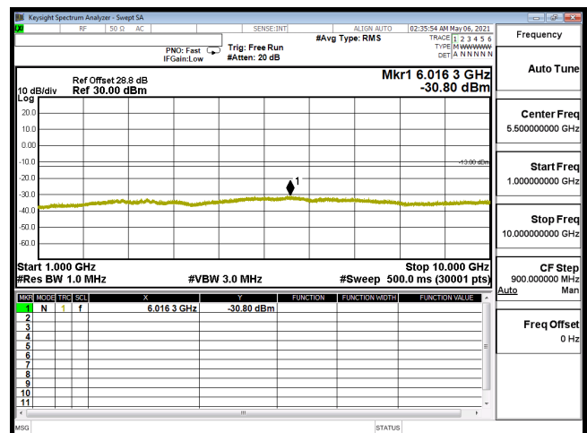
CSE-B12_3M-CH23025-64QAM(1,14)-1G-10G
