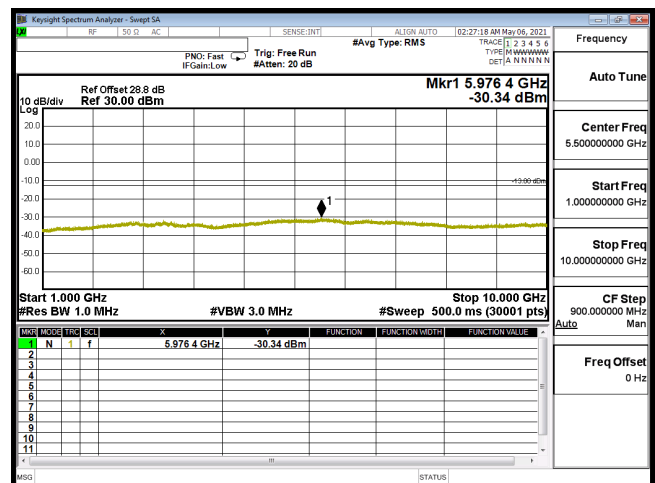
CSE-B12_1.4M-CH23173-64QAM(3,2)-1G-10G
