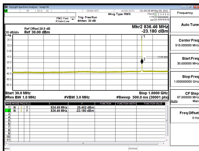
CSE-B5_5M-CH20525-16QAM(1,0)-30M-1G
