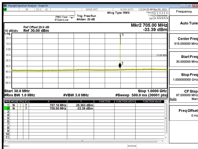
CSE-B12_1.4M-CH23095-16QAM(1,0)-30M-1G
