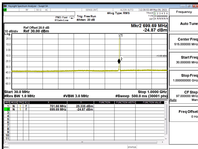
CSE-B12_3M-CH23025-64QAM(1,14)-30M-1G
