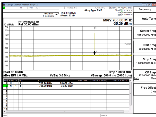
CSE-B12_1.4M-CH23095-64QAM(1,5)-30M-1G
