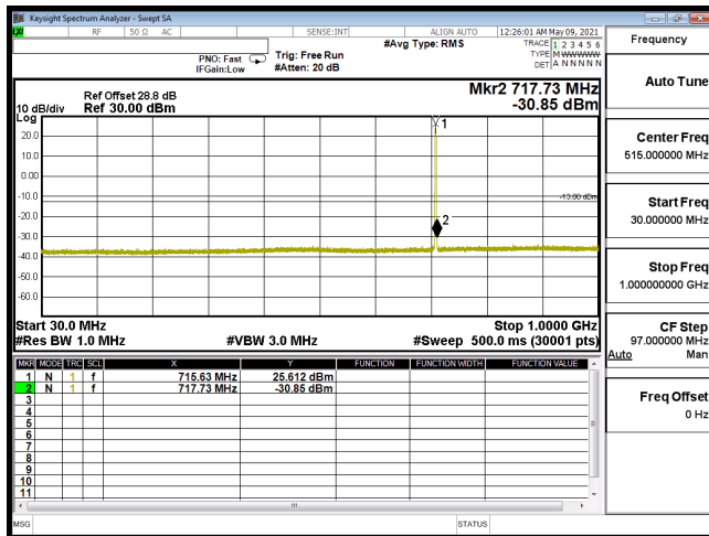
CSE-B12_1.4M-CH23173-QPSK(1,5)-30M-1G
