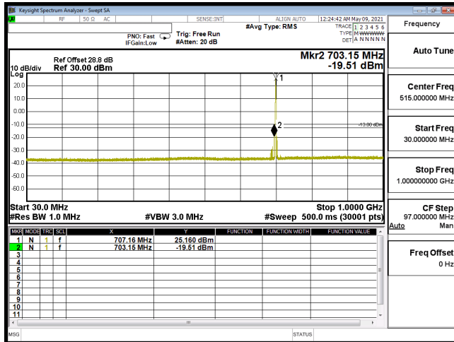
CSE-B12_1.4M-CH23095-QPSK(3,0)-30M-1G
