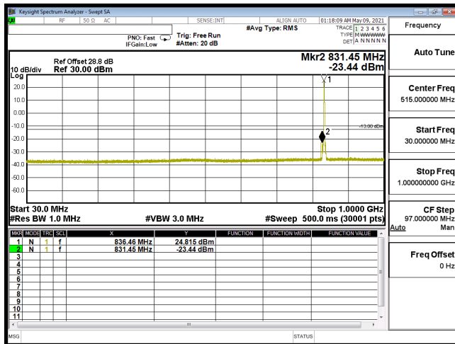
CSE-B5_10M-CH20525-QPSK(1,25)-30M-1G
