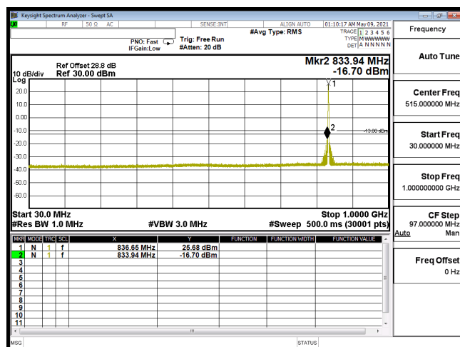
CSE-B5_5M-CH20525-QPSK(1,12)-30M-1G
