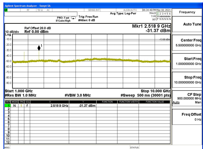
CSE-B5_10M-CH20600-64QAM(1,0)-1G-10G
