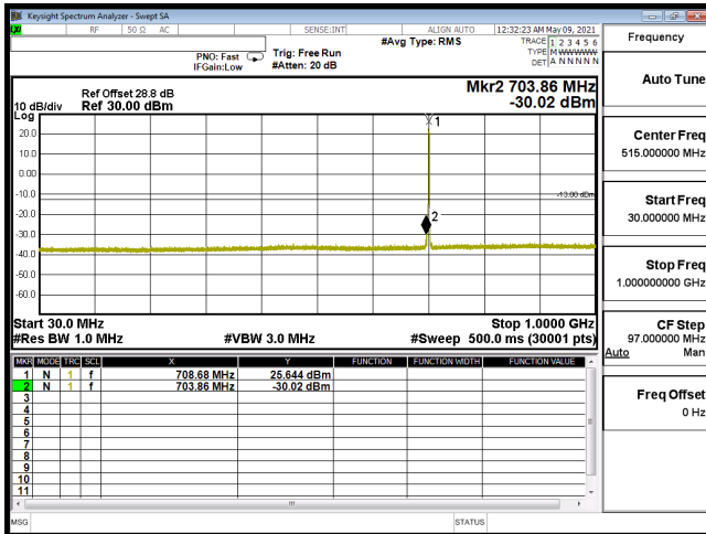
CSE-B12_3M-CH23095-QPSK(1,14)-30M-1G
