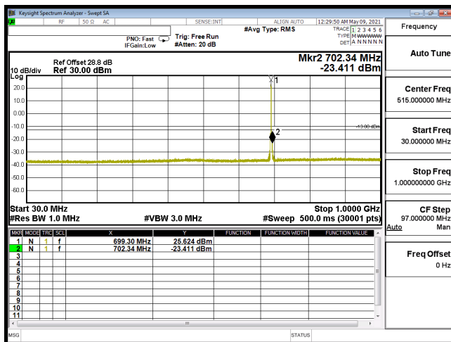
CSE-B12_3M-CH23025-16QAM(1,0)-30M-1G
