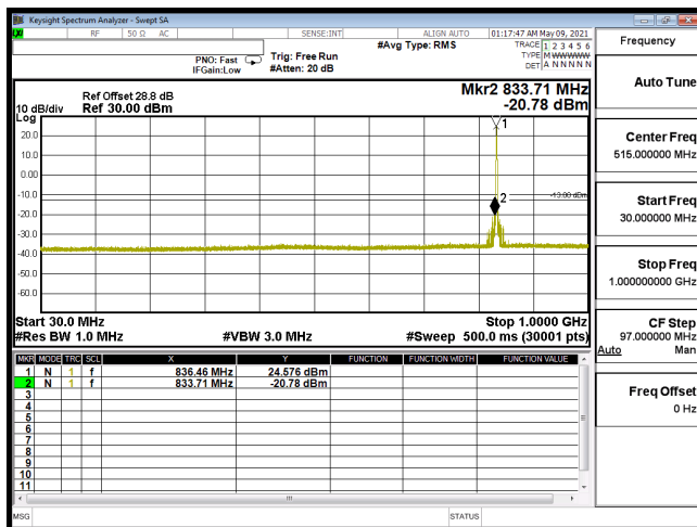
CSE-B5_10M-CH20525-16QAM(1,25)-30M-1G
