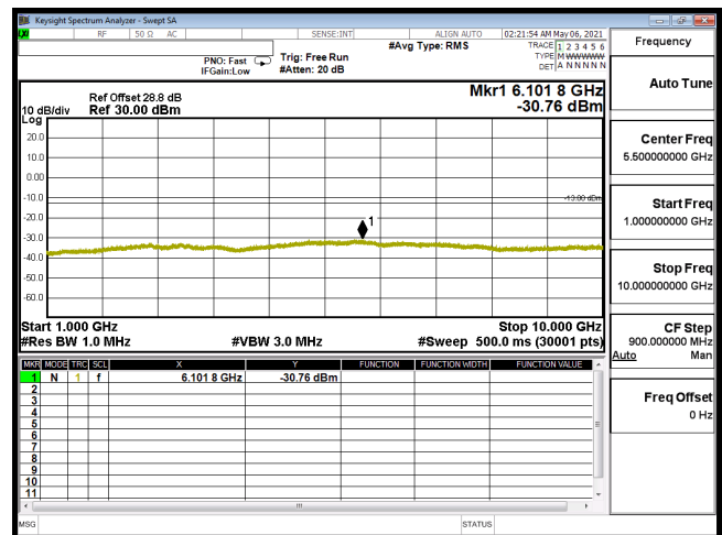
CSE-B12_1.4M-CH23095-16QAM(1,0)-1G-10G
