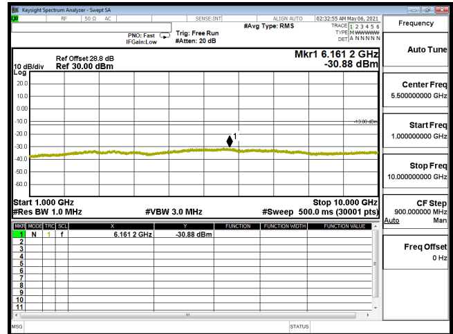
CSE-B12_1.4M-CH23017-QPSK(1,2)-1G-10G
