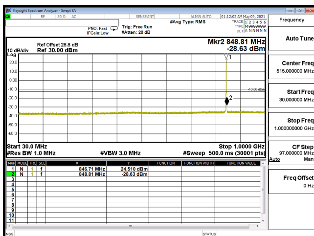
CSE-B5_5M-CH20625-64QAM(1,12)-30M-1G
