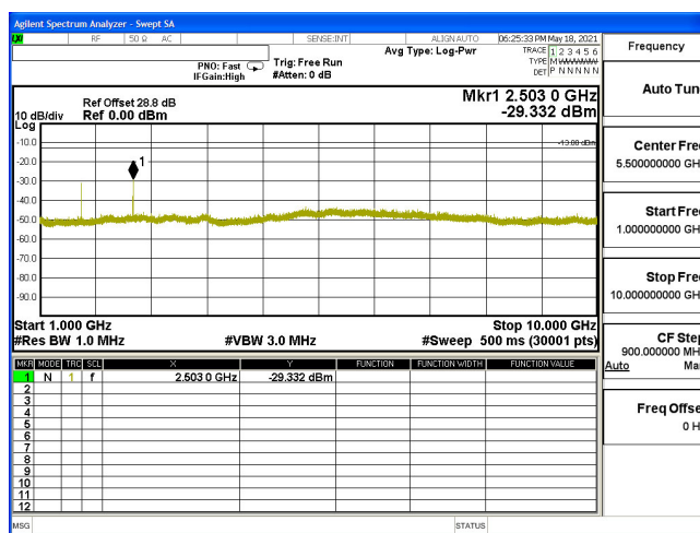
CSE-B5_5M-CH20525-16QAM(1,0)-1G-10G
