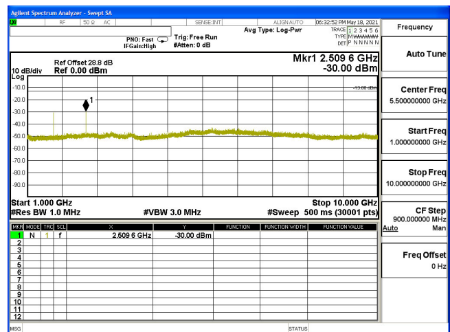
CSE-B5_10M-CH20525-64QAM(1,25)-1G-10G
