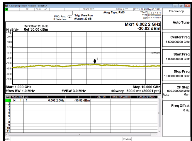
CSE-B12_1.4M-CH23095-64QAM(1,5)-1G-10G
