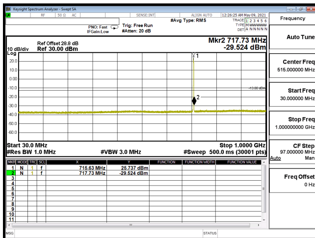
CSE-B12_1.4M-CH23173-16QAM(1,5)-30M-1G
