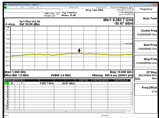
CSE-B12_3M-CH23095-16QAM(1,7)-1G-10G
