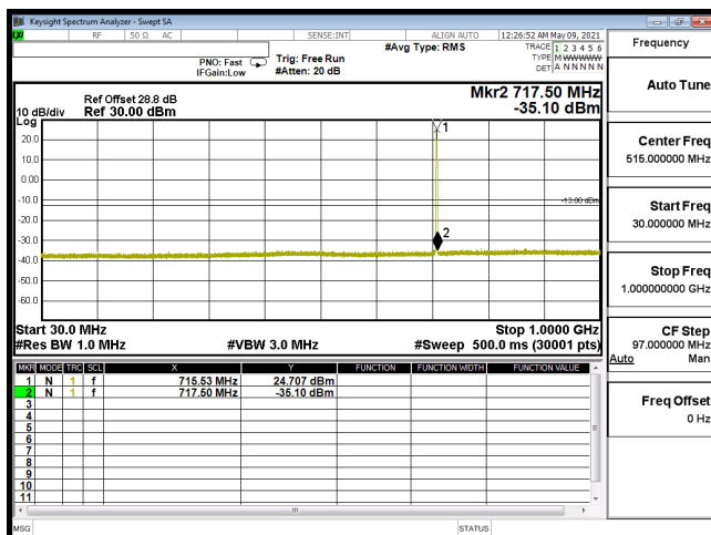
CSE-B12_1.4M-CH23173-64QAM(3,2)-30M-1G
