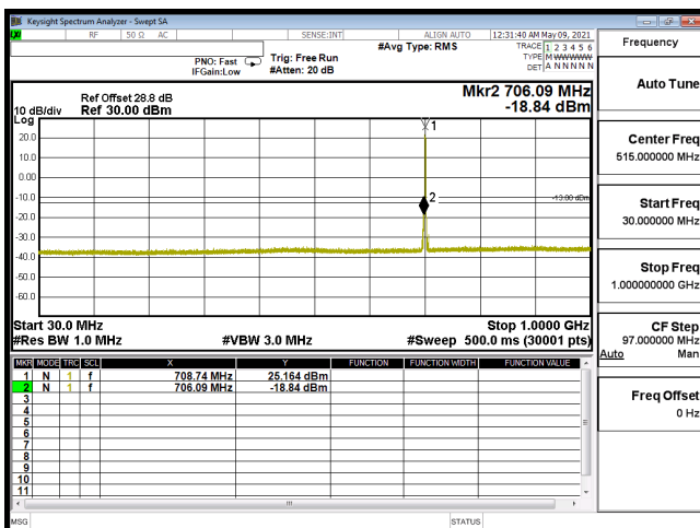
CSE-B12_3M-CH23095-64QAM(1,14)-30M-1G
