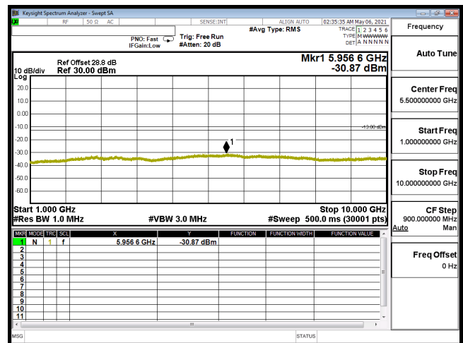
CSE-B12_3M-CH23025-16QAM(1,0)-1G-10G
