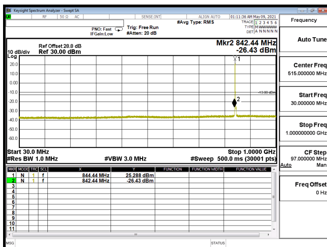
CSE-B5_5M-CH20625-16QAM(1,0)-30M-1G
