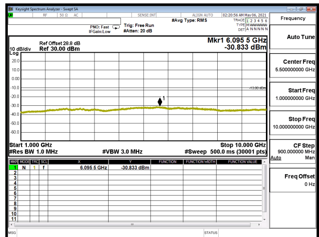
CSE-B12_1.4M-CH23017-64QAM(1,2)-1G-10G
