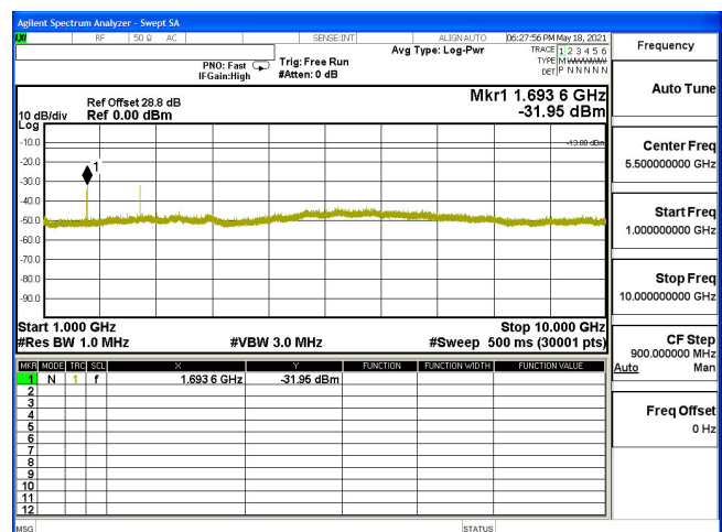
CSE-B5_5M-CH20625-64QAM(1,12)-1G-10G
