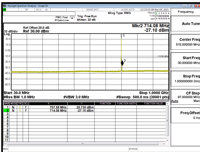
CSE-B12_3M-CH23095-16QAM(1,7)-30M-1G
