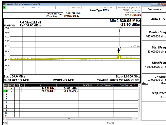
CSE-B5_5M-CH20625-QPSK(1,12)-30M-1G
