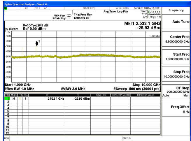
CSE-B5_10M-CH20600-QPSK(1,25)-1G-10G
