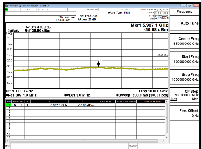
CSE-B12_1.4M-CH23173-16QAM(1,5)-1G-10G
