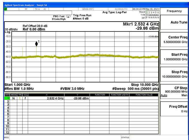
CSE-B5_10M-CH20600-16QAM(1,25)-1G-10G
