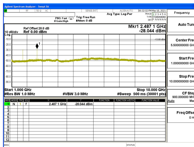
CSE-B5 10M-CH20450-16QAM(1,25)-1G-10G
