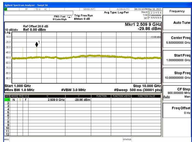
CSE-B5_10M-CH20525-16QAM(1,25)-1G-10G
