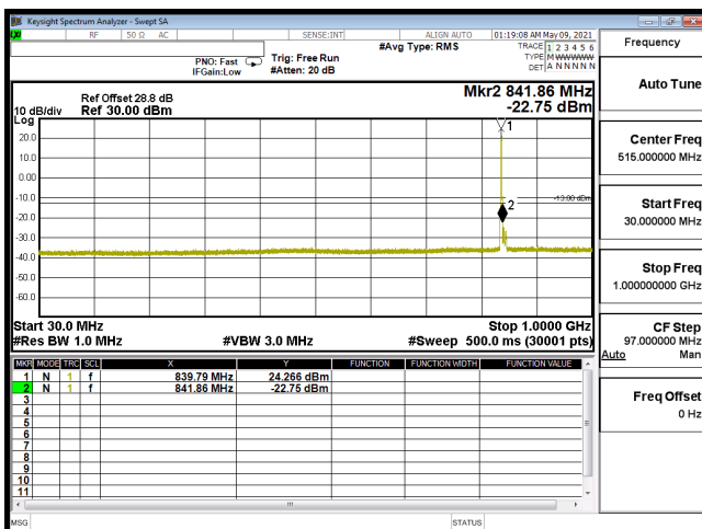
CSE-B5_10M-CH20600-64QAM(1,0)-30M-1G
