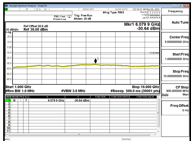
CSE-B12_3M-CH23095-64QAM(1,14)-1G-10G
