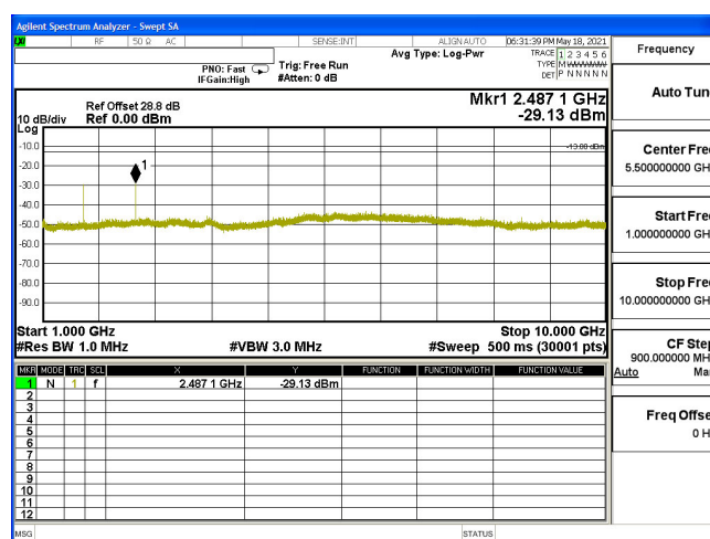
CSE-B5 10M-CH20450-QPSK(1,25)-1G-10G
