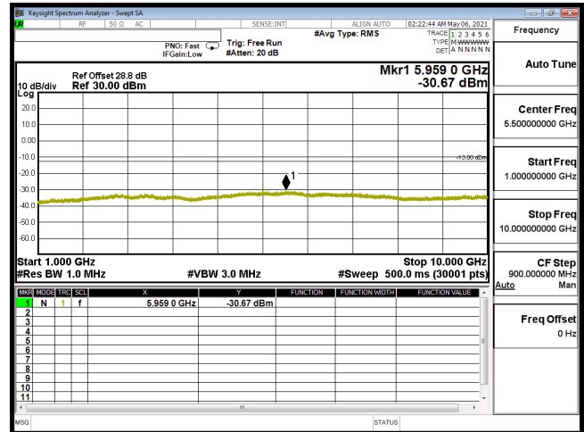
CSE-B12_1.4M-CH23095-QPSK(3,0)-1G-10G
