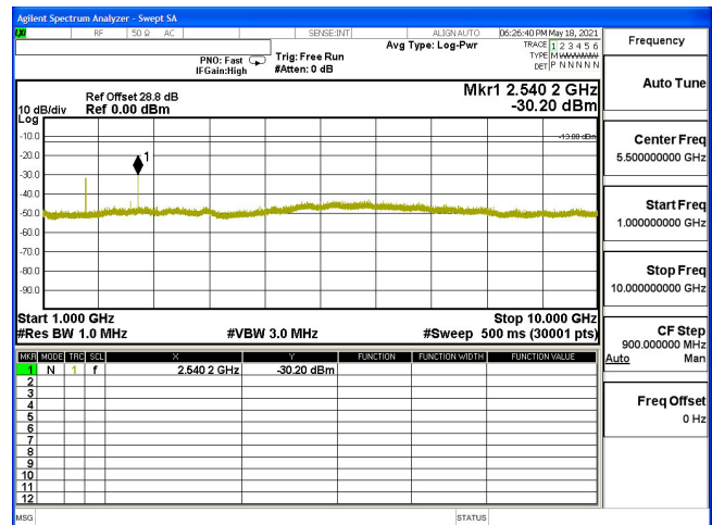
CSE-B5_5M-CH20625-QPSK(1,12)-1G-10G
