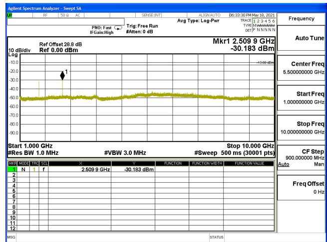
CSE-B5_10M-CH20525-QPSK(1,25)-1G-10G
