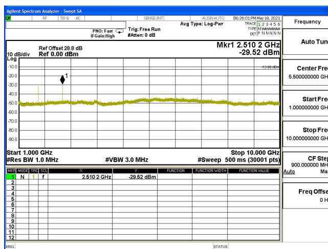
CSE-B5_5M-CH20525-QPSK(1,12)-1G-10G
