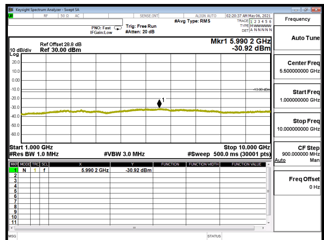
CSE-B12_1.4M-CH23017-16QAM(1,2)-1G-10G
