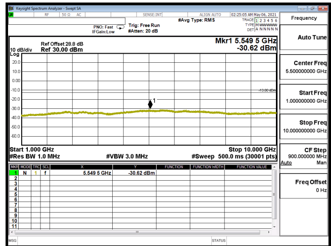
CSE-B12_1.4M-CH23173-QPSK(1,5)-1G-10G
