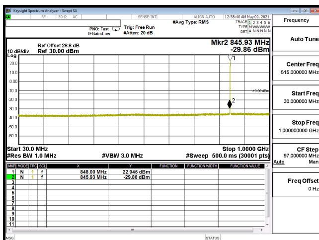
CSE-B5_1.4M-CH20643-64QAM(3,0)-30M-1G
