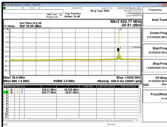
CSE-B5_1.4M-CH20525-16QAM(1,0)-30M-1G
