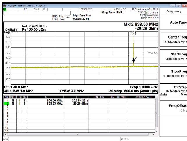
CSE-B5_1.4M-CH20525-64QAM(1,2)-30M-1G
