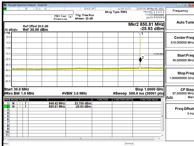
CSE-B5_1.4M-CH20643-QPSK(3,3)-30M-1G
