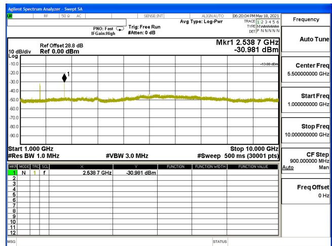
CSE-B5_3M-CH20635-16QAM(1,0)-1G-10G
