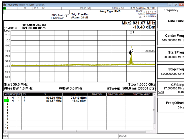
CSE-B5_1.4M-CH20525-QPSK(3,0)-30M-1G
