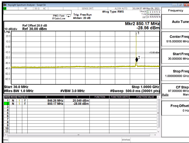
CSE-B5_3M-CH20635-QPSK(1,0)-30M-1G
