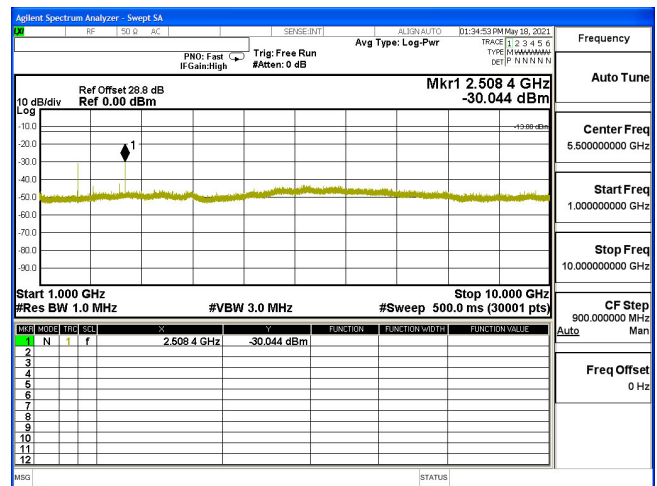
CSE-B5_1.4M-CH20525-16QAM(1,0)-1G-10G
