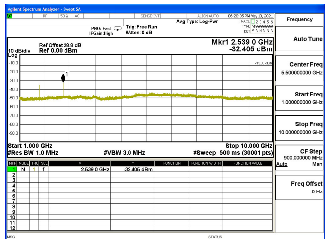
CSE-B5_3M-CH20635-64QAM(1,0)-1G-10G
