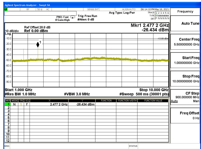
CSE-B5_3M-CH20415-QPSK(1,7)-1G-10G
