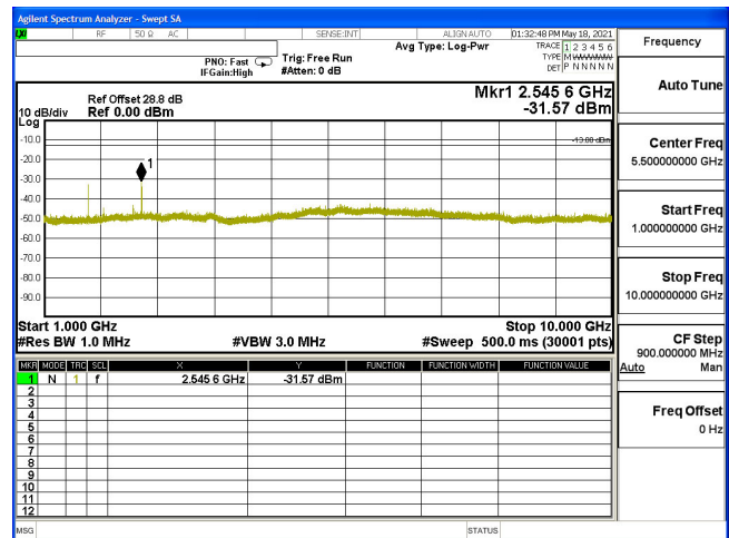
CSE-B5_1.4M-CH20643-QPSK(3,3)-1G-10G
