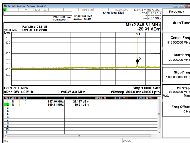
CSE-B5_1.4M-CH20643-16QAM(1,0)-30M-1G
