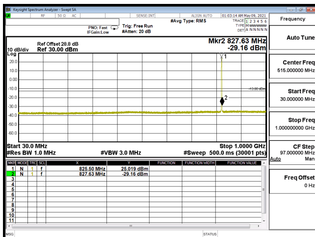
CSE-B5_3M-CH20415-64QAM(1,7)-30M-1G
