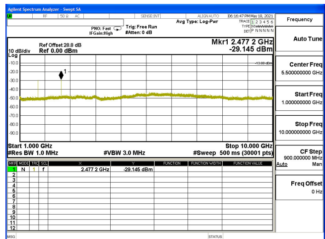
CSE-B5_3M-CH20415-64QAM(1,7)-1G-10G
