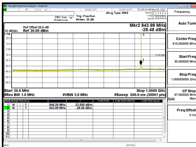
CSE-B5_3M-CH20635-64QAM(1,0)-30M-1G
