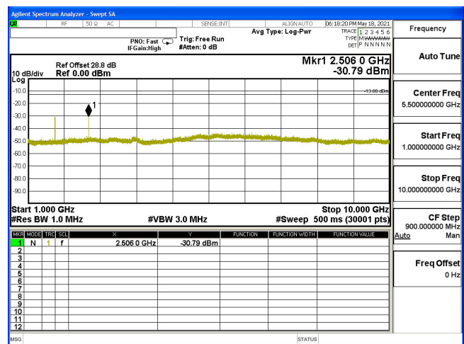
CSE-B5_3M-CH20525-16QAM(1,0)-1G-10G
