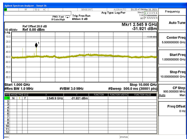
CSE-B5_1.4M-CH20643-16QAM(1,0)-1G-10G
