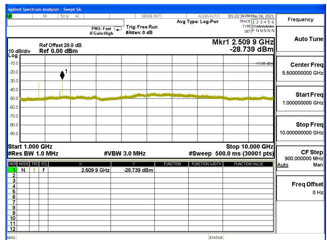
CSE-B5_1.4M-CH20525-64QAM(1,2)-1G-10G
