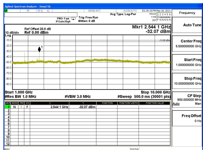
CSE-B5_1.4M-CH20643-64QAM(3,0)-1G-10G
