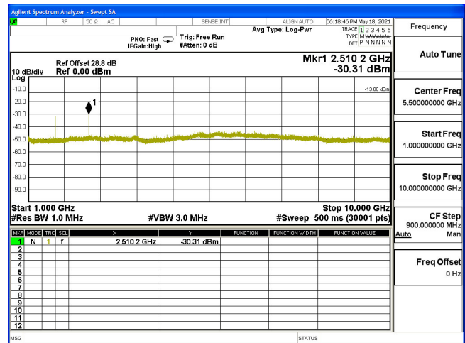
CSE-B5_3M-CH20525-QPSK(1,7)-1G-10G
