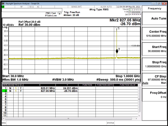
CSE-B5_1.4M-CH20407-64QAM(3,3)-30M-1G
