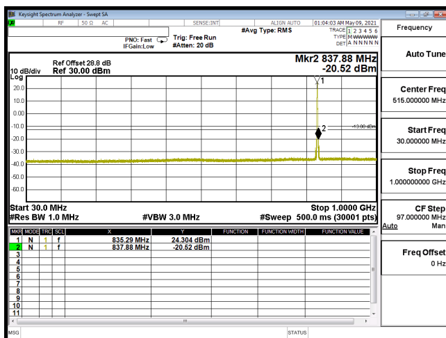
CSE-B5_3M-CH20525-16QAM(1,0)-30M-1G
