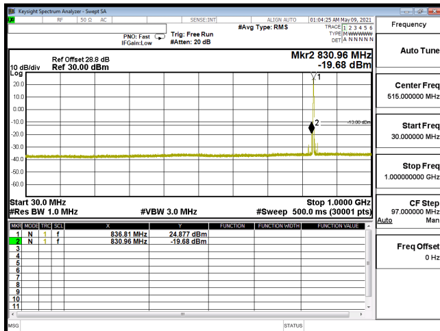
CSE-B5_3M-CH20525-QPSK(1,7)-30M-1G
