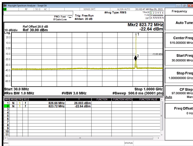
CSE-B5_3M-CH20415-16QAM(1,14)-30M-1G
