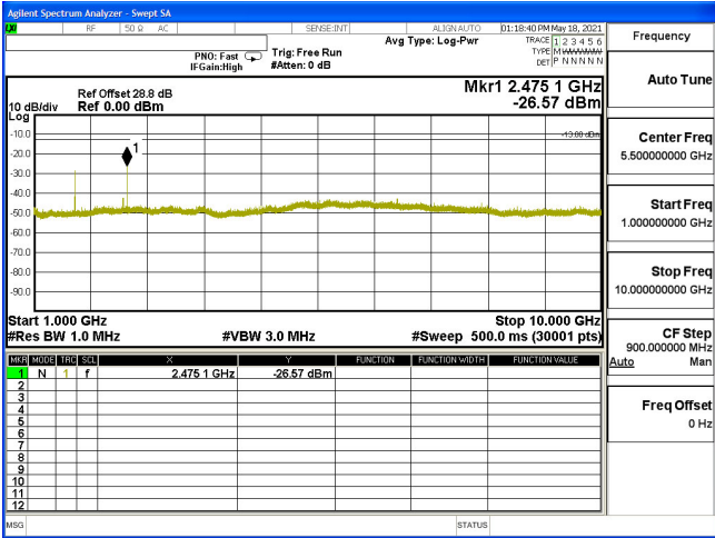
CSE-B5_1.4M-CH20407-QPSK(3,3)-1G-10G
