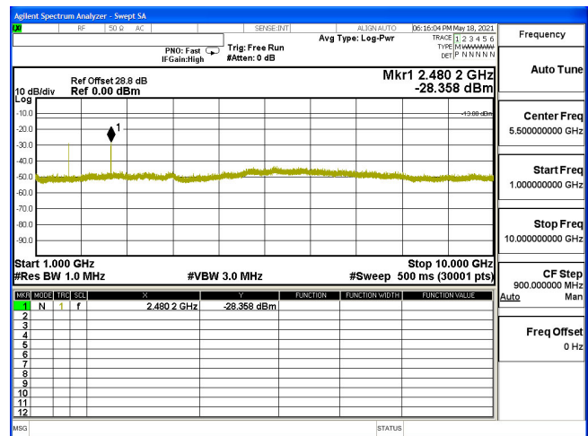
CSE-B5_3M-CH20415-16QAM(1,14)-1G-10G
