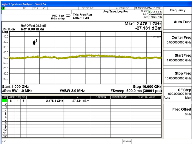
CSE-B5_1.4M-CH20407-16QAM(1,5)-1G-10G
