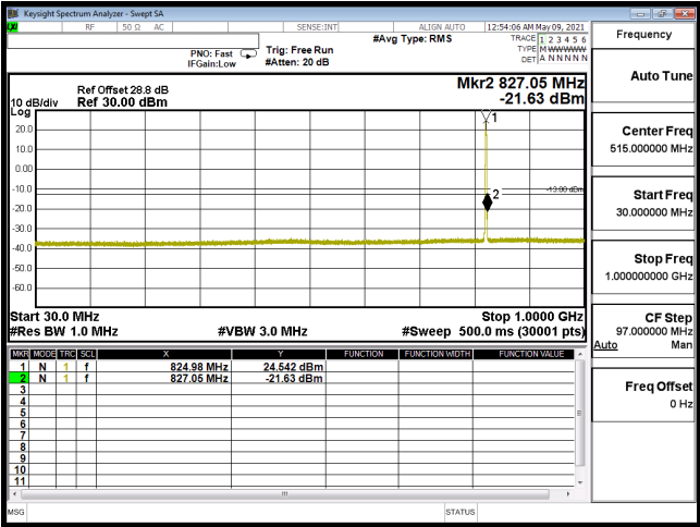
CSE-B5_1.4M-CH20407-QPSK(3,3)-30M-1G
