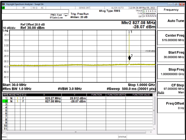
CSE-B5_1.4M-CH20407-16QAM(1,5)-30M-1G
