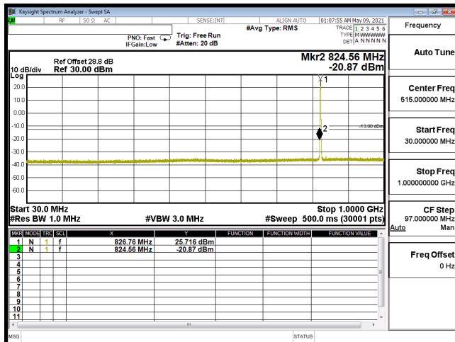
CSE-B5_5M-CH20425-QPSK(1,12)-30M-1G
