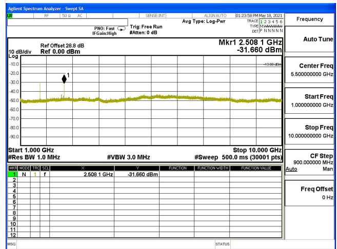
CSE-B5_1.4M-CH20525-QPSK(3,0)-1G-10G
