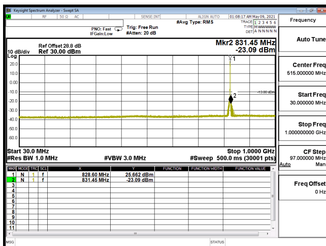
CSE-B5_5M-CH20425-16QAM(1,24)-30M-1G
