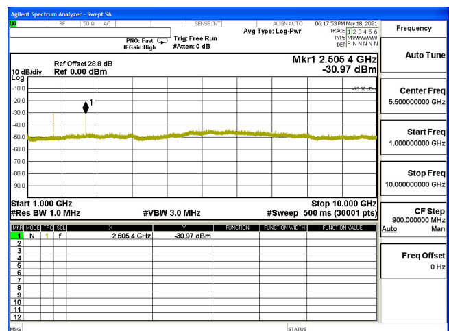
CSE-B5_3M-CH20525-64QAM(1,0)-1G-10G
