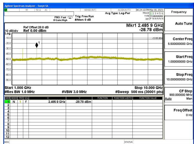
CSE-B5_5M-CH20425-16QAM(1,24)-1G-10G
