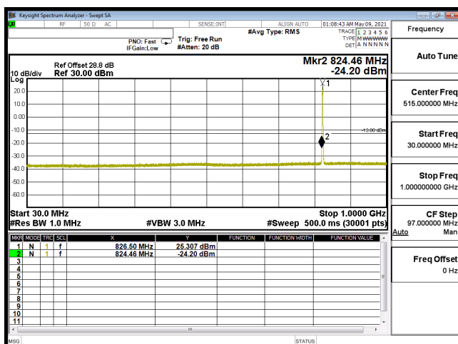
CSE-B5_5M-CH20425-64QAM(1,12)-30M-1G
