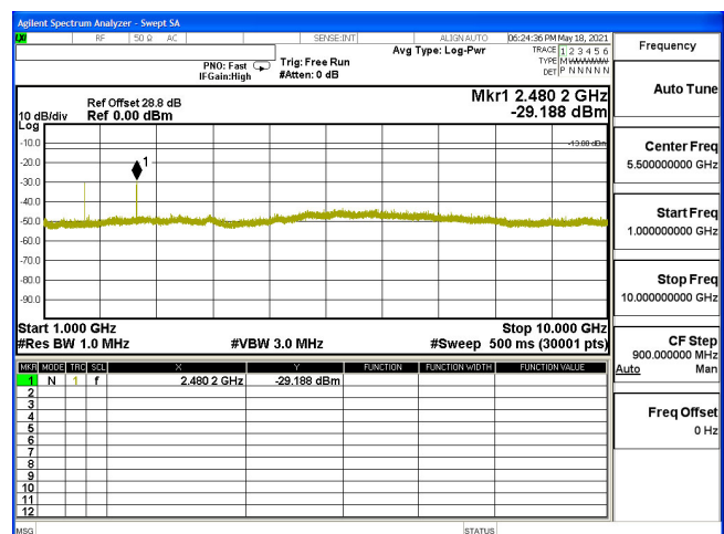
CSE-B5_5M-CH20425-64QAM(1,12)-1G-10G
