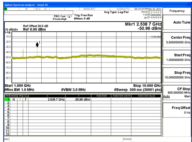
CSE-B5_3M-CH20635-QPSK(1,0)-1G-10G
