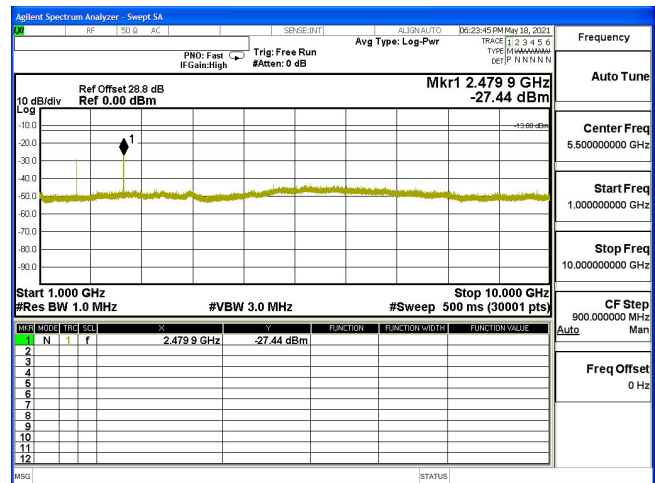
CSE-B5_5M-CH20425-QPSK(1,12)-1G-10G
