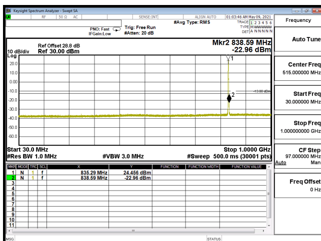
CSE-B5_3M-CH20525-64QAM(1,0)-30M-1G
