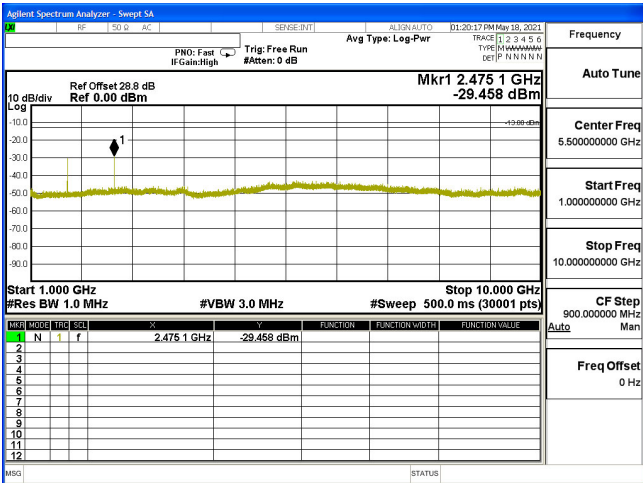
CSE-B5_1.4M-CH20407-64QAM(3,3)-1G-10G
