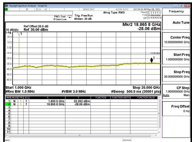
CSE-B2_5M-CH18625-64QAM(1,0)-1G-20G
