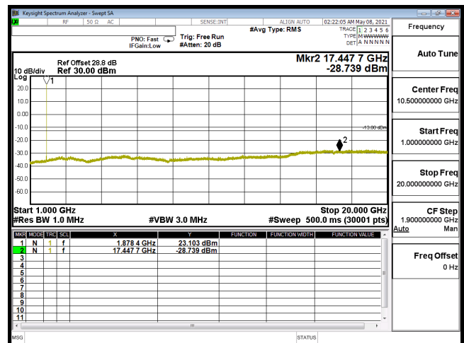
CSE-B2_3M-CH18900-QPSK(1,0)-1G-20G
