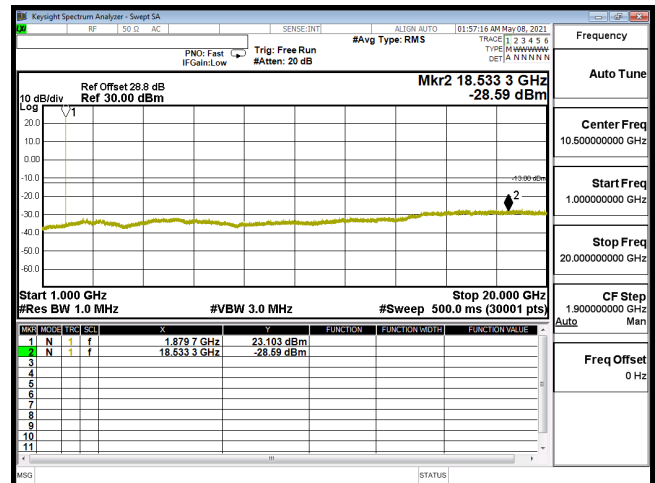
CSE-B2_1.4M-CH18900-QPSK(1,0)-1G-20G
