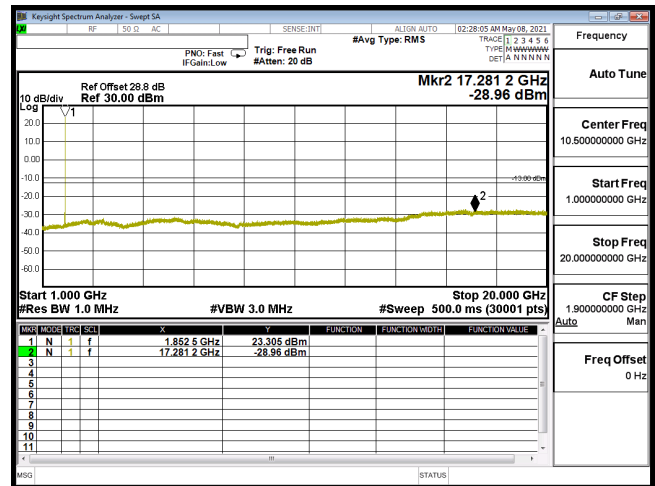
CSE-B2_5M-CH18625-QPSK(1,12)-1G-20G
