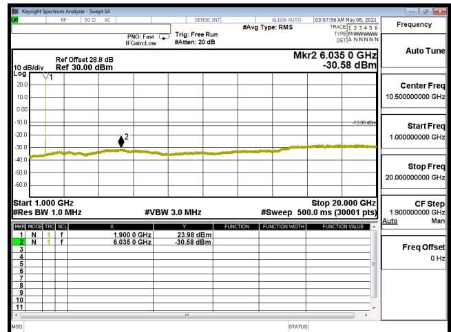
CSE-B2_20M-CH19100-QPSK(1,50)-1G-20G
