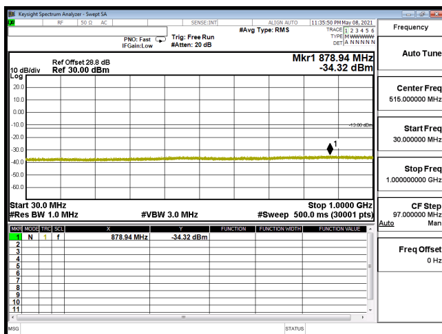
CSE-B2_3M-CH18900-16QAM(1,7)-30M-1G
