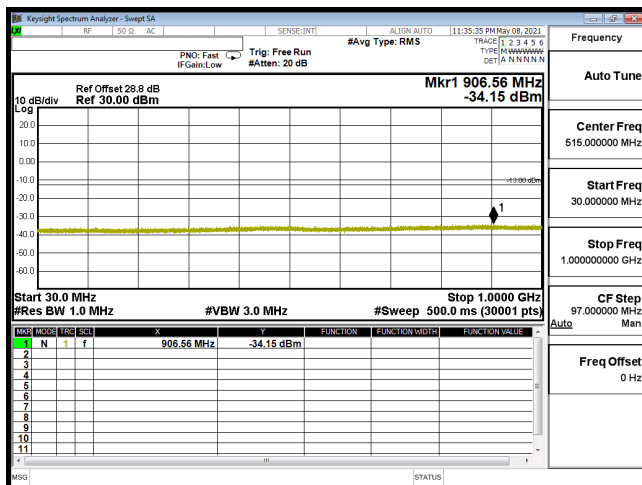
CSE-B2_3M-CH18900-QPSK(1,0)-30M-1G
