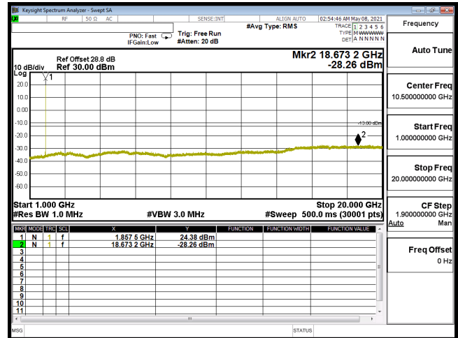
CSE-B2_15M-CH18675-QPSK(1,37)-1G-20G
