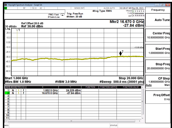
CSE-B2_5M-CH18625-16QAM(1,12)-1G-20G
