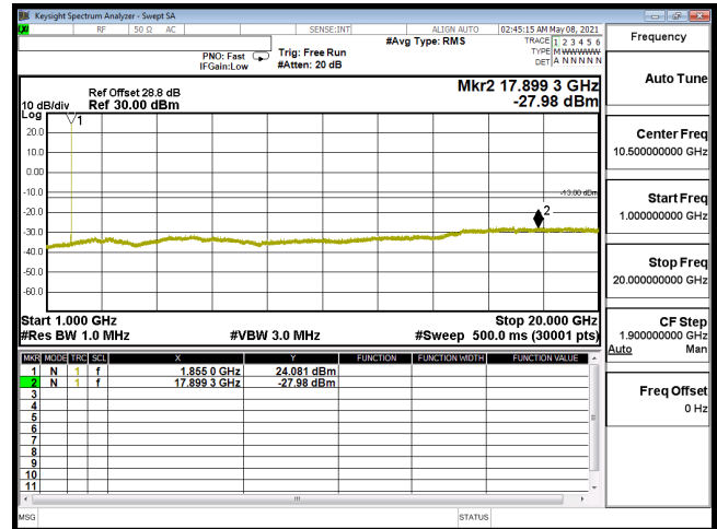
CSE-B2_10M-CH18625-QPSK(1,25)-1G-20G
