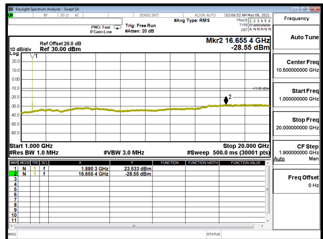
CSE-B2_20M-CH18900-16QAM(1,50)-1G-20G
