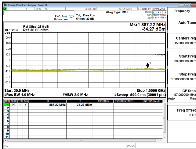
CSE-B2_3M-CH19185-QPSK(1,7)-30M-1G
