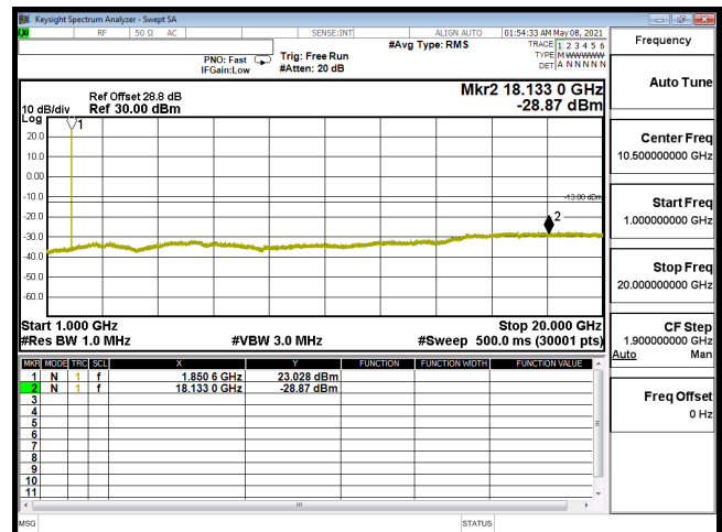
CSE-B2_1.4M-CH18607-16QAM(1,0)-1G-20G
