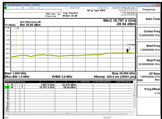
CSE-B2_15M-CH18675-64QAM(1,37)-1G-20G
