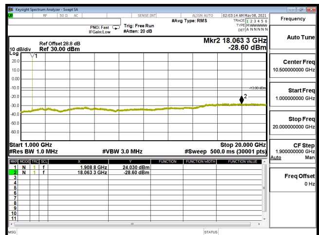
CSE-B2_1.4M-CH19193-64QAM(1,0)-1G-20G
