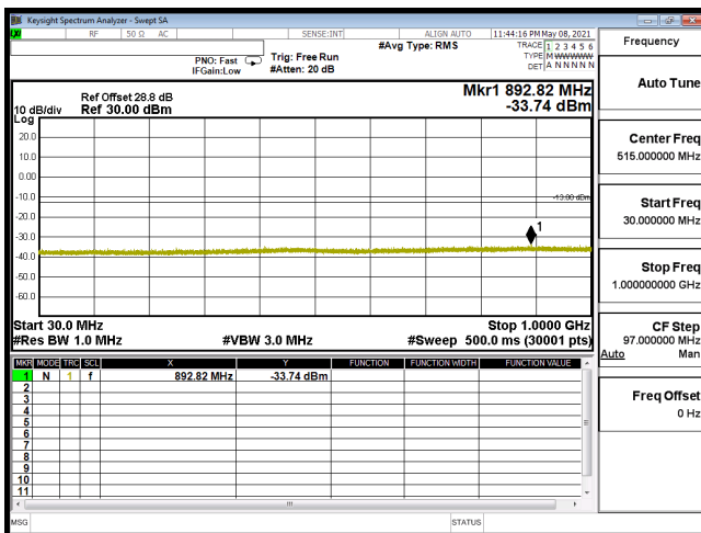
CSE-B2_10M-CH18900-16QAM(1,25)-1G-20G
