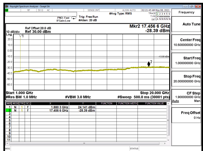
CSE-B2_3M-CH18900-16QAM(1,7)-1G-20G
