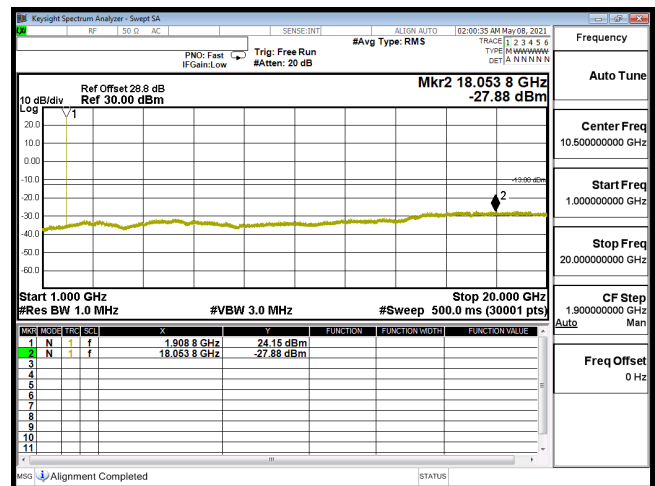
CSE-B2_1.4M-CH19193-16QAM(1,0)-1G-20G
