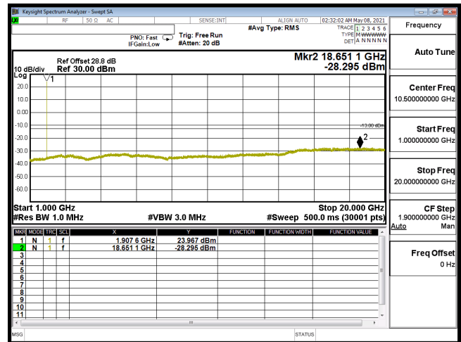
CSE-B2_5M-CH19175-QPSK(1,12)-1G-20G
