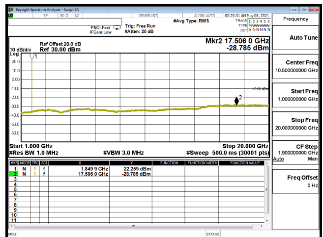
CSE-B2_3M-CH18615-64QAM(1,0)-1G-20G
