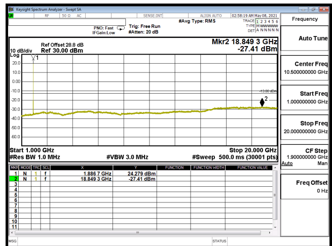
CSE-B2_15M-CH18900-16QAM(1,74)-1G-20G
