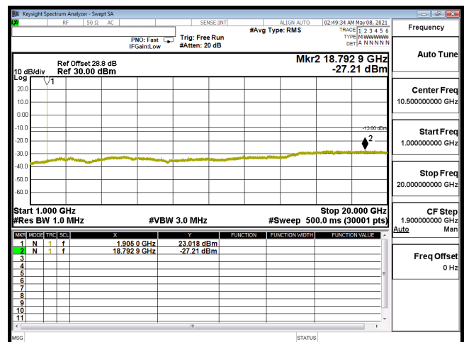
CSE-B2_10M-CH19150-64QAM(1,25)-1G-20G
