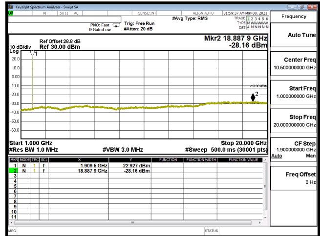
CSE-B2_1.4M-CH19193-QPSK(3,3)-1G-20G
