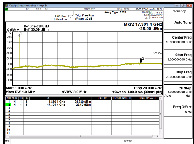
CSE-B2_20M-CH18700-16QAM(1,50)-1G-20G
