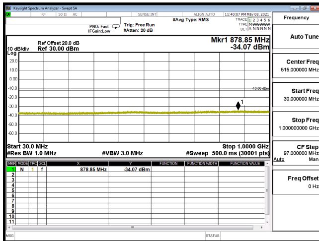
CSE-B2_5M-CH19175-QPSK(1,12)-30M-1G
