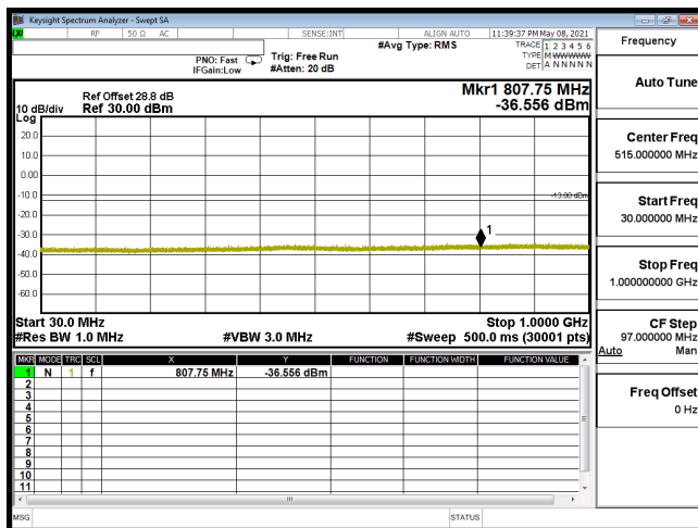
CSE-B2_5M-CH18900-16QAM(1,12)-30M-1G
