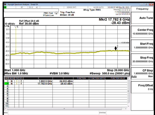
CSE-B2_15M-CH19125-16QAM(1,37)-1G-20G
