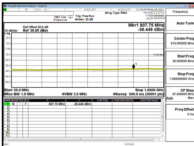
CSE-B2_5M-CH18900-64QAM(1,0)-30M-1G
