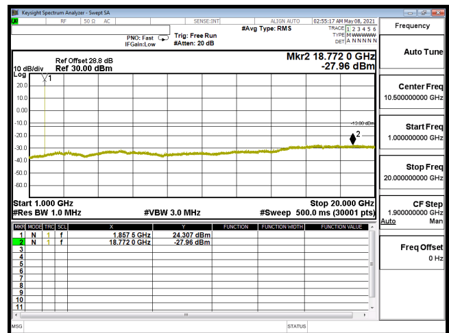
CSE-B2_15M-CH18675-16QAM(1,37)-1G-20G
