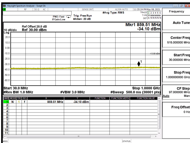
CSE-B2_3M-CH18615-64QAM(1,0)-30M-1G
