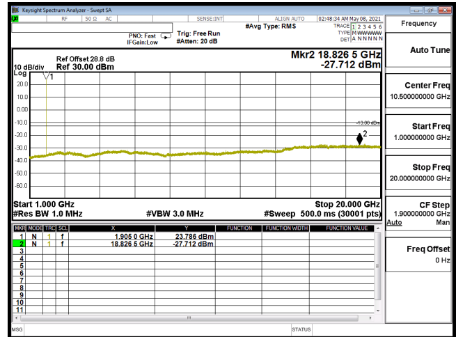
CSE-B2_10M-CH19150-QPSK(1,25)-1G-20G
