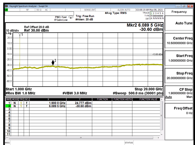
CSE-B2_20M-CH19100-16QAM(1,50)-1G-20G
