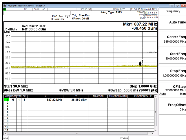
CSE-B2_3M-CH19185-64QAM(1,7)-30M-1G
