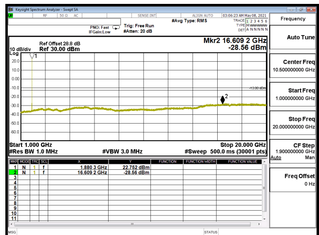
CSE-B2_20M-CH18900-64QAM(1,50)-1G-20G
