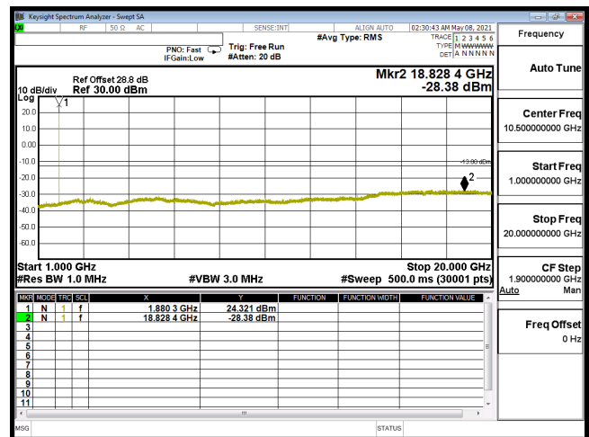
CSE-B2_5M-CH18900-16QAM(1,12)-1G-20G
