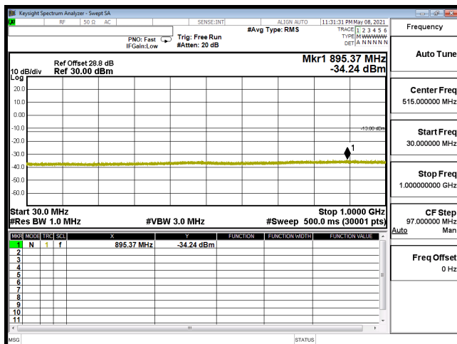
CSE-B2_1.4M-CH18607-64QAM(1,5)-30M-1G
