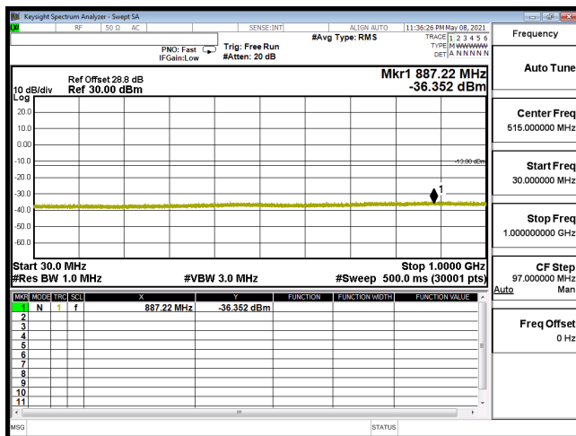
CSE-B2_3M-CH19185-16QAM(1,0)-30M-1G
