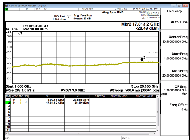
CSE-B2_15M-CH19125-64QAM(1,37)-1G-20G
