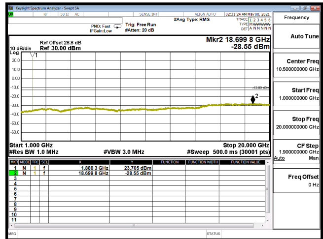
CSE-B2_5M-CH18900-QPSK(1,12)-1G-20G
