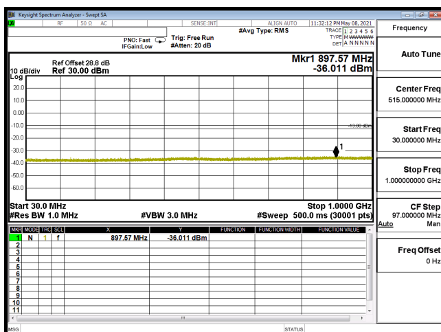
CSE-B2_1.4M-CH18900-64QAM(1,2)-30M-1G
