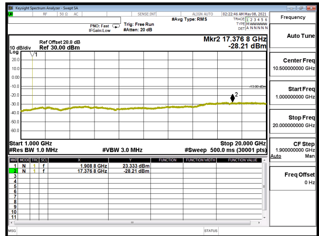
CSE-B2_3M-CH19185-QPSK(1,7)-1G-20G
