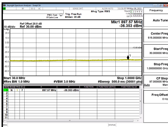
CSE-B2_1.4M-CH18900-16QAM(1,5)-30M-1G
