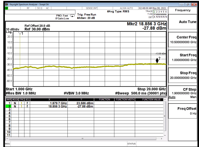
CSE-B2_10M-CH18900-QPSK(1,25)-1G-20G
