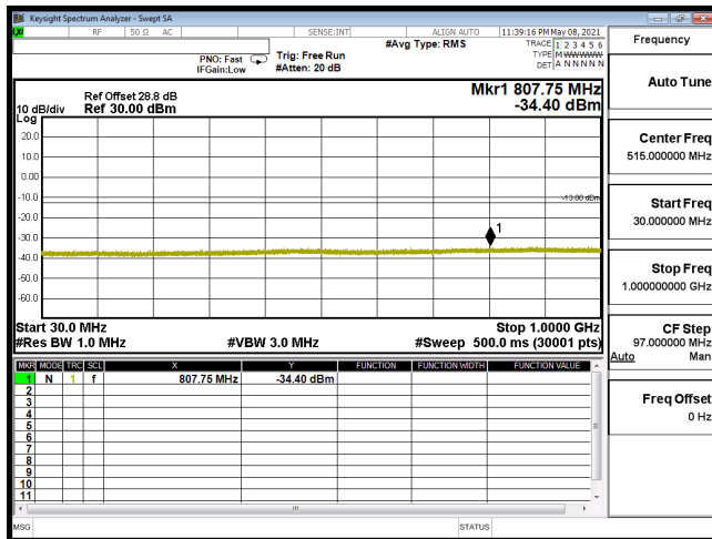
CSE-B2_5M-CH18900-QPSK(1,12)-30M-1G
