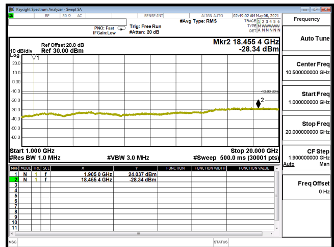
CSE-B2_10M-CH19150-16QAM(1,25)-1G-20G
