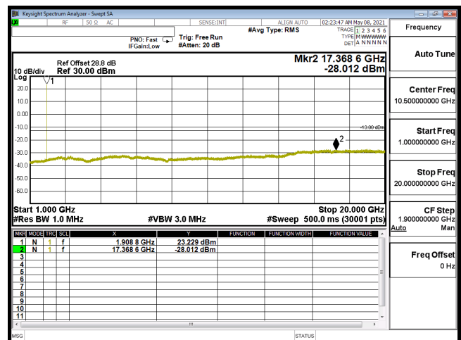
CSE-B2_3M-CH19185-64QAM(1,7)-1G-20G
