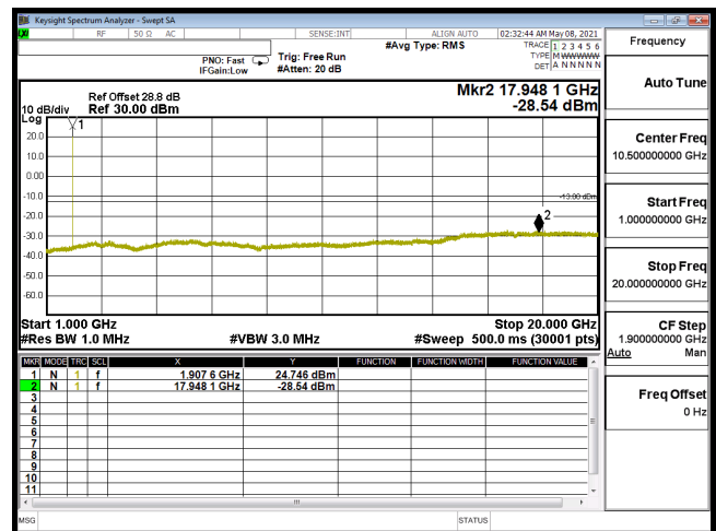
CSE-B2_5M-CH19175-16QAM(1,12)-1G-20G
