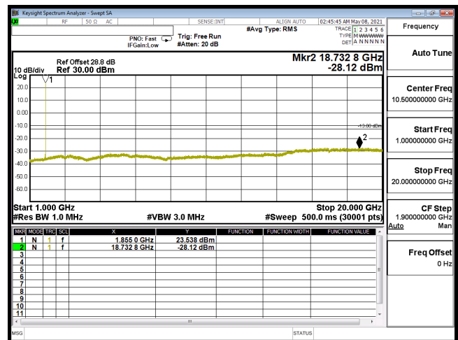
CSE-B2_10M-CH18625-16QAM(1,25)-1G-20G
