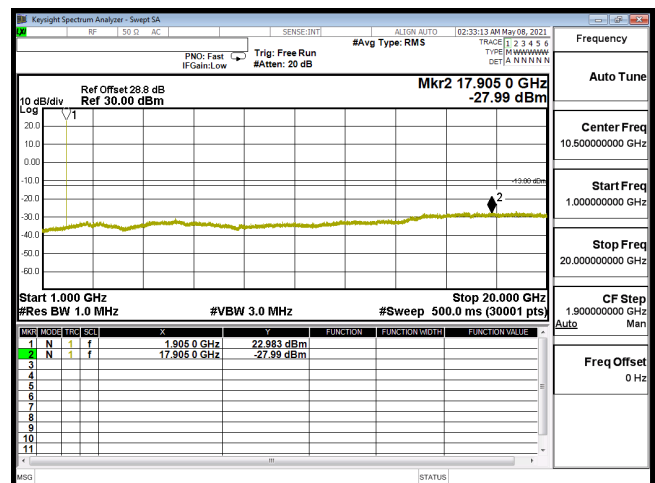
CSE-B2_5M-CH19175-64QAM(1,0)-1G-20G
