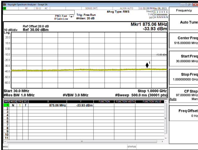
CSE-B2_1.4M-CH19193-QPSK(3,3)-30M-1G
