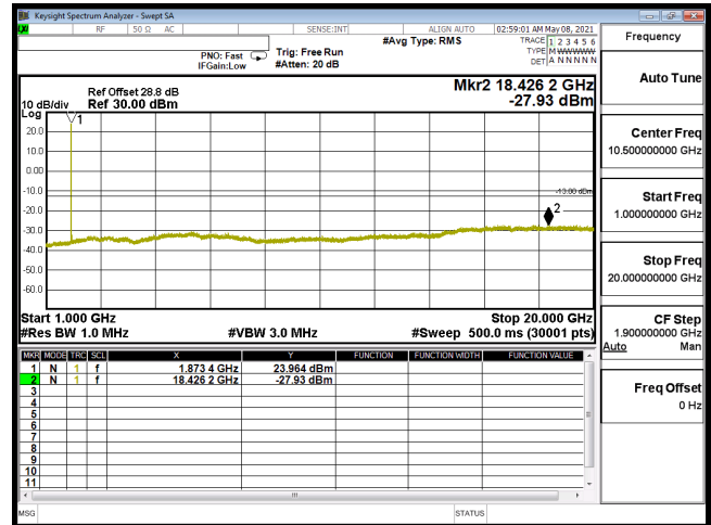
CSE-B2_15M-CH18900-QPSK(1,0)-1G-20G
