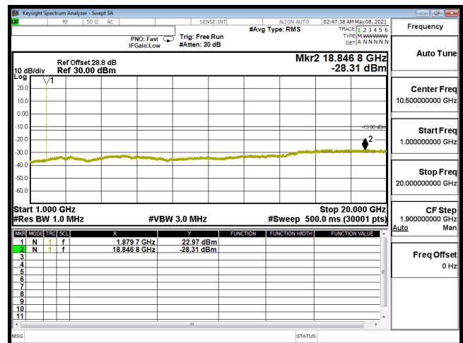
CSE-B2_10M-CH18900-16QAM(1,25)-1G-20G
