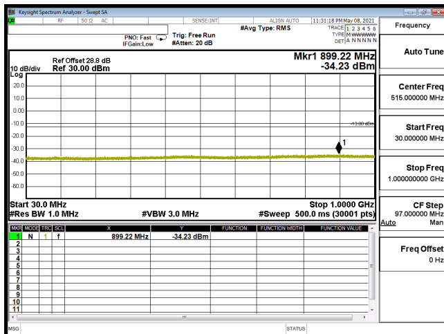
CSE-B2_1.4M-CH18607-16QAM(1,0)-30M-1G
