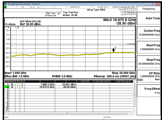
CSE-B2_20M-CH18900-QPSK(1,50)-1G-20G
