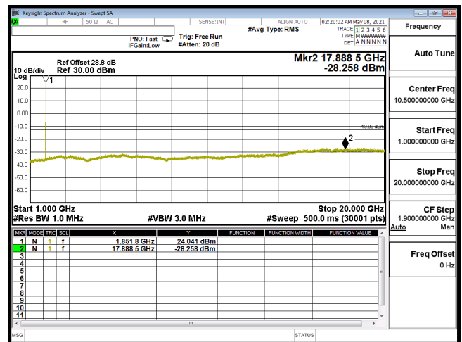
CSE-B2_3M-CH18615-16QAM(1,7)-1G-20G
