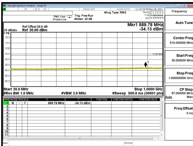
CSE-B2_1.4M-CH19193-16QAM(1,0)-30M-1G
