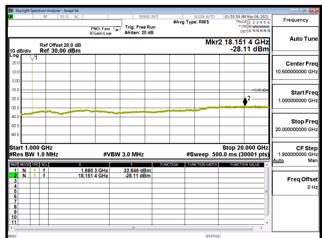
CSE-B2_1.4M-CH18900-64QAM(1,2)-1G-20G
