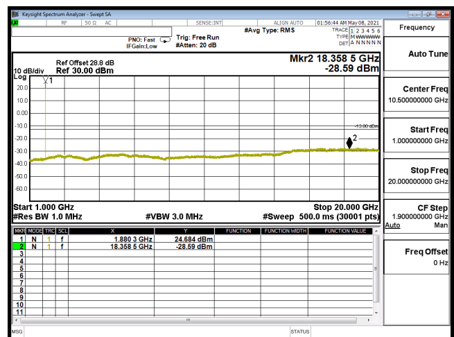
CSE-B2_1.4M-CH18900-16QAM(1,5)-1G-20G
