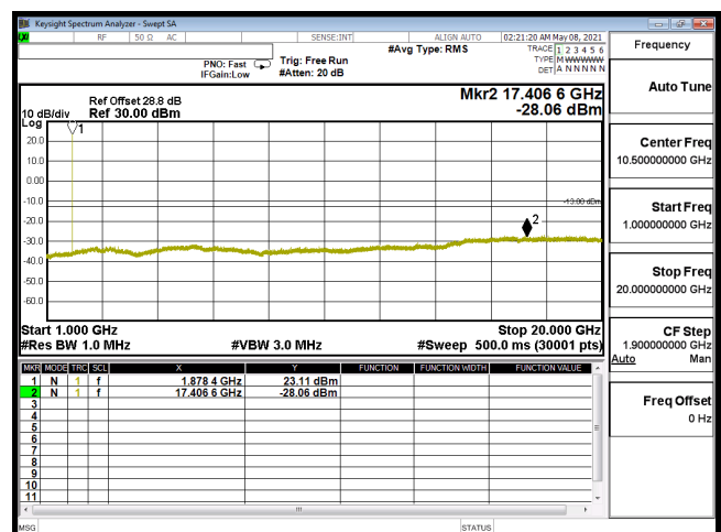
CSE-B2_3M-CH18900-64QAM(1,0)-1G-20G
