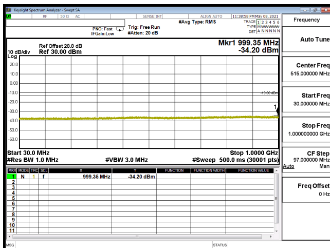
CSE-B2_5M-CH18625-64QAM(1,0)-30M-1G
