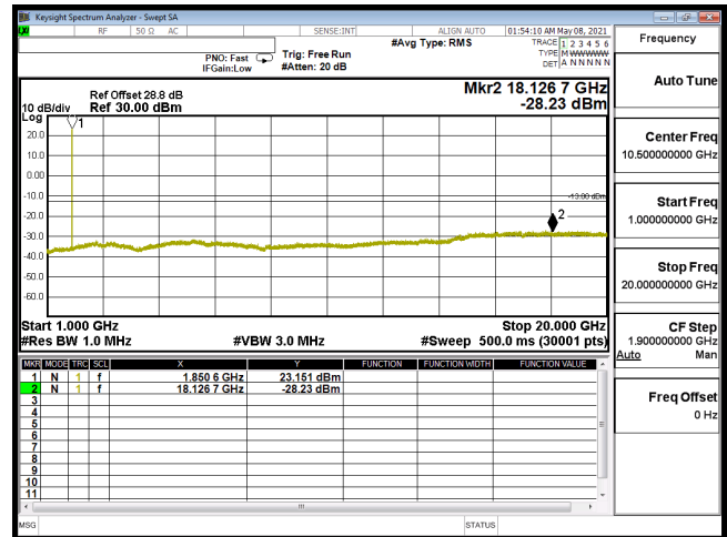
CSE-B2_1.4M-CH18607-QPSK(1,0)-1G-20G
