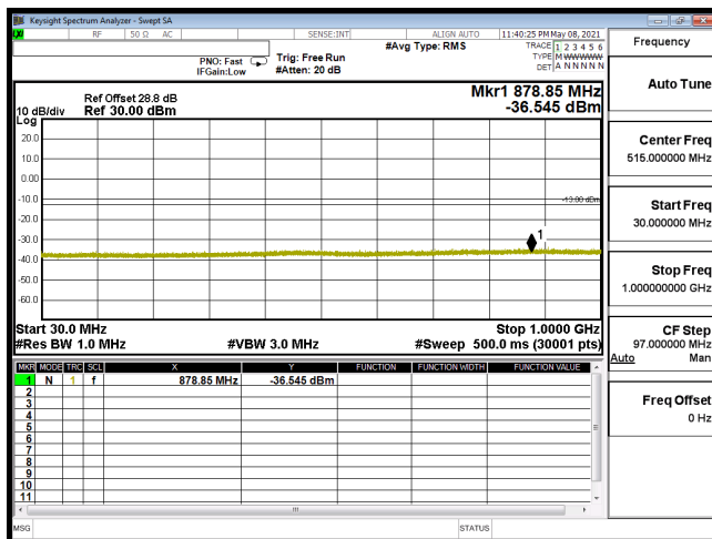
CSE-B2_5M-CH19175-16QAM(1,12)-30M-1G
