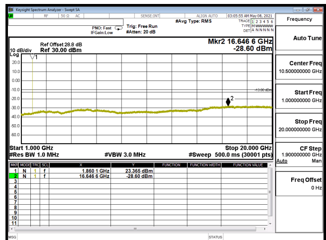
CSE-B2_20M-CH18700-64QAM(1,50)-1G-20G
