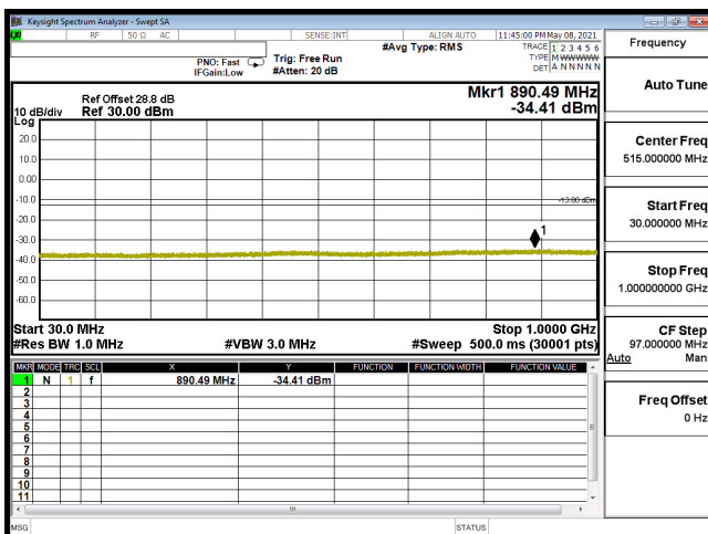
CSE-B2_10M-CH19150-64QAM(1,25)-1G-20G
