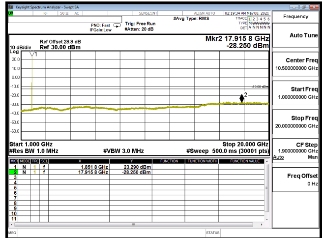
CSE-B2_3M-CH18615-QPSK(1,7)-1G-20G
