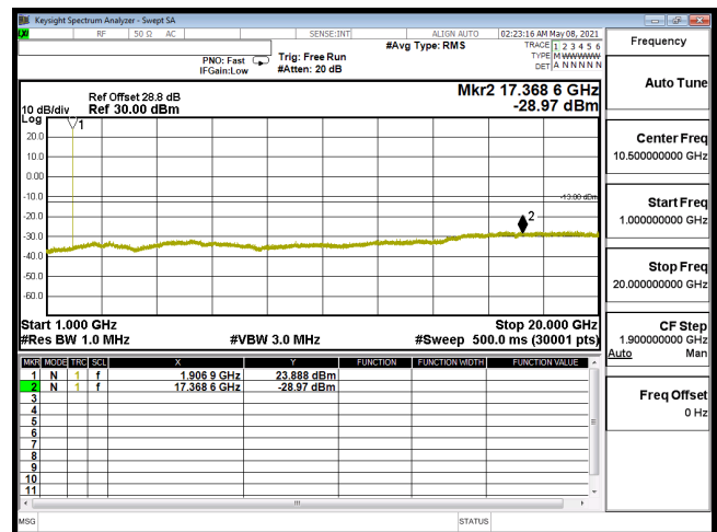
CSE-B2_3M-CH19185-16QAM(1,0)-1G-20G
