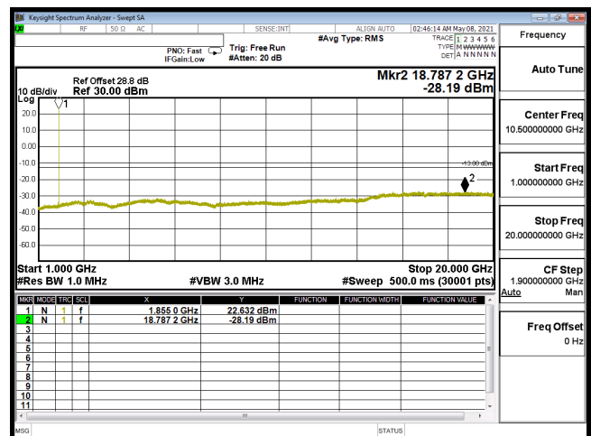
CSE-B2_10M-CH18625-64QAM(1,25)-1G-20G
