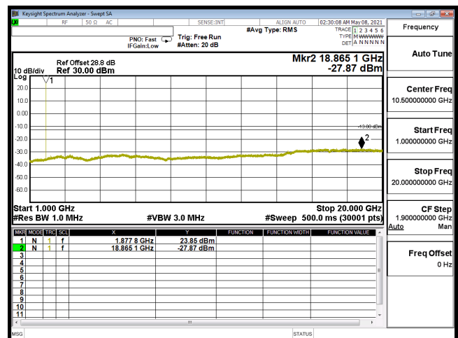
CSE-B2_5M-CH18900-64QAM(1,0)-1G-20G
