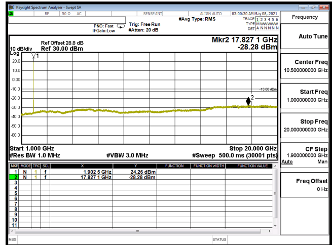
CSE-B2_15M-CH19125-QPSK(1,37)-1G-20G
