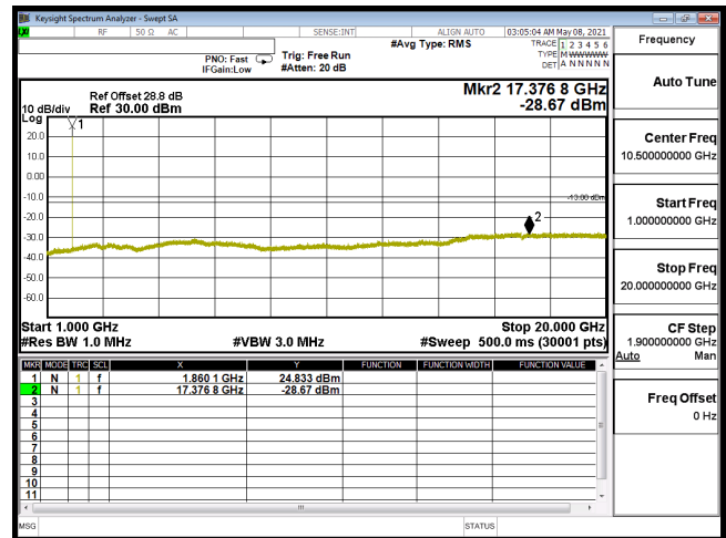
CSE-B2_20M-CH18700-QPSK(1,50)-1G-20G
