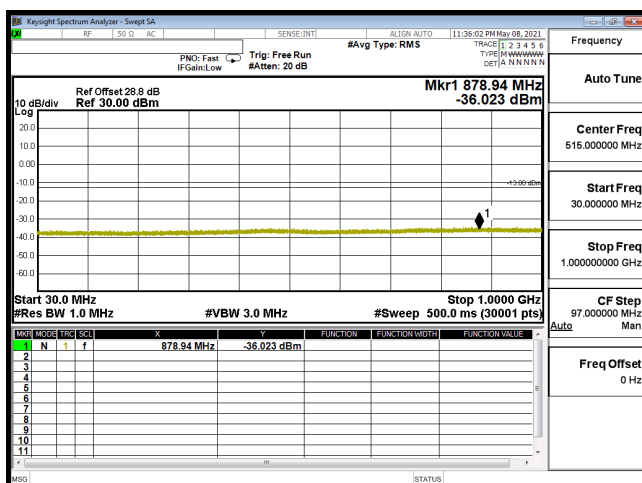
CSE-B2_3M-CH18900-64QAM(1,0)-30M-1G
