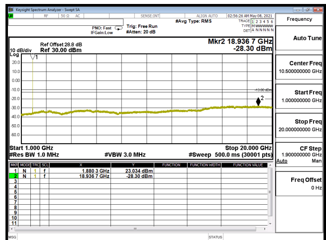
CSE-B2_15M-CH18900-64QAM(1,37)-1G-20G
