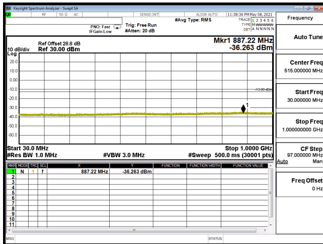
CSE-B2_5M-CH18625-QPSK(1,12)-30M-1G
