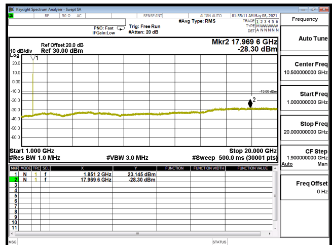
CSE-B2_1.4M-CH18607-64QAM(1,5)-1G-20G
