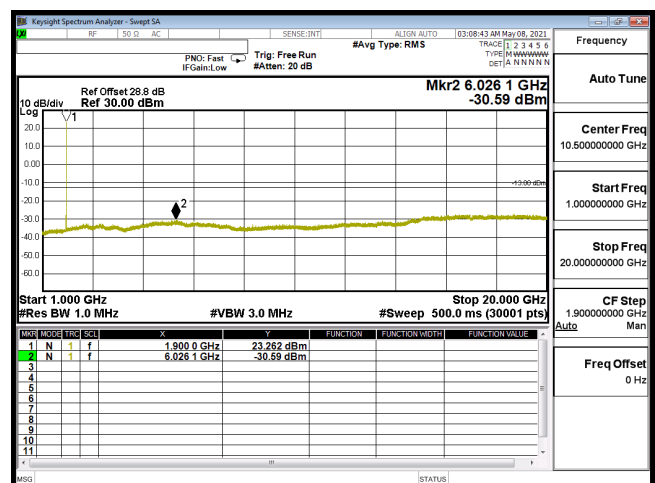
CSE-B2_20M-CH19100-64QAM(1,50)-1G-20G
