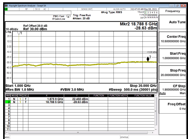
CSE-B2_10M-CH18900-64QAM(1,0)-1G-20G
