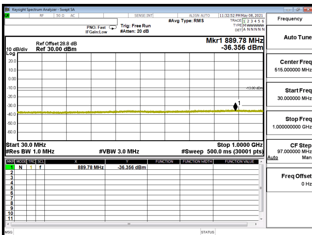
CSE-B2_1.4M-CH19193-64QAM(1,0)-30M-1G
