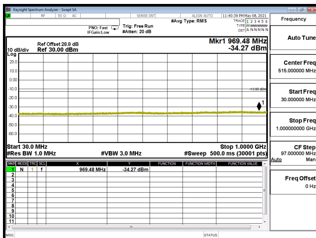
CSE-B2_5M-CH19175-64QAM(1,0)-30M-1G
