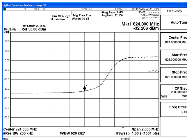
EDGE(10M+10M)-2ULCA_5B-64QAM_829(50,0)+838.9(50,0)
