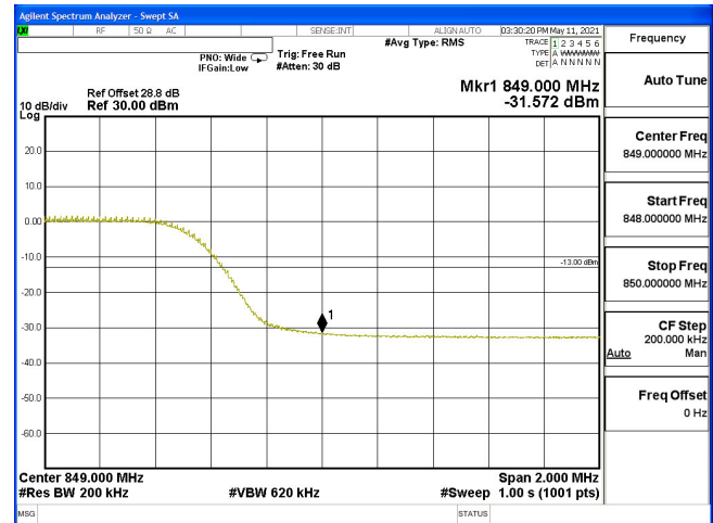
EDGE(10M+10M)-2ULCA_5B-QPSK_834.1(50,0)+844(50,0)
