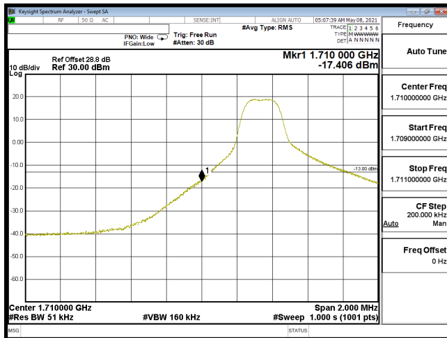
EDGE-B66_5M-CH131997-QPSK(1,0)
