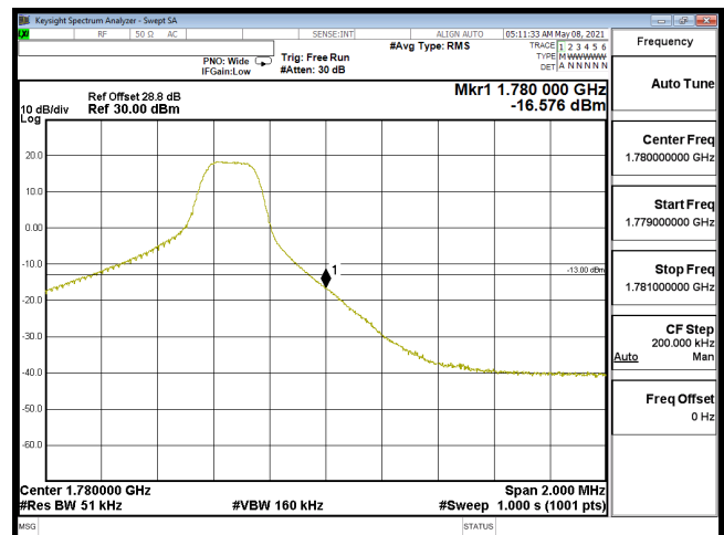
EDGE-B66_5M-CH132647-16QAM(1,24)
