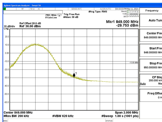
EDGE(10M+10M)-2ULCA_5B-16QAM_834.1(1,0)+844(1,49)
