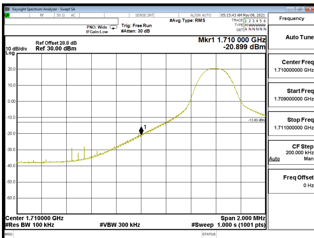
EDGE-B66_10M-CH132022-16QAM(1,0)
