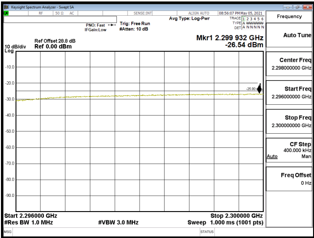
EDGE-B30_10M-CH27710-QPSK(50,0)-Verify2
