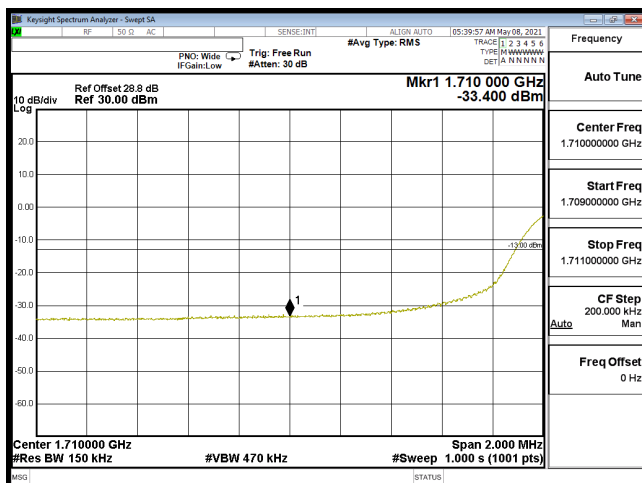
EDGE-B66_20M-CH132072-64QAM(100,0)
