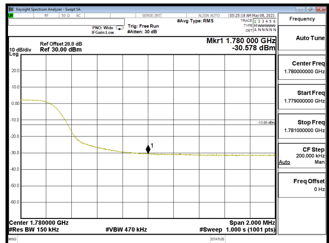
EDGE-B66_15M-CH132597-16QAM(75,0)
