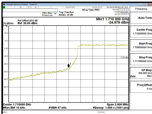
EDGE-B66_1.4M-CH131979-16QAM(6,0)
