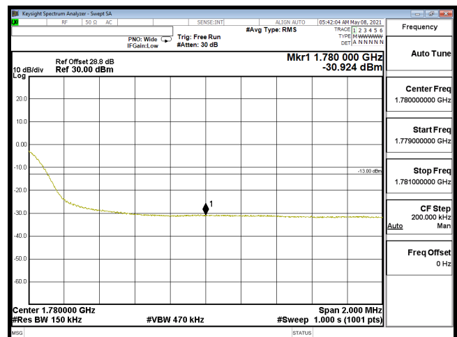
EDGE-B66_20M-CH132572-64QAM(100,0)
