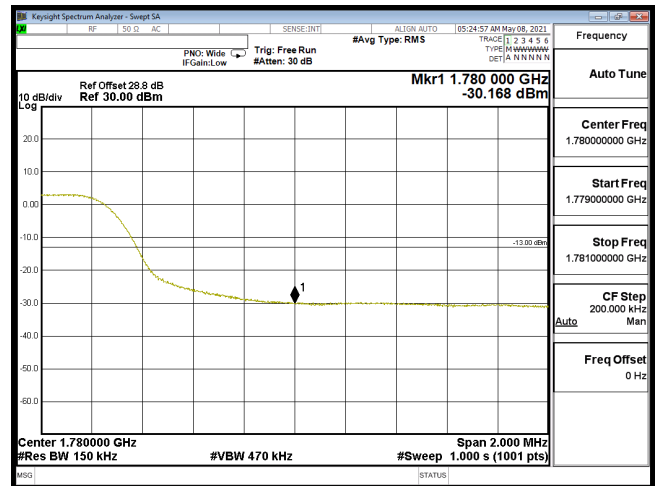
EDGE-B66_15M-CH132597-QPSK(75,0)
