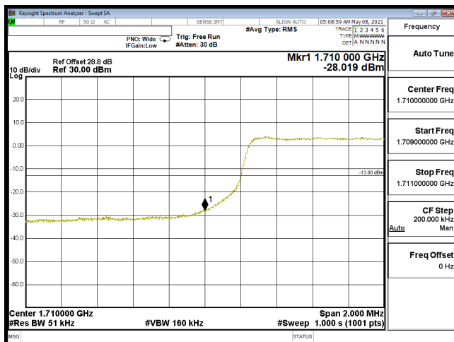
EDGE-B66_5M-CH131997-16QAM(25,0)
