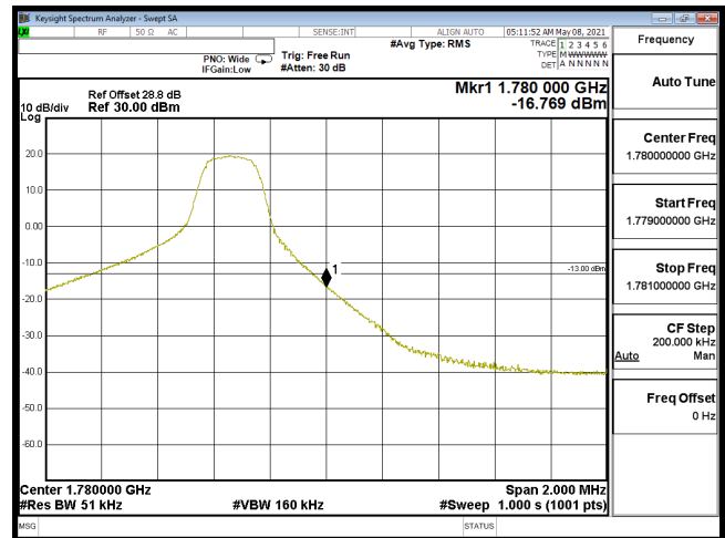
EDGE-B66_5M-CH132647-QPSK(1,24)
