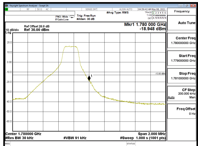
EDGE-B66_3M-CH132657-16QAM(1,14)
