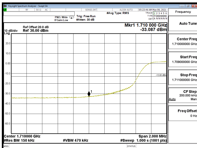
EDGE-B66_15M-CH132047-64QAM(75,0)
