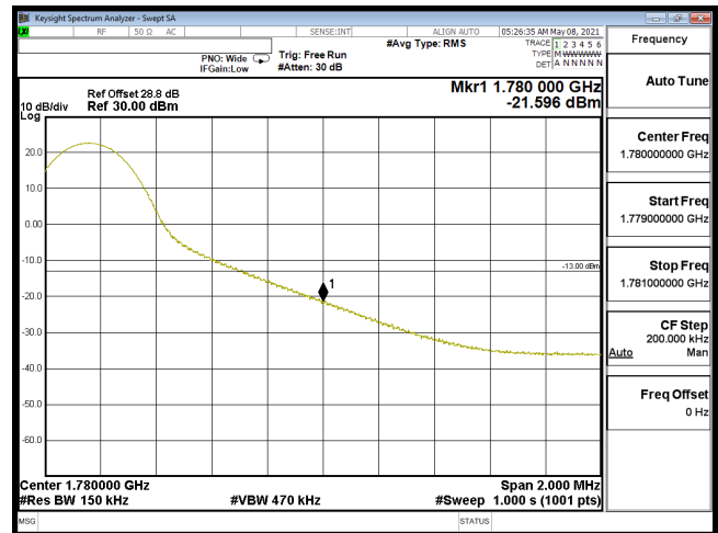
EDGE-B66_15M-CH132597-QPSK(1,74)
