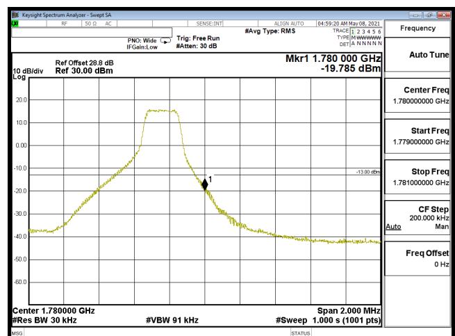
EDGE-B66_3M-CH132657-64QAM(1,14)
