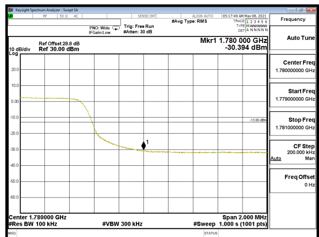
EDGE-B66_10M-CH132622-16QAM(50,0)
