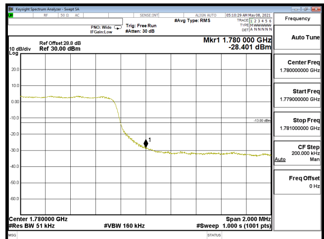
EDGE-B66_5M-CH132647-16QAM(25,0)
