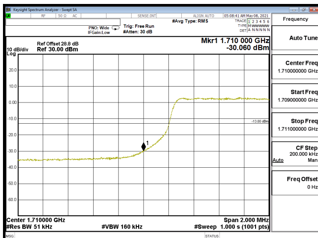
EDGE-B66_5M-CH131997-64QAM(25,0)
