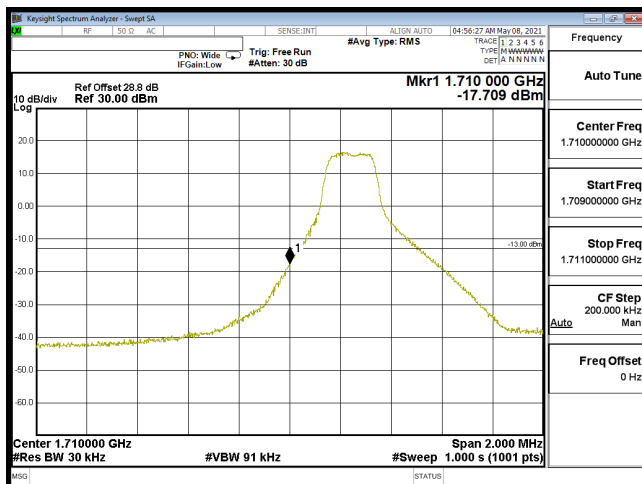
EDGE-B66_3M-CH131987-16QAM(1,0)
