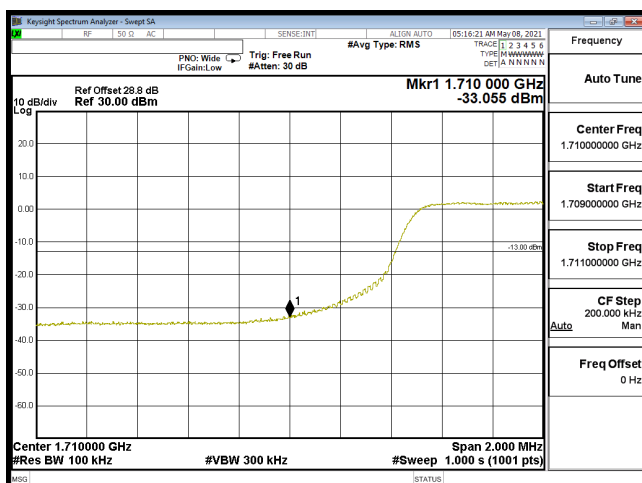
EDGE-B66_10M-CH132022-64QAM(50,0)
