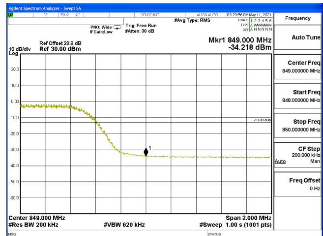
EDGE(10M+10M)-2ULCA_5B-16QAM_834.1(50,0)+844(50,0)
