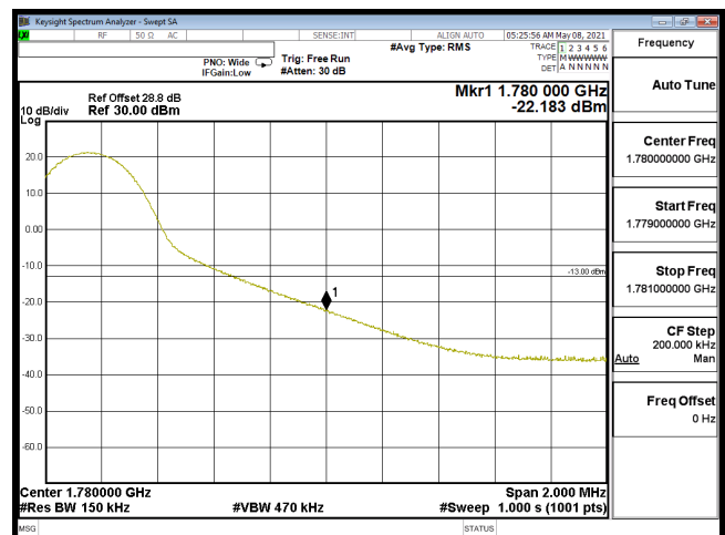
EDGE-B66_15M-CH132597-64QAM(1,74)
