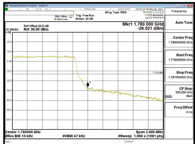
EDGE-B66_1.4M-CH132665-16QAM(6,0)
