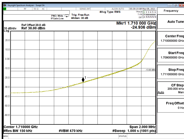
EDGE-B66_20M-CH132072-16QAM(1,0)
