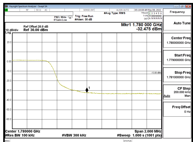
EDGE-B66_10M-CH132622-64QAM(50,0)
