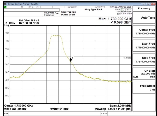
EDGE-B66_3M-CH132657-QPSK(1,14)
