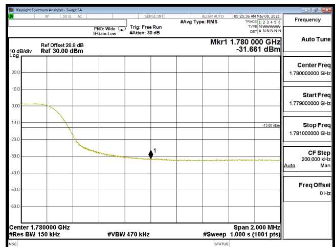
EDGE-B66_15M-CH132597-64QAM(75,0)
