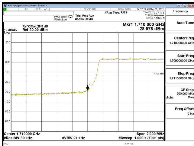
EDGE-B66_3M-CH131987-16QAM(15,0)
