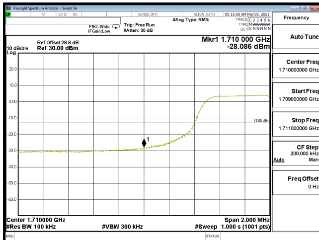
EDGE-B66_10M-CH132022-QPSK(50,0)
