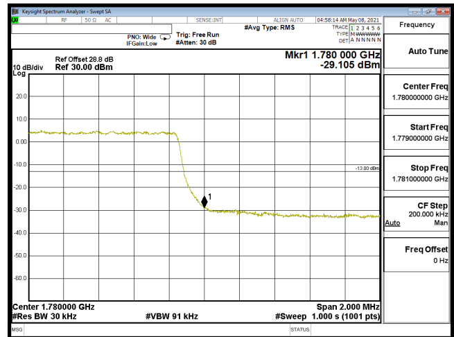
EDGE-B66_3M-CH132657-QPSK(15,0)
