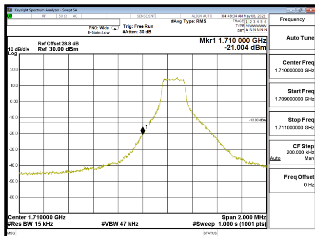
EDGE-B66_1.4M-CH131979-QPSK(1,0)
