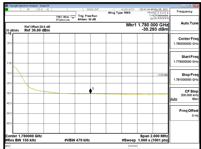
EDGE-B66_20M-CH132572-16QAM(100,0)
