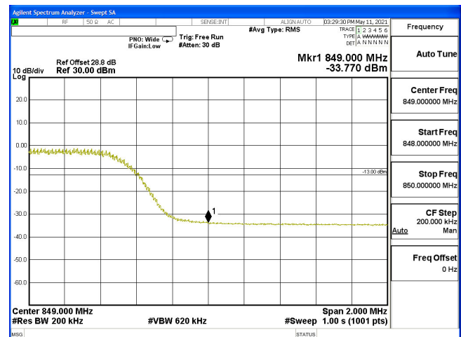
EDGE(10M+10M)-2ULCA_5B-64QAM_834.1(50,0)+844(50,0)
