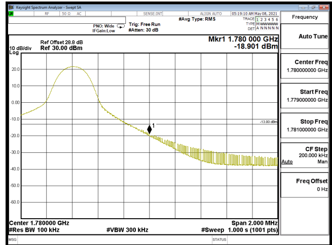
EDGE-B66_10M-CH132622-QPSK(1,49)
