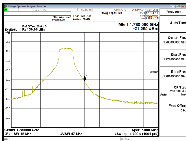
EDGE-B66_1.4M-CH132665-64QAM(1,5)
