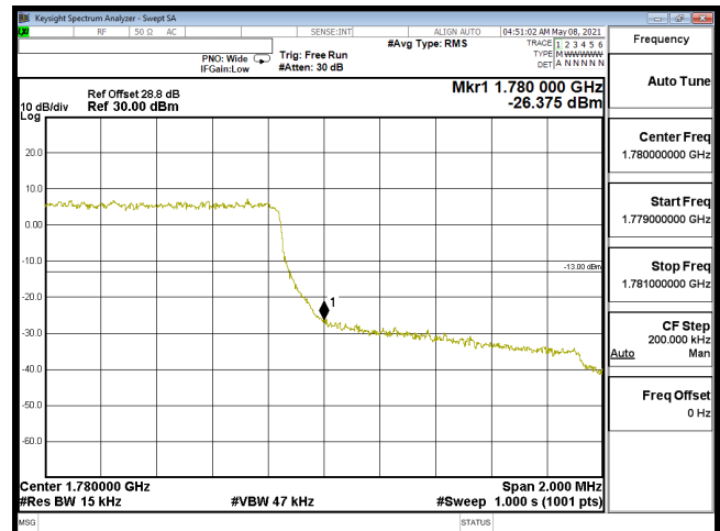
EDGE-B66_1.4M-CH132665-QPSK(6,0)
