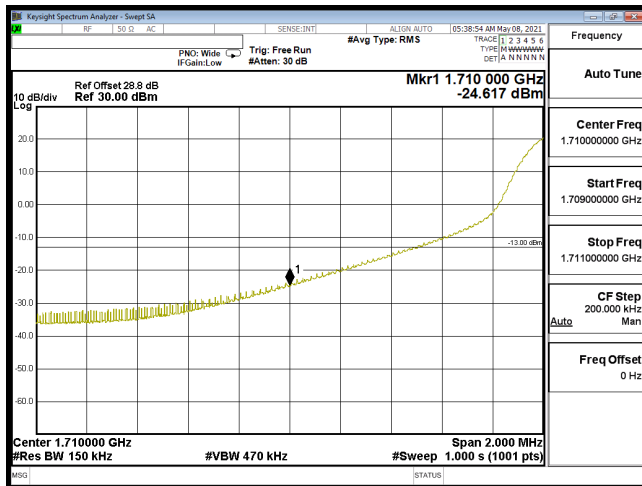
EDGE-B66_20M-CH132072-QPSK(1,0)
