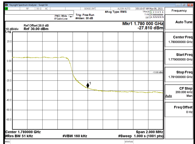
EDGE-B66_5M-CH132647-QPSK(25,0)
