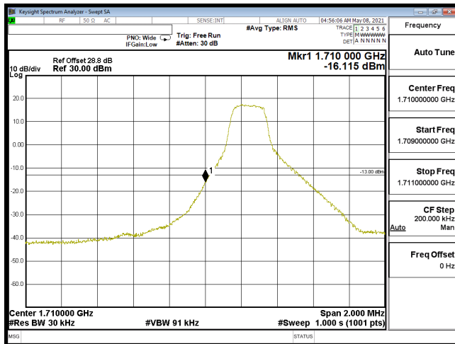
EDGE-B66_3M-CH131987-QPSK(1,0)
