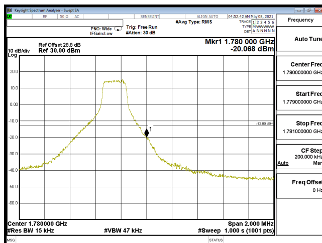
EDGE-B66_1.4M-CH132665-QPSK(1,5)
