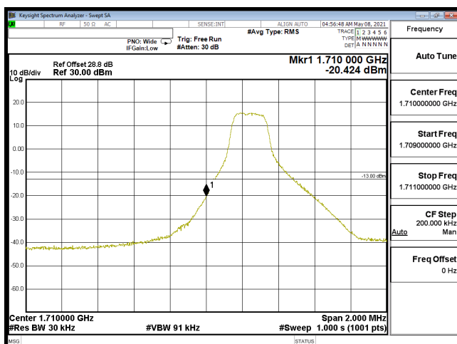
EDGE-B66_3M-CH131987-64QAM(1,0)
