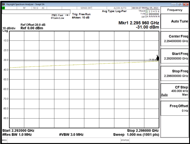
EDGE-B30_10M-CH27710-QPSK(50,0)-Verify1
