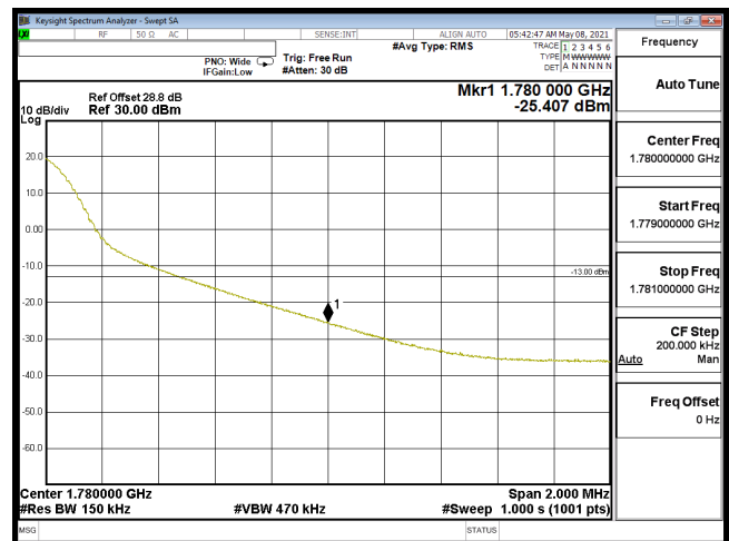
EDGE-B66_20M-CH132572-16QAM(1,99)
