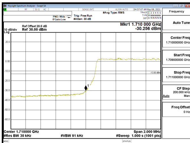
EDGE-B66_3M-CH131987-64QAM(15,0)
