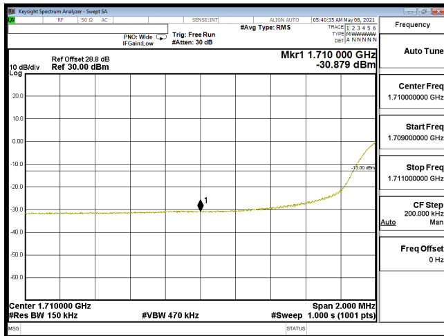
EDGE-B66_20M-CH132072-QPSK(100,0)
