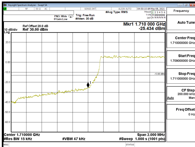
EDGE-B66_1.4M-CH131979-QPSK(6,0)
