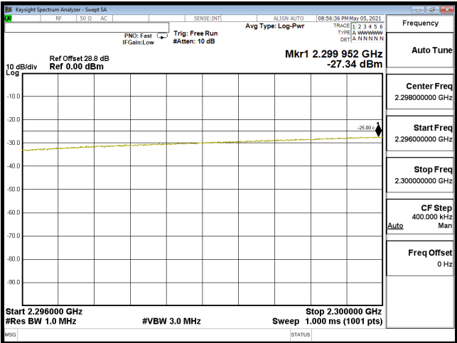
EDGE-B30_10M-CH27710-16QAM(50,0)-Verify
