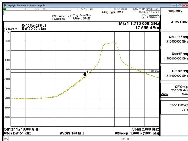
EDGE-B66_5M-CH131997-16QAM(1,0)
