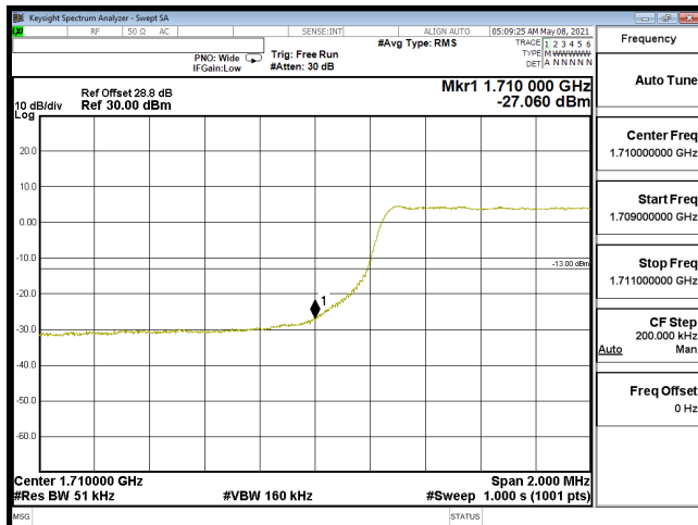
EDGE-B66_5M-CH131997-QPSK(25,0)
