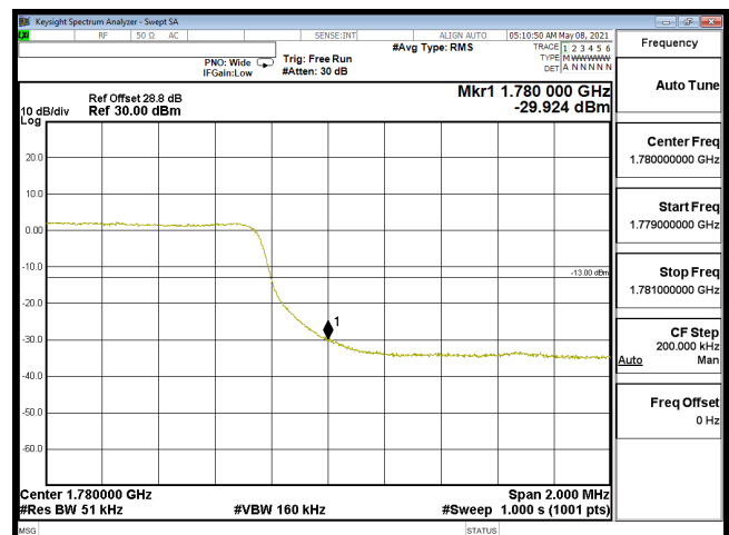
EDGE-B66_5M-CH132647-64QAM(25,0)
