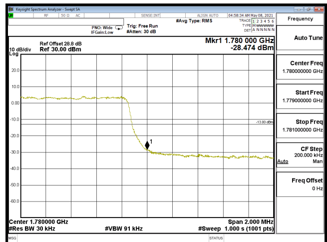
EDGE-B66_3M-CH132657-16QAM(15,0)
