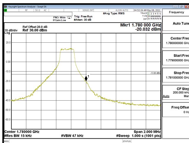
EDGE-B66_1.4M-CH132665-16QAM(1,5)
