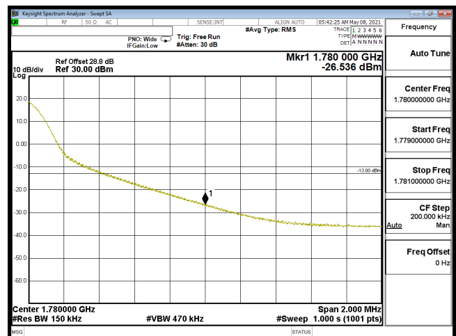
EDGE-B66_20M-CH132572-64QAM(1,99)
