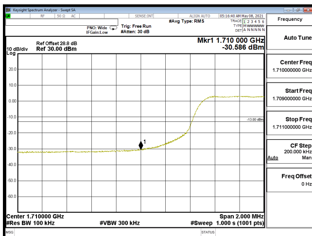
EDGE-B66_10M-CH132022-16QAM(50,0)
