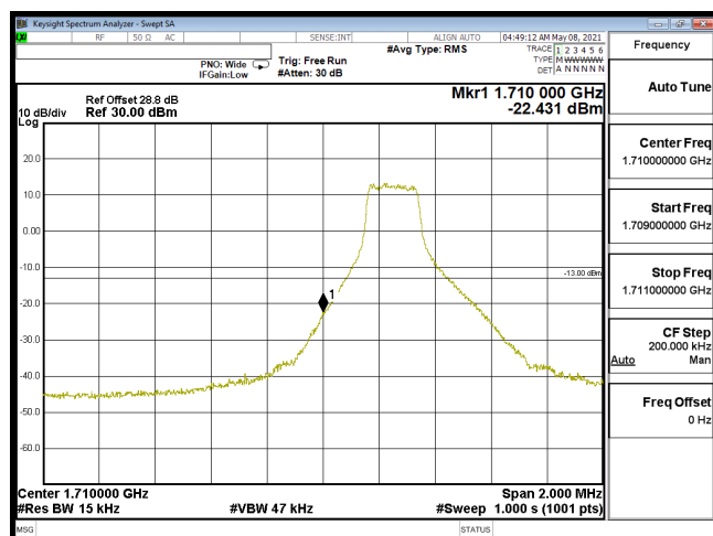
EDGE-B66_1.4M-CH131979-64QAM(1,0)
