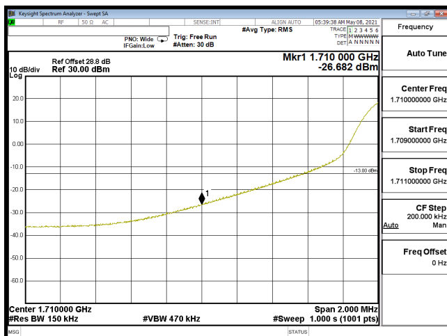
EDGE-B66_20M-CH132072-64QAM(1,0)
