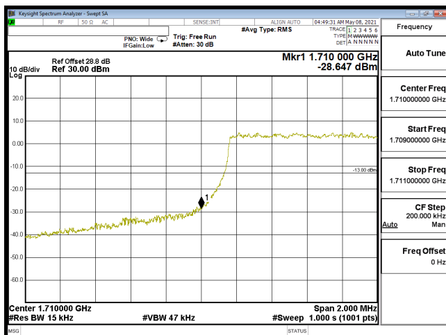
EDGE-B66_1.4M-CH131979-64QAM(6,0)
