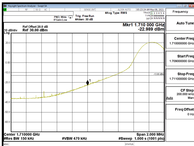
EDGE-B66_15M-CH132047-64QAM(1,0)
