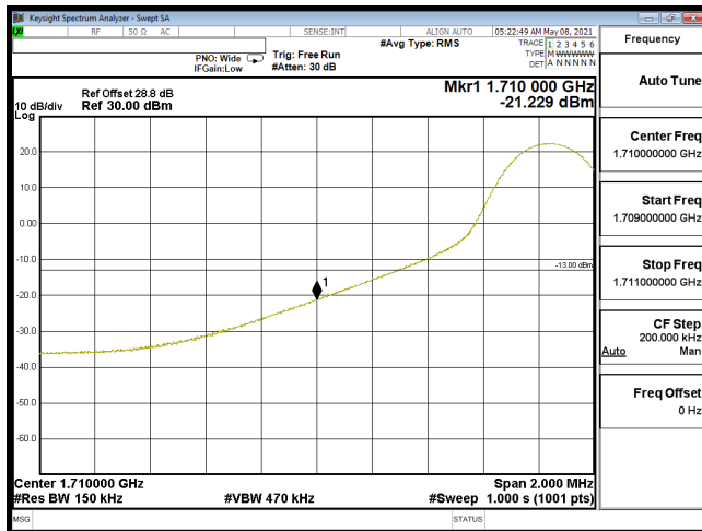
EDGE-B66_15M-CH132047-QPSK(1,0)
