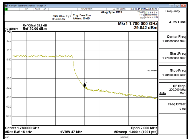
EDGE-B66_1.4M-CH132665-64QAM(6,0)
