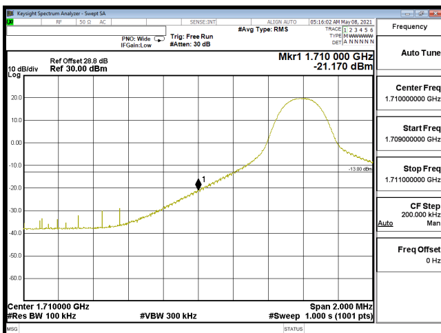
EDGE-B66_10M-CH132022-64QAM(1,0)
