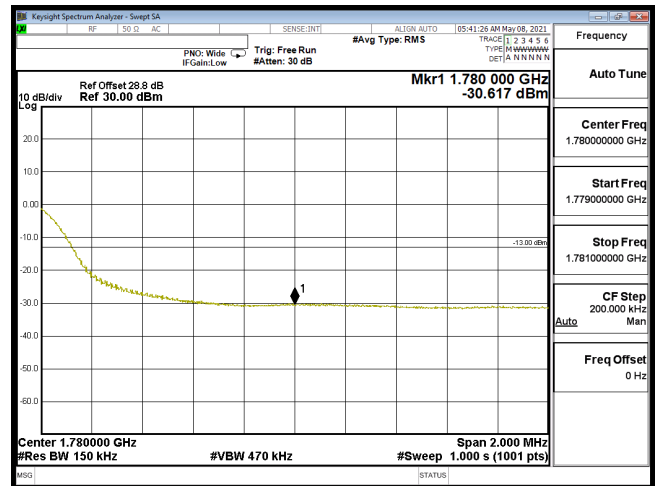
EDGE-B66_20M-CH132572-QPSK(100,0)
