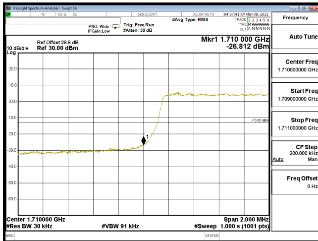
EDGE-B66_3M-CH131987-QPSK(15,0)
