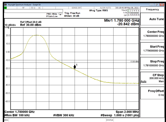
EDGE-B66_10M-CH132622-16QAM(1,49)
