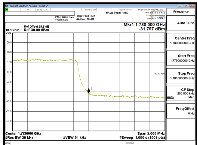
EDGE-B66_3M-CH132657-64QAM(15,0)
