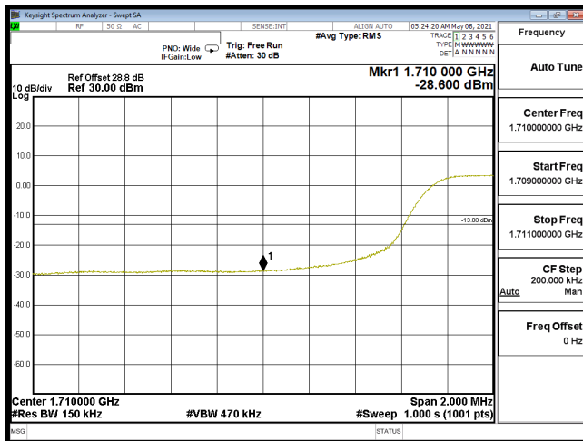
EDGE-B66_15M-CH132047-QPSK(75,0)
