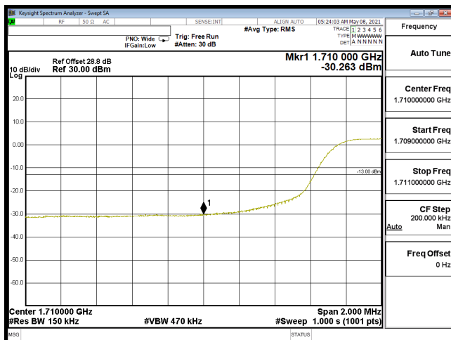
EDGE-B66_15M-CH132047-16QAM(75,0)
