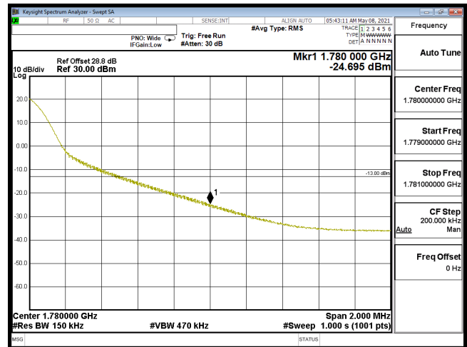
EDGE-B66_20M-CH132572-QPSK(1,99)
