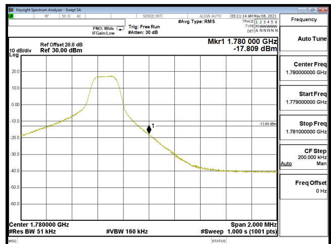
EDGE-B66_5M-CH132647-64QAM(1,24)
