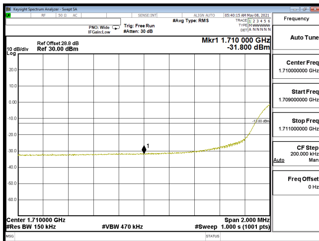
EDGE-B66_20M-CH132072-16QAM(100,0)
