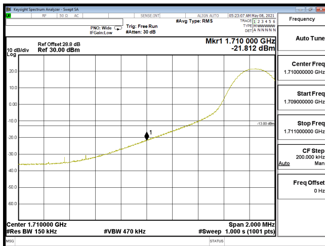
EDGE-B66_15M-CH132047-16QAM(1,0)
