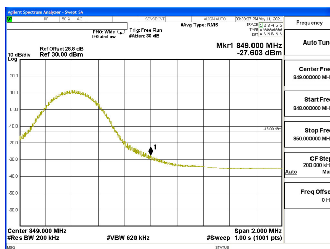
EDGE(10M+10M)-2ULCA_5B-64QAM_834.1(1,0)+844(1,49)
