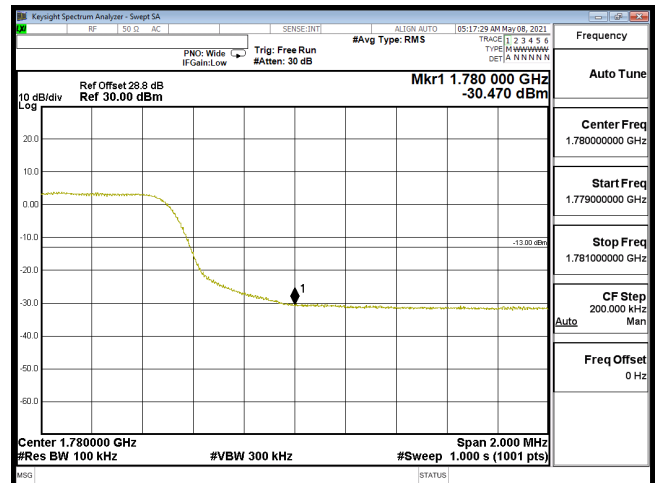
EDGE-B66_10M-CH132622-QPSK(50,0)
