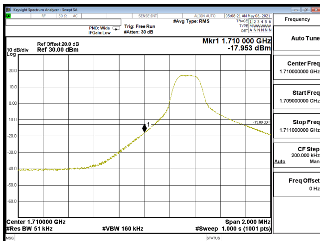
EDGE-B66_5M-CH131997-64QAM(1,0)
