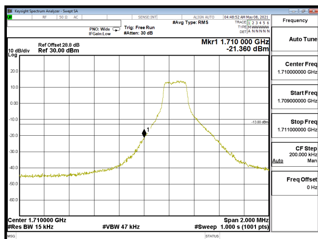
EDGE-B66_1.4M-CH131979-16QAM(1,0)
