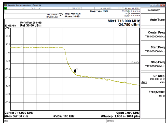
EDGE-B12_1.4M-CH23173-16QAM(6,0)
