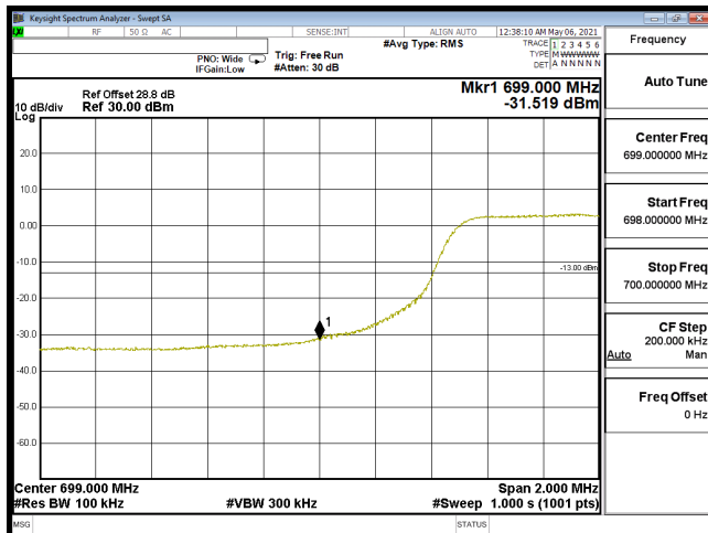
EDGE-B12_10M-CH23060-QPSK(50,0)
