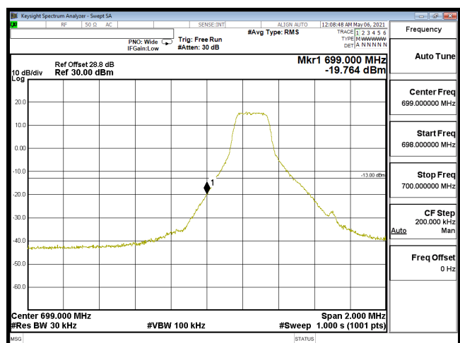
EDGE-B12_1.4M-CH23017-16QAM(1,0)
