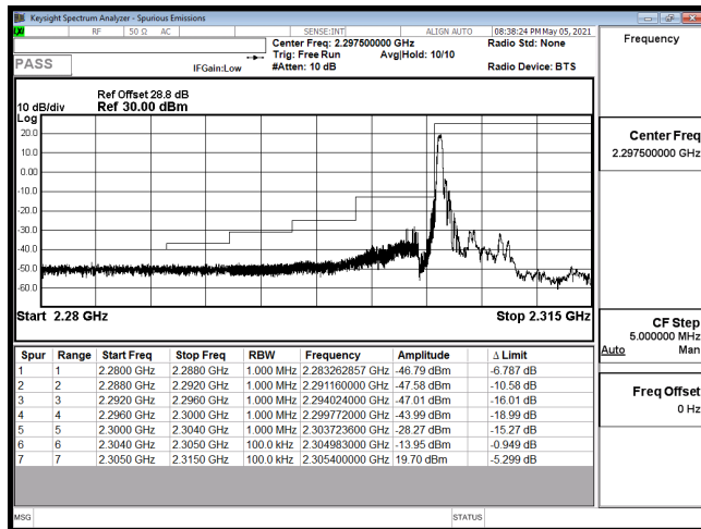
EDGE-B30_5M-CH27685-QPSK(1,0)
