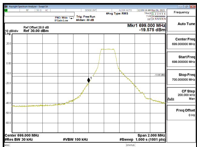
EDGE-B12_1.4M-CH23017-64QAM(1,0)
