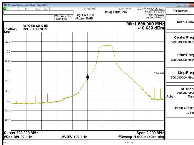
EDGE-B12_3M-CH23025-QPSK(1,0)
