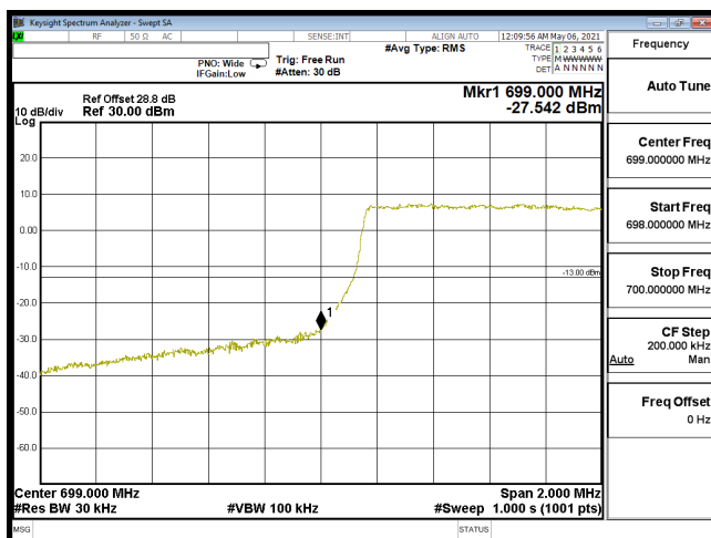
EDGE-B12_1.4M-CH23017-16QAM(6,0)
