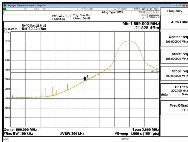
EDGE-B12_10M-CH23060-16QAM(1,0)
