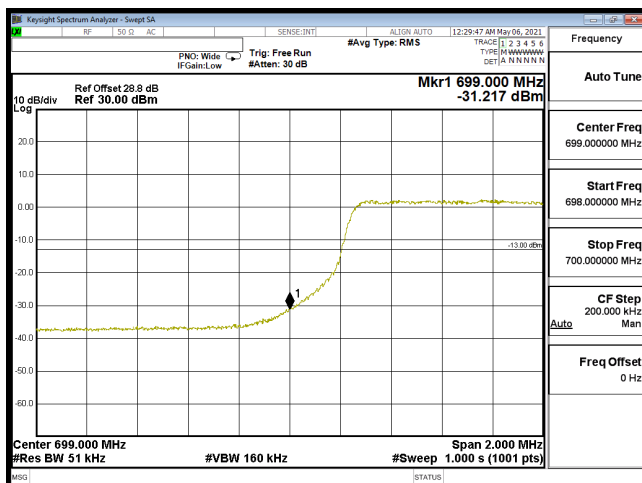
EDGE-B12_5M-CH23035-64QAM(25,0)
