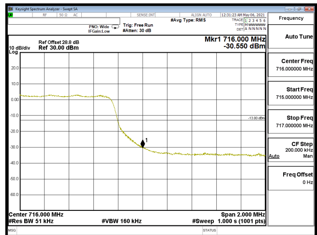
EDGE-B12_5M-CH23155-16QAM(25,0)
