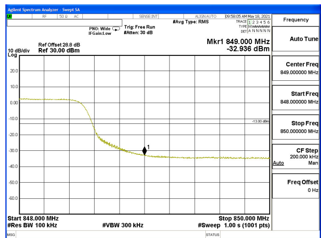
EDGE-B5_10M-CH20600-16QAM(50,0)
