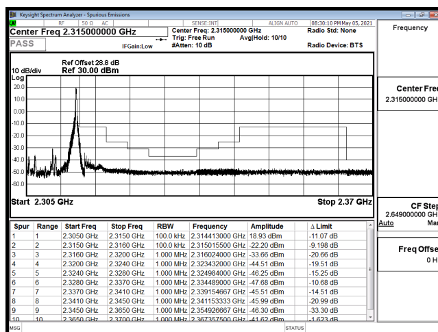
EDGE-B30_10M-CH27710-64QAM(1,49)
