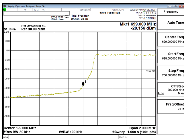
EDGE-B12_1.4M-CH23017-64QAM(6,0)
