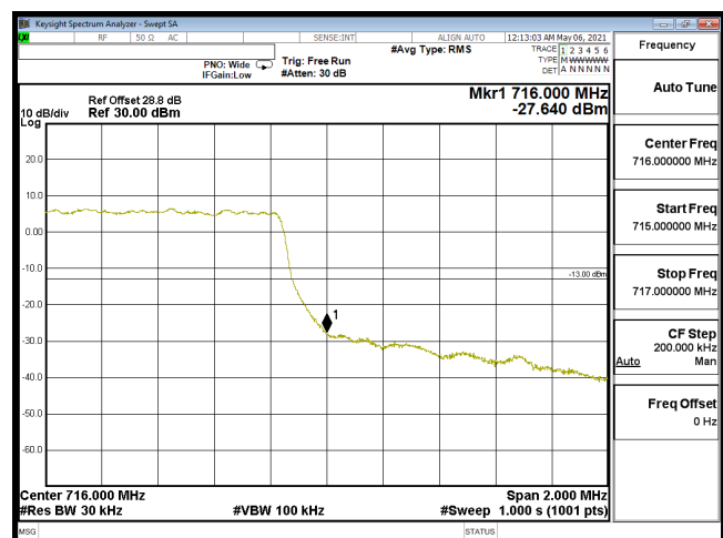
EDGE-B12_1.4M-CH23173-64QAM(6,0)
