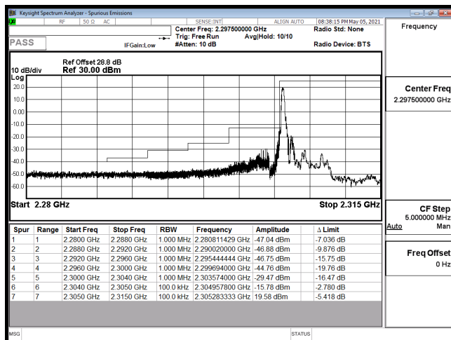
EDGE-B30_5M-CH27685-16QAM(1,0)
