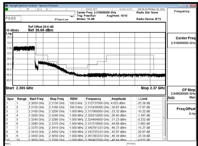
EDGE-B30_10M-CH27710-16QAM(50,0)
