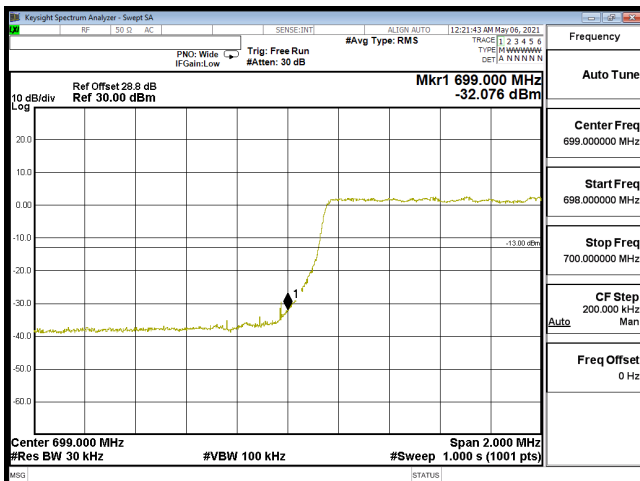
EDGE-B12_3M-CH23025-64QAM(15,0)
