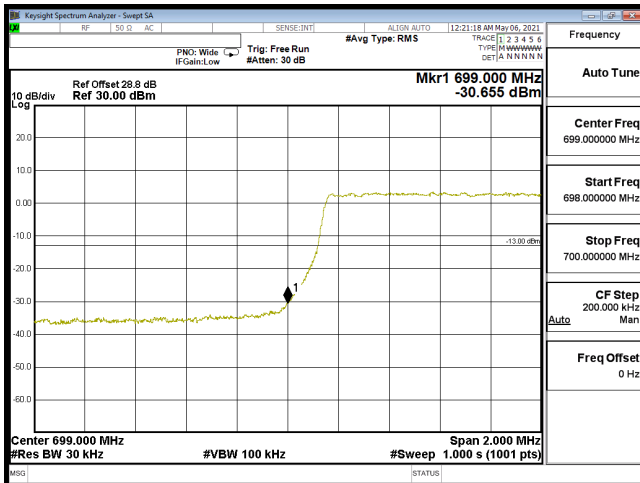
EDGE-B12_3M-CH23025-16QAM(15,0)
