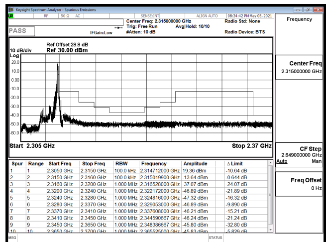
EDGE-B30_5M-CH27735-64QAM(1,24)
