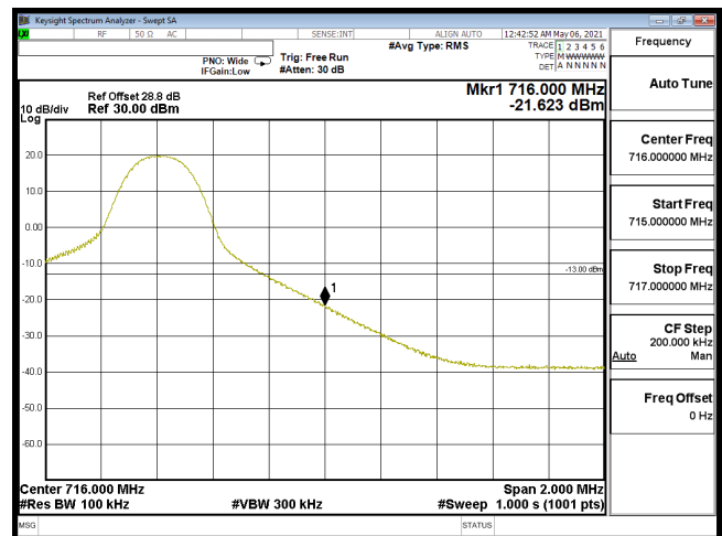
EDGE-B12_10M-CH23130-16QAM(1,49)
