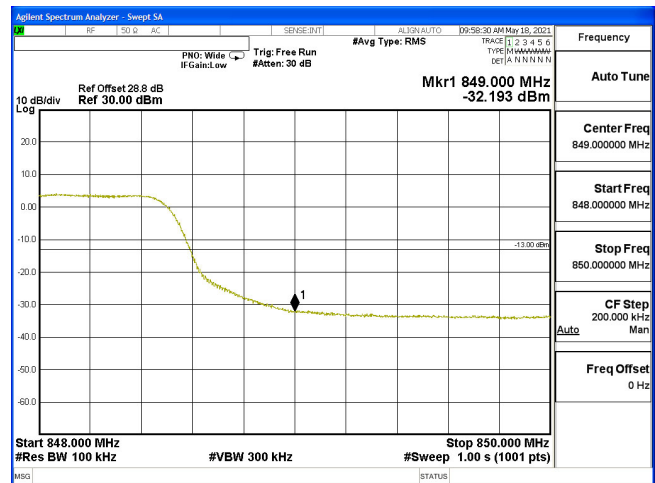
EDGE-B5_10M-CH20600-QPSK(50,0)
