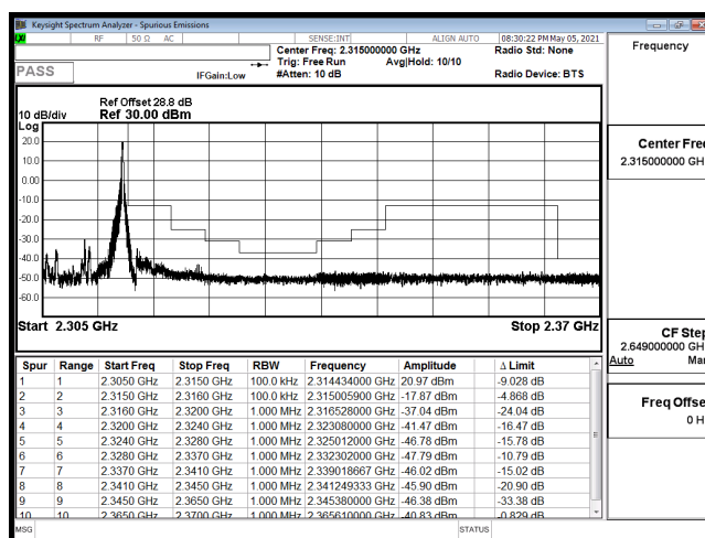
EDGE-B30_10M-CH27710-16QAM(1,49)
