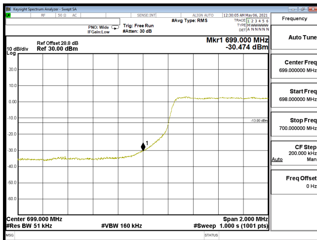
EDGE-B12_5M-CH23035-16QAM(25,0)
