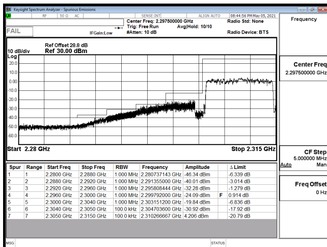
EDGE-B30_10M-CH27710-16QAM(50,0)
