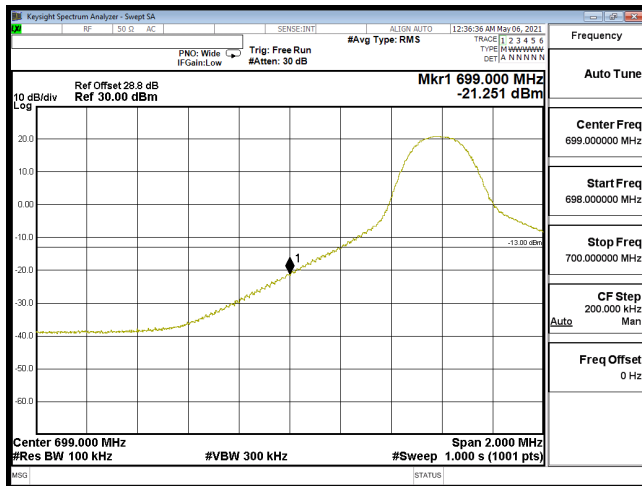
EDGE-B12_10M-CH23060-QPSK(1,0)
