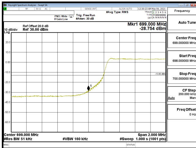
EDGE-B12_5M-CH23035-QPSK(25,0)
