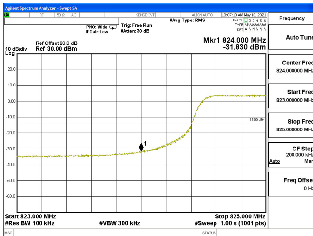
EDGE-B5_10M-CH20450-QPSK(50,0)
