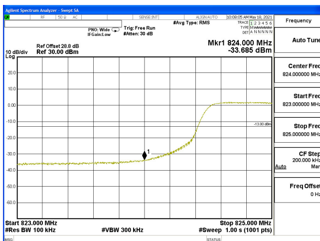
EDGE-B5_10M-CH20450-64QAM(50,0)
