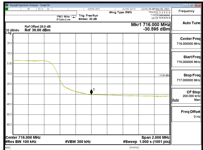
EDGE-B12_10M-CH23130-QPSK(50,0)
