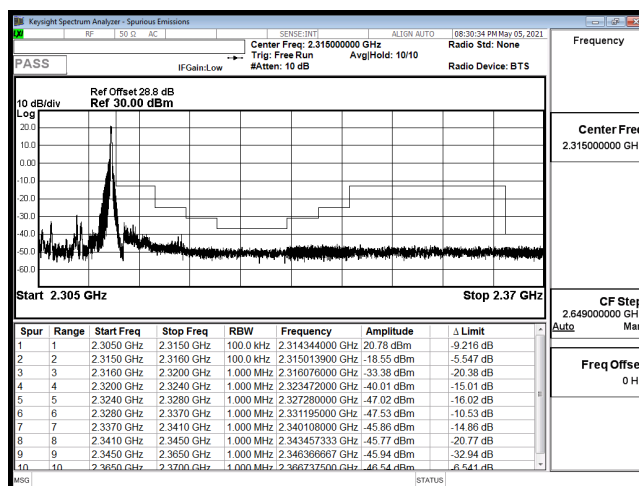
EDGE-B30_10M-CH27710-QPSK(1,49)
