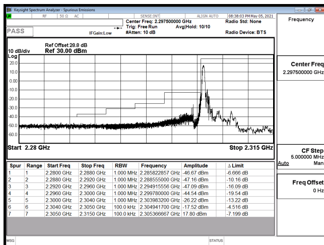
EDGE-B30_5M-CH27685-64QAM(1,0)
