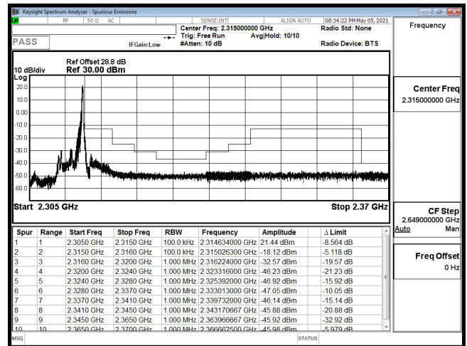
EDGE-B30_5M-CH27735-QPSK(1,24)
