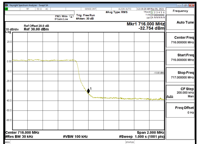
EDGE-B12_3M-CH23165-64QAM(15,0)
