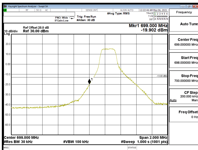
EDGE-B12_3M-CH23025-16QAM(1,0)
