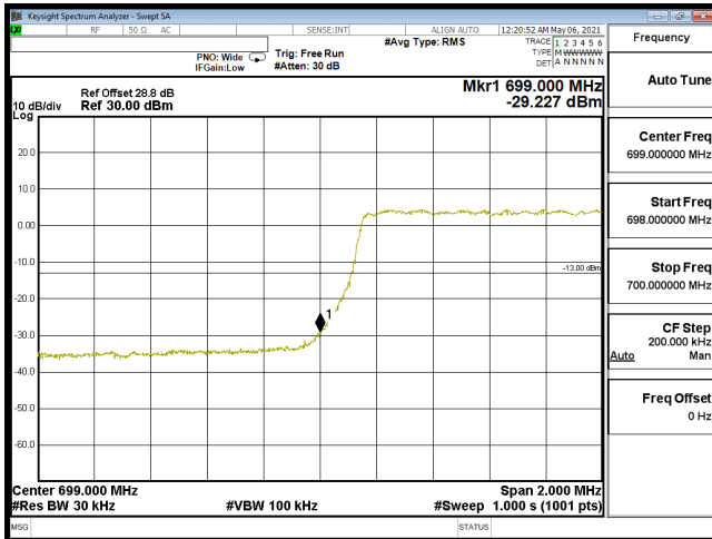
EDGE-B12_3M-CH23025-QPSK(15,0)
