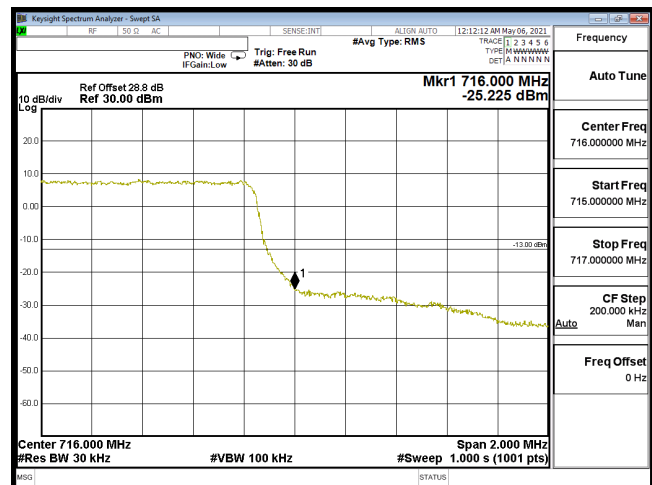
EDGE-B12_1.4M-CH23173-QPSK(6,0)
