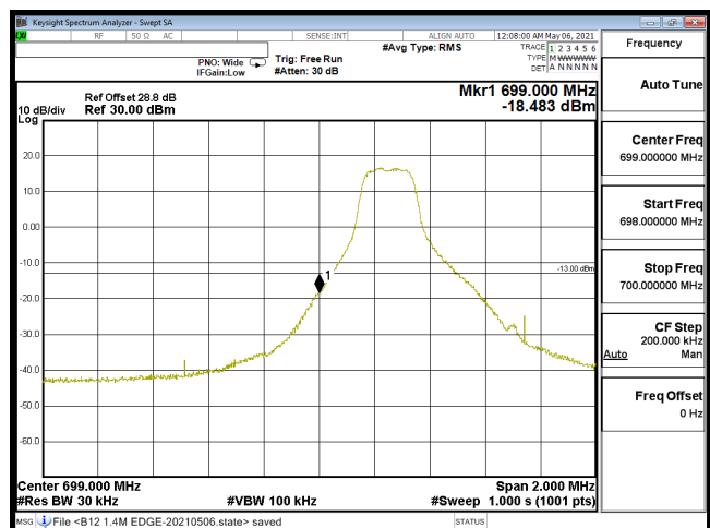
EDGE-B12_1.4M-CH23017-QPSK(1,0)
