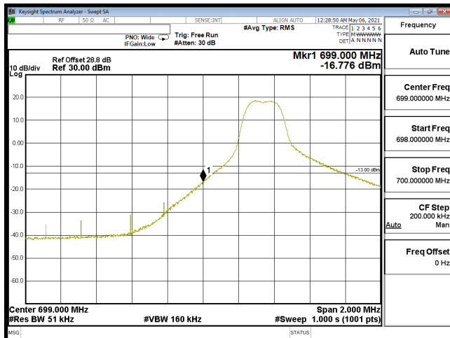
EDGE-B12_5M-CH23035-QPSK(1,0)
