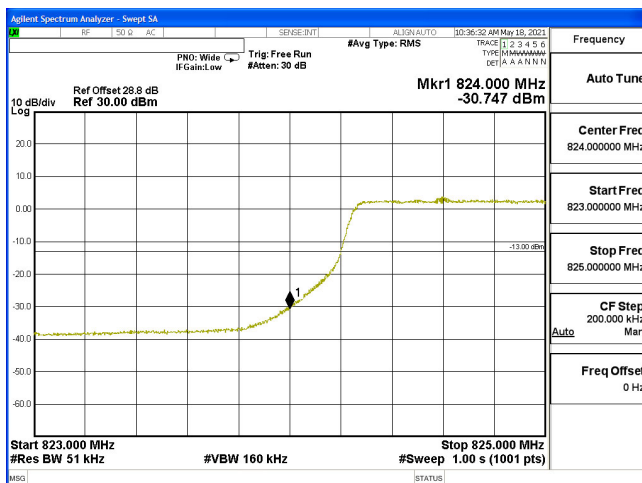
EDGE-B5_5M-CH20425-64QAM(25,0)
