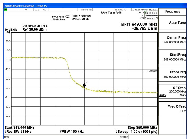
EDGE-B5_5M-CH20625-16QAM(25,0)
