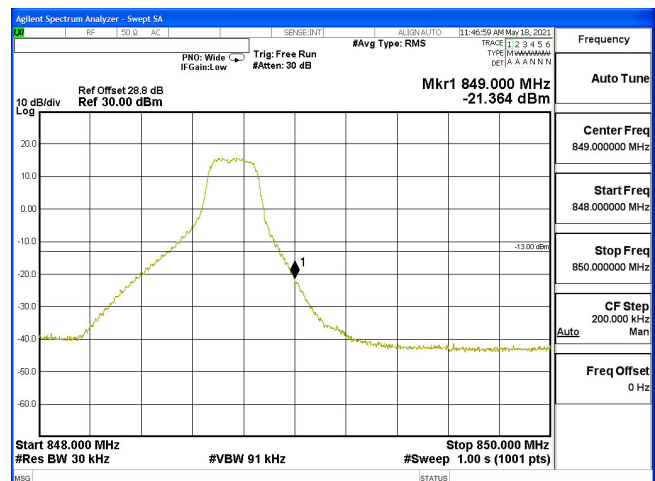
EDGE-B5_3M-CH20635-64QAM(1,14)
