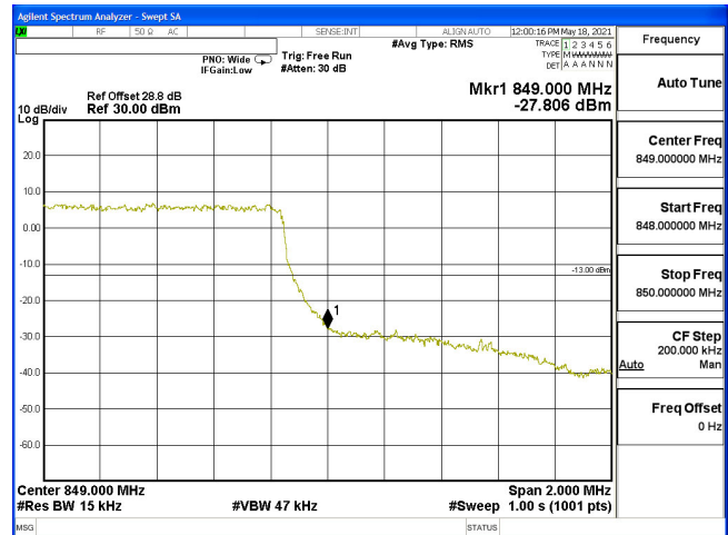
EDGE-B5_1.4M-CH20643-QPSK(6,0)
