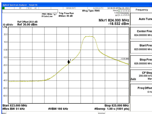
EDGE-B5_5M-CH20425-64QAM(1,0)
