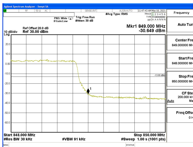
EDGE-B5_3M-CH20635-16QAM(15,0)
