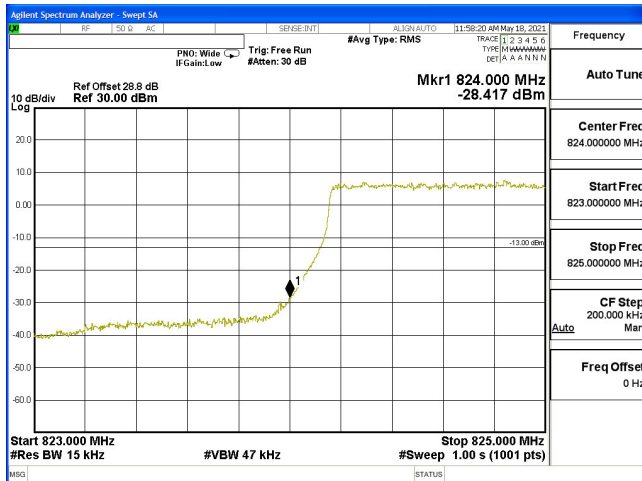
EDGE-B5_1.4M-CH20407-QPSK(6,0)
