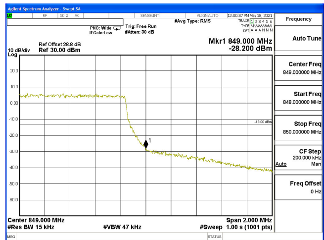
EDGE-B5_1.4M-CH20643-16QAM(6,0)
