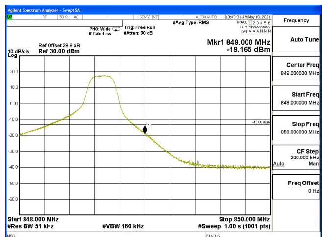
EDGE-B5_5M-CH20625-64QAM(1,24)
