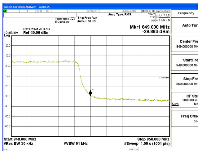
EDGE-B5_3M-CH20635-QPSK(15,0)
