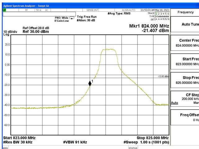
EDGE-B5_3M-CH20415-64QAM(1,0)
