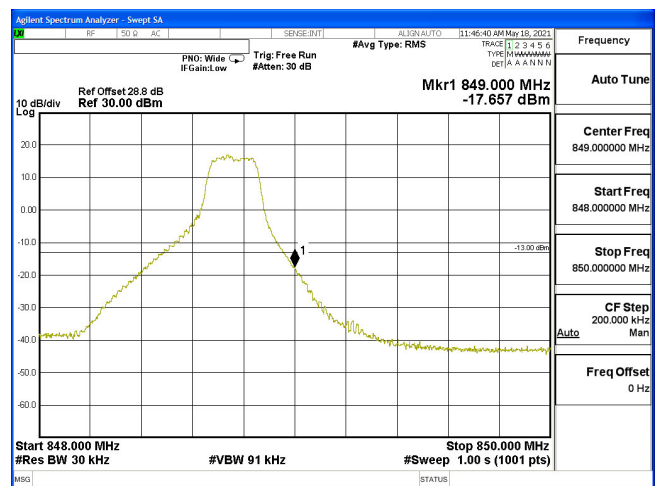
EDGE-B5_3M-CH20635-16QAM(1,14)
