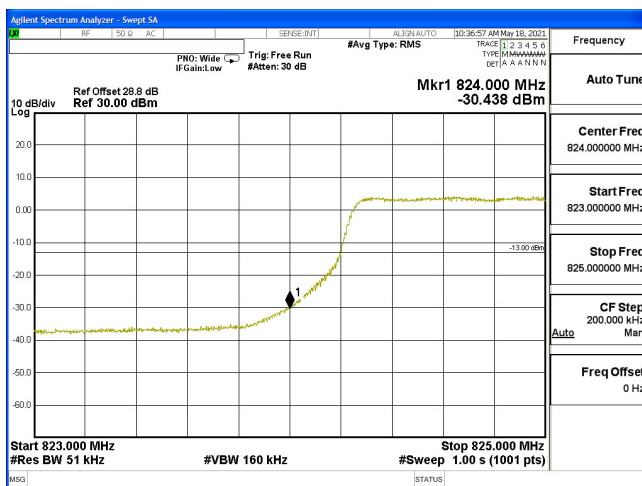
EDGE-B5_5M-CH20425-16QAM(25,0)
