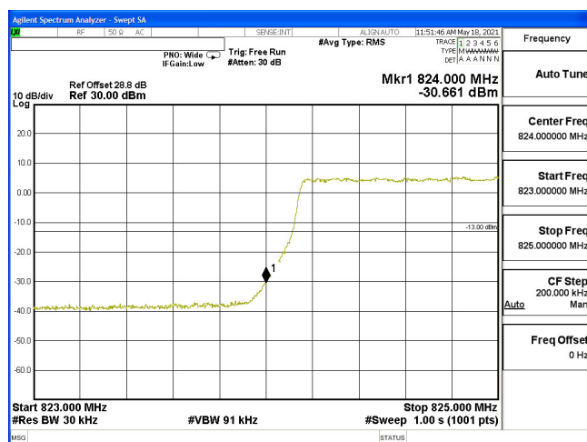
EDGE-B5_3M-CH20415-QPSK(15,0)
