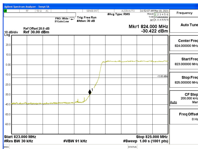
EDGE-B5_3M-CH20415-16QAM(15,0)
