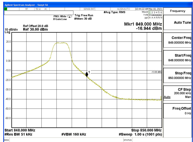
EDGE-B5_5M-CH20625-QPSK(1,24)
