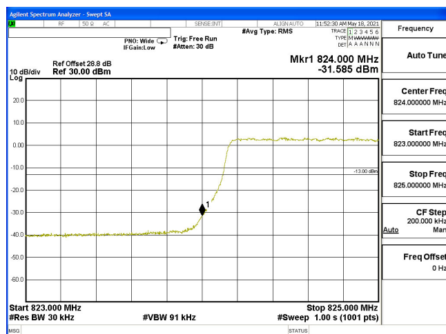
EDGE-B5_3M-CH20415-64QAM(15,0)
