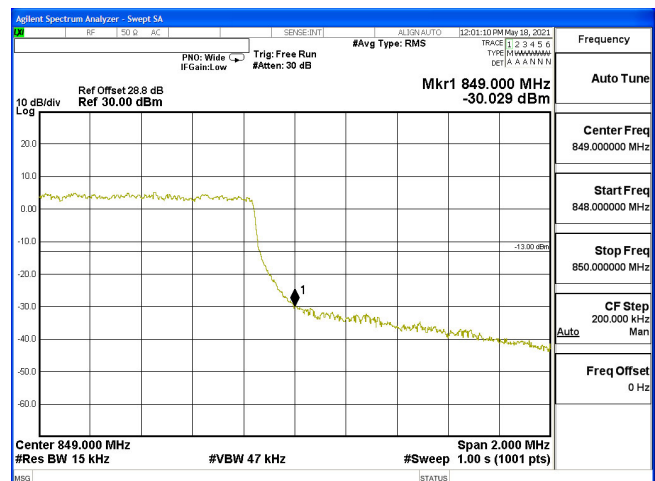
EDGE-B5_1.4M-CH20643-64QAM(6,0)
