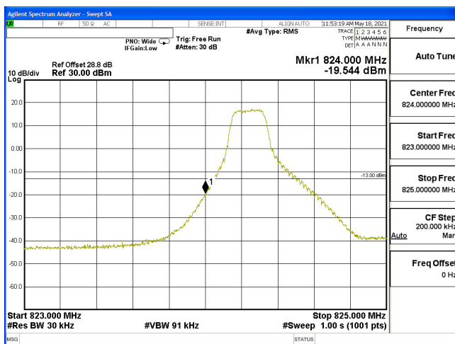
EDGE-B5_3M-CH20415-16QAM(1,0)
