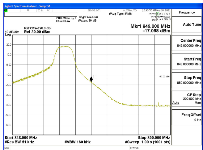
EDGE-B5_5M-CH20625-16QAM(1,24)
