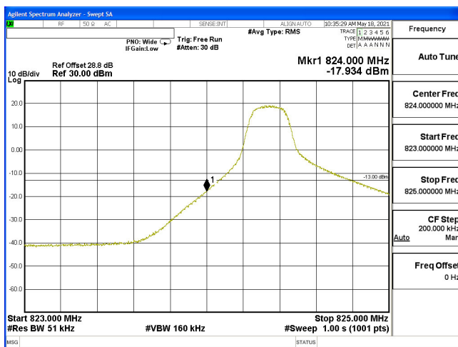
EDGE-B5_5M-CH20425-16QAM(1,0)
