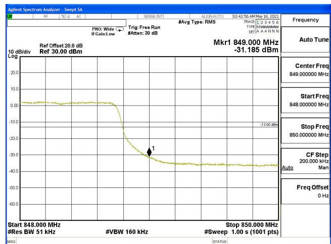
EDGE-B5_5M-CH20625-64QAM(25,0)
