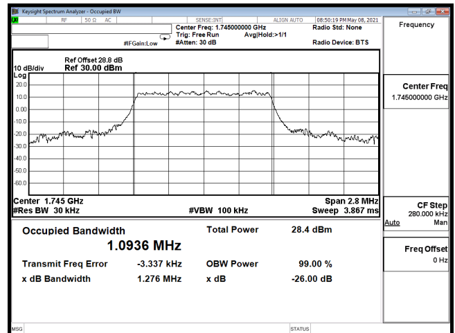
OCC-B66_1.4M-CH132322-64QAM
