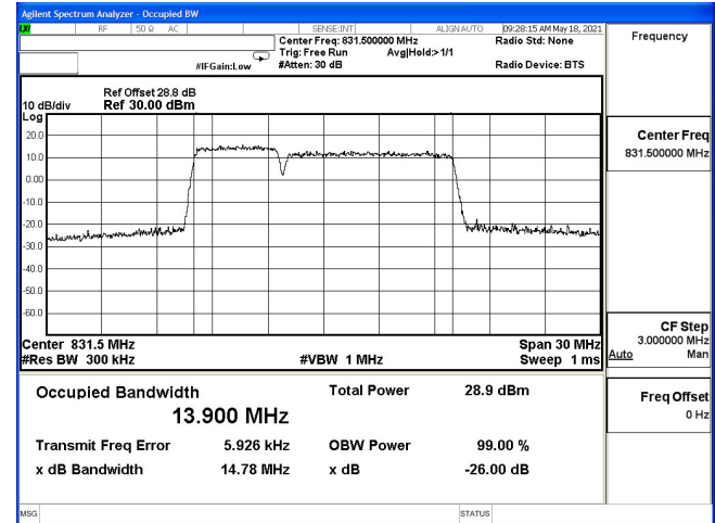
OCC(5M+10M)-2ULCA_5B-16QAM_826.8(25,0)+834(50,0)
