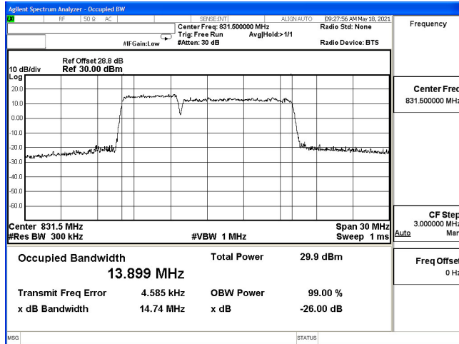
OCC(5M+10M)-2ULCA_5B-QPSK_826.8(25,0)+834(50,0)
