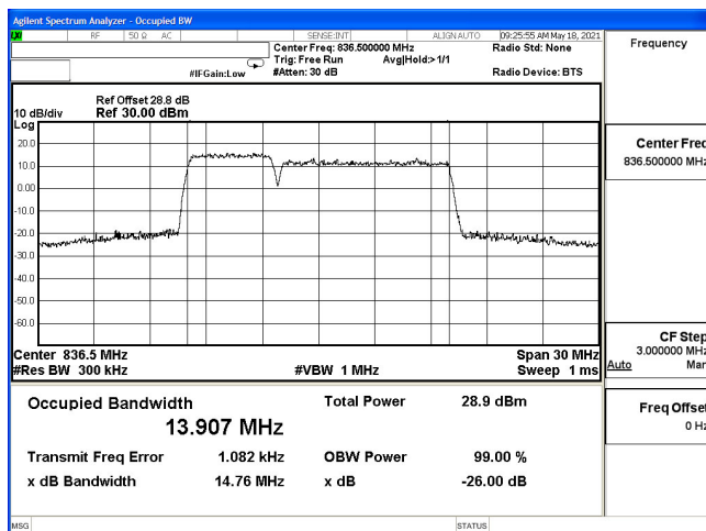
OCC(5M+10M)-2ULCA_5B-16QAM_831.8(25,0)+839(50,0)
