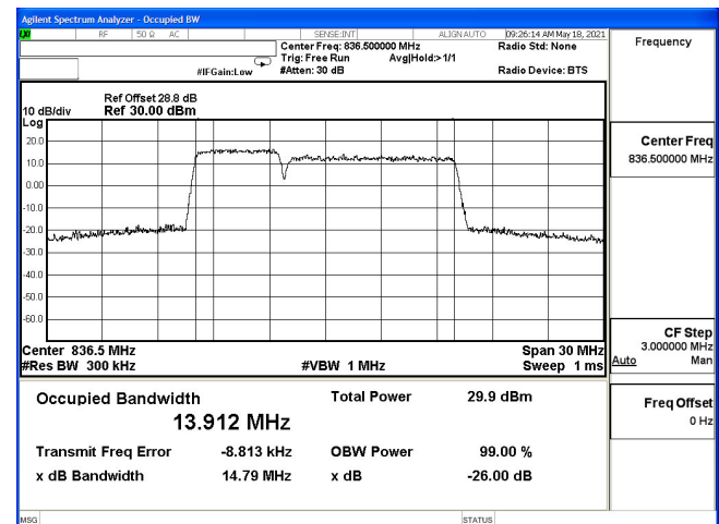
OCC(5M+10M)-2ULCA_5B-QPSK_831.8(25,0)+839(50,0)
