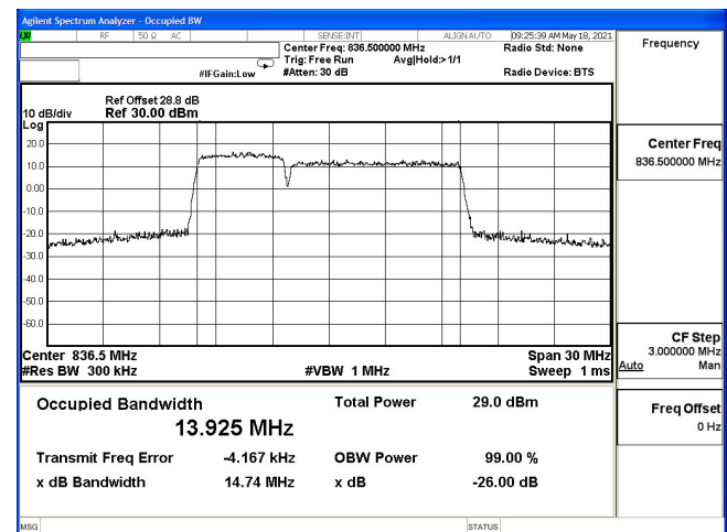
OCC(5M+10M)-2ULCA_5B-64QAM_831.8(25,0)+839(50,0)
