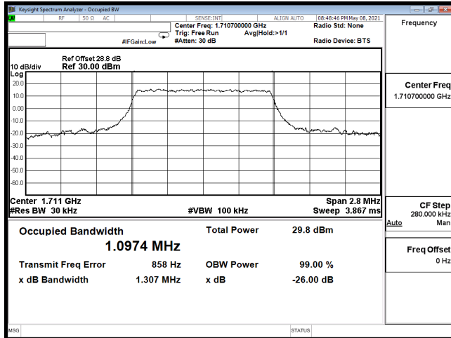
OCC-B66_1.4M-CH131979-QPSK
