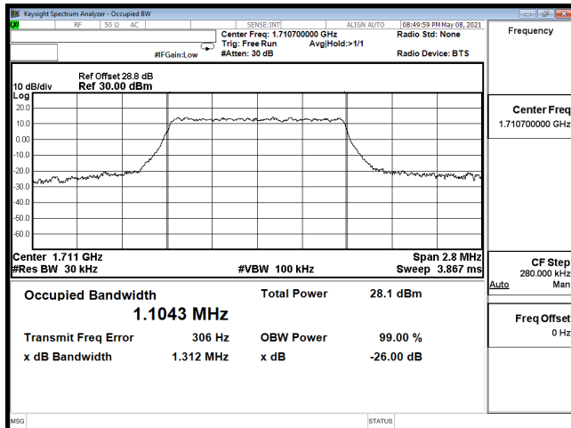
OCC-B66_1.4M-CH131979-64QAM
