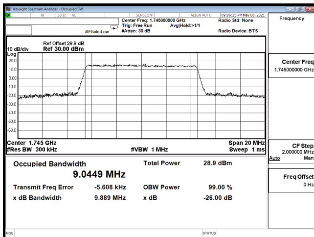
OCC-B66_10M-CH132322-64QAM
