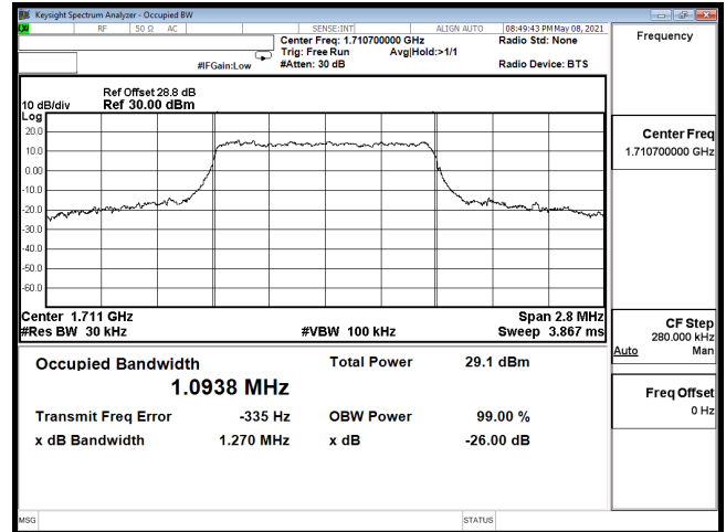
OCC-B66_1.4M-CH131979-16QAM
