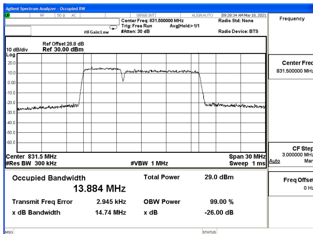
OCC(5M+10M)-2ULCA_5B-64QAM_826.8(25,0)+834(50,0)
