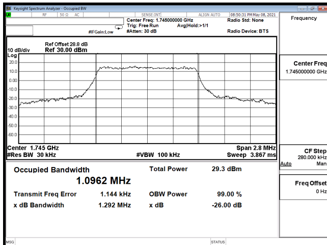
OCC-B66_1.4M-CH132322-16QAM
