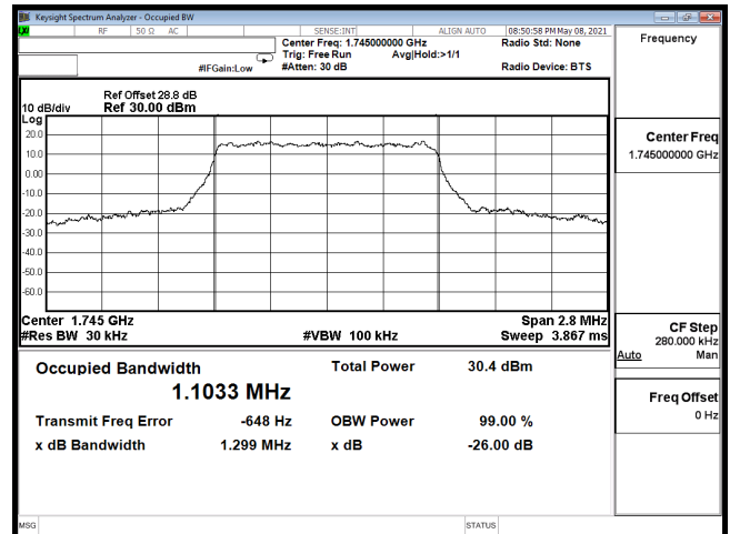
OCC-B66_1.4M-CH132322-QPSK
