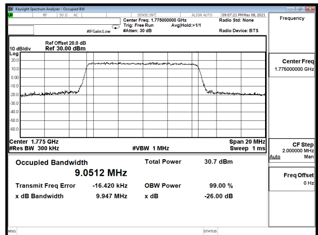
OCC-B66_10M-CH132622-QPSK
