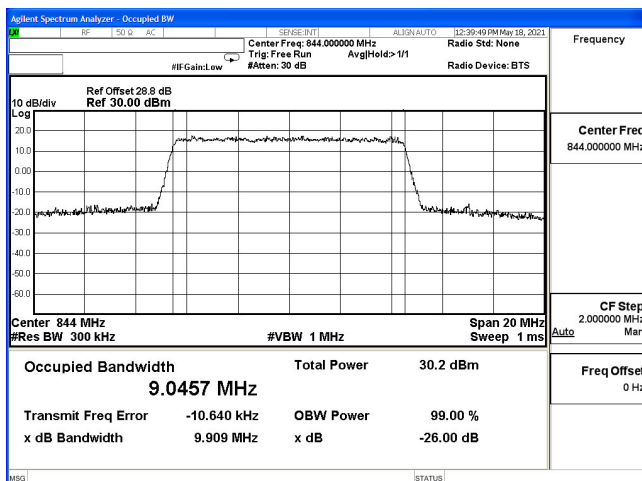
OCC-B5_10M-CH20600-16QAM
