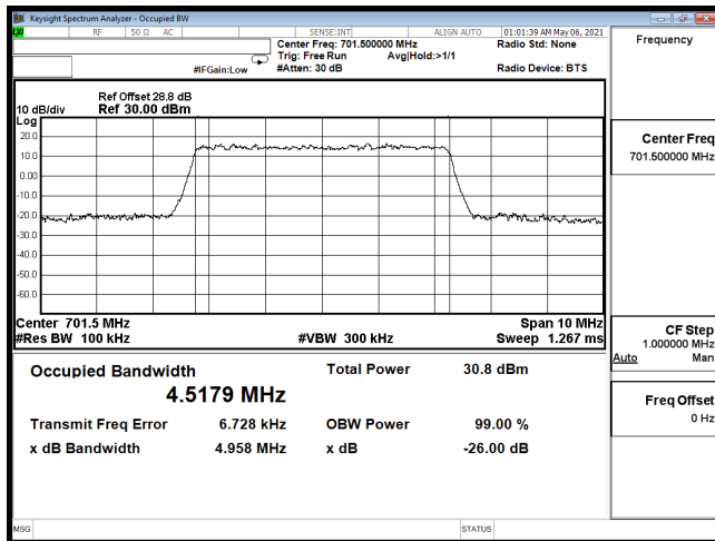
OCC-B12_5M-CH23035-QPSK
