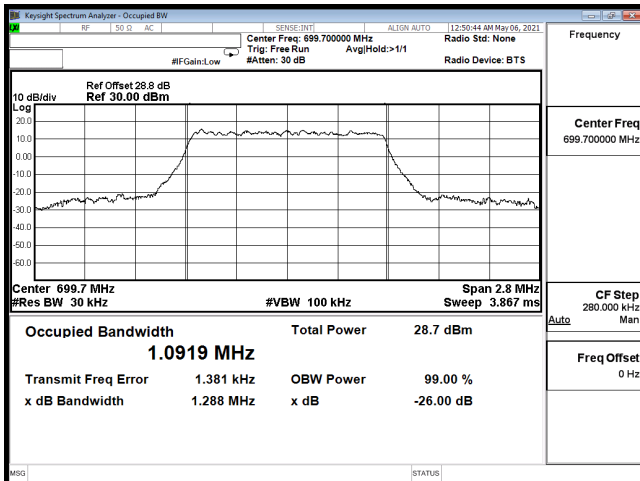
OCC-B12_1.4M-CH23017-64QAM
