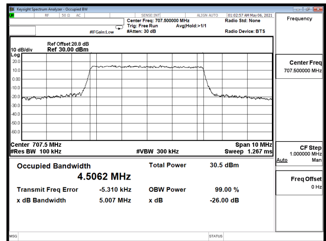
OCC-B12_5M-CH23095-QPSK
