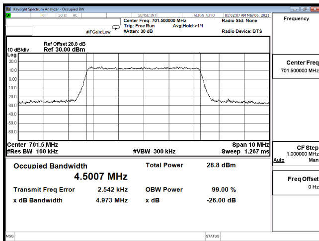
OCC-B12_5M-CH23035-64QAM
