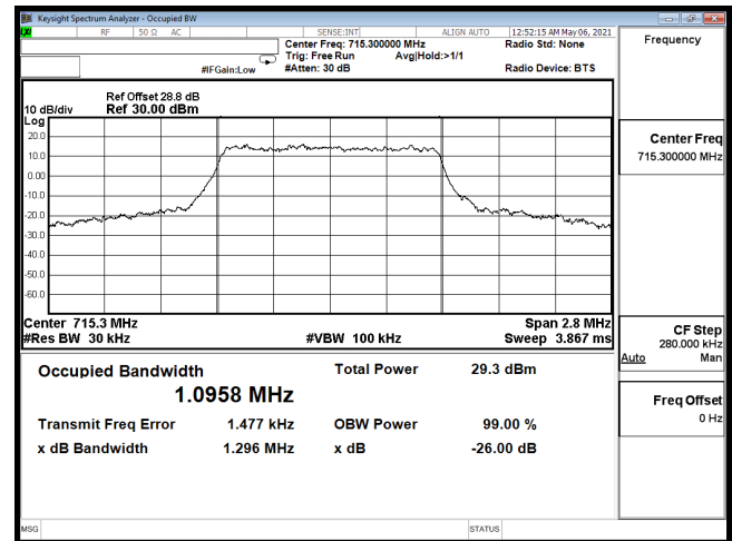
OCC-B12_1.4M-CH23173-16QAM
