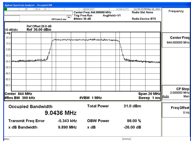
OCC-B5_10M-CH20600-QPSK
