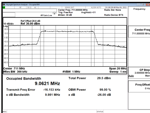
OCC-B12_10M-CH23130-16QAM
