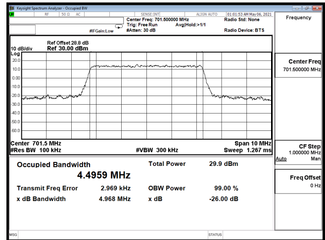
OCC-B12_5M-CH23035-16QAM
