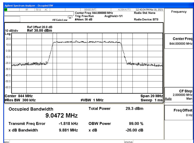
OCC-B5_10M-CH20600-64QAM
