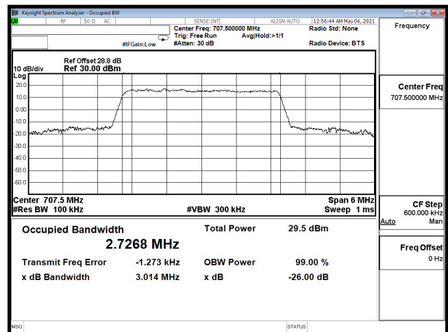
OCC-B12_3M-CH23095-16QAM
