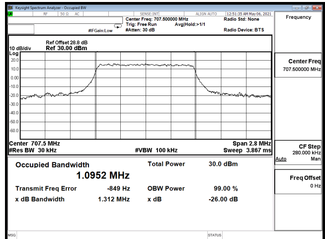
OCC-B12_1.4M-CH23095-QPSK
