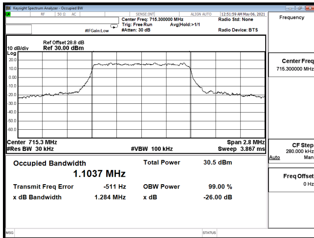
OCC-B12_1.4M-CH23173-QPSK
