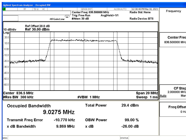
OCC-B5_10M-CH20525-64QAM
