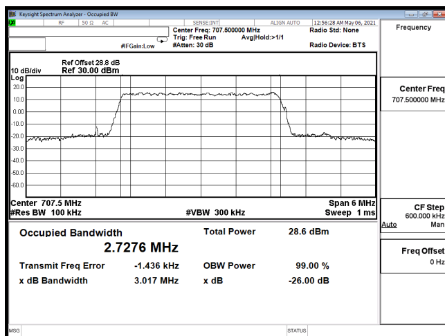
OCC-B12_3M-CH23095-64QAM
