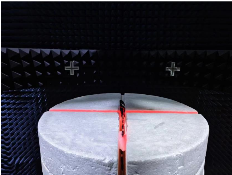
Photo of EUT - ANEPRA5-CAG03-EH
