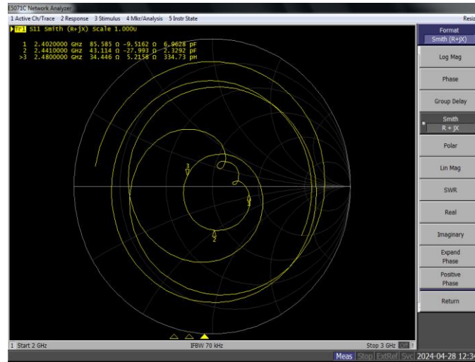
Free Space - ANEPRA5-CAG03-EH (2.4G)
