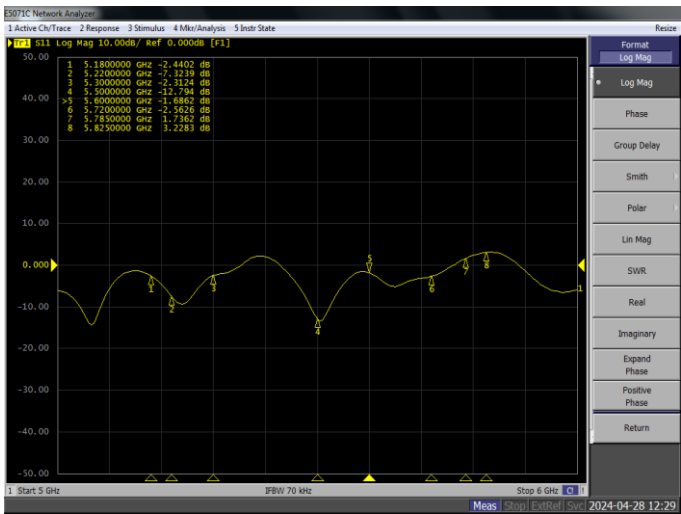
Free Space - ANEPRA5-CAG03-EH (5G)
