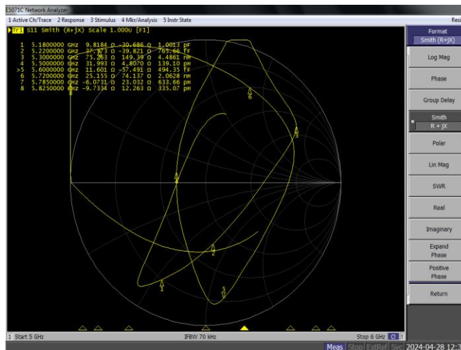
Free Space - ANEPRA5-CAG03-EH (5G)
