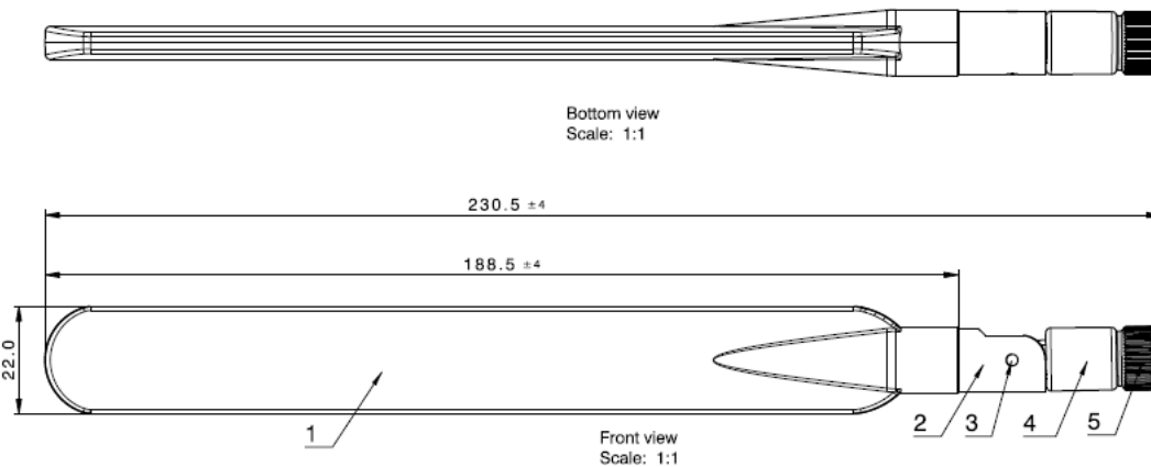
Antenna Dimensions
