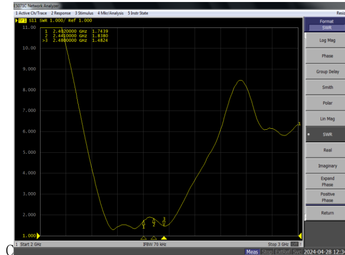
Free Space - ANEPRA5-CAG03-EH (2.4G)
