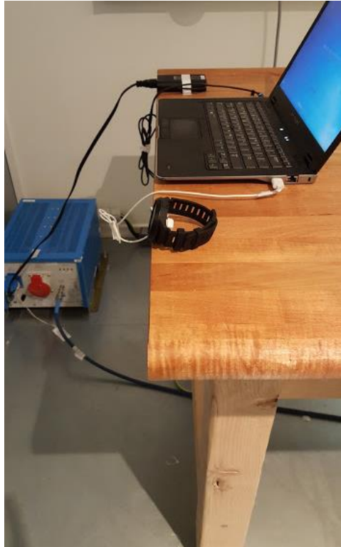
Figure B7 Conducted Emission test set up
