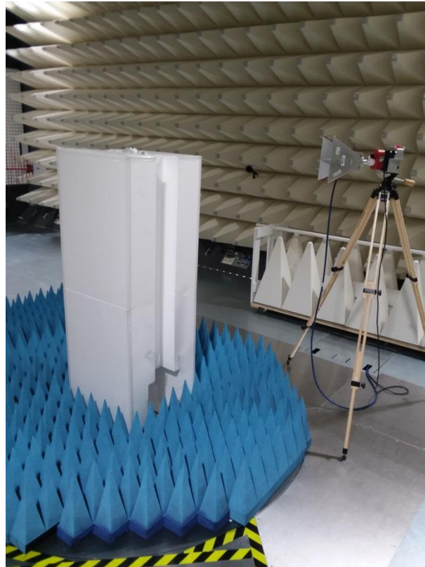
Figure B5. Radiated Emission Setup
