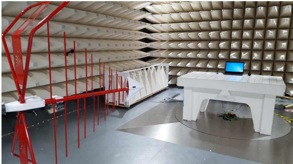
Figure B4. Low Range Radiated Emission test setup using Biconical log antenna
