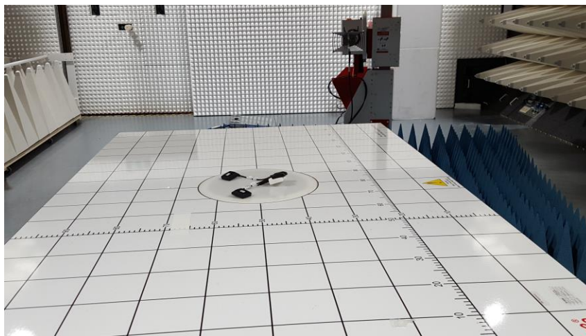
Figure B5. High Range Radiated Emission test setup using Horn antenna
